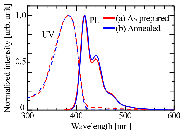
Figure S7. UV and PL spectra of the alternating copolymer in a THF solution; (a) as prepared and (b) after being annealed on a film.
