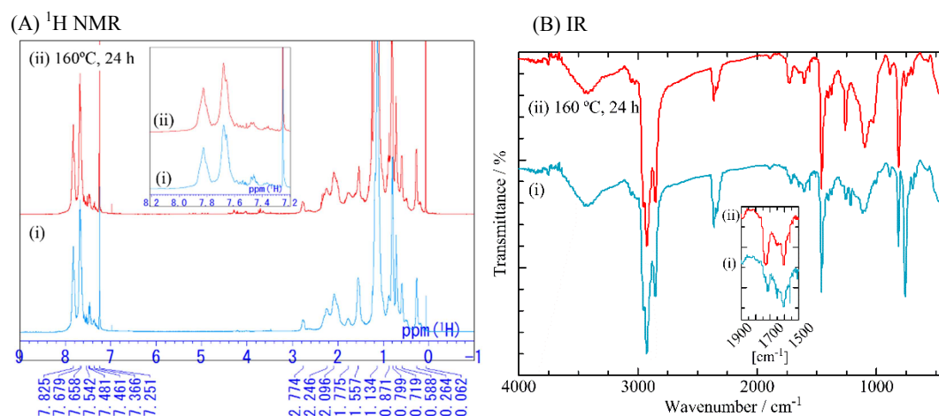
Figure S6. ^1\text{H} NMR (left) and IR (right) spectra of Alt. before (i) and after being annealed (ii). [(thermal annealing) in a film state on a glass plate, 160 °C, 24 h, under air, in the dark; (NMR) in \text{CDCl}_3 , 400 MHz, r.t.; (IR) KBr pellet, r.t.]
