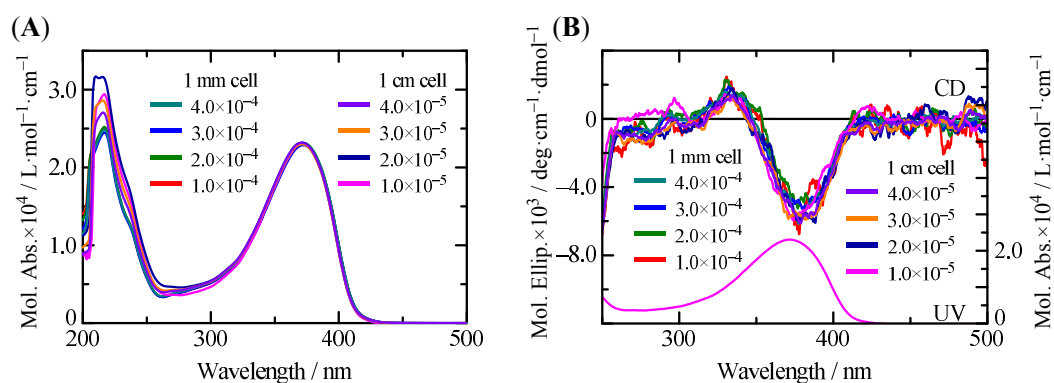
Figure S3. UV spectra (A) and CD spectra with a representative UV spectrum (B) spectra of the alternating copolymer measured at 1.0 \times 10^{-5} M, 2.0 \times 10^{-5} M, 3.0 \times 10^{-5} M, 4.0 \times 10^{-5} M, 1.0 \times 10^{-4} M, 2.0 \times 10^{-4} M, 3.0 \times 10^{-4} M, and 4.0 \times 10^{-4} M in THF.
