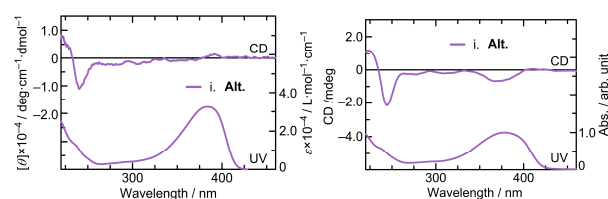
Fig. 1 UV and CD spectra of 9-neomenthyl-9- n -pentylfluorene (NPF) the homopolymer (Homo.) in a THF solution (A), HOMO. in film (B), the random copolymers (Ran.-9/1, -1/1, and -1/9) in a THF solution (C) and in film (D), and the alternating copolymer (Alt.) in a THF solution (E) and in film (F). For solutions; concentration was 1.0 \times 10^{-5} M per residue and cell length was 1 cm. The film CD spectra were obtained by averaging four spectra taken at different orientations of the sample with regard to the incident light beam in order to minimize the effects of linear dichroism (see Fig. S2 for LD and UV spectra of the polymer films).
