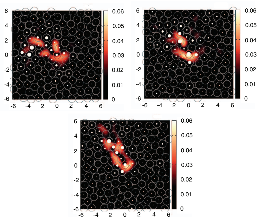
FIG. 12. Samples of the FTLE field ( T = d/v ) superimposed colloidal particles (gray circle). See Sec. III C 2.
