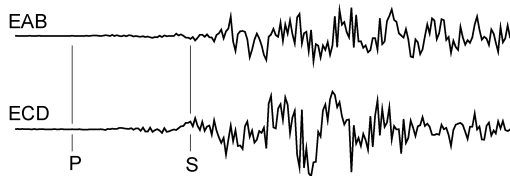
Fig. 3. Strain seismograms of the 1978 and 2005 Miyagi-oki earthquakes in the period of 3 minutes after P wave arrival. Scales of amplitude and time are adjusted to be the same between the two events. Onset times of P and S-waves detected by short-period seismometers are also indicated.
