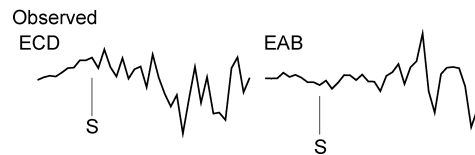
Fig. 4. Enlarged S-wave pulses of the 1978 and 2005 Miyagi-oki earthquakes. Scales of amplitude and time are adjusted to be the same between the two events. Onset time of S-wave detected by short-period seismometers is also indicated.
