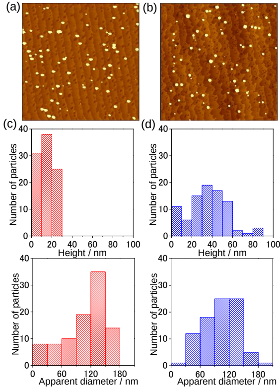
Figure 2. AFM images ( 5 \times 5 \mu\text{m}^2 ) of the Nb-doped \text{TiO}_2(110) surface after electrodeposition at -0.15 V for (a) 1 s and (b) 10 s. (c) and (d) are histograms of apparent diameter and height of the Pt nanoparticles observed in (a) and (b), respectively
