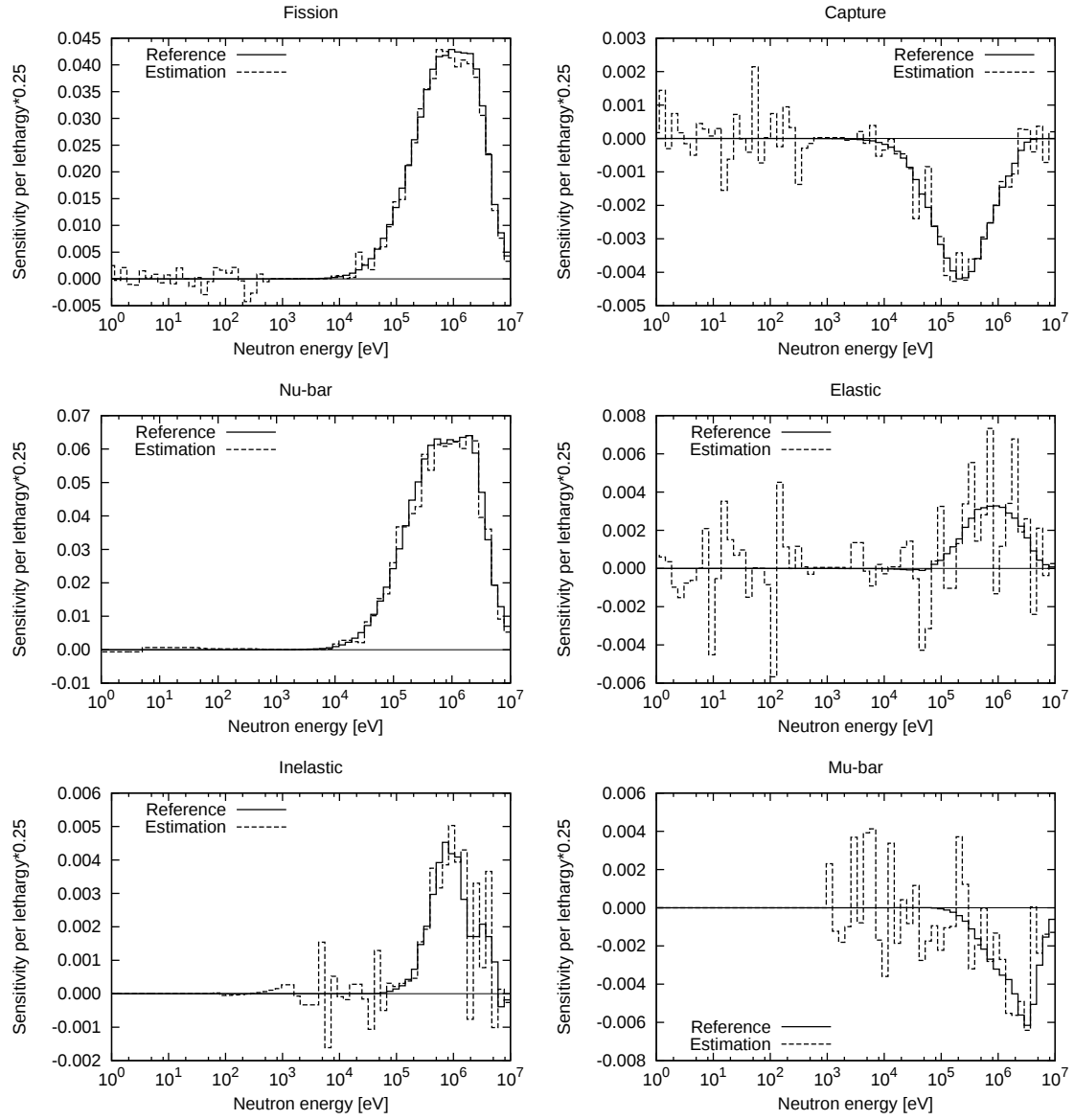
Figure 7: Sensitivity of Flatop-25 criticality to uranium-235 nuclear data. 800 samples are used.
