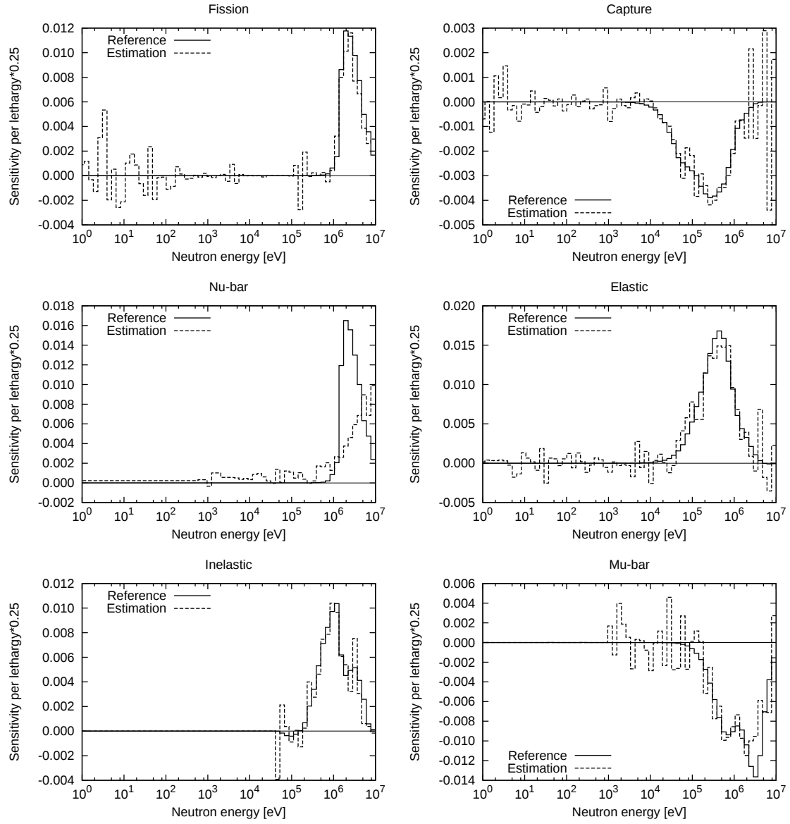
Figure 8: Sensitivity of Flatop-25 criticality to uranium-238 nuclear data. 800 samples are used.
