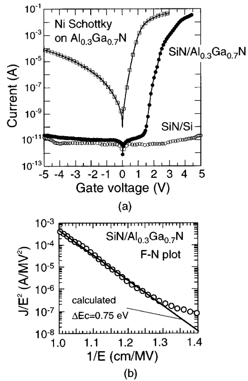
FIG. 13. (a) I - V characteristics of the Al/ \text{SiN}_x / n - \text{Al}_{0.3}\text{Ga}_{0.7}\text{N} structure with the \text{SiN}_x thickness of 20 nm. For comparison, the I - V curves of Ni/ n - \text{Al}_{0.3}\text{Ga}_{0.7}\text{N} and Al/ \text{SiN}_x / n -Si structures are plotted. (b) The plots of \log(J/E^2) vs 1/E for the \text{SiN}_x / n - \text{Al}_{0.3}\text{Ga}_{0.7}\text{N} structure.
