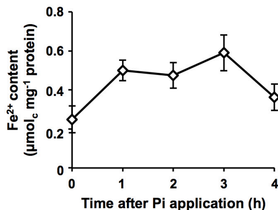
Fig. S3 Dynamics of Fe 2+ during polyphosphate accumulation in extraradical mycelia of Rhizophagus sp. HR1 grown in the mesh bag compartment system. One mM phosphate solution was applied at zero time, and then extraradical mycelia were harvested from the hyphal compartment at 1 h intervals. The levels are expressed as electric charge mol per unit protein. Vertical bars are SE ( n = 3 ). No significant difference in the level was observed among all time points ( P > 0.05 ).
