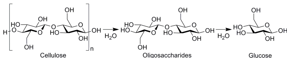
Scheme 1 Hydrolysis of cellulose to glucose.
