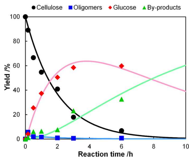
Fig. 3 Time-course of hydrolysis of ball-milled cellulose by \text{H}_2\text{SO}_4 (50 mM) at 418 K. The dots show the experimental data and the lines are the results of kinetic simulations based on eqns (6)–(9).
