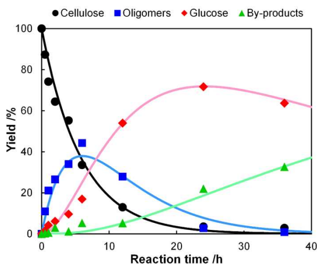
Fig. 2 Time-course of hydrolysis of mix-milled cellulose containing K26 at 418 K. The dots show the experimental data and the lines are the results of kinetic simulations based on eqns (6)–(9).
