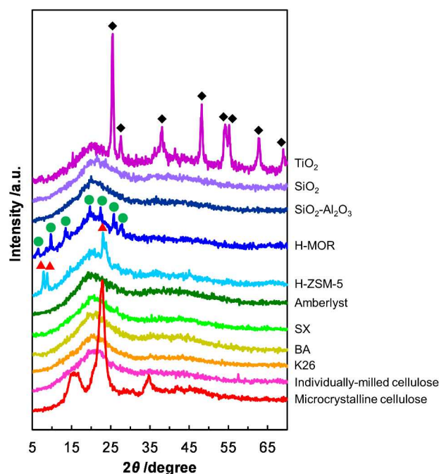
Fig. 1 XRD patterns of mix-milled samples containing cellulose and solid catalysts. The peaks marked with red triangles, green circles and black diamonds are from H-ZSM-5, H-MOR and \text{TiO}_2 , respectively.
