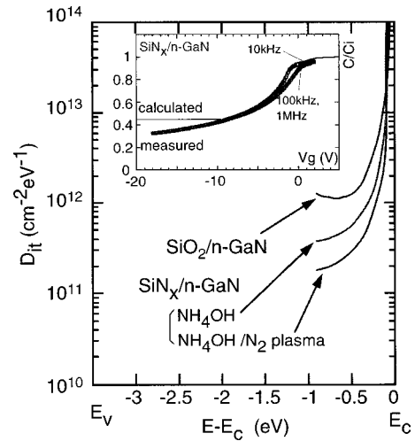
FIG. 8. Distributions of interface state density ( D_{it} ) of the fabricated n\text{-GaN} MIS structures. Typical C-V data obtained from the \text{NH}_4\text{OH}/\text{ECR-N}_2 plasma passivated sample were plotted in the inset.
