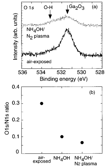
FIG. 3. (a) O 1s spectra of the MOVPE sample after the air exposure and the \text{NH}_4\text{OH}/\text{N}_2 plasma treatments, and (b) change in the XPS integrated intensity of the O 1s level normalized by the N 1s level.
