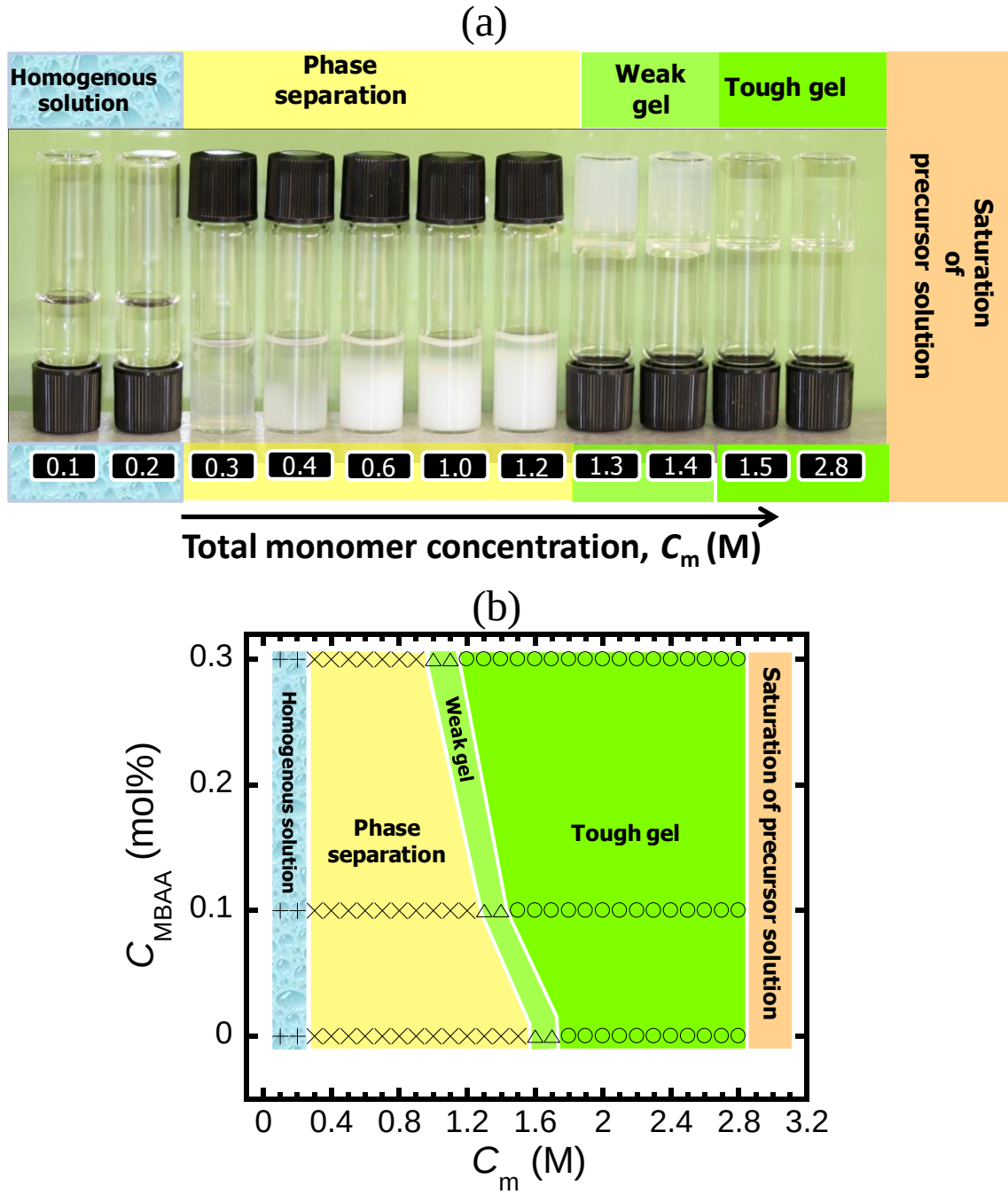
Fig. 2. (a) Photographs of as-prepared samples synthesized at various monomer concentrations ( C_m ) while keeping constant of anionic charge fraction f = 0.52 ( f_{\text{true}}=0.5 ) and chemical cross-linker density C_{\text{MBAA}} = 0.1 mol%. (b) C_m - C_{\text{MBAA}} diagram for f = 0.52 .
