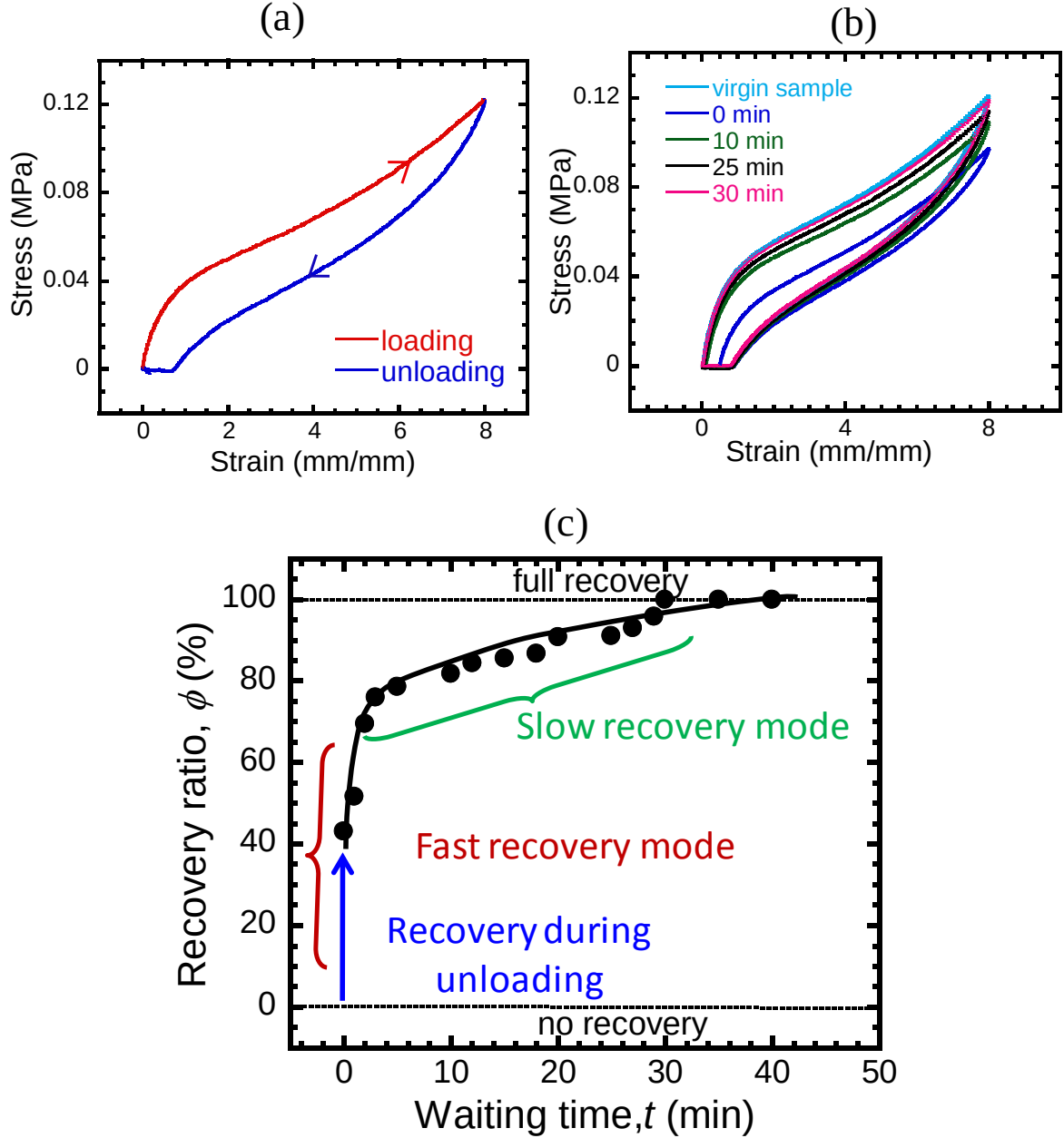
Fig. 6. Hysteresis and self-recovery of the polyampholyte hydrogel P(NaSS-co-DMAEA-Q) 0.5-2.0-0.1. (a) Tensile loading-unloading curves of the gel. (b) Tensile loading-unloading curves of the gel at various waiting times between first cycle and the second cycle. (c) The recovery ratio \phi against the waiting time t . \phi is defined as the area ratio of the hysteresis loop at different waiting times to the hysteresis loop of the virgin sample.
