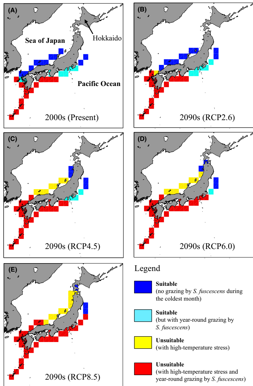
Figure 1. Potential habitats for Ecklonia cava projected using the CMIP5 multimodel mean monthly SSTs in (A) the 2000s and (B–E) the 2090s for RCPs 2.6, 4.5, 6.0, and 8.5, respectively. The results in the 2000s were projected based on a historical simulation for 2000–2005 and the mean of the four RCP simulations for 2006–2009. Blue squares, suitable habitats without high-temperature stress or year-round grazing by S. fuscescens ; light blue squares, suitable habitats without high-temperature stress but with year-round grazing; yellow squares, unsuitable habitats due to high-temperature stress; red squares, unsuitable habitats due to a combination of high-temperature stress and year-round grazing.
