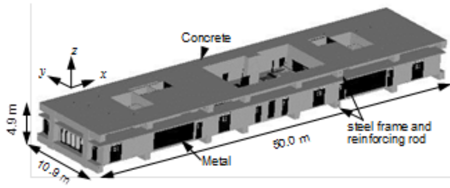
Figure 2.5: Model of Calculation for FDTD simulation (general view).
