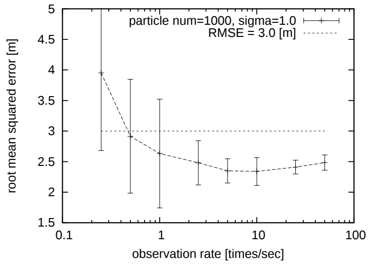
Figure 3.12: RSSI observation transmission vs. positioning accuracy (RMSE).
