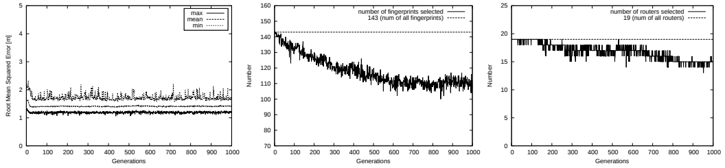
Figure 4.16: Learning curves of GA. All 1 start and using testdata in single room. (left: generation vs. error, center: generation vs. number of selected fingerprints, right: generation vs. number of selected routers)
