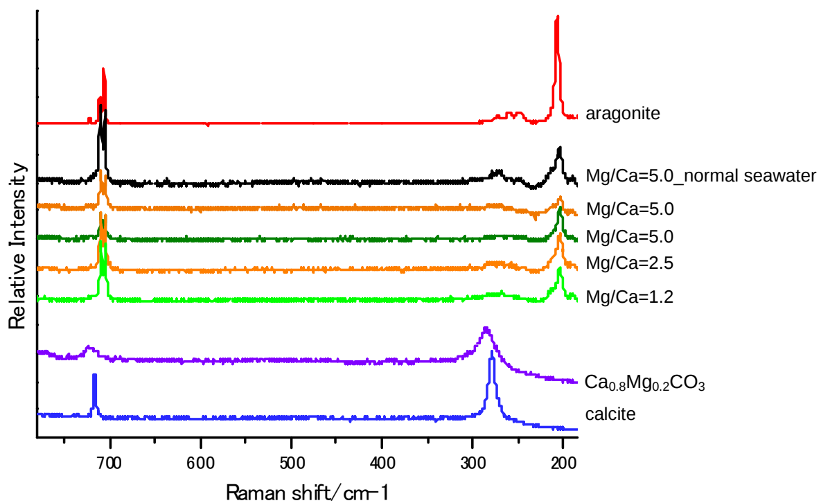
Figure 4-6. Raman patterns of cultured coral skeletons and standard sample, aragonite, calcite, Ca 0.8 Mg 0.2 CO 3 from sponge skeleton. All peaks from cultured coral skeletons seem similar to aragonite.
