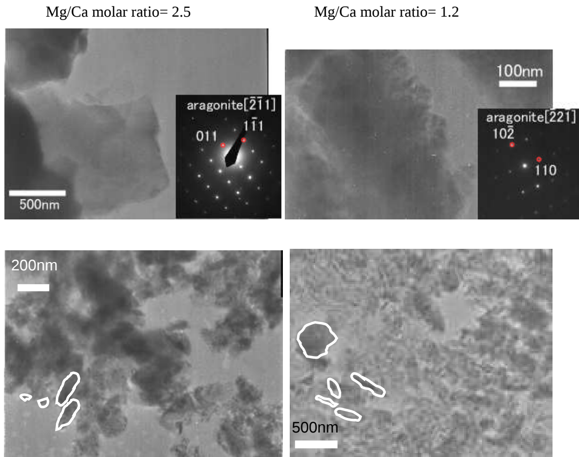
Figure 4-8. TEM photographs from cultured coral skeletons in Mg/Ca molar ratio is 2.5 and 1.2. SEAD patterns indicate the grains are aragonite. Aragonite crystals show needle or granular shape with several micrometer in dimensions.
