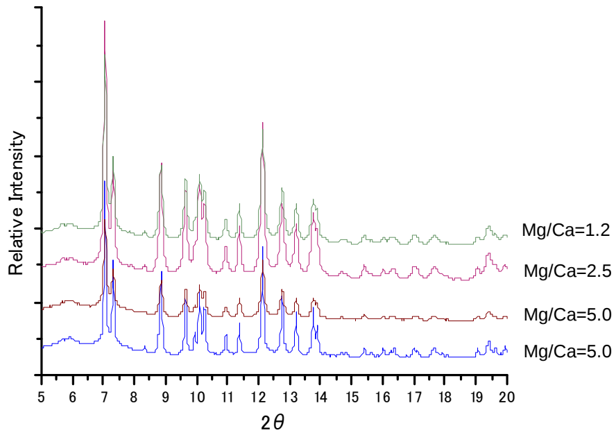
Figure 4-5. X-ray diffraction patterns of cultured coral skeletons. All peaks show aragonite phase.
