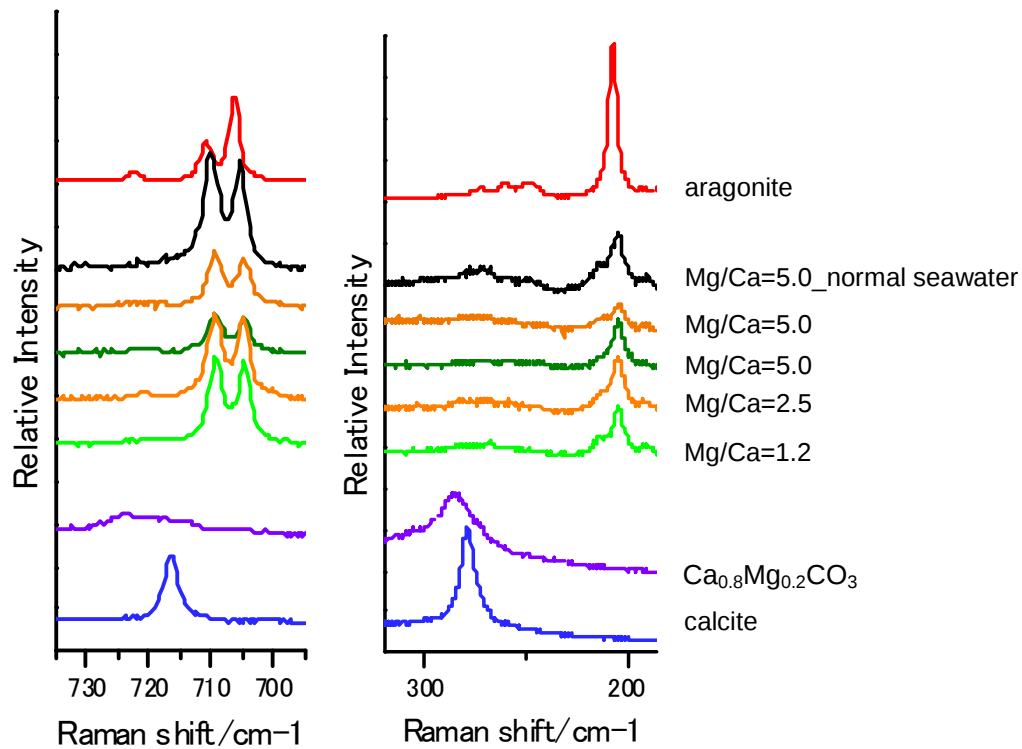
Figure 4-7. Extracts from Fig. 3 which is Raman patterns of cultured coral skeletons and standard sample, aragonite, calcite, \text{Ca}_{0.8}\text{Mg}_{0.2}\text{CO}_3 from sponge skeleton. All peaks from cultured coral skeletons seem similar to aragonite.
