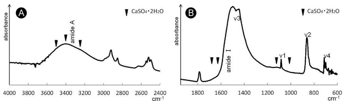
Figure 3-6. Fourier transform infrared spectrometer (FT-IR) profile of the coral fiber area illustrated in Fig. 1. The profiles cover (A) 4000–2400 \text{cm}^{-1} and (B) 2000–600 \text{cm}^{-1} . Mineral aragonite is indicated by prominent absorption at 1490 \text{cm}^{-1} (v3), 1080 \text{cm}^{-1} (v1), 870–875 \text{cm}^{-1} (v2), and 699 \text{cm}^{-1} and 712 \text{cm}^{-1} (v4). There are not major bands for gypsum 673 \text{cm}^{-1} , 1681 \text{cm}^{-1} , 1618 \text{cm}^{-1} and 3549 to 3242 \text{cm}^{-1} having doublet at least, or major bands for anhydrite doublet 676–616 \text{cm}^{-1} .
