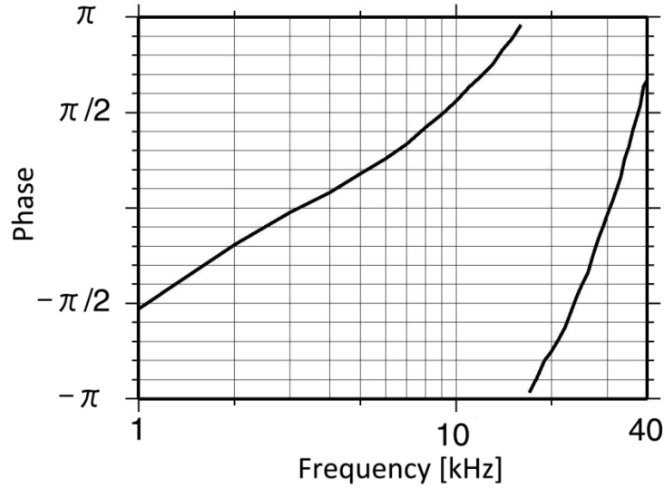
Figure 2.7. Frequency characteristic of phase including main-amplifier and pre-amplifier.
