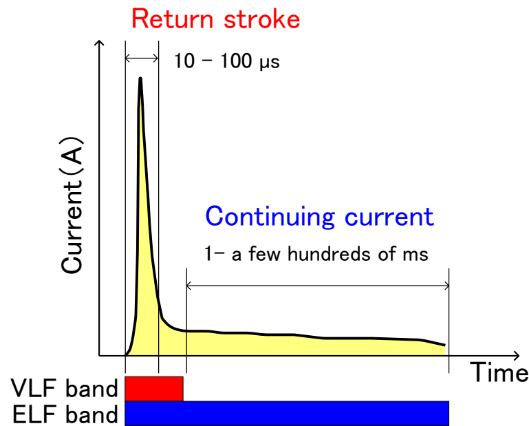
Figure 3.1. Schematic diagram of lightning current.
