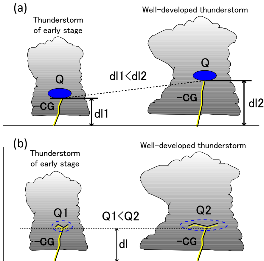
Figure 4.22. Schematic diagram of inferred relationship between the thunderstorm evolution and distribution of electrical charges.
