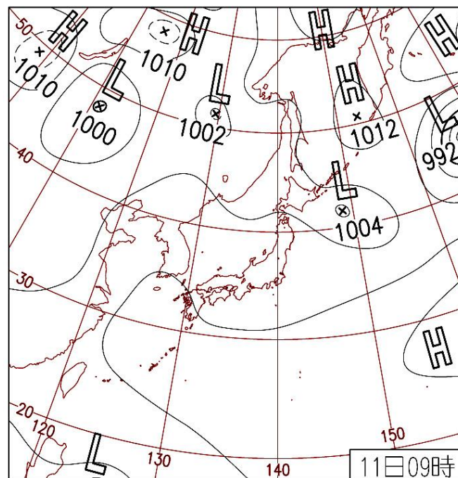
Figure 4.14. Surface weather chart at 09 h (JST), August 11, 2013.
