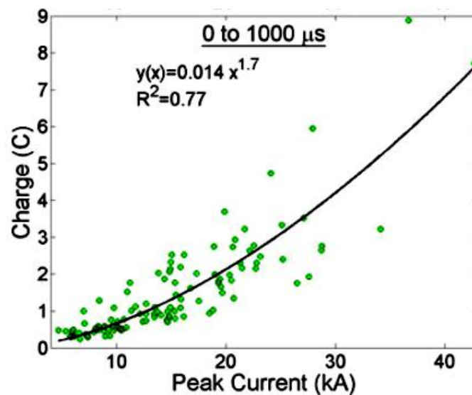
Figure 3.32. Charge with a duration of 1 ms versus peak current in rocket-triggered lightning in Florida [Schoene et al., 2010].
