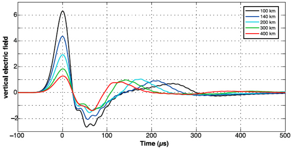
Figure 3.2. Simulated vertical electric field waveform in the VLF range at different distance. The reflection altitude is assumed at 73 km, daytime [Haddad et al. , 2012].
