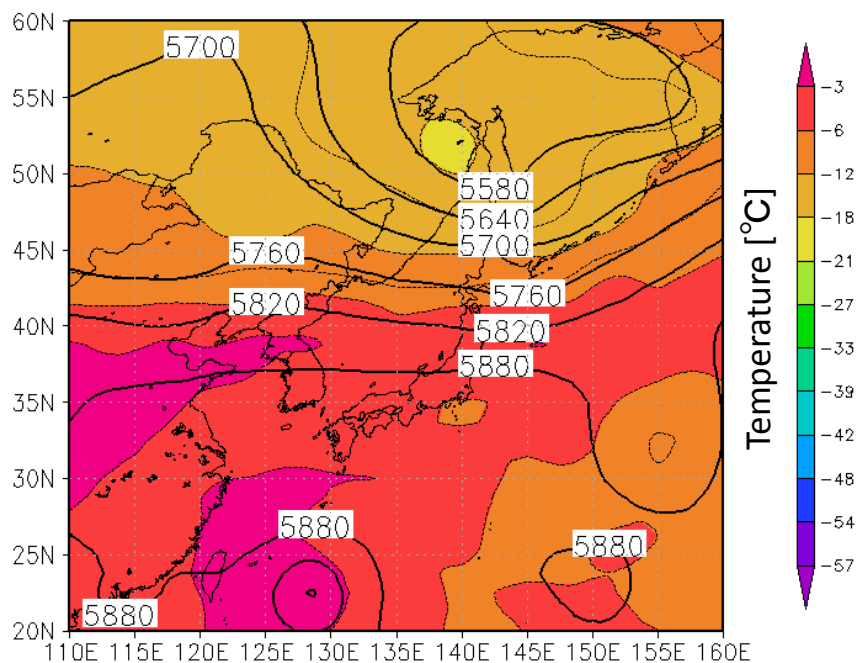
Figure 4.3. 500-hPa level upper weather chart at 21 h (JST), July 11, 2013. The black line is isohypse, color contour is an air temperature at 500 hPa at isobaric surface.
