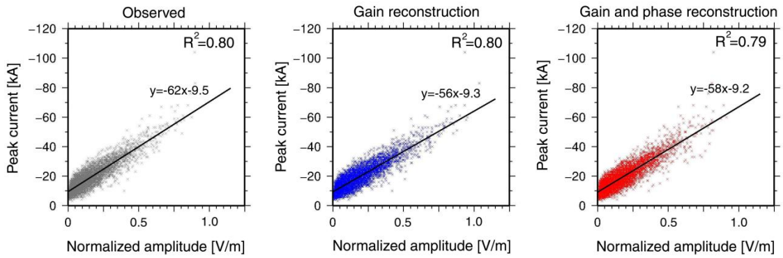
Figure 3.9. Three scatter plots of the normalized amplitude ( V_n ) versus the peak current of JLDN data ( I_{peak} ) in the case of -CG. Left panel: observed E-field, center panel: gain reconstructed E-field, right panel: gain and phase reconstructed E-field.
