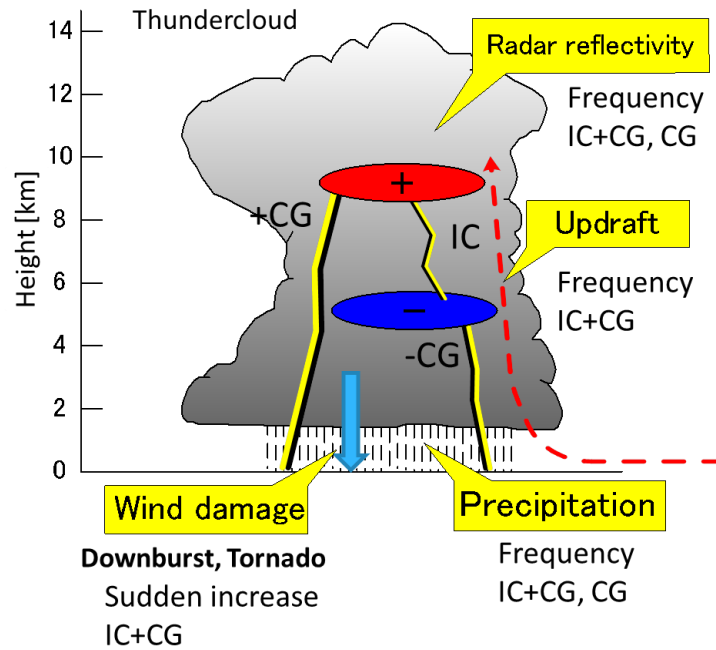
Figure 1.3 Schematic diagram of relationship between atmospheric parameters and lightning activity.
