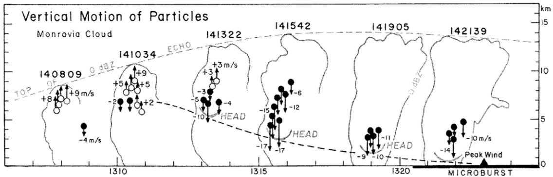
Figure 4.23. Time history of the vertical motion of the largest most reflective precipitation particles during the evolution of the downburst-producing downdraft [Fujita, 1992].
