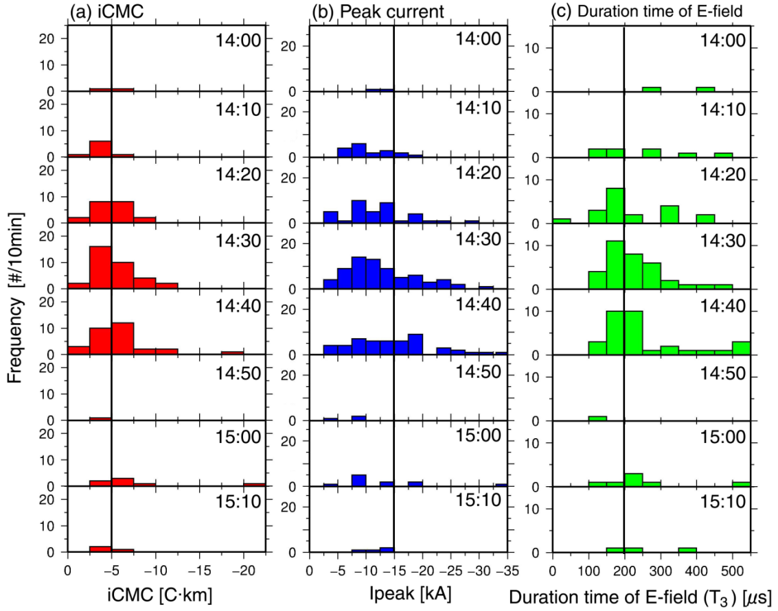
Figure 4.8. Time variation of frequency distribution of (a) iCMC, (b) peak current and (c) duration time of electric field ( T_3 ) on July 11, 2013 from 14:00 to 15:10 (JST).
