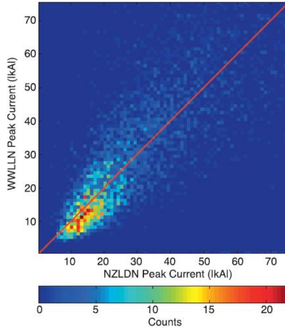
Figure 3.28. WWLLN peak current vs NZLDN return-stroke peak current for three time periods in 2009 using 5260 matches [Hutchins et al. , 2012].
