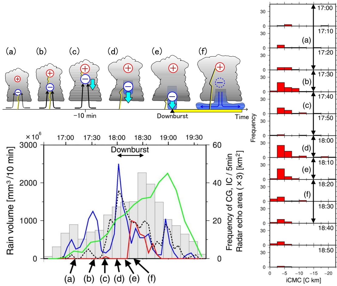
Figure 4.25. Stages (a)~(f) shown in Figure 4.24 superimposed on Figure 4.19 (left panel) and on Figure 4.21 (a) (right panel), respectively.
