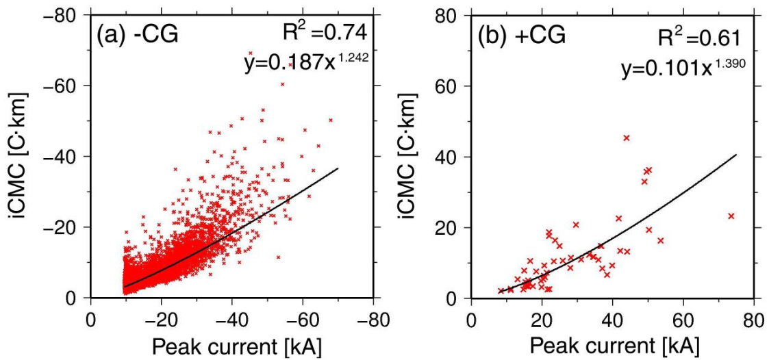
Figure 3.25. Scatter plot of iCMC [C·km] versus estimated peak current [kA]. (a) negative CG, (b) positive CG.
