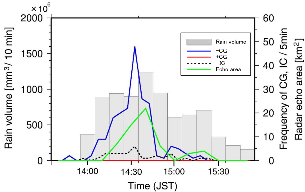
Figure 4.6. Evolution of the rain volume, area of echo height more than 12 km and lightning flash rate on July 11, 2013 from 13:50 to 15:50 (JST).
