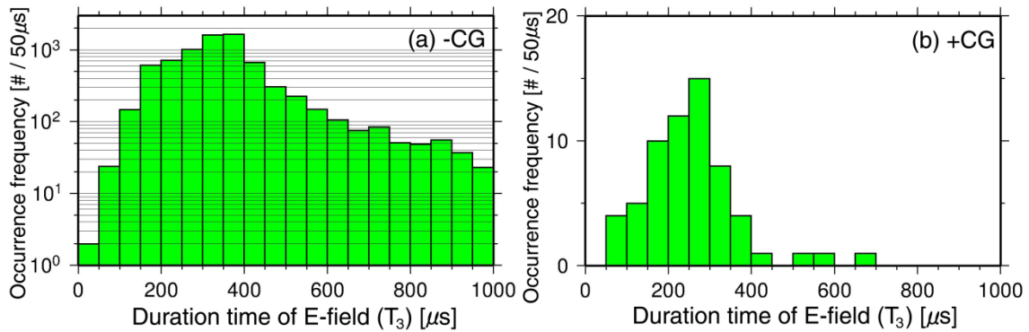
Figure 3.24. Occurrence frequency of duration time of electric field ( T_3 ). (a) negative CG, (b) positive CG.
