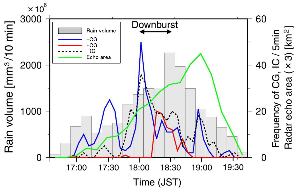
Figure 4.19. Evolution of the rain volume, echo top area and lightning flash rate on August 11, 2013 from 16:40 to 19:10 (JST).
