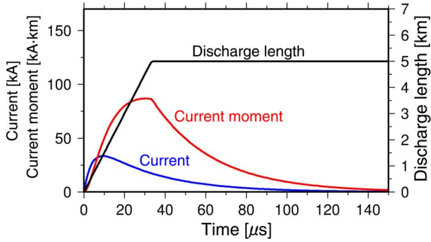
Figure 3.16. Relationship between the discharge length and the current moment.
