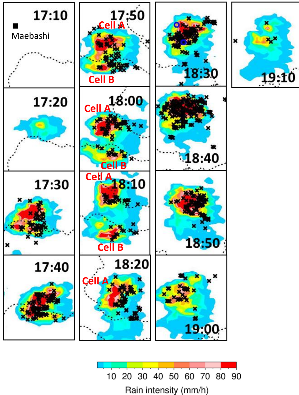
Figure 4.10. Evolution of the precipitation area on July 11, 2013 from 17:10 to 19:10 (JST). The CG lightning flash location during a 10 min period centered on the radar time are plotted. The black cross indicates a negative CG. The blue circle indicates a positive CG.
