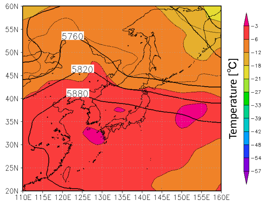
Figure 4.16. 500-hPa level upper weather chart at 09 h (JST), August 11, 2013. The black line is isohypse, color contour is an air temperature at 500 hPa at isobaric surface.
