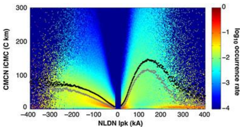
Figure 3.33. Normalized scatter density plot of iCMC versus NLDN peak current ( I_{pk} ) for 13.1 million NLDN-identified CG strokes. Each vertical slice denotes the probability distribution function of iCMC (on a logarithmic color scale) for the given value of I_{pk} , and the mean and median iCMC for each value of I_{pk} are marked with black and gray dots, respectively [Cummer et al. , 2013].
