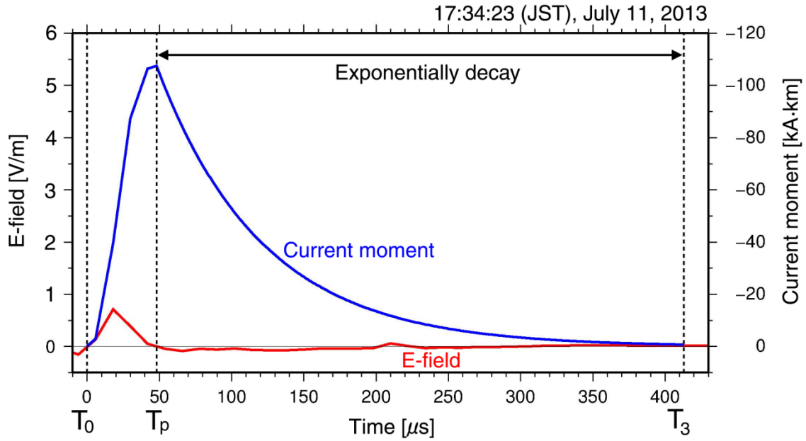
Figure 3.19. Example of conversion from the relative current moment to the absolute value of current moment between T_0 and T_3 on 17:34:23 (JST), July 11, 2013.
