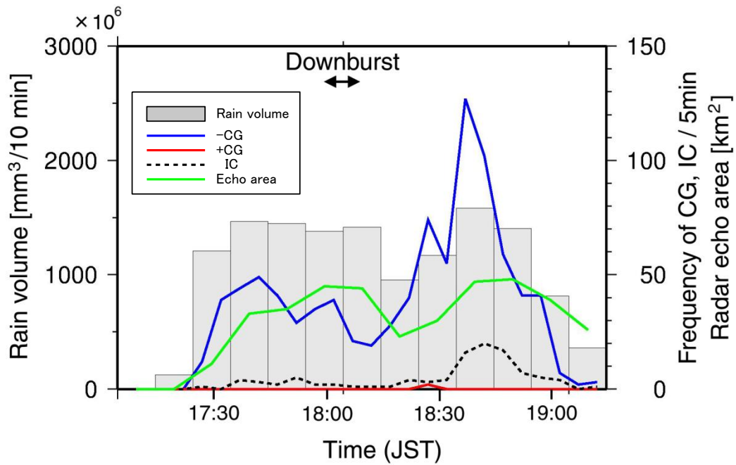
Figure 4.11. Evolution of the rain volume, area of echo height more than 12 km and lightning flash rate on July 11, 2013 from 16:40 to 19:10 (JST).
