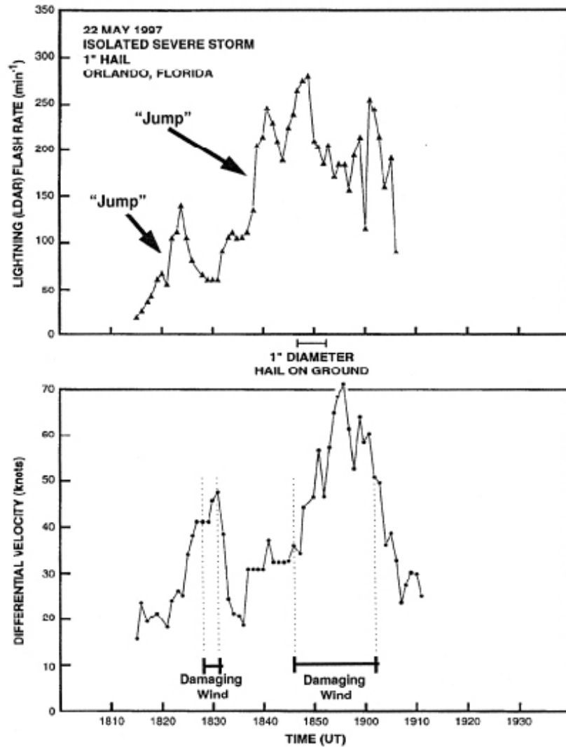
Figure 1.5. May 22, 1997 hailstorm with severe microburst near Orlando. (a) History of total lightning flash rate, and (b) history of differential radial Doppler velocity at the surface [Williams et al. , 1999].
