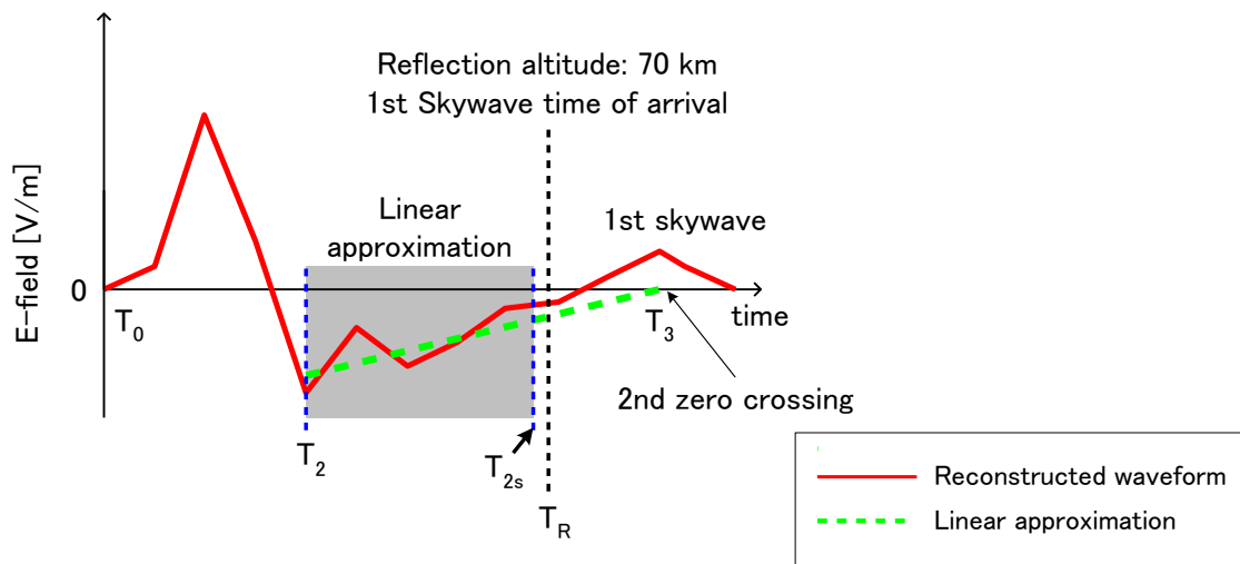
Figure 3.11. Schematic diagram of removing the first skywave from the reconstructed waveform.
