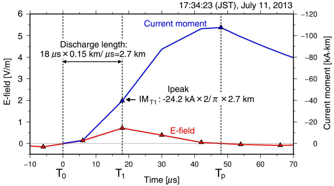
Figure 3.18. Example of conversion from the relative current moment to the absolute value of current moment between T_0 and T_p on 17:34:23 (JST), July 11, 2013. The red line is the reconstructed electric field waveform, and the blue line is the converted current moment. The symbols of red triangle are the data points.
