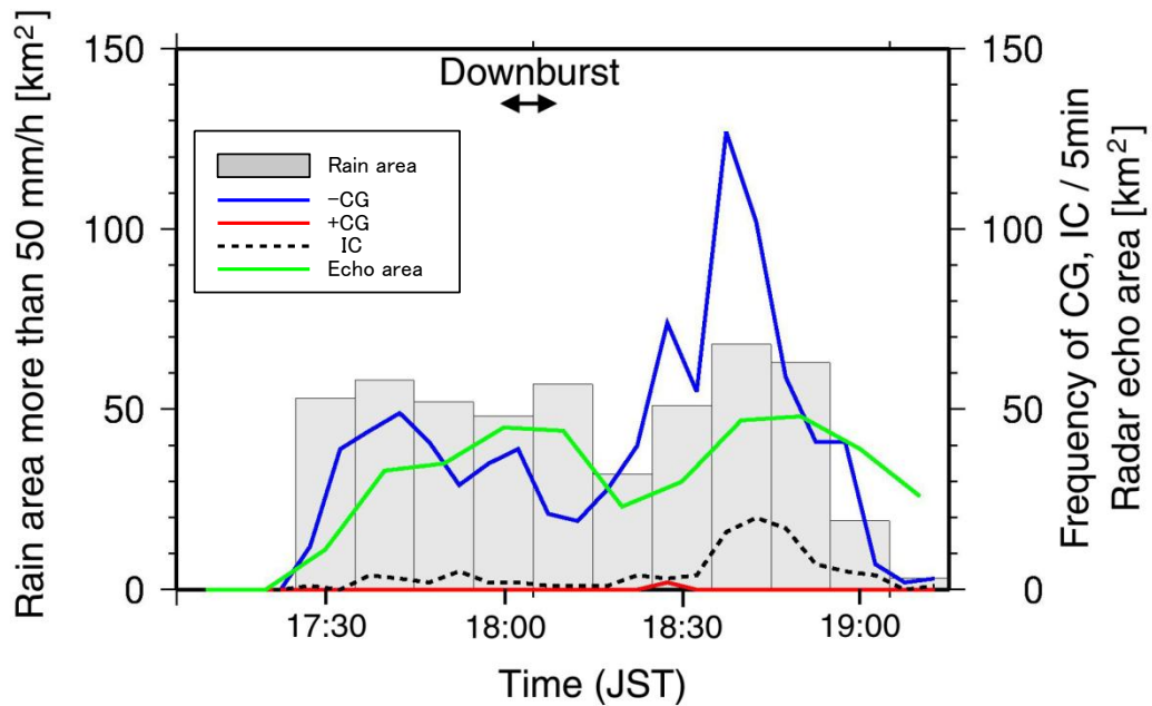
Figure 4.12. Evolution of the rain area more than 50 mm/h, area of echo height more than 12 km and lightning flash rate on July 11, 2013 from 17:10 to 19:10 (JST).
