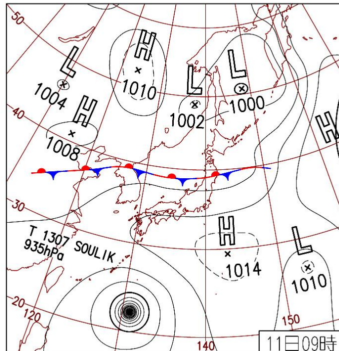
Figure 4.1. Surface weather chart at 09 h (JST), July 11, 2013.
