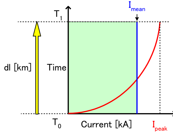
Figure 3.17. Relationship between the peak current and the absolute value of current moment at the time of T_1 ( T_{I_{peak}} ).
