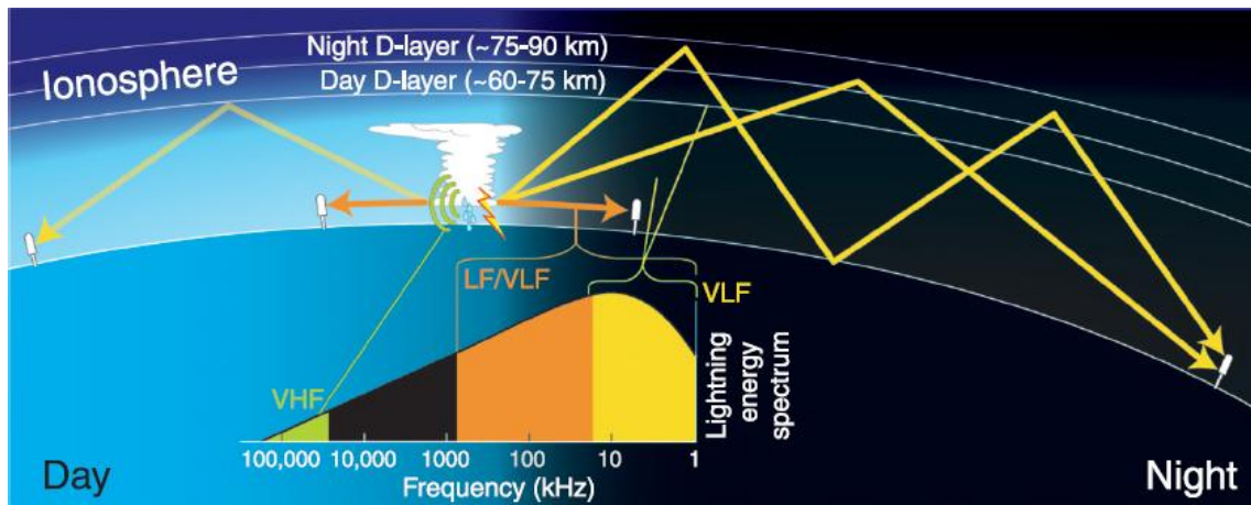
Figure 1.8 Schematic diagram of the earth-ionosphere waveguide, which allows VLF (3 kHz – 30 kHz) emissions from thunderstorms (sferics) to propagate thousands of kilometers through reflection [Pessi et al. , 2009].
