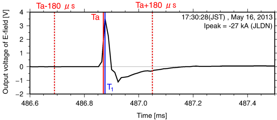
Figure 3.6. Example of identified waveform of the electric field of Yamanashi site.
