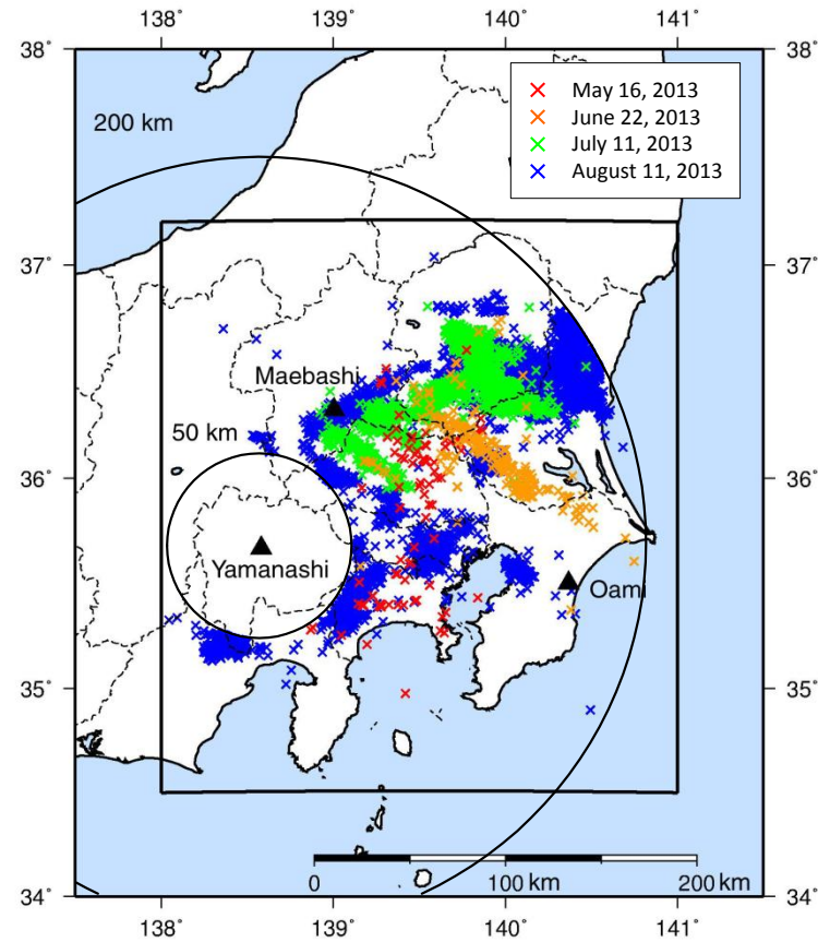
Figure 3.3. Area of analysis and lightning location of each day.
