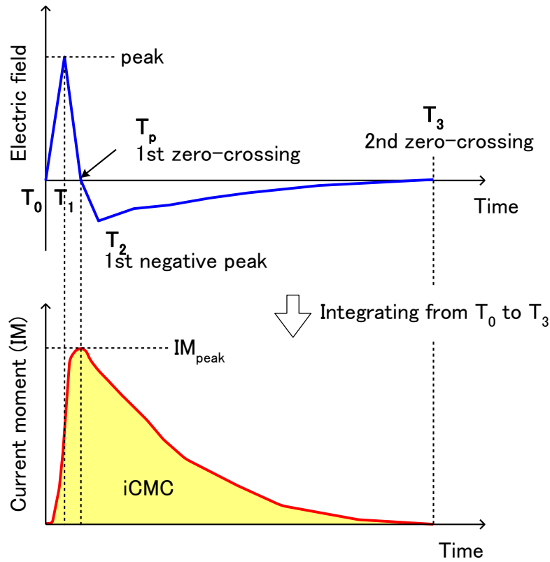
Figure 3.4. Schematic diagram of a concept of iCMC estimation.
