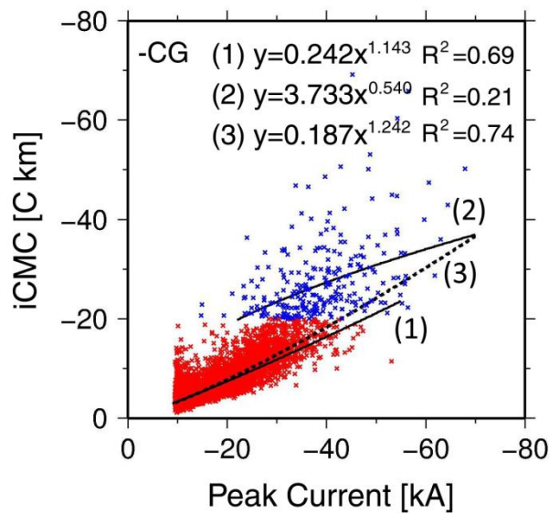
Figure 3.31. Peak current estimated from VLF data versus iCMC of -CG. The red cross shows iCMC more than -20 C·km, the blue cross shows iCMC less than -20 C·km.
