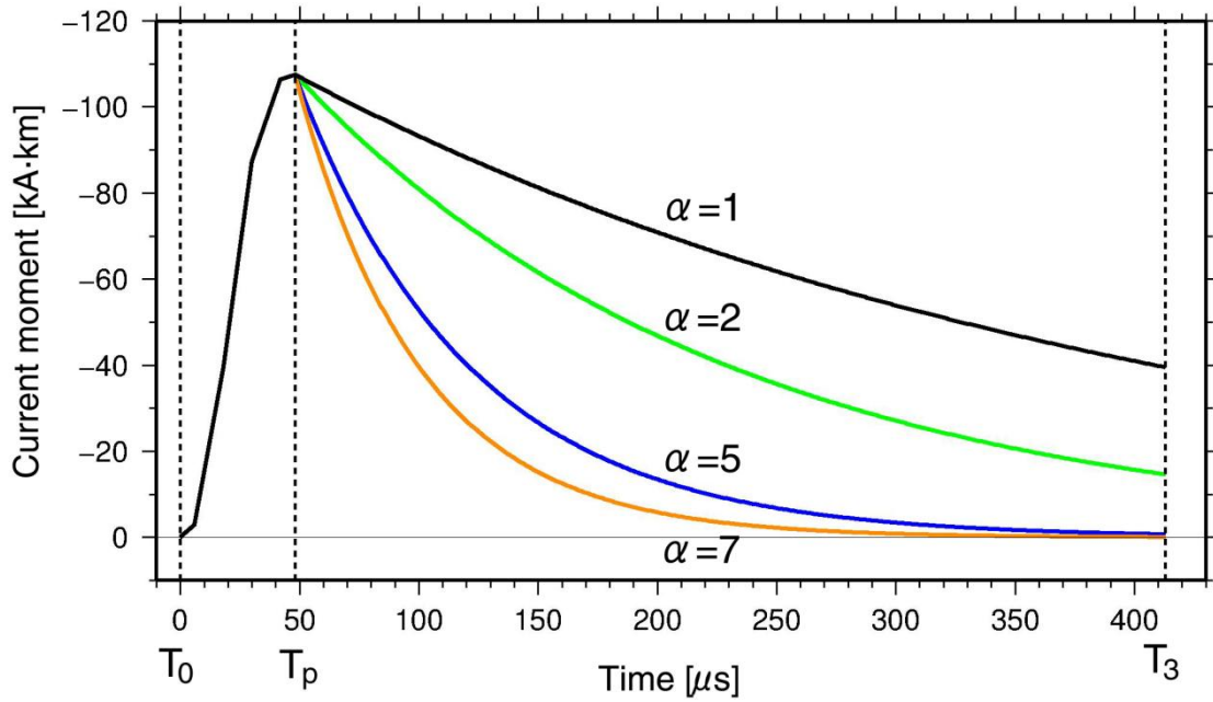
Figure 3.14. The time variation of current moment by different time constant.
