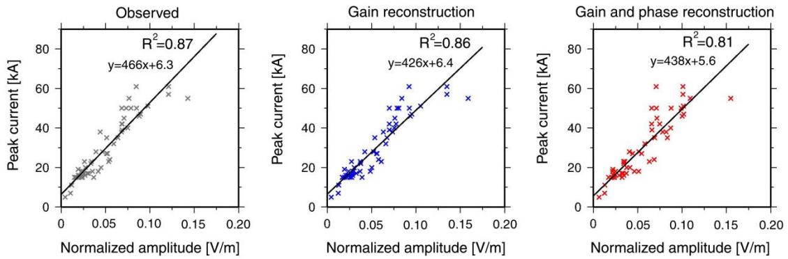
Figure 3.10. Three scatter plots of the normalized amplitude ( V_n ) versus the peak current of JLDN data ( I_{peak} ) in the case of +CG. Left panel: observed E-field, center panel: gain reconstructed E-field, right panel: gain and phase reconstructed E-field.
