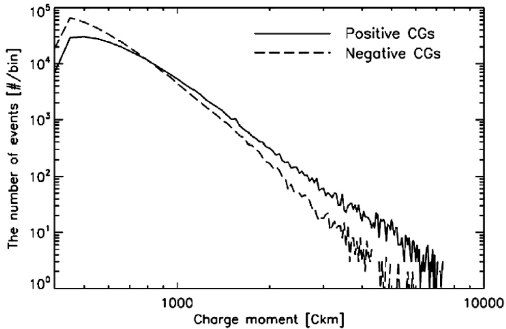
Figure 1.2. Distribution of charge moments with whole events. The number of positive CGs and negative ones are 182,689 and 288,046 respectively. [Yamashita et al. , 2011].
