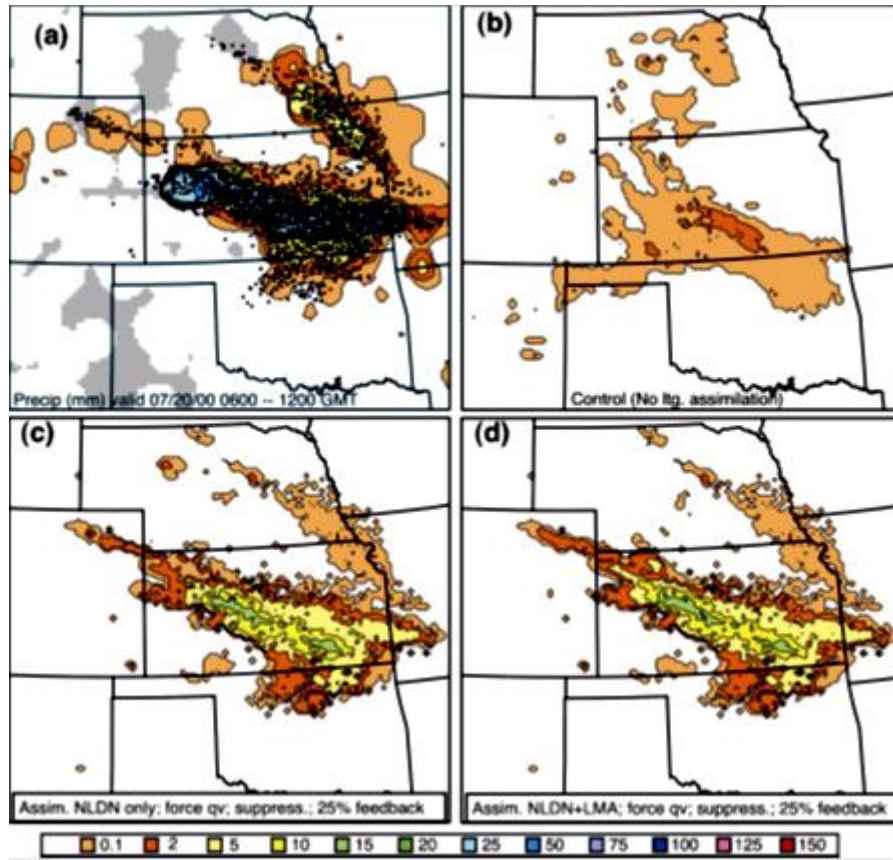
Figure 1.6. Observed and modeled total precipitation (mm) for a 6-h period starting 0600 UTC 20 Jul 2000 during the spinup period. (a) Rain gauge data with sampled NLDN strikes. (The 1st and 30th strikes are plotted in each 10-km grid box.) Gray-filled areas indicate data voids. (b) Pure forecast (no lightning assimilation). (c) With assimilation of CG lightning from NLDN, moisture forcing, and full suppression. (d) With assimilation of both CG and total (LMA) lightning, moisture forcing, full suppression, and 25% feedback of KF precipitation [Mansell et al. , 2007]
