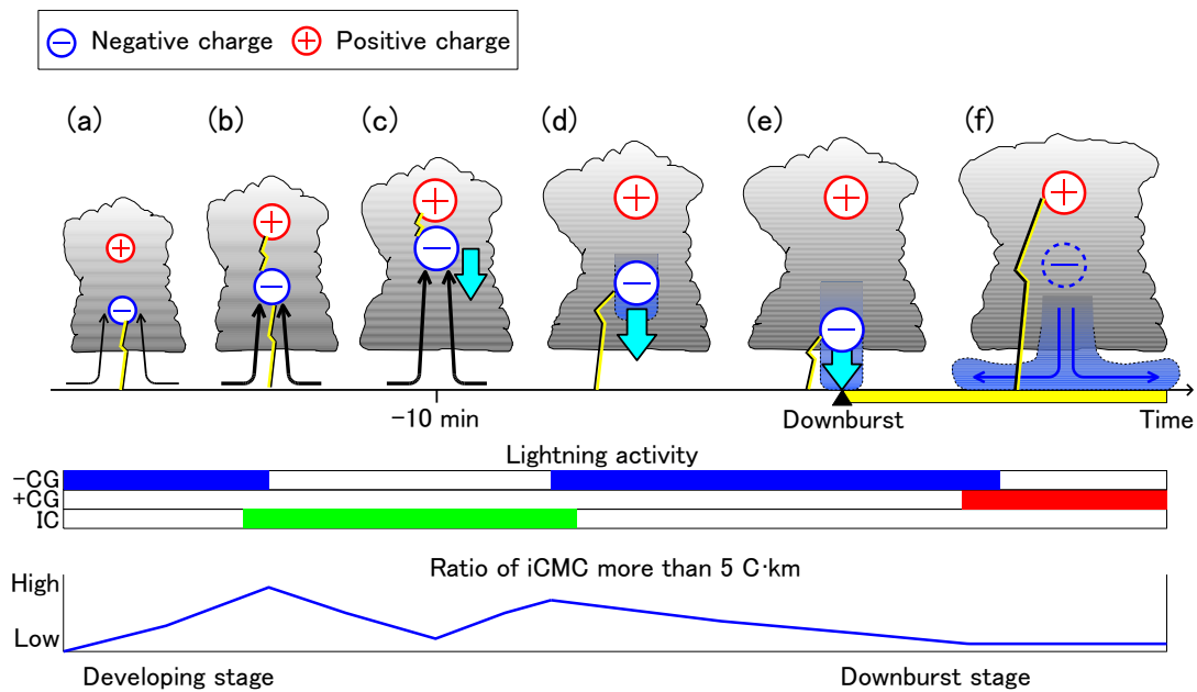
Figure 4.24. The time variation of inferred vertical motion of charge and lightning activities in the downburst-producing thundercloud. Blue circles and red circles display negative and positive charge center, respectively. Black arrow displays updraft, and thick aqua arrow displays downdraft. Color bars indicate which type of lightning activity dominate. Blue, red and green bar show the -CG, +CG and IC activity. Yellow bar shows the period of occurrence of the downburst at the surface. Blue line indicates the time variation of the ratio of iCMC more than 5 C·km in absolute value.
