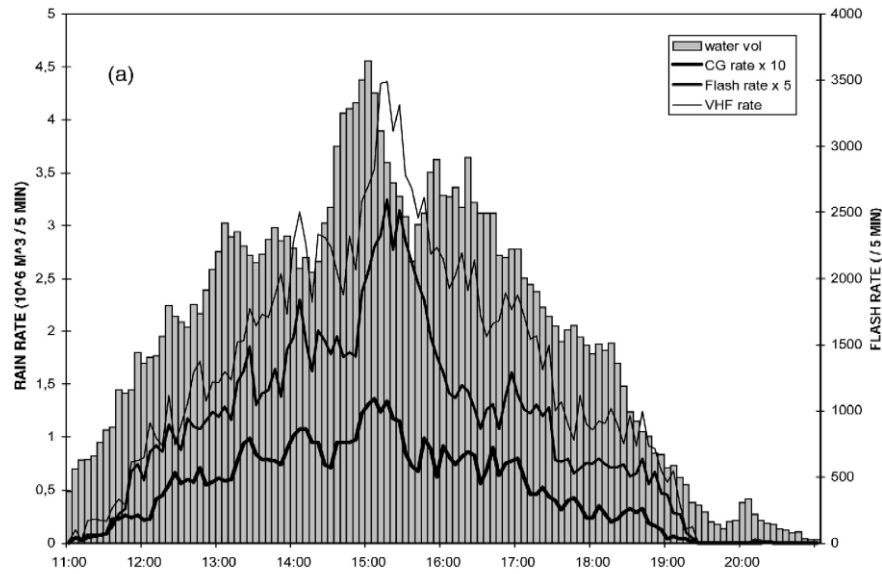
Figure 1.4. Evolution of the rain rate and of the flash rates. (a) July 11, 1997 [Soula and Chauzy, 2001].
