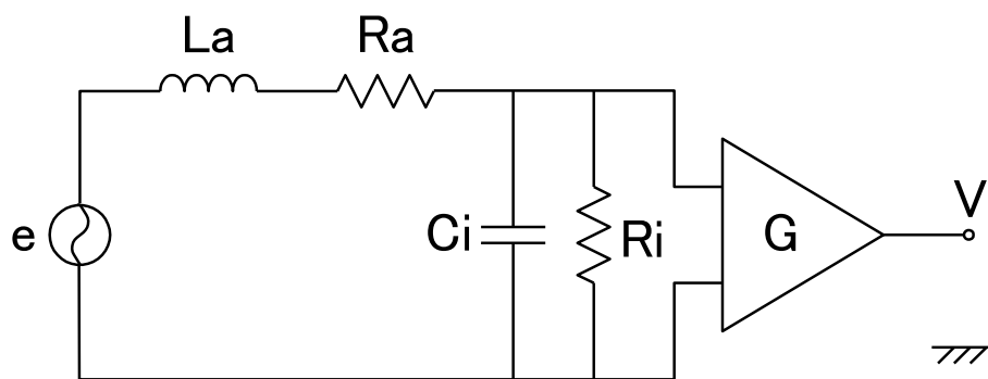
Figure 2.8. Equivalent electric circuit of the antenna and pre-amplifier.
