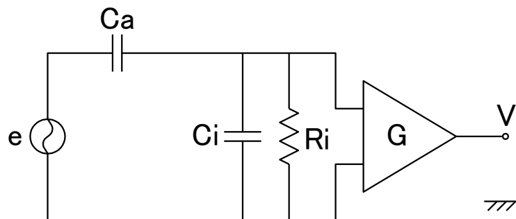
Figure 2.4. Equivalent electric circuit of the antenna and pre-amplifier.
