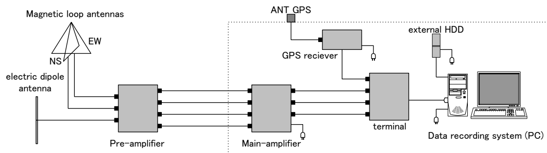
Figure 2.1. Block diagram of the VLF observation system.
