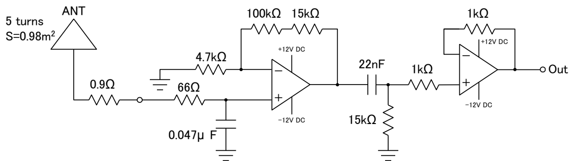
Figure 2.9. Circuit diagram of the pre-amplifier.
