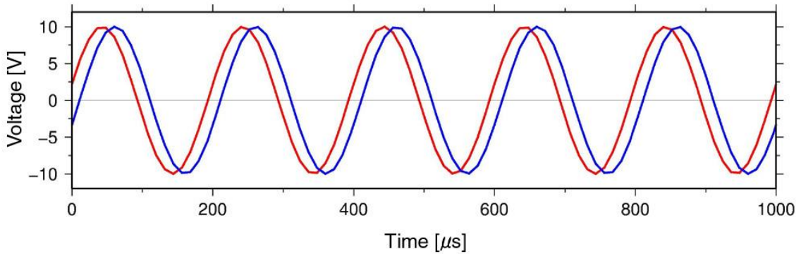
Figure 3.7. Verification result of the gain and phase reconstruction of sin wave at 5 kHz. The waveforms indicated in blue and in red are input signal and reconstructed signal, respectively.
