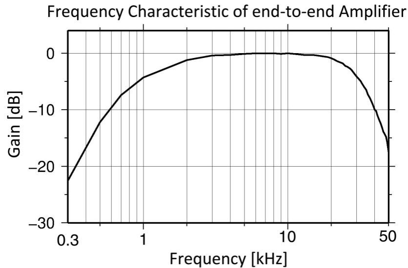
Figure 2.6. Frequency characteristic of gain including main-amplifier and pre-amplifier.
