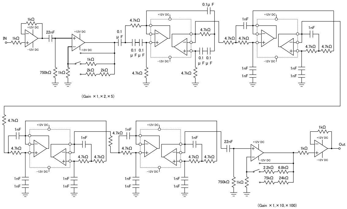
Figure 2.5. Circuit diagram of the main-amplifier.
