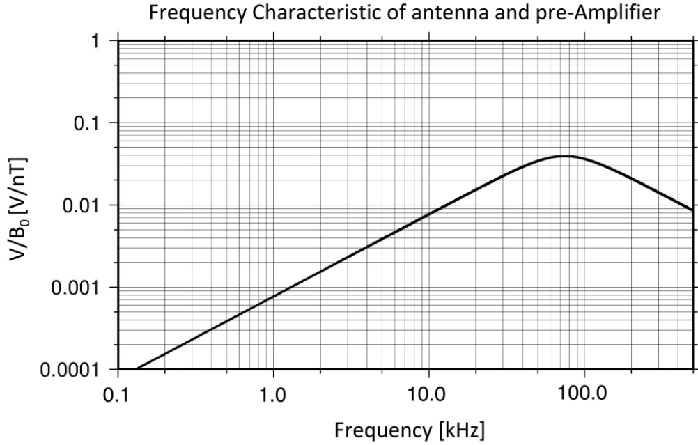
Figure 2.12. Frequency characteristic of gain of magnetic field.
