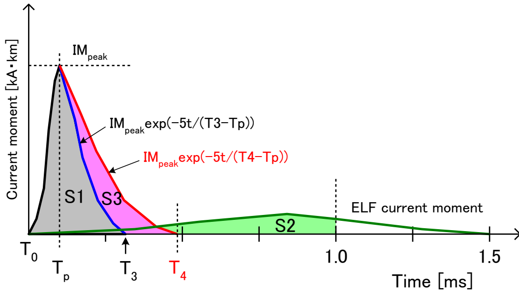
Figure 3.20. Schematic diagram of correcting integration interval of waveform using the current moment estimated by ELF waveform.
