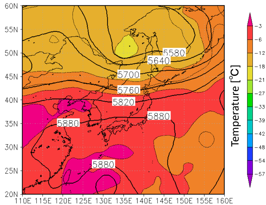
Figure 4.2. 500-hPa level upper weather chart at 09 h (JST), July 11, 2013. The black line is isohypse, and color contour is an air temperature at 500 hPa at isobaric surface.
