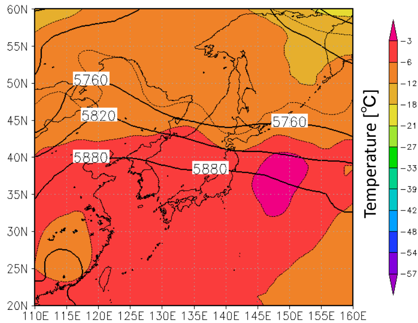
Figure 4.15. 500-hPa level upper weather chart at 09 h (JST), August 11, 2013. The black line is isohypse, color contour is an air temperature at 500 hPa at isobaric surface.
