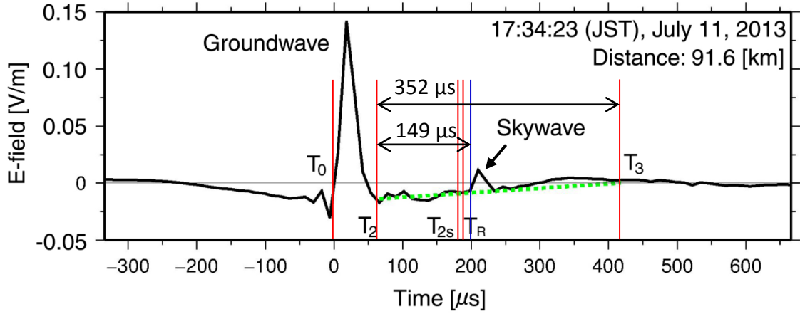
Figure 3.12. Example of reconstructed waveform and calculated T_R , T_{2s} and T_3 .
