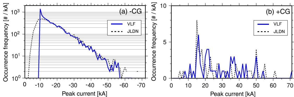
Figure 3.22. Occurrence frequency of peak current estimated by VLF and JLDN. (a) negative CG, (b) positive CG.
