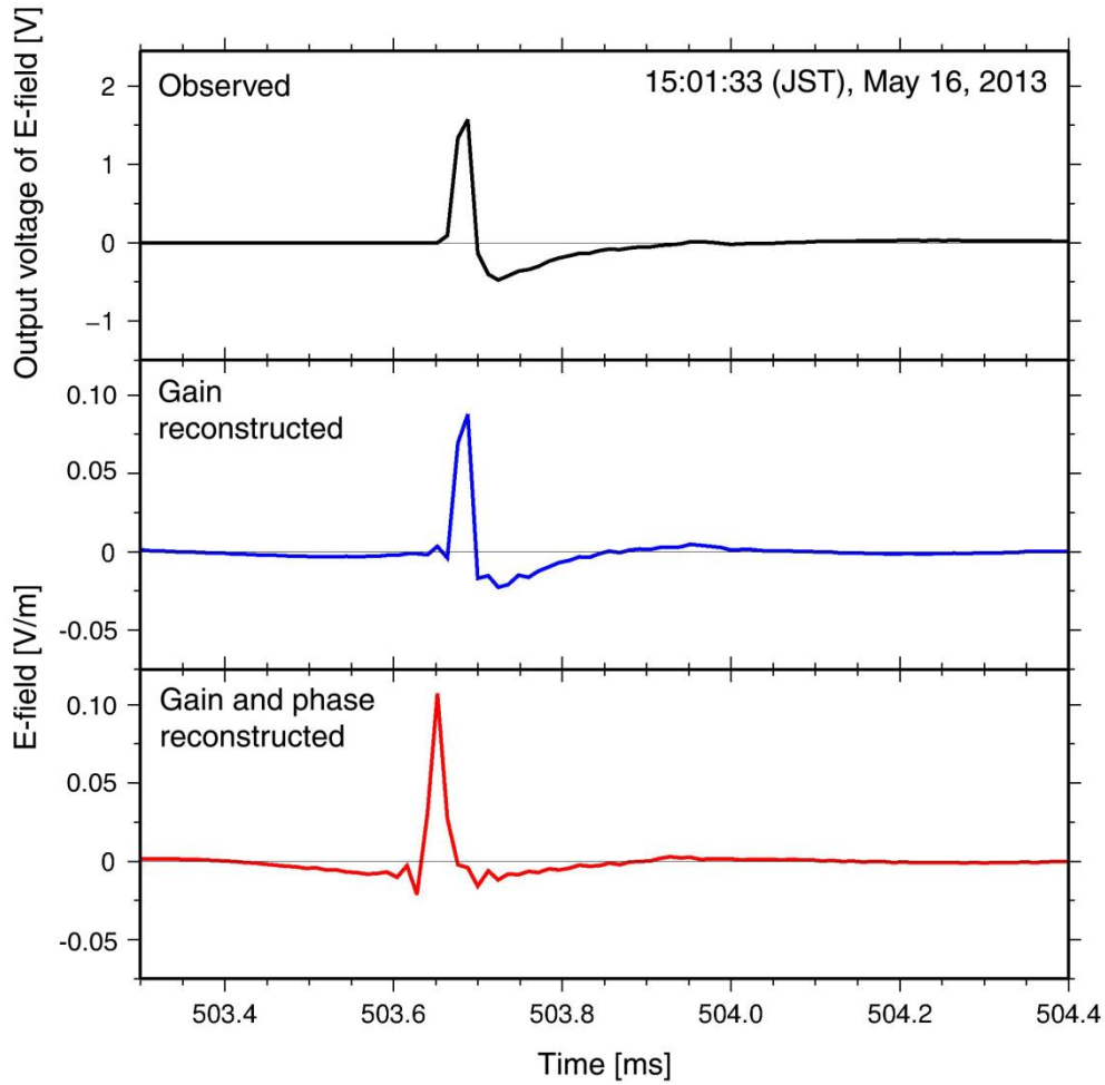
Figure 3.8. Example of reconstruction of the waveform observed at Yamanashi site.
