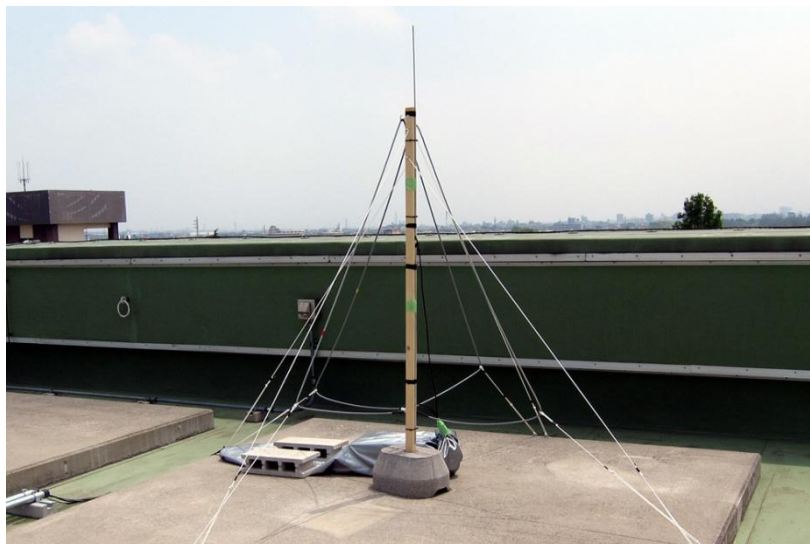
Figure 2.14. External view of the antenna of Maebashi site.
