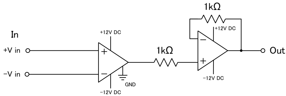
Figure 2.3. Circuit diagram of the pre-amplifier
