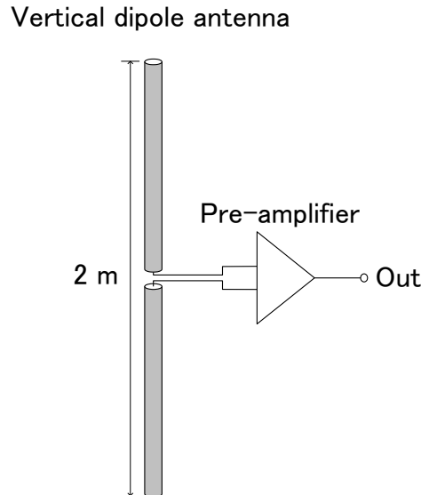
Figure 2.2. Schematic diagram of the antenna and pre-amplifier.
