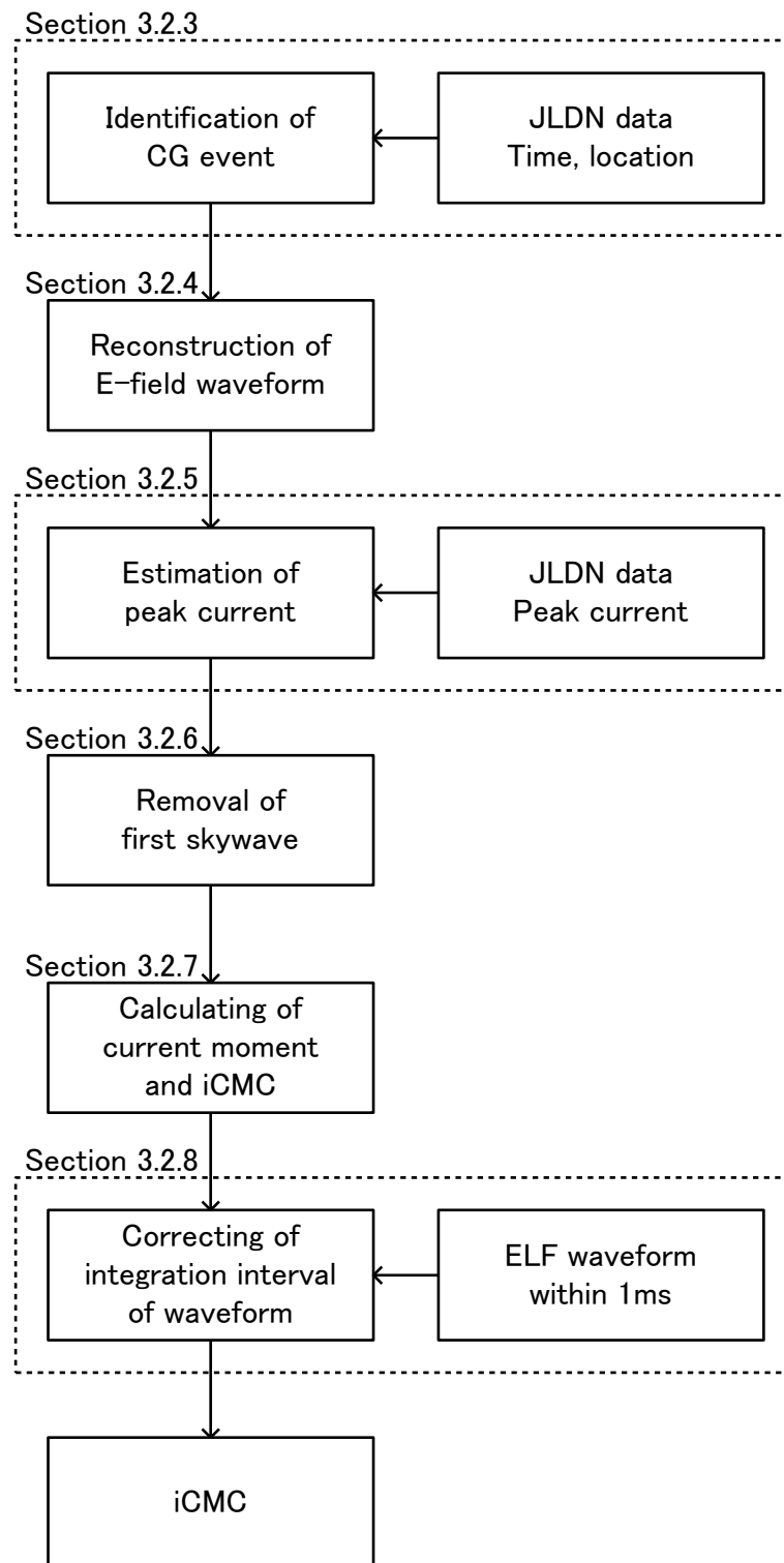
Figure 3.5. Flow diagram of the estimation of iCMC.
