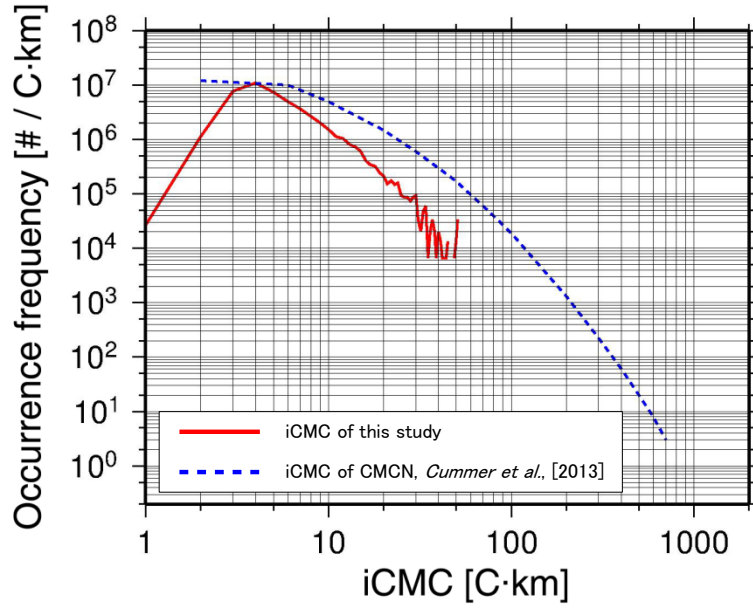
Figure 3.29. Distribution of iCMC for -CG lightning events. Red solid line is distribution of iCMC of this study, and blue dashed line is distribution of iCMC adapted from Cummer et al. , [2013].
