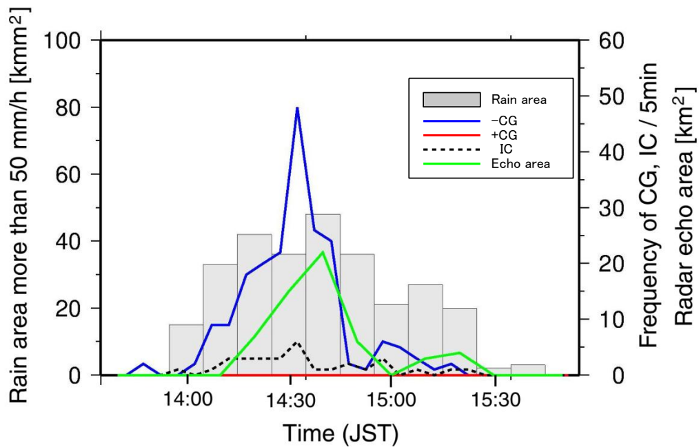
Figure 4.7. Evolution of the rain area more than 50 mm/h, area of echo height more than 12 km and lightning flash rate on July 11, 2013 from 13:50 to 15:50 (JST).
