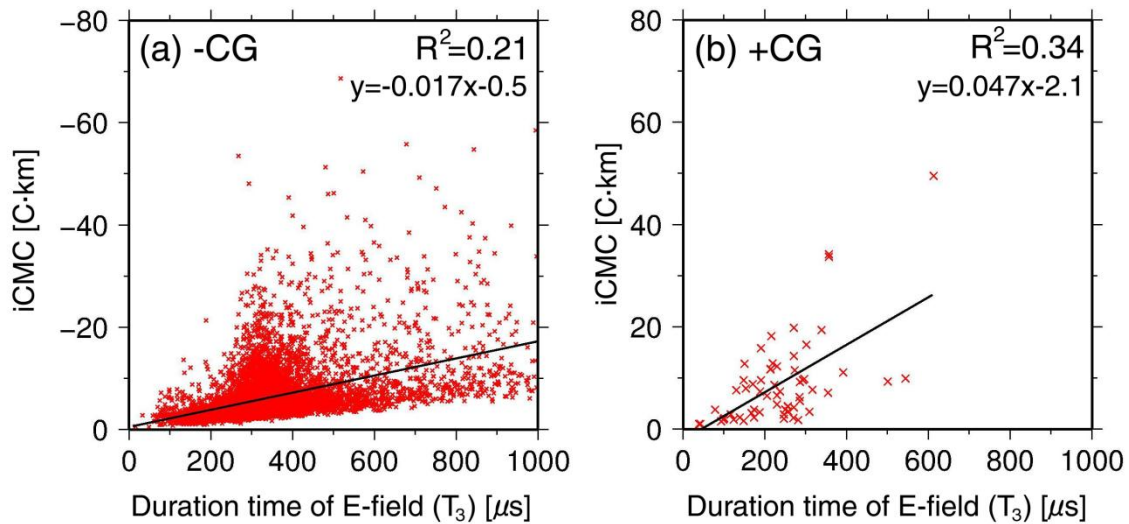
Figure 3.26. Scatter plot of the duration time of sferic ( T_3 ) [ \mu s] versus iCMC [C·km]. (a) negative CG, (b) positive CG.
