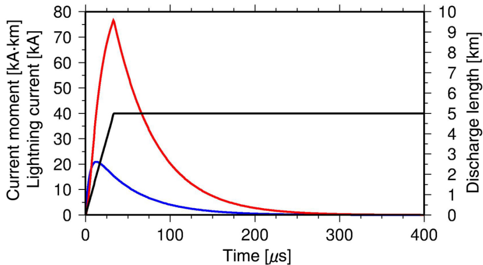
Figure 3.30. Typical current of return stroke and current moment. Red line is the current moment, blue line is the lightning current, and black line is the discharge length.
