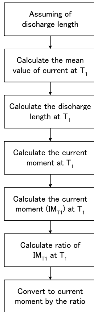
Figure 3.15. Flow diagram of converting the relative current moment to the absolute value of current moment.
