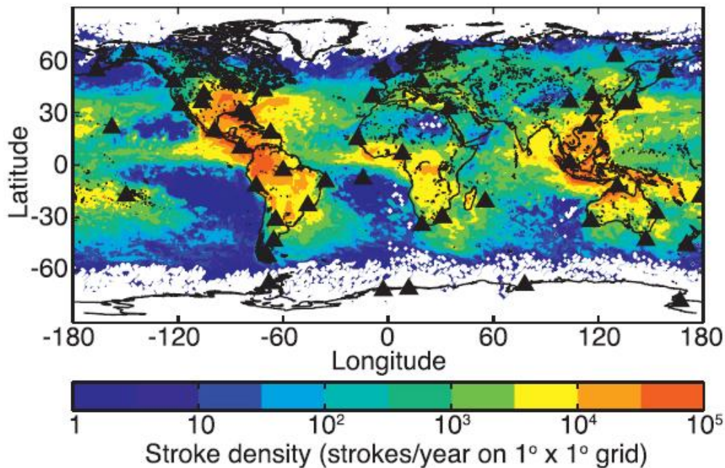
Figure 1.10. WWLLN 2010 global stroke on 1^\circ \times 1^\circ grid, station location shown (black triangles) [Hutchins et al. , 2012].
