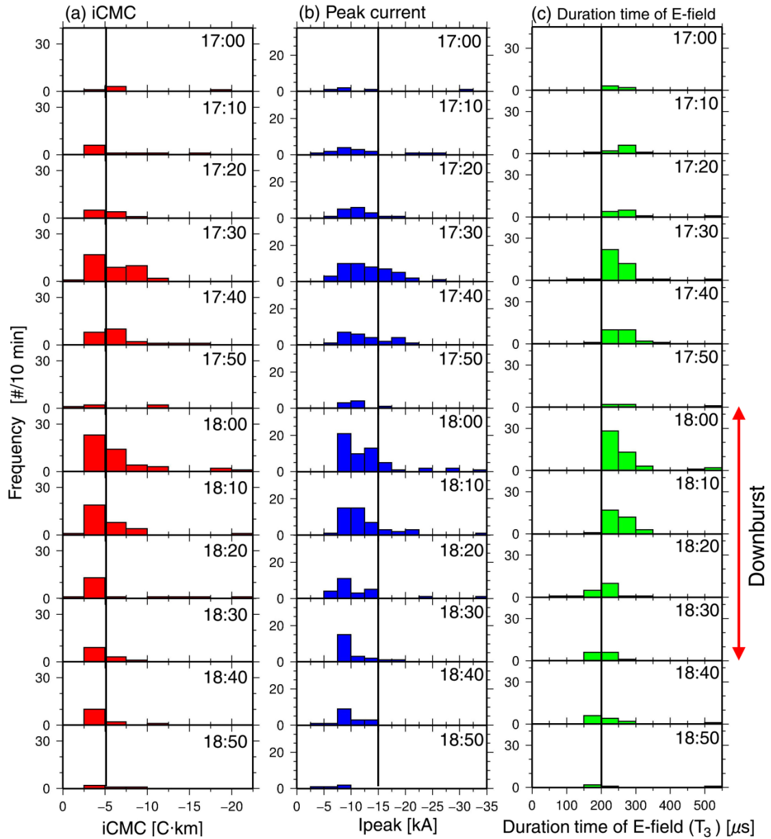
Figure 4.21. Time variation of frequency distribution of (a) iCMC, (b) peak current and (c) duration time of electric field ( T_3 ) on August 11, 2013 from 17:00 to 18:50 (JST).
