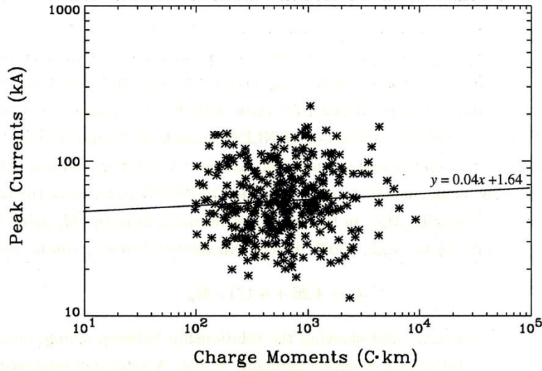
Figure 3.34. Scatter plot of the charge moments versus the peak currents for 331 events of sprite-including CG discharge [Sato, 2004].
