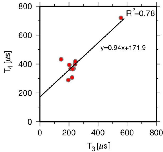
Figure 3.21. Scatter plot of T_3 versus T_4 . The black line is linear approximation with R^2=0.78 .
