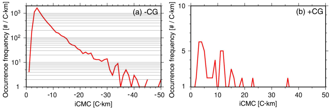
Figure 3.23. Occurrence frequency of iCMC. (a) negative CG, (b) positive CG.
