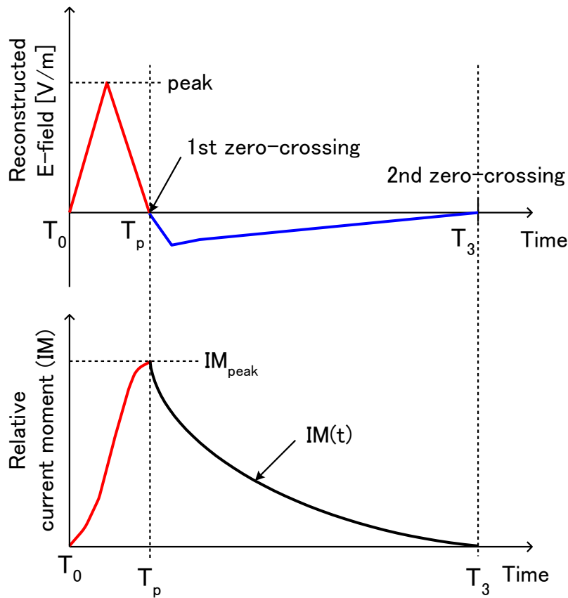
Figure 3.13. Schematic diagram of calculating a relative current moment.
