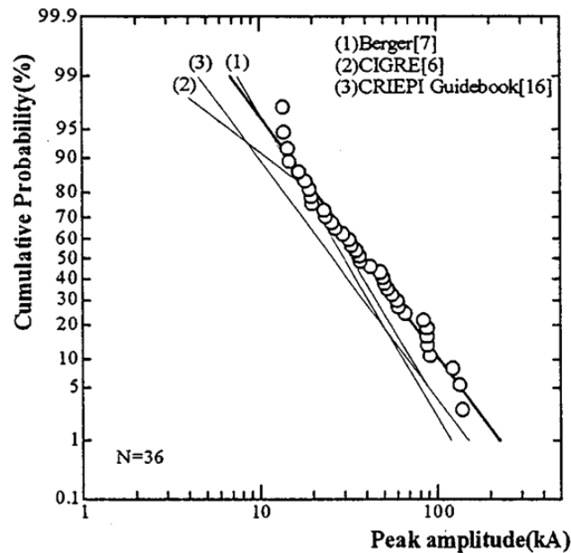
Figure 1.1. Cumulative frequency distributions of peak current of lightning strokes [Narita et al. , 2000].
