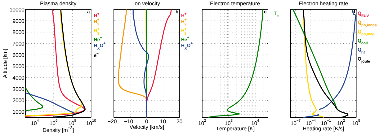
Figure 4.4: Plasma parameters in the mid-latitude at 0 LT. Each panel is same as Fig.4.2.
