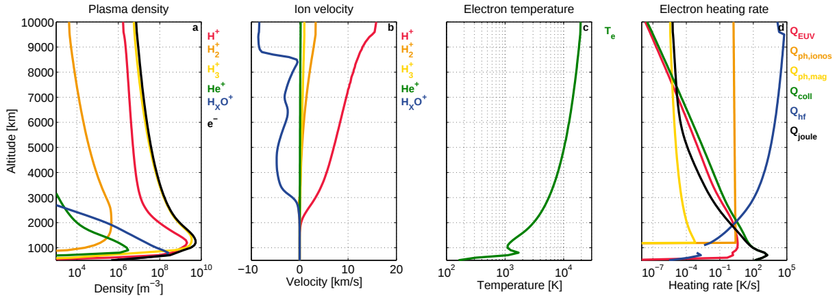
Figure 4.2: Plasma parameters in the mid-latitude at 12 LT. The plasma density profiles are shown in panel a. Red line is \text{H}^+ , orange line is \text{H}_2^+ , yellow line is \text{H}_3^+ , green line is \text{He}^+ , blue line is \text{H}_x\text{O}^+ , and black line shows electron. The velocity profiles are shown in panel b, and colors are same as panel a. The electron temperature is shown in panel c (green line). The heating rates are shown in panel d. Red line shows the heating rate due to the solar EUV, orange line shows the heating rate due to the photoelectron from ionosphere, yellow line shows the heating rate due to the photoelectron due to magnetosphere, green line shows the heating rate due to the collision, blue line shows the rate due to the heat flow, and black line shows the joule heating.
