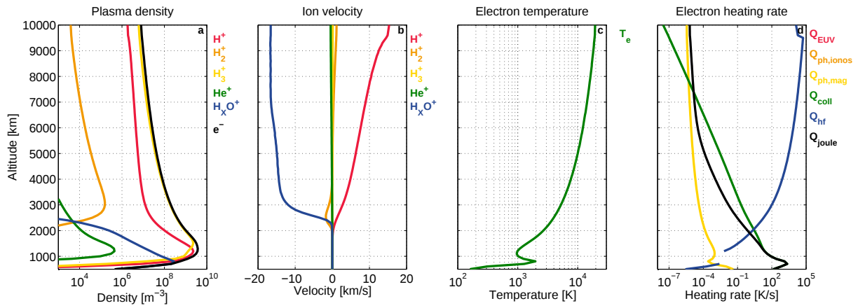
Figure 4.3: Plasma parameters in the mid-latitude at 18 LT. Each panel is same as Fig.4.2.
