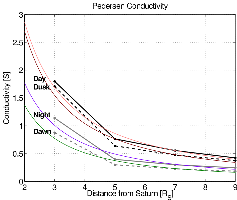
Figure 5.5: Integrated Pedersen conductivities in each L and their fitting curve. Black solid line indicates 12 LT, black dashed line indicates 18 LT, grey solid line indicates 0 LT and grey dashed line indicates 6 LT. The fitting curves are pink for day, brown for dusk, purple for night and green for dawn.
