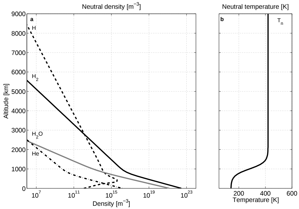
Figure 4.1: Background atmospheric (a) density and (b) temperature. Black dashed line shows H, black solid line shows \text{H}_2 , black dashed-dotted line shows He and grey solid line shows \text{H}_2\text{O} .
