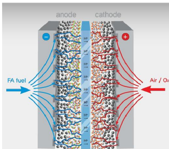
Figure 1.1. (a) The schematic illustration of direct liquid fuel cells. Adopted from Electrochemical Reaction & Technology Laboratory at GIST [6].
