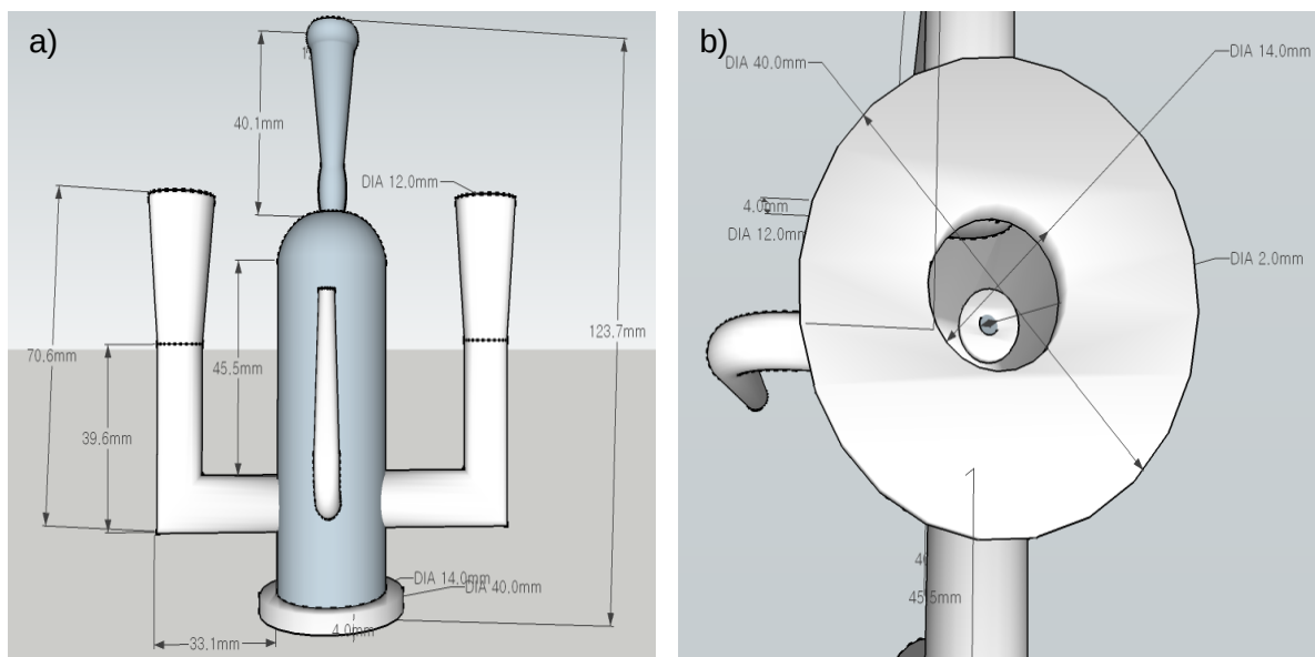
Figure 2.2. Schematic drawing of the experimental setup for electrochemical reaction cell.
