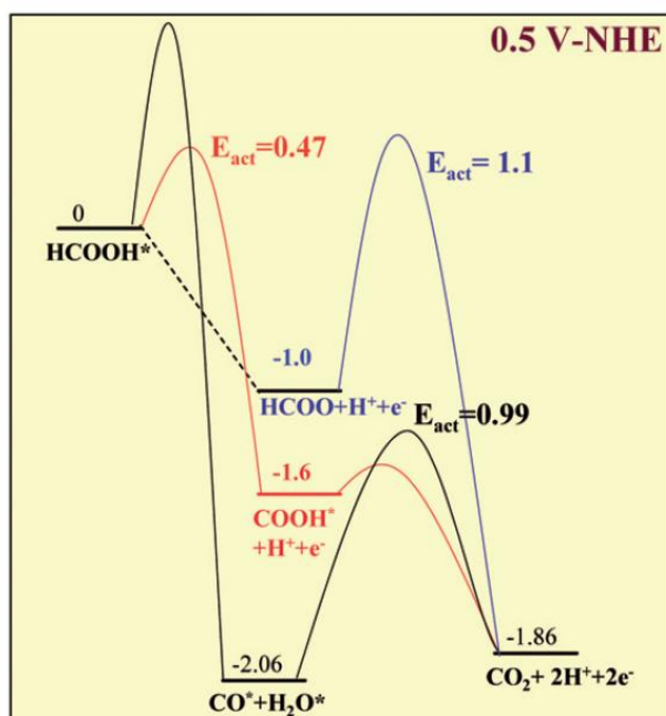
Figure 1.8. DFT-calculated potential energy surface for the direct, indirect, and formate paths for the oxidation of formic acid over Pt(111) to \text{CO}_2 held at a constant potential of 0.5 V. Adopted from [45].
