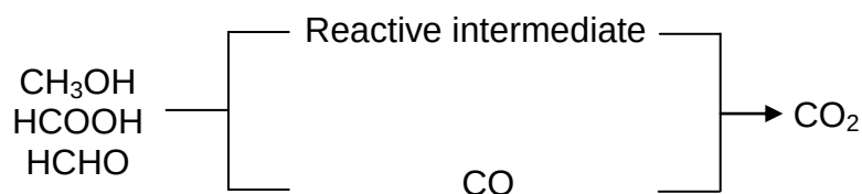
Figure 1.4. Dual-path mechanism for oxidation of methanol, formic acid and formaldehyde at a Pt electrode.
