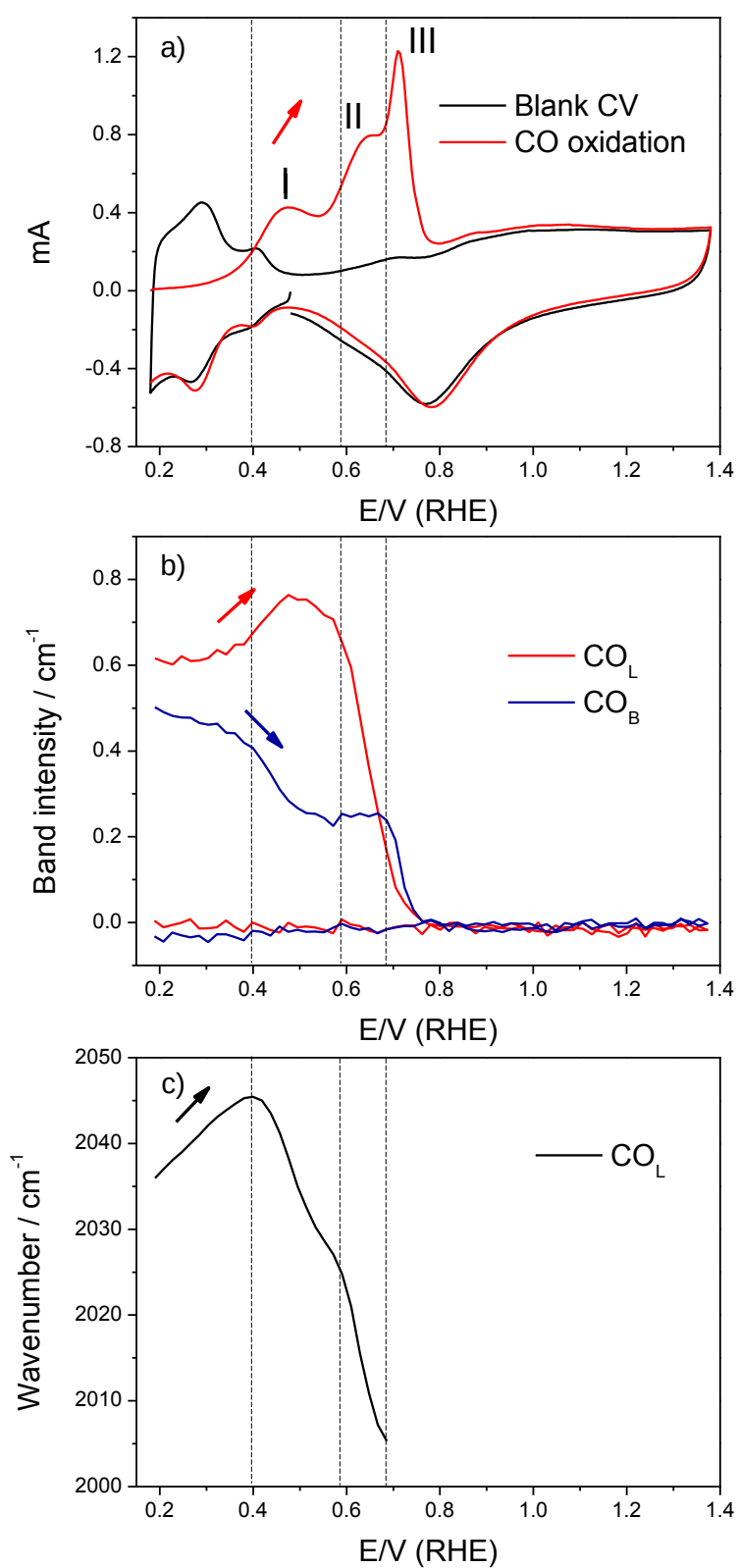
Figure 3.2. (a) Cyclic voltammetry of electrooxidation of CO. (b) Potential dependence of the integrated band intensity of \text{CO}_L (red), \text{CO}_B (blue), and (c) vibration frequency of \text{CO}_L . Scan rate is 50 \text{ mV s}^{-1} .
