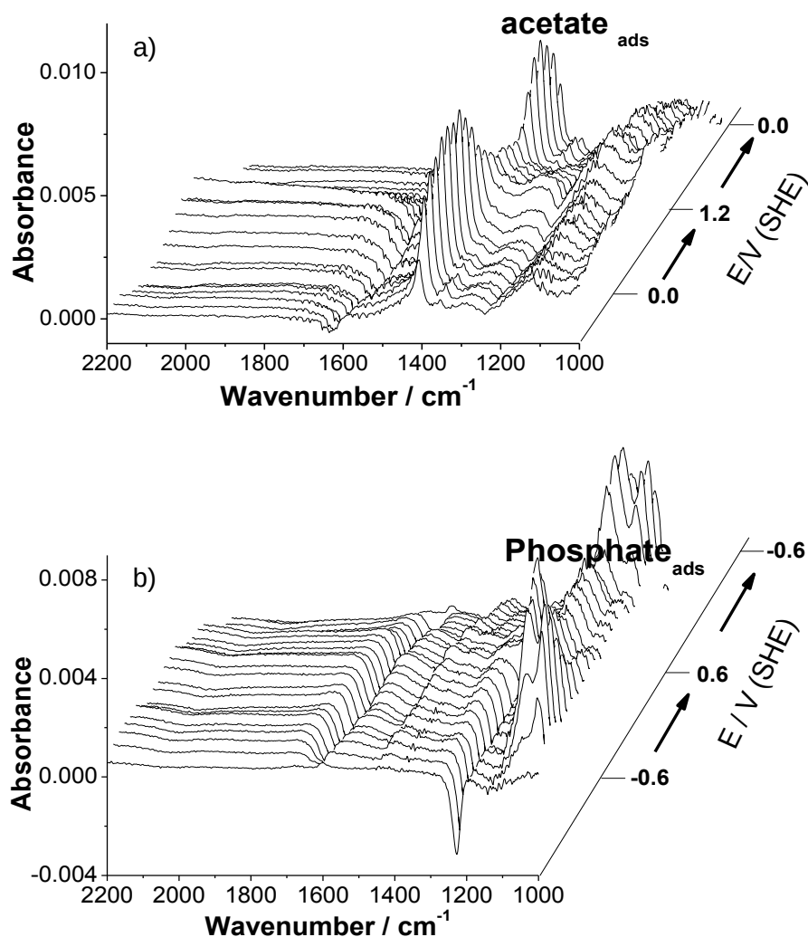
Figure 4.5. SEIRA spectra of the surface of a Pt thin film electrode sequentially collected at 20 mV s -1 in buffer solution with (a) pH 1.5 and (b) 11.6 containing 100 mM CH 3 COOH.
