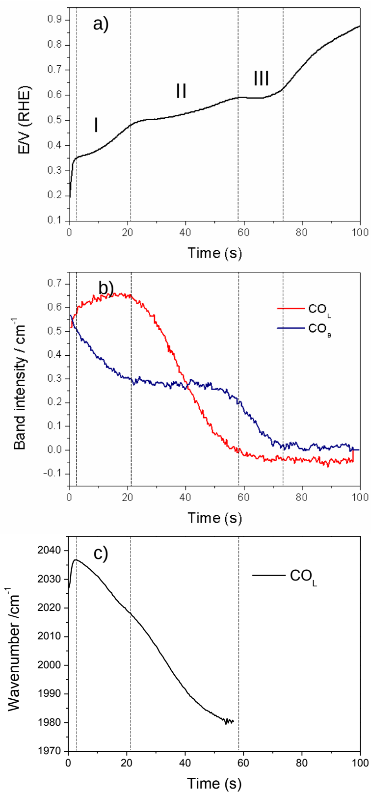
Figure 3.5. (a) Potential transient under galvanostatic condition. (b) The integrated band intensities of CO L (red), CO B (blue), and (c) vibrational frequency of CO L (black).
