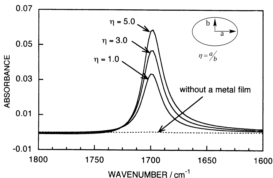
Figure 1.14. SEIRA spectra of a model molecule adsorbed on Ag island films simulated by using the Bruggeman effective-medium models. The mass thickness of the Ag film is 8 nm. The dashed trace is the spectrum of a molecular layer on the substrate ( \text{CaF}_2 ) without a metal film. \eta represents the aspect ratio of the metal ellipsoid. Adopted from [51].
