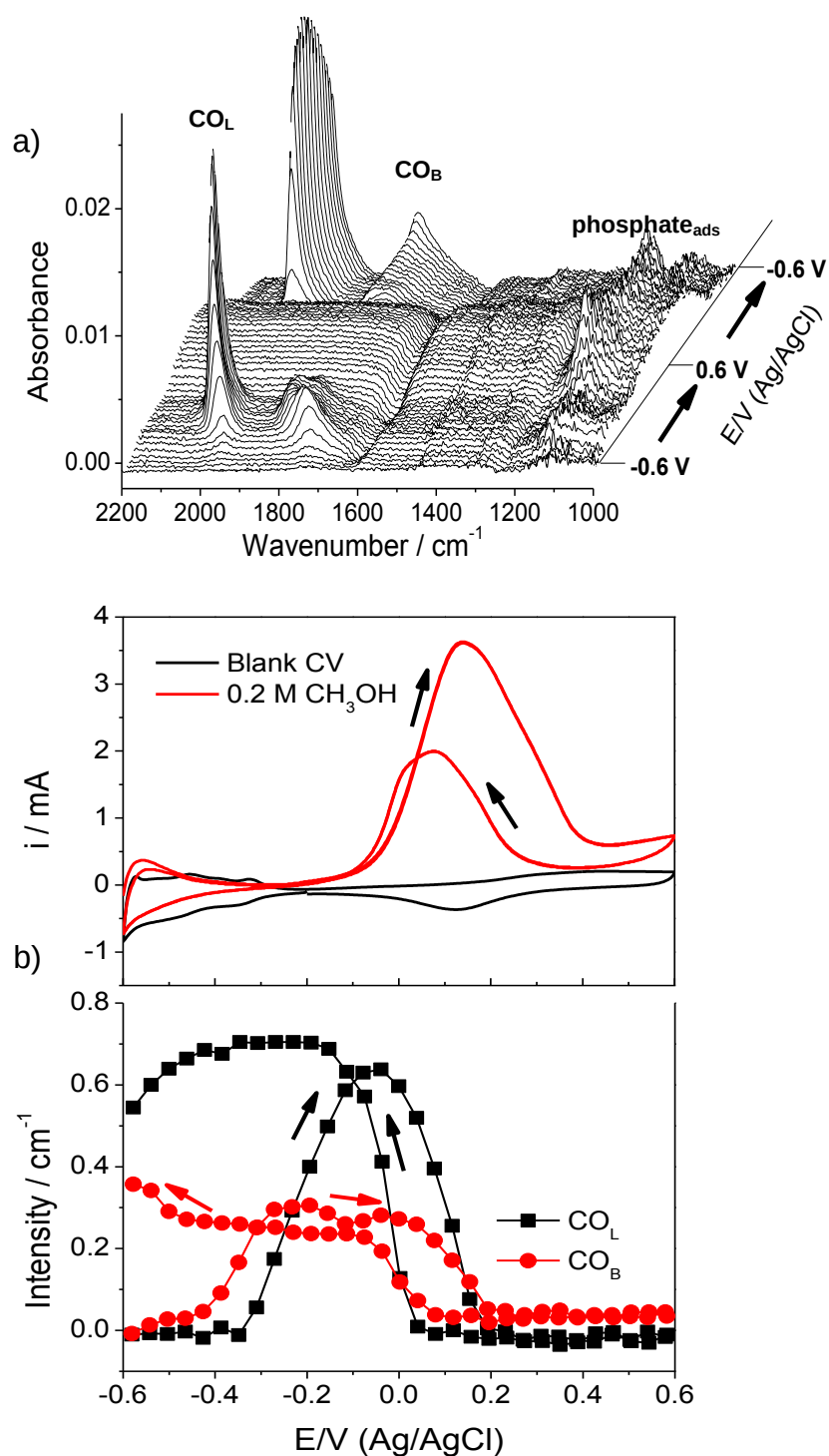
Figure 5.6. (a) SEIRA spectra of the surface of a Pt thin film electrode sequentially collected during a potential sweep from -0.6 to 0.6 and back to -0.6 V at 20 \text{ mV s}^{-1} in buffer solution with pH 7.6 containing 0.2 M \text{CH}_3\text{OH} . (b) CV recorded simultaneously with the SEIRA spectra (upper) and the potential dependence of the integrated intensities of \text{CO}_L and \text{CO}_B taken from (a). The solid line is
