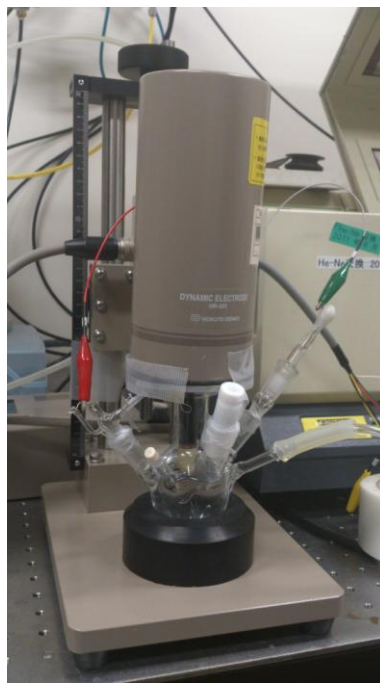
Figure 2.1. Rotating electrode system.
