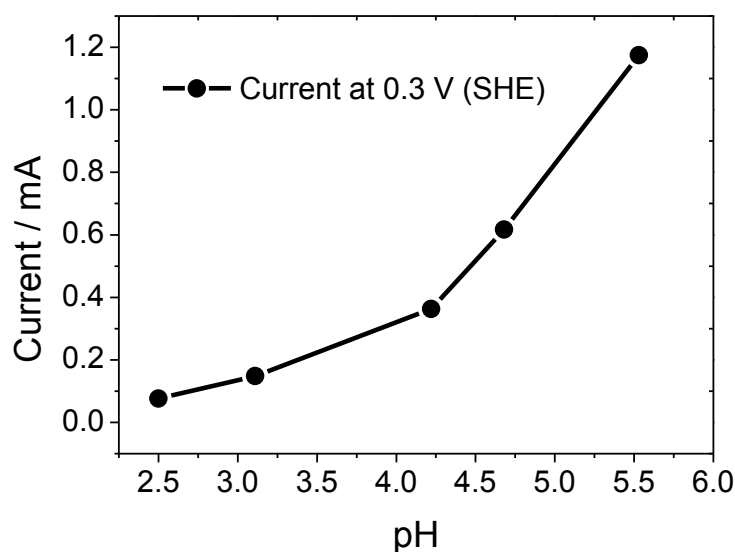
Figure 4.1. Dependence of pH on the current at 0.3 V (vs. SHE) on the Pt electrode (0.34 cm 2 ) in the presence 10 mM HCOONa. Adopted from [25].
