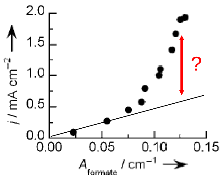
Figure 1.7. Nonlinear relationship between oxidation current j and the band intensity of bridge-bonded adsorbed formate A_{\text{formate}} . A_{\text{formate}} is the average of 10 spectra around t=0.5 s. Adopted from [36].
