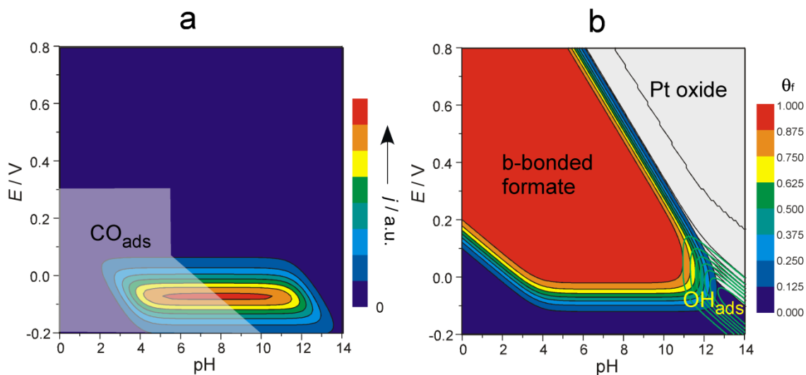
Figure 4.11. Simulation when bridge-bonded formate is assumed to be site-blocking spectator (i.e., k_2^{\text{eq}} = 0 ). (a) Both oxidation current and (b) bridge bonded formate coverage are simulated.
