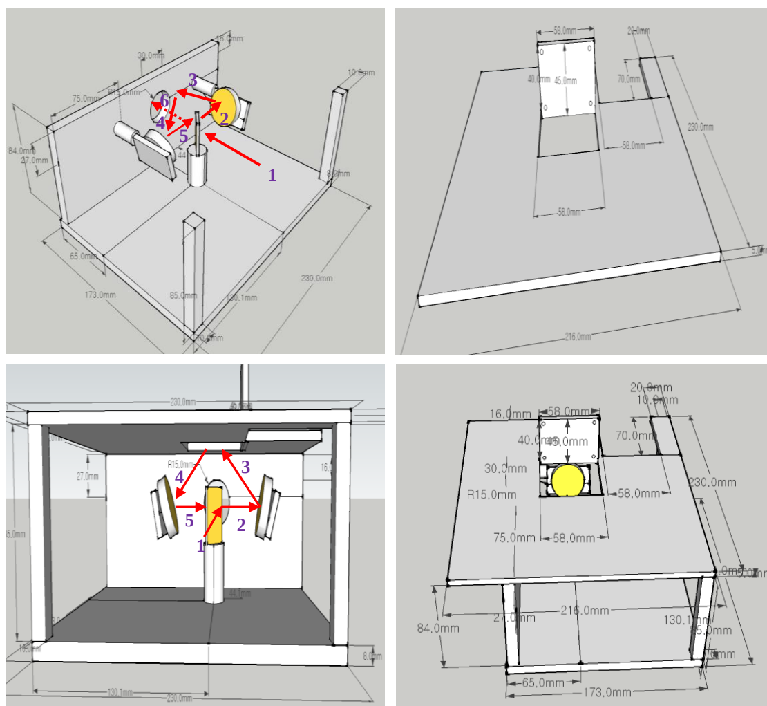
Figure 2.5. Schematic of the homemade single reflection accessory.
