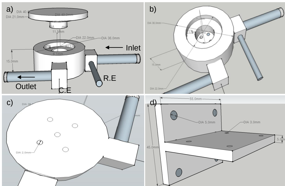
Figure 2.3. Schematic drawing of a flow cell made of Kel-F : (a) front view (b) top view (c) bottom view, and (d) flow cell holder.
