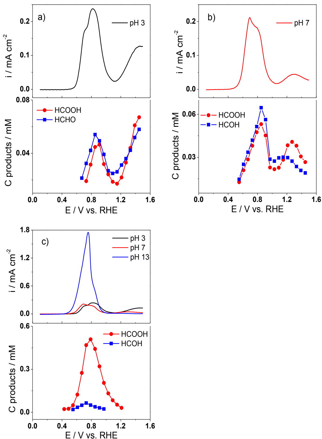
Figure 5.4. Potential dependence of the concentrations of byproducts formed during 0.2 M methanol oxidation in 0.2 M phosphate buffer solution of (a) pH 3, (b) pH 7, and (c) pH 13 measured with on-line HPLC. Top panels are the LSVs simultaneously recorded with the HPLC analysis. Note that, since 0.5 mM \text{H}_2\text{SO}_4 was used as the eluent, the real product is formate in the neutral and
