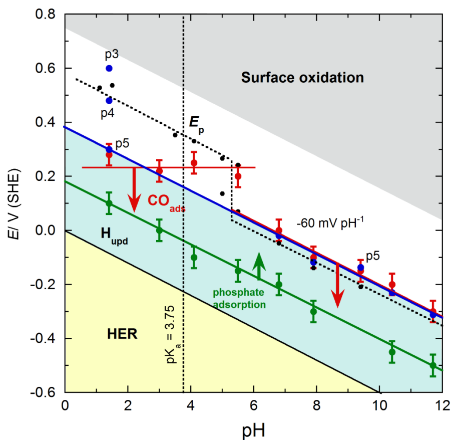
Figure 4.7. Pourbaix diagram of the \text{HCOOH}/\text{HCOO}^- oxidation on Pt. Black symbols: peak potential of the anodic peak, E_p , taken from Ref. [49] ; blue symbols: peak potentials of the anodic peaks or shoulders in the negative-going scan; red symbols: onset potential of \text{CO}_{\text{ads}} formation in the negative-going sweep; green symbols: onset potential of the adsorption of phosphate anions in the positive-going scan. See further details in the text.
