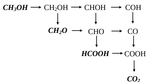
Figure 5.1. The Bagotzky model for electrooxidation of methanol in acidic media. Adopted from [6].
