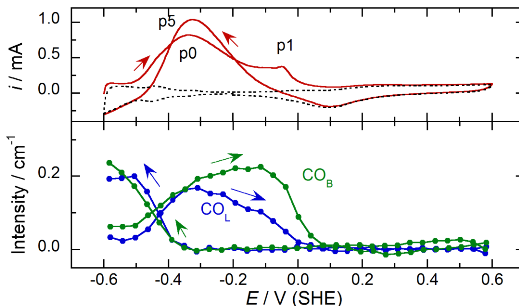
Figure 4.6. CV for 20 mM \text{HCOO}^- in buffer solution with pH 11.7 at 20 \text{ mV s}^{-1} (upper panel) and recorded simultaneously with the SEIRA spectra (upper panel) and the potential dependence of the integrated intensities of the \text{CO}_L and \text{CO}_B bands taken from SEIRA spectra collected simultaneously with the CV (lower panel). The dashed trace in the upper panel is the CV in the same electrolyte without \text{HCOONa} .
