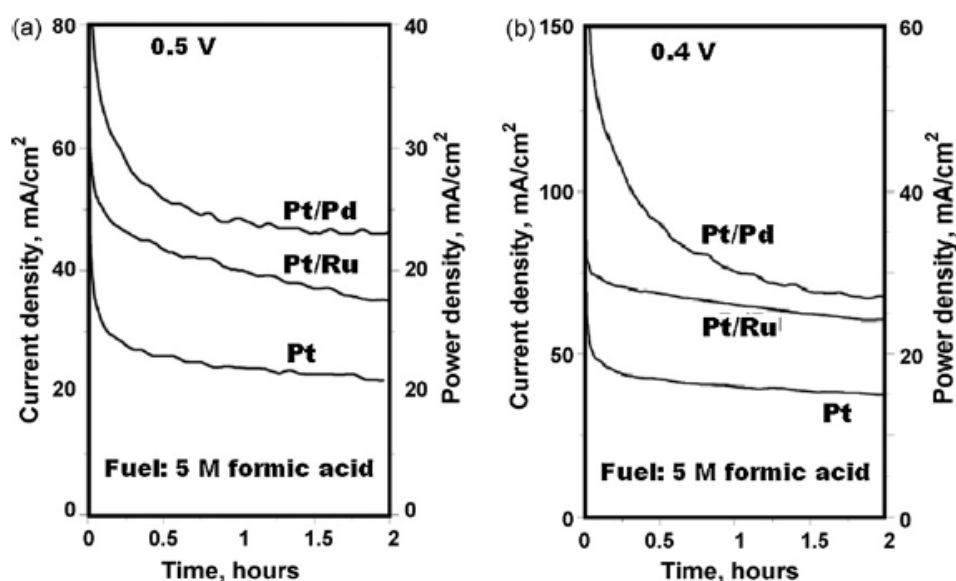
Figure 1.3. Constant voltage tests on a DFAFC at cell potentials of (a) 0.5 V and (b) 0.4 V. Catalysts: platinum black, Pt/Ru, and Pt/Pd; fuel: 5 M formic acid at 0.2 ml/min; cell temperature was 30°C. Adopted from [13]
