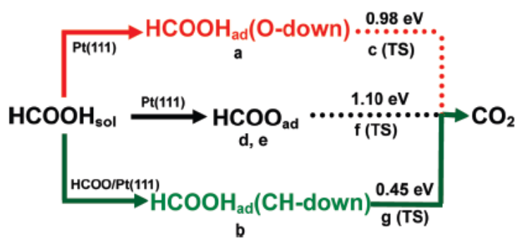
Figure 1.9. Triple pathways for formic acid ( \text{HCOOH}_{\text{sol}} ) oxidation leading to \text{CO}_2 at Pt/ \text{H}_2\text{O} interface. The data are the calculated barriers. Adopted from [46].
