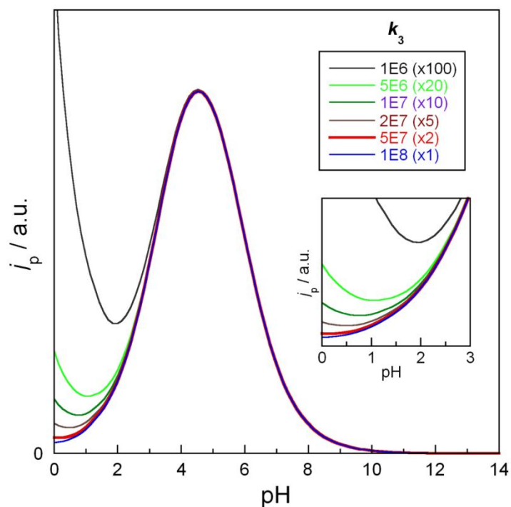
Figure 4.12. Simulation for contribution of \text{HCOO}^- oxidation to the total current varying the k_3^{\text{eq}} .
