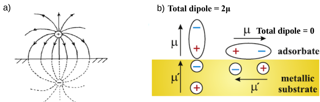
Figure 1.16. Qualitative explanation of the orientation selection rule for dipole surface scattering: (a) the lines of force and the electrical image resulting from a positive charge over the surface of a conductor (the metal surface is the upper line above the hatched area). (b) the image dipole within the substrate compensates the effect of the adsorbed dipole for paralleled orientation but enhances the effect of dipoles with a normal orientation. Adopted from [65].
