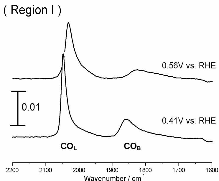
Figure 3.3. Change in spectra features before and after peak I in figure 3.2.
