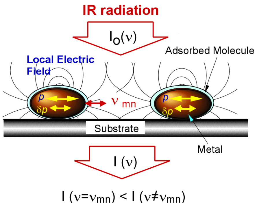
Figure 1.12. Schematic representation of the electromagnetic mechanism of SEIRA on metal island films. Incident photon field I_0 polarizes the metal islands and the dipole p generates an
