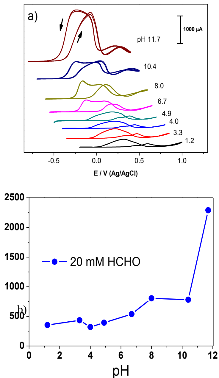
Figure 5.3. (a) Cyclic voltammograms of a rotating Pt disk electrode (1000 rpm) in 0.2 M phosphate buffer solutions containing 20 mM HCHO recorded at 50 \text{ mV s}^{-1} . The pH values of the solutions are shown in the figure. (b) The pH dependence of peak current in the negative-going scan.
