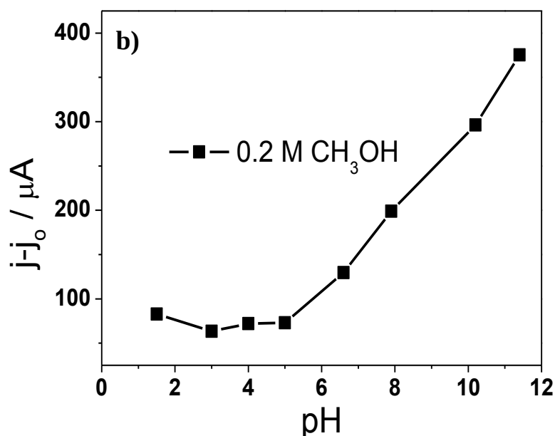
Figure 5.2. (a) Cyclic voltammograms of a rotating Pt disk electrode (1000 rpm) in 0.2 M phosphate buffer solutions containing 0.2 M \text{CH}_3\text{OH} recorded at 50 \text{ mV s}^{-1} . The pH values of the solutions are shown in the figure. (b) Peak current in the positive-going scan.
