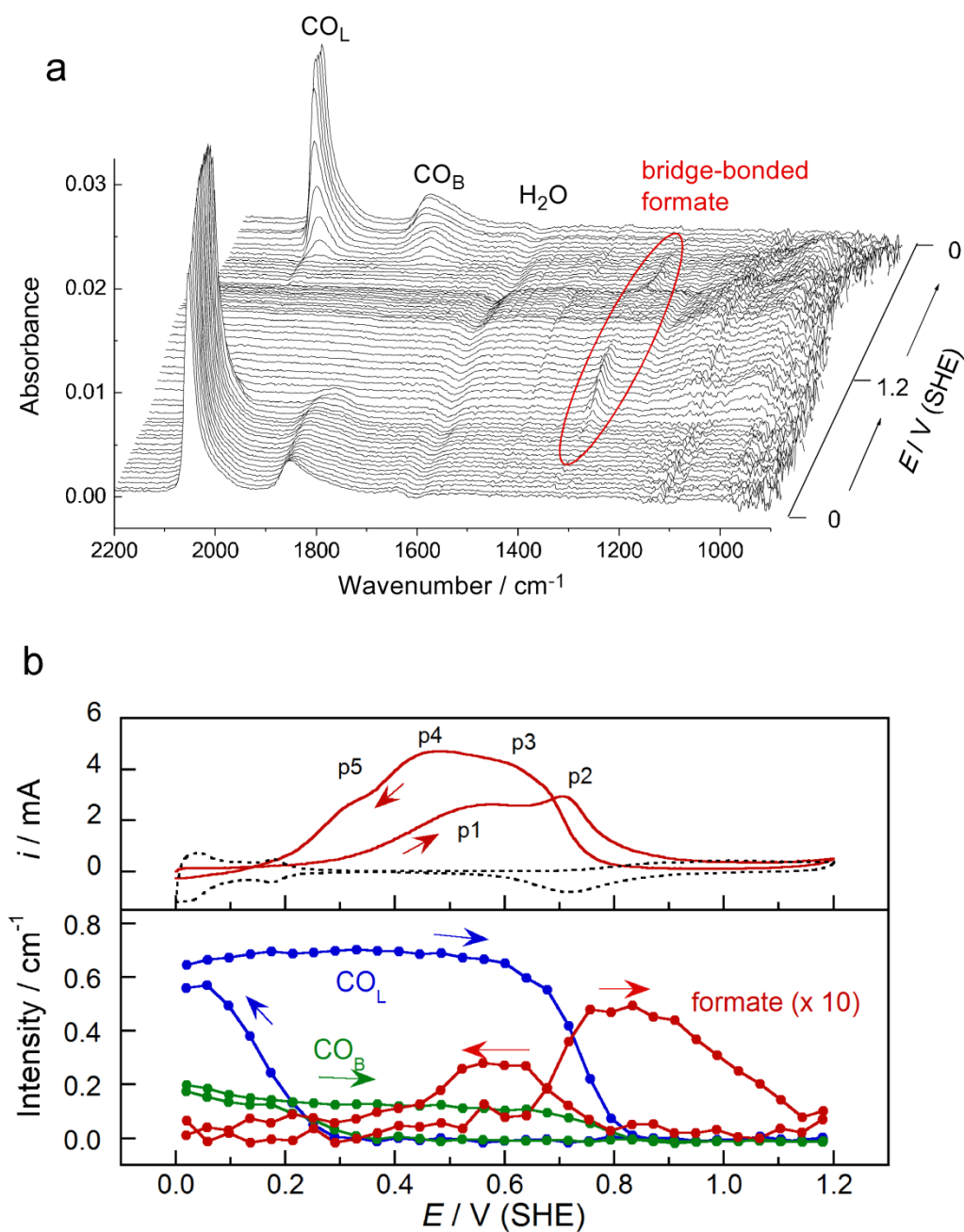
Figure 4.3. (a) SEIRA spectra of the surface of a Pt thin film electrode sequentially collected during a potential sweep from 0 to 1.2 and back to 0 V at 20\text{ mV s}^{-1} in buffer solution with pH 1.5
