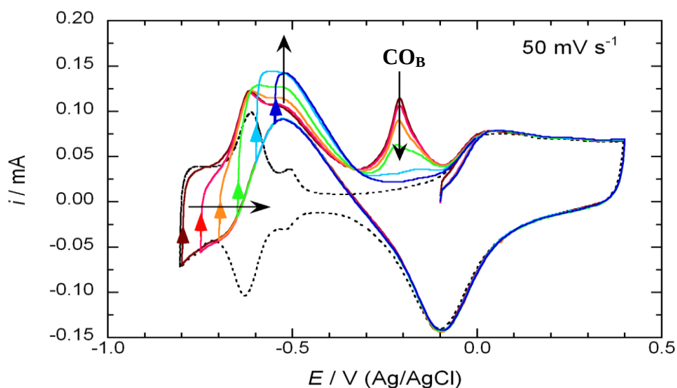
Figure 4.8. Variance of CV measured at 50 \text{ mV s}^{-1} on Pt in 0.1 \text{ M NaOH} and 10 \text{ mM HCOONa} as a function of lower potential limit. Initial potential is -0.1 \text{ V} and then potential is scanned in the forward direction and back to lower potential limit.
