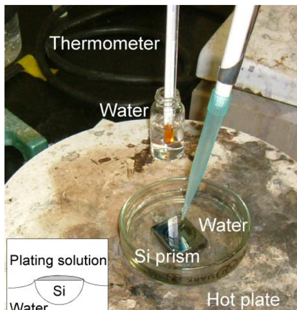
Figure 2.4. Chemical deposition of a thin Pt film on Si on a hot plate. The temperature of the prism is kept at 60°C by immersing water bath.
