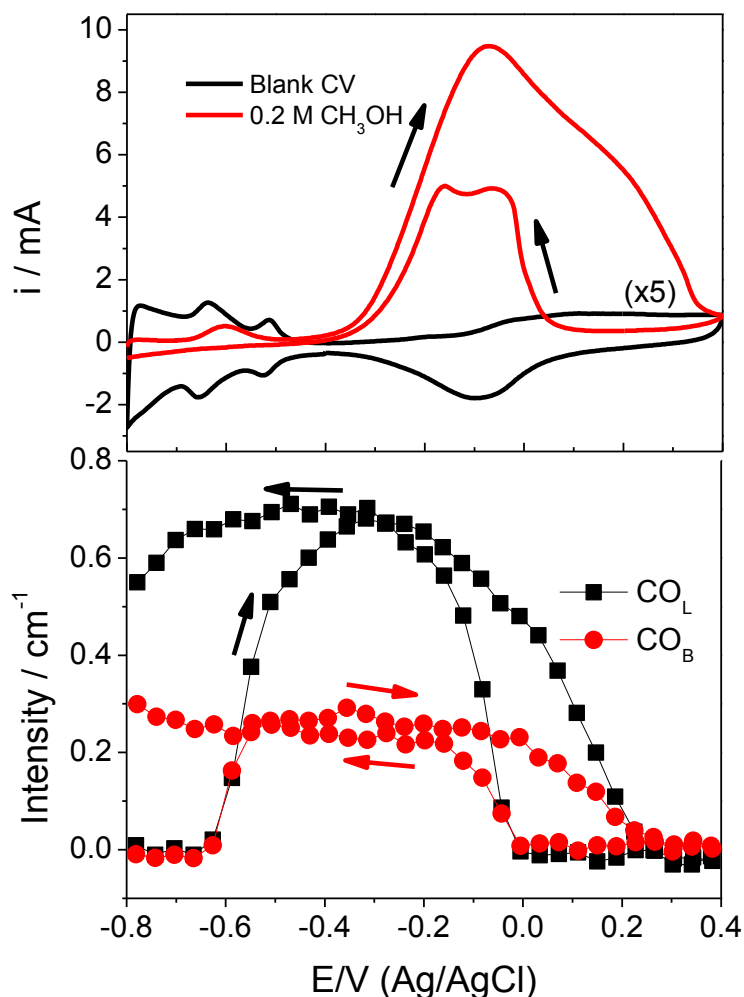
Figure 5.7. CV recorded simultaneously with the SEIRA spectra (upper) and the potential dependence of the integrated intensities of \text{CO}_L and \text{CO}_B at 20 \text{ mV s}^{-1} in buffer solution with pH 11.6 containing 0.2 \text{ M CH}_3\text{OH} . The solid line is the CV in the same electrolyte without \text{CH}_3\text{OH} .
