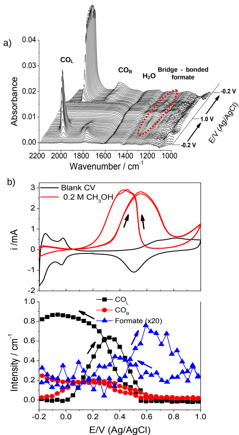
Figure 5.5. (a) SEIRA spectra of the surface of a Pt thin film electrode sequentially collected during a potential sweep from -0.2 to 1.0 and back to -0.2 V at 20 \text{mV s}^{-1} in buffer solution with pH 1.5 containing 0.2 M \text{CH}_3\text{OH} . (b) CV recorded simultaneously with the SEIRA spectra (upper) and
