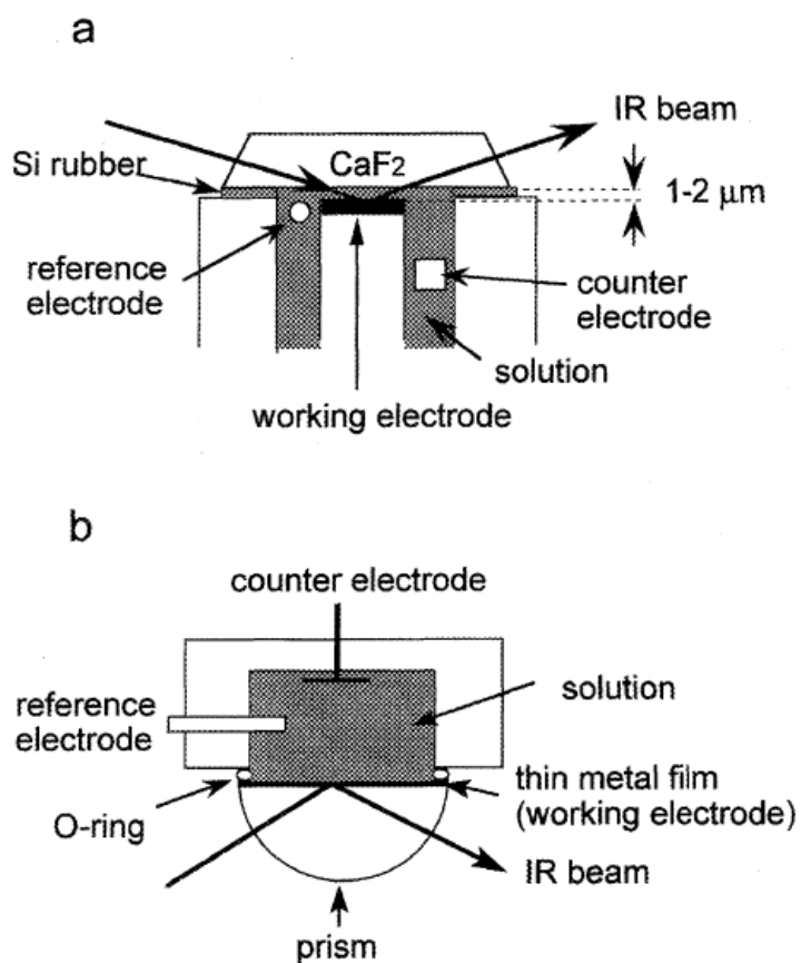
Figure 1.5. Electrochemical cells and optical arrangements used for in situ characterization of electrode/electrolyte interfaces with IRAS and ATR-SEIRAS techniques (a and b, respectively). Adopted from [57].
