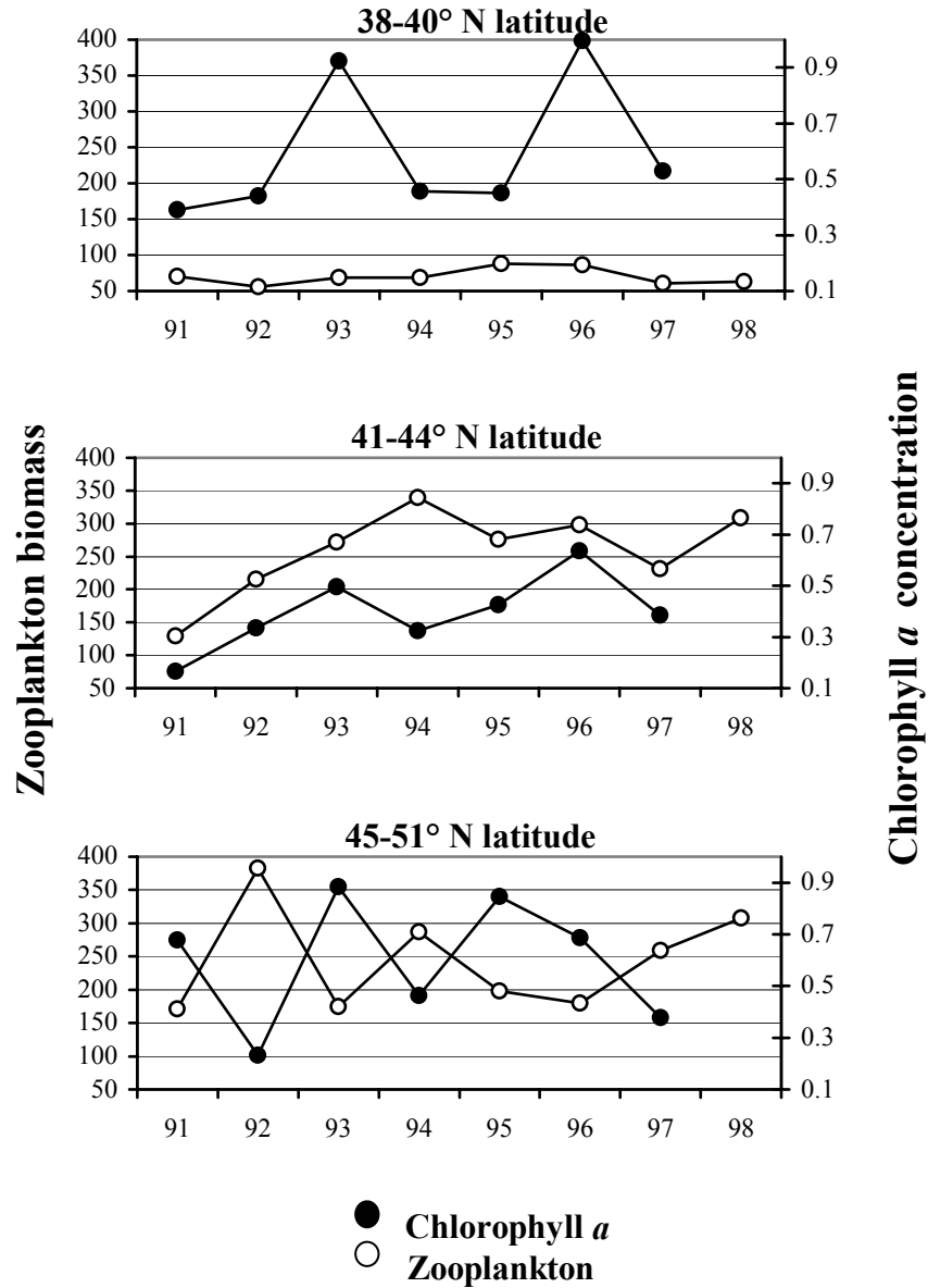
Figure 1.5. Comparison of mean chlorophyll a concentration (µg/l; 1991-1997) and mean zooplankton biomass (mg/m 3 ; 1991-1998) grouped by latitude along a transect at 180° longitude in the central North Pacific Ocean. Chlorophyll a data from Shiomoto et al. (1999), and zooplankton data from Tadokoro et al. (1995), Nagasawa and Ishida (1997, 1998), and Nagasawa and Ueno (1999).
