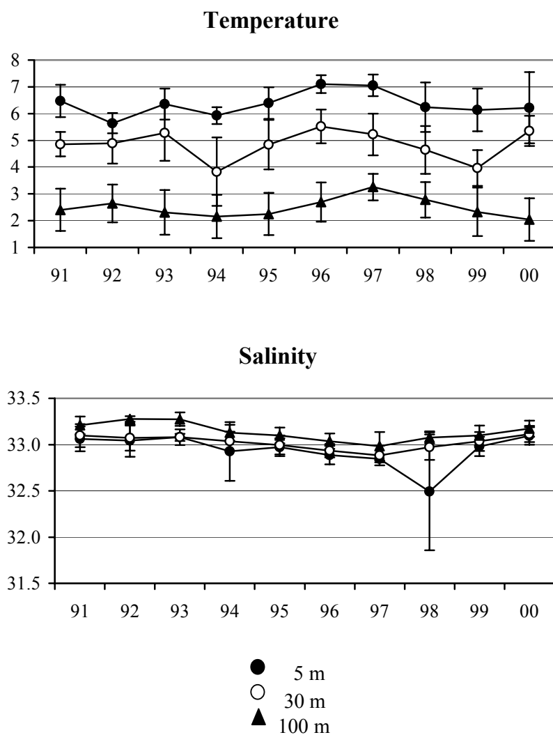
Figure 1.4. Seawater temperature (°C, upper panel) and salinity (psu, lower panel) at three depths along the transect at 180° longitude in the central Bering Sea, 1991-2000. Plotted values are the mean and \pm one standard deviation for data collected from 52-58°N latitude.
