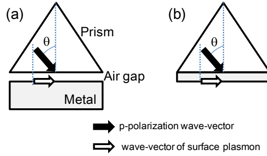
Figure 1.1 Otto configuration(a) and Kretschmann configuration(b).
