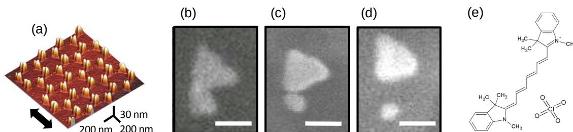
Figure 5.1. AFM image of the Ag-NSL substrate ( d = 350 nm) (a); SEM image of the Ag-NSL substrate (b-d), the second deposition angle \theta = 19^\circ (b), 21^\circ (c), 23^\circ (d), scale bar indicate 50 nm; the HITC molecular structure (e).
