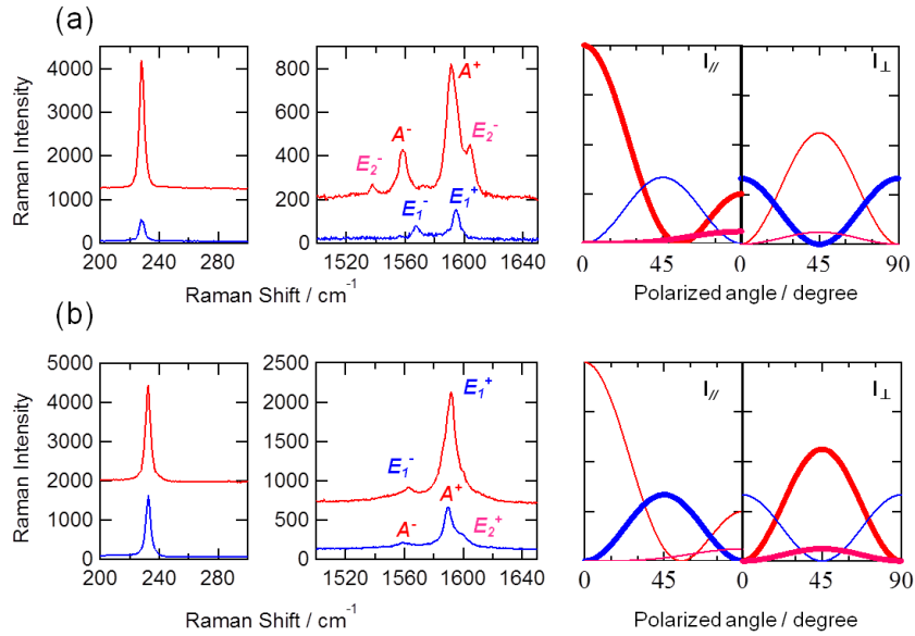
Figure 4.2 Polarized Raman spectra of different site, Excitation power I_{\text{ex}} = 0.2 \text{ mW} , exposure time t_{\text{ex}} = 1 \text{ s} . \omega_{\text{RBM}} = 228 \text{ cm}^{-1} , d = 1.04 \text{ nm} , semiconducting (10, 5) nanotube (a) and \omega_{\text{RBM}} = 233 \text{ cm}^{-1} , d = 1.00 \text{ nm} , semiconducting (11, 3) nanotube (b).
