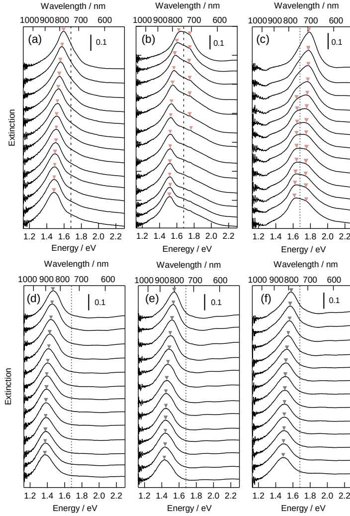
Figure 6.3 extinction spectra in 0.1 M NaClO 4 aqueous solution : Au20@HITC (a), Au30@HITC (b), Au40@HITC (c), Au20 (d), Au30 (e), Au40 (f), dotted line was exciton energy of HITC. The electrochemical potential were from +0.3 V of bottom to -0.9 V of top, spectra were acquired in each 0.1 V change.
