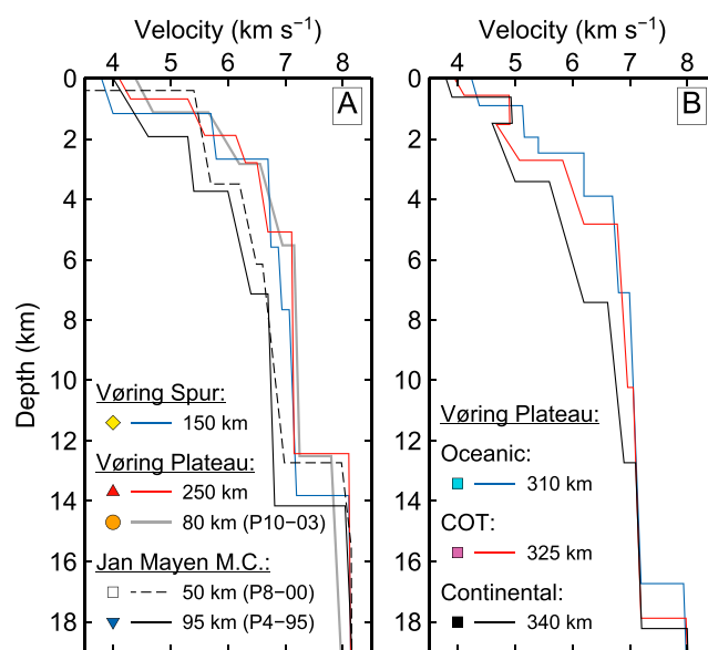
Figure 12. Profile 11-03 1-D velocity profiles compared between zones, to the northern Vøring Plateau, and to the Jan Mayen microcontinent. Zero depth is adjusted to the top of the first layer with velocity exceeding 3 \text{ km s}^{-1} . Kilometer values indicate 1-D positions along the modeled profiles. Color symbols refer to positions in Figures 1, 2, 9, and 13. (a) Typical Vøring Spur velocities are similar to that of the outer Vøring Plateau but higher than velocities of the Jan Mayen microcontinent from OBS Profile 8-00 [Breivik et al., 2012] and from OBS Profile 4-95 [Kodaira et al., 1998]. Outer Vøring Plateau velocities are also compared to a 1-D velocity profile from Profile 10-03 farther north on the plateau, at seafloor spreading anomaly 23. (b) Defining the continent-ocean transition (COT). The COT 1-D profile is in the middle of the hatched region at 325 km from Figure 9. The 1-D profile located 15 km seaward of that is similar to the outer margin and the Vøring Spur as seen in Figure 12a. Lower midcrustal velocities comparable to the Jan Mayen continental crust are found 15 km landward of the COT 1-D profile.
