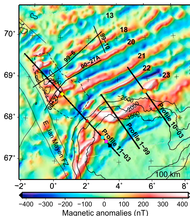
Figure 13. Magnetic map over the study area with OBS survey navigation, illuminated from the NW. The central part of the map is covered by the newer surveys RAS-03 and JAS-05 [Olesen et al. , 2007; Gernigon et al. , 2009], and marginal parts by the compilation of Verhoef et al. [1996]. Some bathymetric contours and the extent of thick oceanic crust (dashed line) under the Vøring Spur [Breivik et al. , 2008] are shown, and seafloor spreading anomalies are annotated. (Approximate ages: A23: 51.4 Ma, A22: 49.4 Ma, A21: 47.1 Ma, A20: 43.2 Ma, A18: 39.3 Ma, and A13: 33.3 Ma [Cande and Kent, 1995].) The positions of the MCS lines in Figure 16 are shown by thin black lines. Positions of 1-D velocity profiles shown in Figure 12 are indicated by color symbols.
