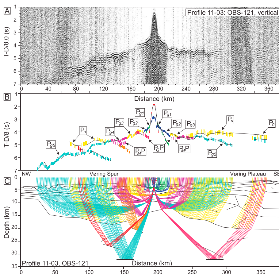
Figure 6. Data, interpretation, and ray tracing of OBS 121, Profile 11-03, Vøring Spur and Plateau. (a) OBS data, vertical component, and offset-dependent scaling. (b) Arrival time interpretation and model reproduction. Phase picks are shown by vertical bars, where the height of the bar shows interpretation uncertainty. Calculated times for each phase are shown by solid black lines. (c) Ray tracing of the velocity model. Ray colors correspond to the pick bar colors in Figure 6b.
