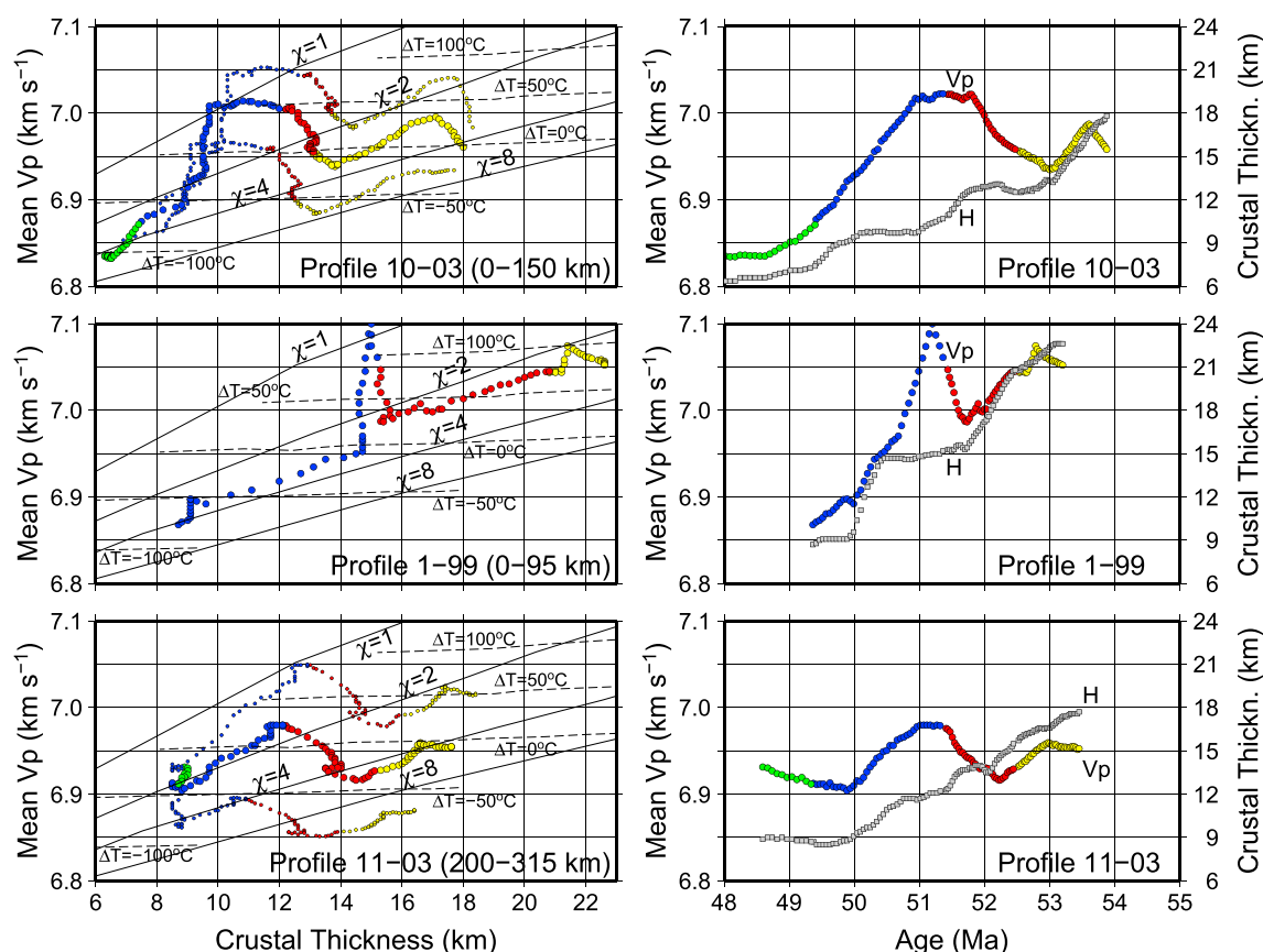
Figure 14. (left column) Crustal thickness variations plotted against mean V_p of the igneous crust for Profile 11-03, Profile 1-99, and Profile 10-03, using the Holbrook et al. [2001] corrections. Sampling interval is 1 km horizontally. The mantle melting curves indicate the degree of active upwelling ( \chi = 1 is passive), while \Delta T shows deviation from a normal potential mantle temperature of 1280°C. Small symbols indicate minimum and maximum velocity models. (right column) The same data plotted against age for Profile 11-03, Profile 1-99, and Profile 10-03. Crustal thickness ( H ) is shown by gray squares, while mean velocity ( V_p ) is shown by color-filled circles. Colors indicate position relative to magnetic seafloor spreading anomalies (Figure 14, left and right columns). Yellow: from COT to A24a, red: A24a to A23, blue: A23 to A22, and green: A22 to A21.
