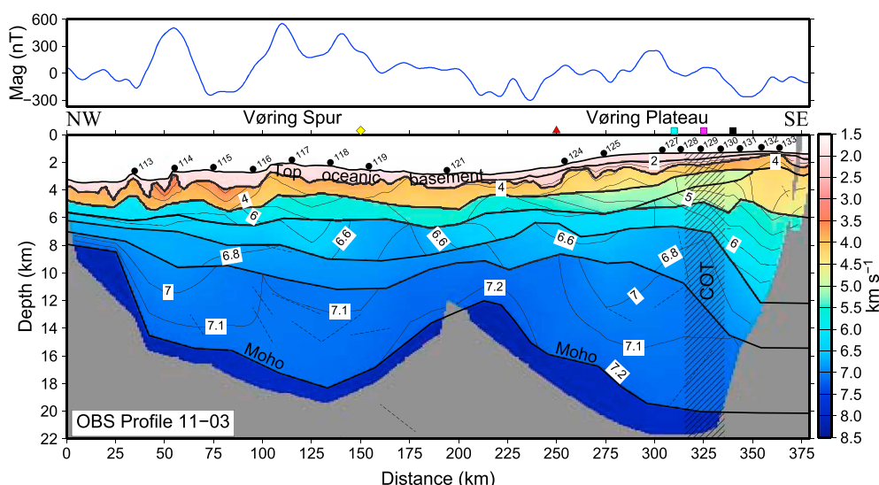
Figure 9. Gridded crustal velocity model of Profile 11-03. See Figure 2 for location. The parts of the model not covered by rays are masked; floating reflectors (dashed lines) do not constrain velocity and are not included in the ray coverage. The OBS/H locations are numbered on the seafloor. Hachures indicate the continent-ocean transition (COT). Velocity contour interval is 0.2 \text{ km s}^{-1} , except for the lowermost crustal layer where it is 0.1 \text{ km s}^{-1} . Positions of 1-D velocity profiles shown in Figure 12 are indicated by their respective color symbols. The magnetic track collected along profile is shown above.
