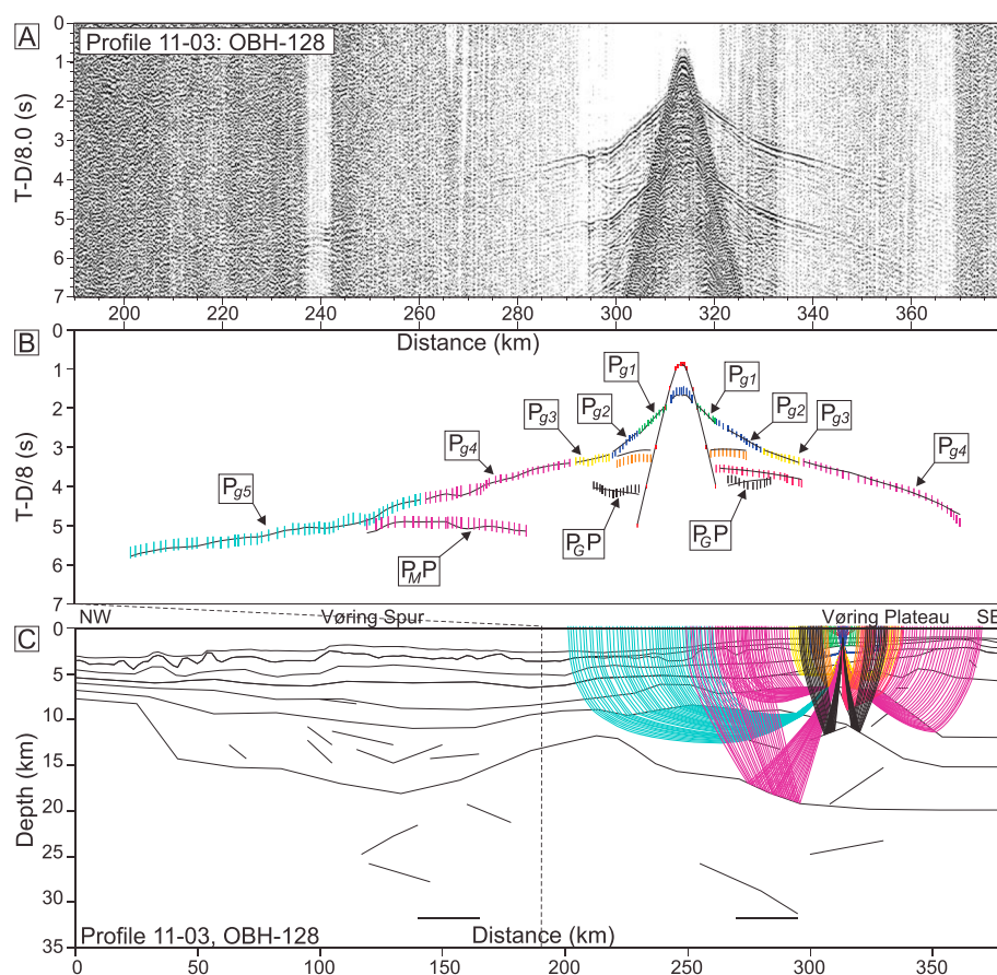
Figure 8. Data, interpretation, and ray tracing of OBH 128, Profile 11-03, Vøring Plateau. (a) Hydrophone data and offset-dependent scaling. (b) Arrival time interpretation and model reproduction. Phase picks are shown by vertical bars, where the height of the bar shows interpretation uncertainty. Calculated times for each phase are shown by solid black lines. (c) Ray tracing of the velocity model. Ray colors correspond to the pick bar colors in Figure 8b.
