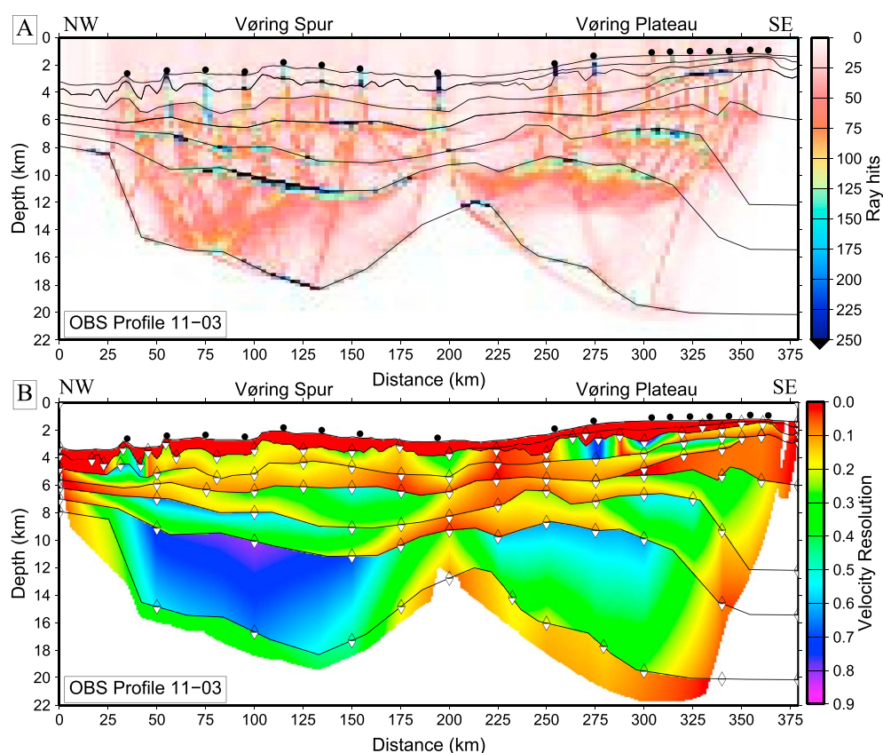
Figure 10. Ray coverage and velocity node resolution. (a) Gridded ray coverage of the Profile 11-03 velocity model, excluding floating reflectors. The binning is 2.5 km horizontally and 0.25 km with depth. (b) Gridded resolution parameters of the P wave velocity nodes obtained from inversion, omitting the water layer. Velocity nodes in the top and bottom of the layers are shown in white inverted triangles and transparent triangles, respectively.
