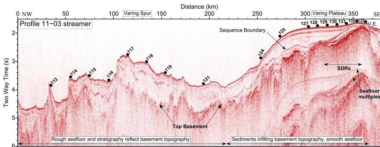
Figure 3. Single-channel streamer reflection seismic data of Profile 11-03. OBS/H locations are shown with filled black circles, with the instrument number above. SDRs: Seaward Dipping Reflectors; VE: Vøring Escarpment.
