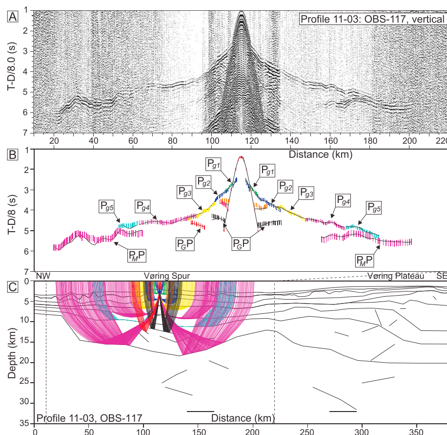
Figure 5. Data, interpretation, and ray tracing of OBS 117, Profile 11-03, Vøring Spur. (a) OBS data, vertical component, and offset-dependent scaling. (b) Arrival time interpretation and model reproduction. Phase picks are shown by vertical bars, where the height of the bar shows interpretation uncertainty. Calculated times for each phase are shown by solid black lines. (c) Ray tracing of the velocity model. Ray colors correspond to the pick bar colors in Figure 5b.
