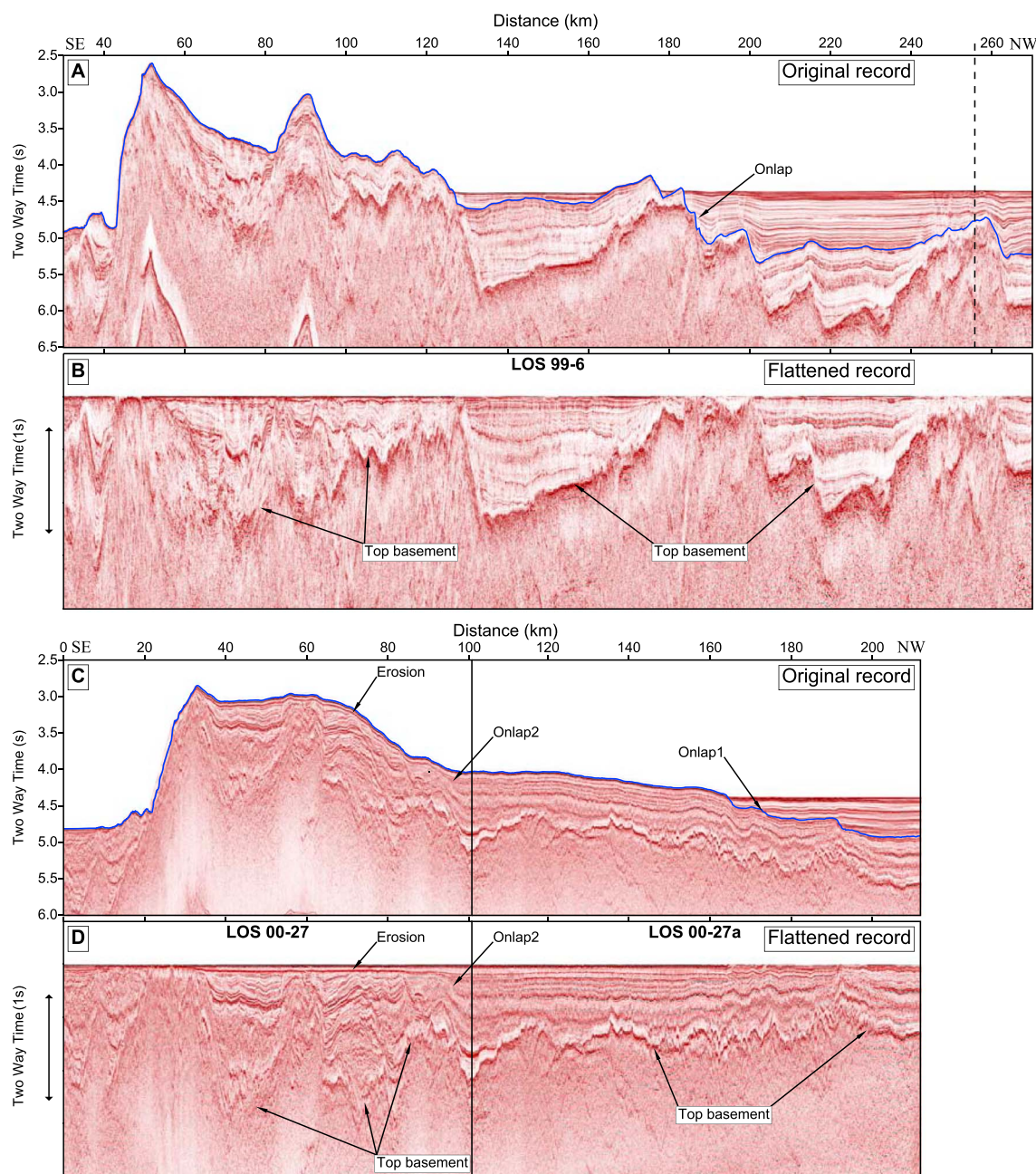
Figure 16. Sediment deposition pattern over and around the Vøring Spur. The main unconformity associated with uplift of the high is indicated by blue lines, extended along bathymetry over the high, used to reconstruct preuplift geometry. Locations are shown in Figures 2 and 13. (a) LOS 99-6, tie to LOS 99-10 (Figure 17) is shown by dashed line. (b) LOS 99-6 flattened on seafloor/unconformity. (c) LOS 00-27/27a composite line showing the sedimentation pattern along a seafloor lineation from where it is buried in the basin to become exposed in the Vøring Spur. (d) Flattened on seafloor/unconformity (Onlap1). Onlap within the deepest sedimentary section (Onlap2) shows an earlier inversion event. Some early erosion of sediments can be seen on the northern flank of the Vøring Spur.
