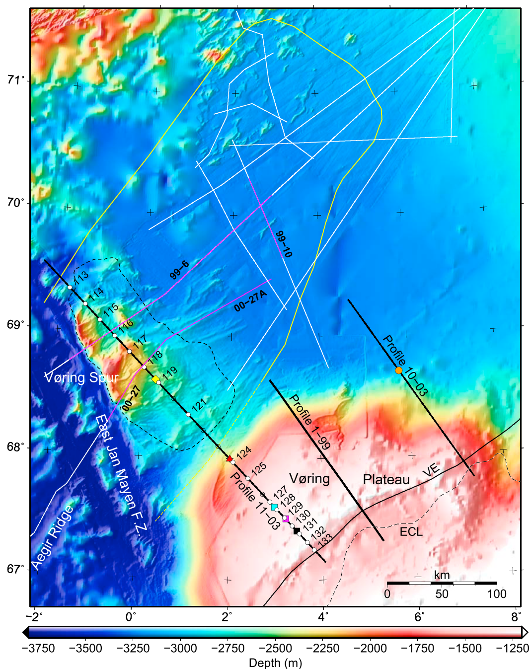
Figure 2. International Bathymetric Chart of the Arctic Ocean (IBCAO) (v.2) bathymetry [Jakobsson et al., 2008] with high-resolution side scan bathymetry overlay. The location of OBS profiles discussed is shown with black lines. Instrument locations for Profile 11-03 are marked with circles; those returning useful data are white filled and annotated. Multichannel seismic (MCS) survey lines are shown in white, with seismic example locations marked in magenta. Dashed line shows extent of thick crust under the Vøring Spur, while yellow line shows the extent of the inversion event mapped from the MCS profiles [Breivik et al., 2008]. Positions of additional 1-D velocity profiles shown in Figure 12 are indicated by color symbols. ECL: Eastern limit Cenozoic lavas; VE: Vøring Escarpment [Skogseid, 1994].
