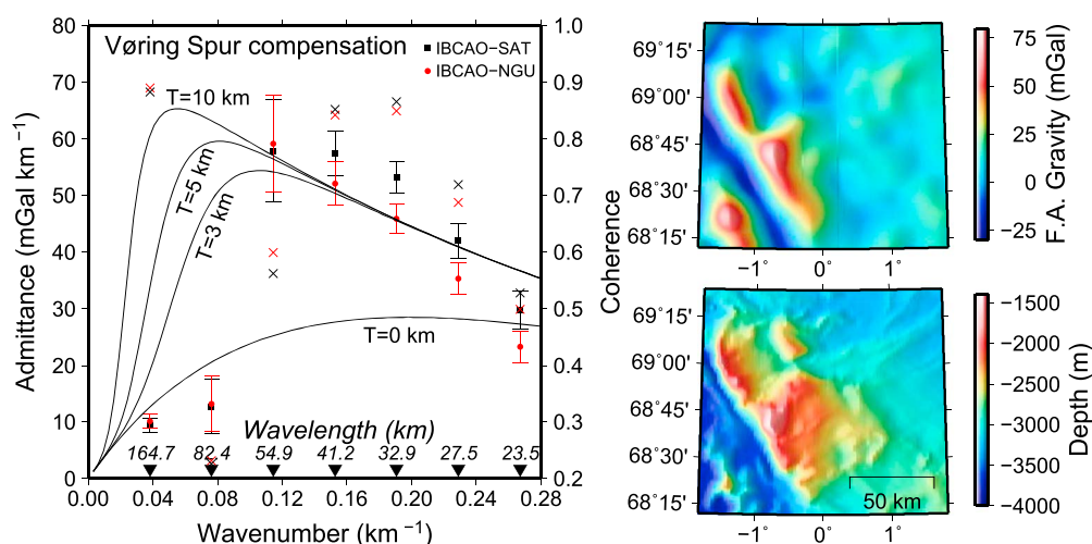
Figure 18. The admittance function (red and black filled symbols with 1\sigma error bars) between two different free-air gravity grids and IBCAO (v.2) bathymetry for the Vøring Spur. See text for details. On the right-hand side, we show the IBCAO (v.2) bathymetry and the DTU10 satellite gravity used. The results are compared to four different elastic plate thicknesses (0, 3, 5, and 10 km), documenting a very low plate strength. The coherence at the specific wavelengths is shown by crosses.
