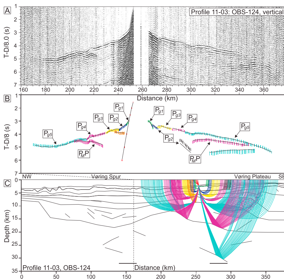
Figure 7. Data, interpretation, and ray tracing of OBS 124, Profile 11-03, Vøring Plateau. (a) OBS data, vertical component, and offset-dependent scaling. (b) Arrival time interpretation and model reproduction. Phase picks are shown by vertical bars, where the height of the bar shows interpretation uncertainty. Calculated times for each phase are shown by solid black lines. (c) Ray tracing of the velocity model. Ray colors correspond to the pick bar colors in Figure 7b.
