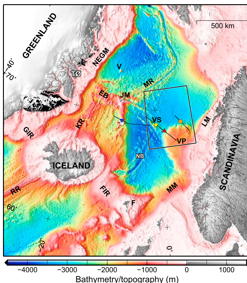
Figure 1. Regional location map based on ETOPO-2 bathymetry/topography [Sandwell and Smith, 1997] showing positions of various features discussed in the text. Black areas onshore Greenland indicate early Cenozoic basalt flows or intrusions. AR: Aegir Ridge, EB: Eggvin Bank, F: Faeroes, FIR: Faeroes-Iceland Ridge, GIR: Greenland-Iceland Ridge, JM: Jan Mayen, KR: Kolbeinsey Ridge, LM: Lofoten Margin, MM: Møre Margin, MR: Mohn Ridge, NB: Norway Basin, NEGM: North-east Greenland Margin, RR: Reykjanes Ridge, TØ: Traill Ø, VP: Vøring Plateau, VS: Vøring Spur, and V: Vesteris Seamount. Positions of some of the 1-D velocity profiles derived from ocean bottom seismometer (OBS) profiles shown in Figure 12a are indicated by color symbols. The frame shows the position of Figure 2.
