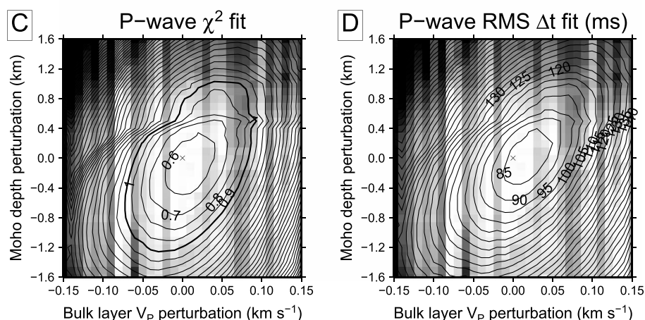
Figure 11. Profile 11-03 P wave model sensitivity to lower crustal velocity changes against Moho depth based on P_{g5} , P_{M5} , and P_n phases. (a and b) Model sensitivity for the outer Vøring Plateau; (c and d) model sensitivity for the Vøring Spur. Background shading indicates the ability of the model to trace arrivals to all observed locations. The shading starts at 2% loss and reaches black at 10% loss.
