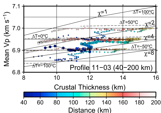
Figure 15. Crustal thickness variations plotted against mean V_p for the Vøring Spur from Profile 11-03, based on the corrections of Holbrook et al. [2001]. Small symbols indicate minimum and maximum velocity models derived from Figure 11. Color codes show position along model. Other symbols are as in Figure 14.
