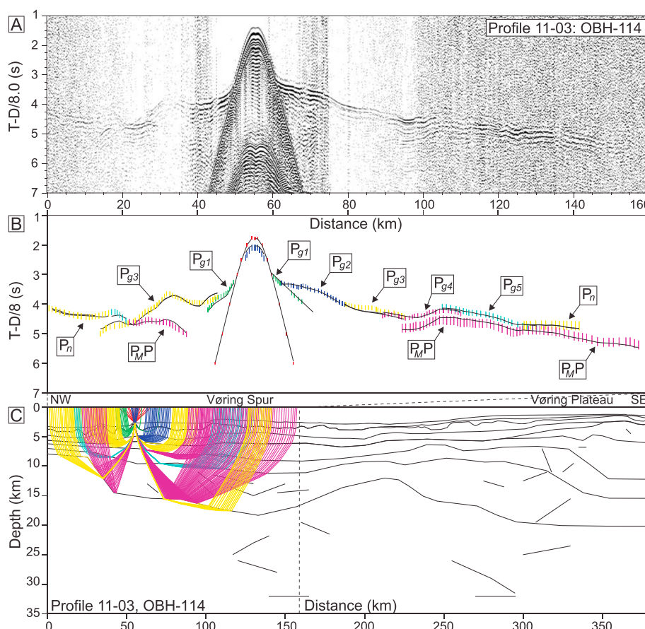
Figure 4. Data, interpretation, and ray tracing of OBH 114, Profile 11-03, Vøring Spur. (a) Hydrophone data, offset-dependent scaling. (b) Arrival time interpretation and model reproduction. Phase picks are shown by vertical bars, where the height of the bar shows interpretation uncertainty. Calculated times for each phase are shown by solid black lines. (c) Ray tracing of the velocity model. Ray colors correspond to the pick bar colors in Figure 4b.
