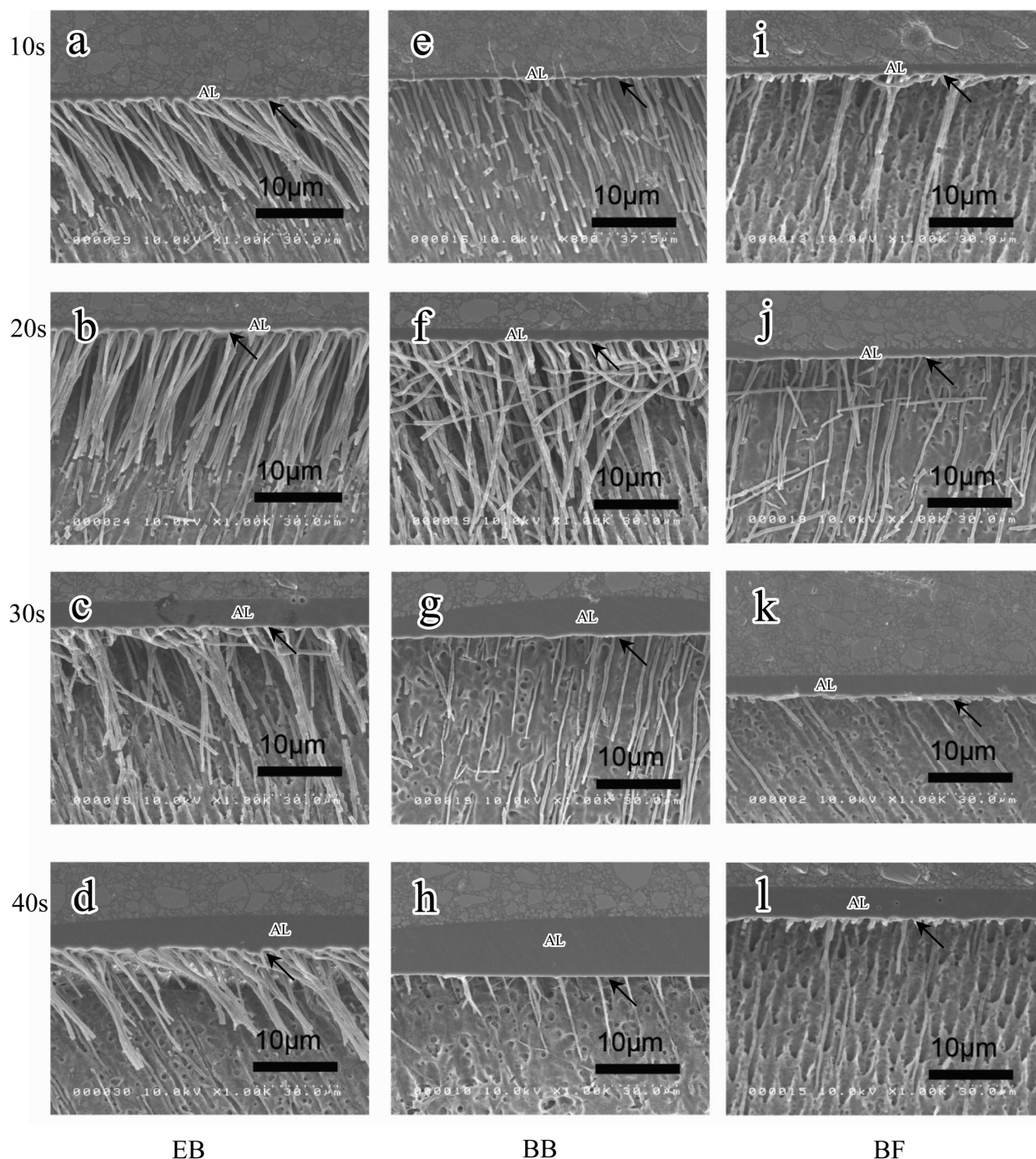
Fig. 4 The SEM observations for resin-dentin interface.
