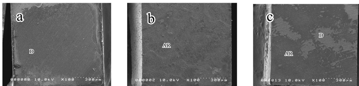
Fig. 2 Field-emission scanning electron micrographs of de-bonded samples show their fractured surfaces. (a) adhesive; (b) cohesive; (c) mixed. Abbreviations: adhesive resin (AR) ; dentin (D).
