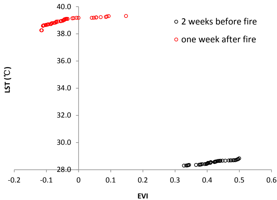
Figure 3-4 Fire-induced LST-EVI space changes in May, 2003
