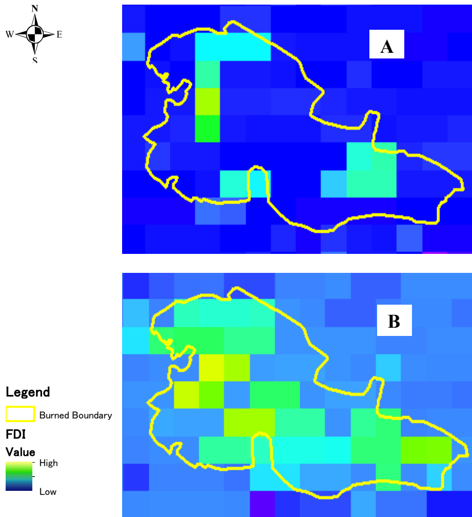
Figure 3-5 Fire Disturbance Index (FDI): 2 week before the fire (up), and one week after the fire (down). This illustrates that the abrupt impact that wildfire has on the landscape can be detected by FDI
