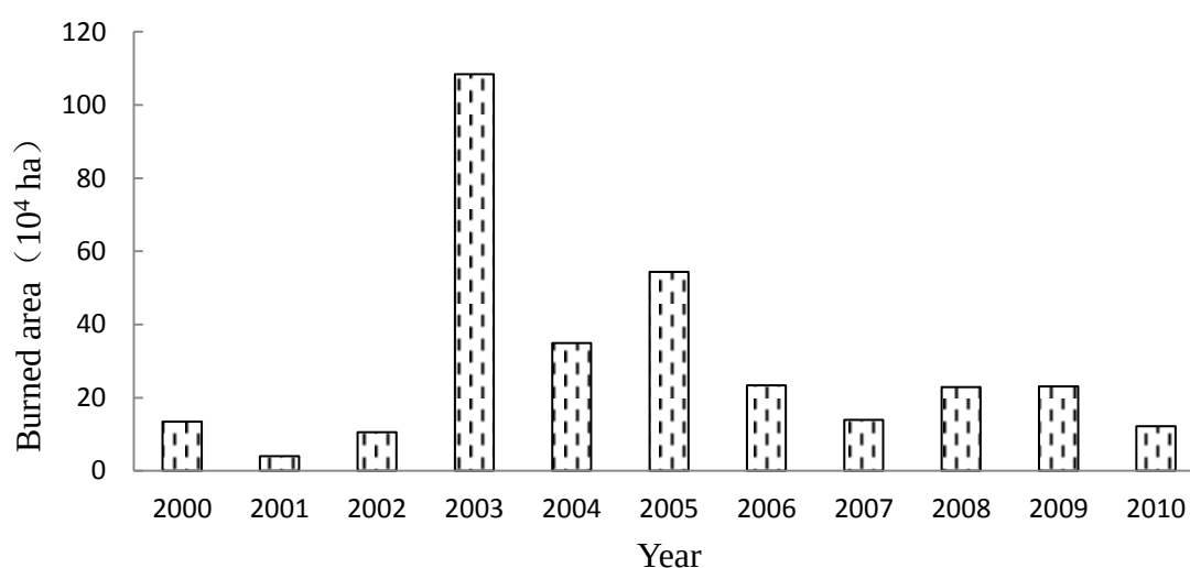
Figure 3-7 Total fire area in Northeast China from 2000 to 2010 according to MODIS data
