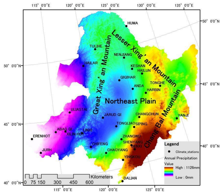
Figure 3-9 Meteorological parameters in Northeast China
