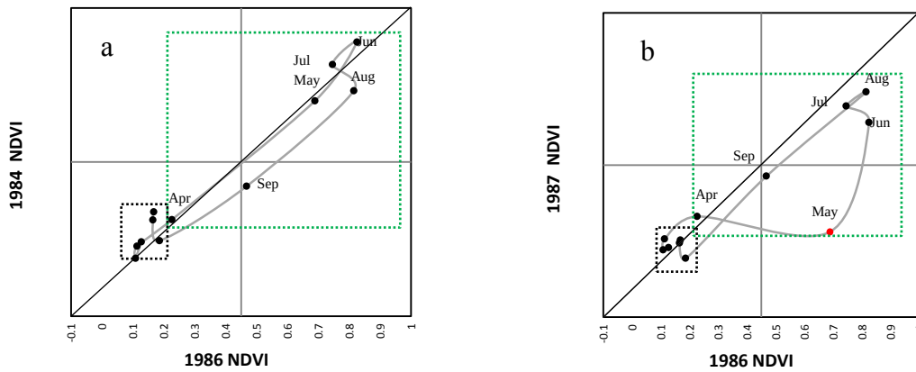
Figure 5-6 Monthly NDVI trajectories of a normal year (a) and the fire year (b). The points within the green box represent the growing season (April to October), while the points within the black box represent the snow cover season (November to March). The red point represents the month that the fire occurred
