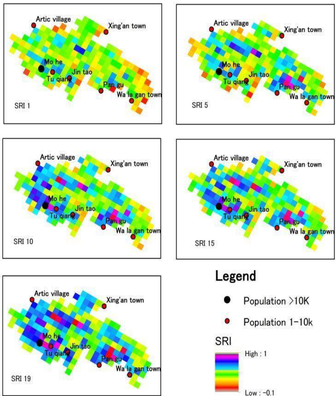
Figure 5-8 The trajectory of the post-fire stands regrowth index (SRI) for the relative year 1, 5, 10, 15 and 19
