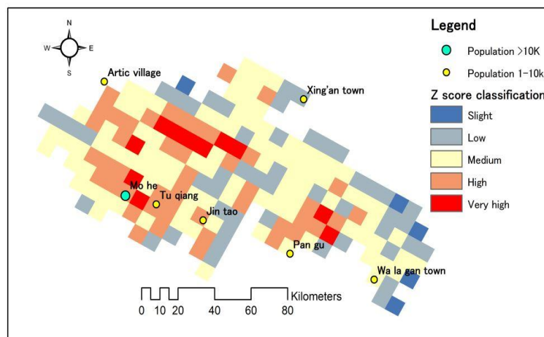
Figure 5-3 The fire damage of the entire burned area divided into five classes: Very high (VH), High (H), Moderate (M), Low (L) and Slight (S)
