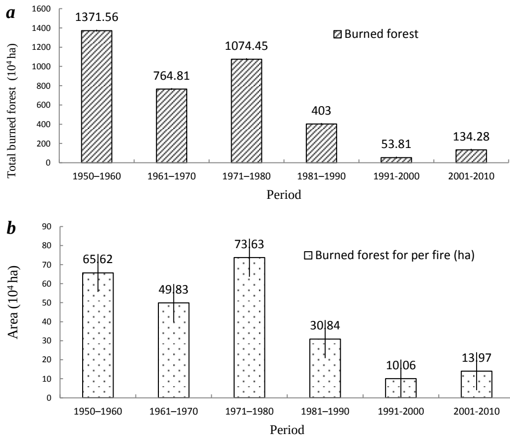
Figure 2- 4 Burned area shift in every 10 years period, Total burned forest area (a); average burned forest area for single fire (b)
