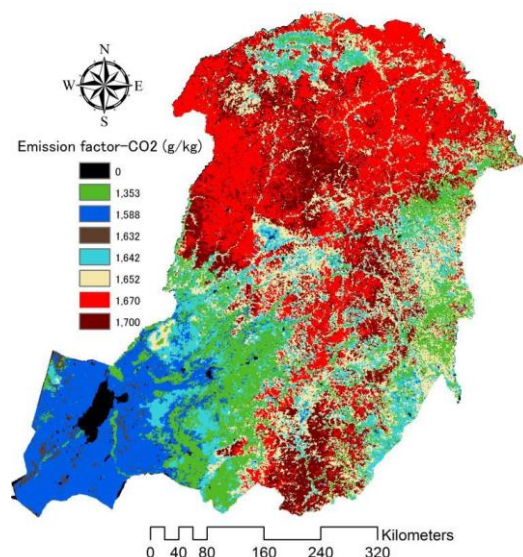
Figure 4-3 The determination of CO 2 emission factor in china. The emission factors of other emitted species (CH 4 , CO, PM 10 , PM 2.5 , SO 2 , BC and NO x ) were also determined in the same way
