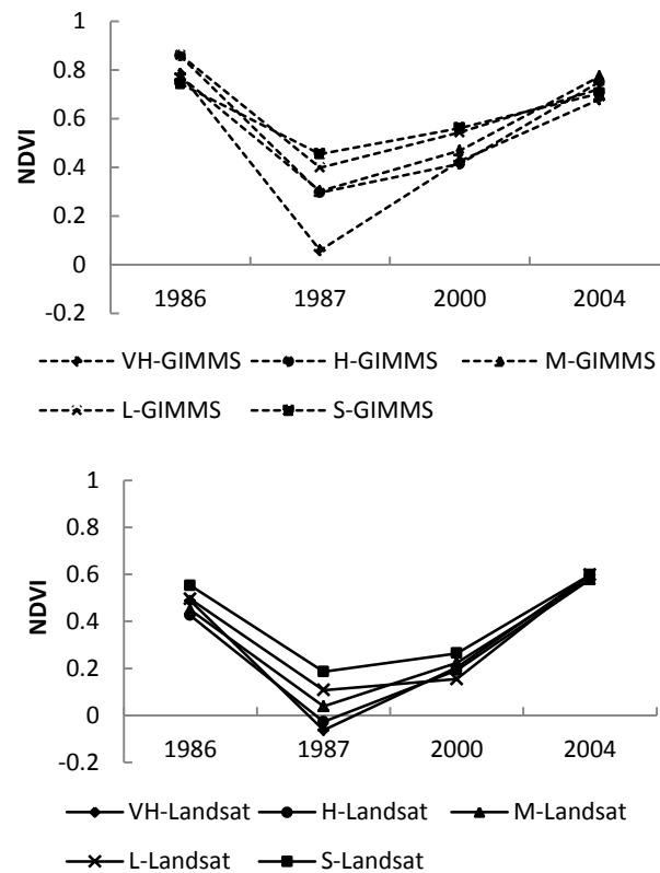
Figure 5- 11 Comparison GIMMS NDVI (up) with Landsat NDVI (down)
