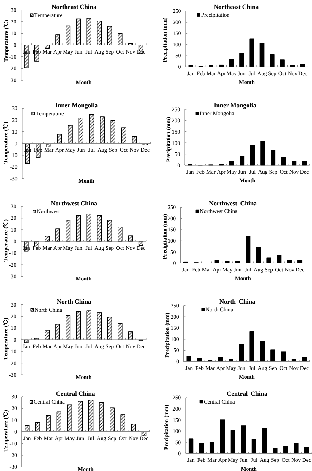
Figure 2- 14 Climate characteristics of each 9 sub-regions in China
