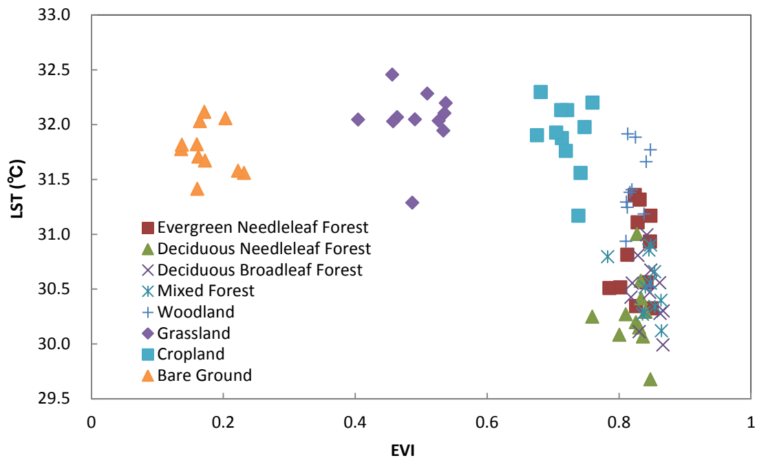
Figure 3- 2 Characteristics of various land-cover types in LST-EVI space in Northeast China
