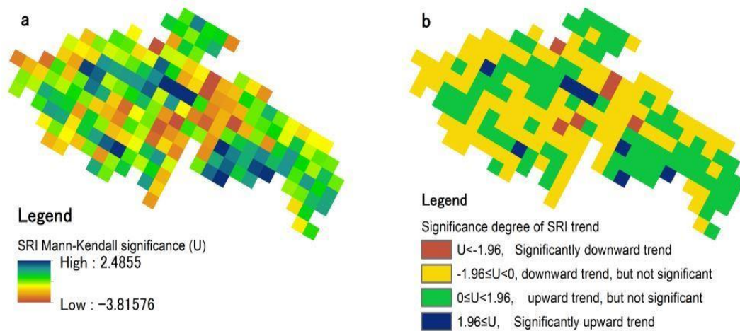
Figure 5-9 (a) The stands regrowth index (SRI) significance distribution using a non-parametric Mann-Kendall test and (b) the degree of significance degree for the post-fire stands regrowth index (SRI) trend using a non-parametric Mann-Kendall test.
