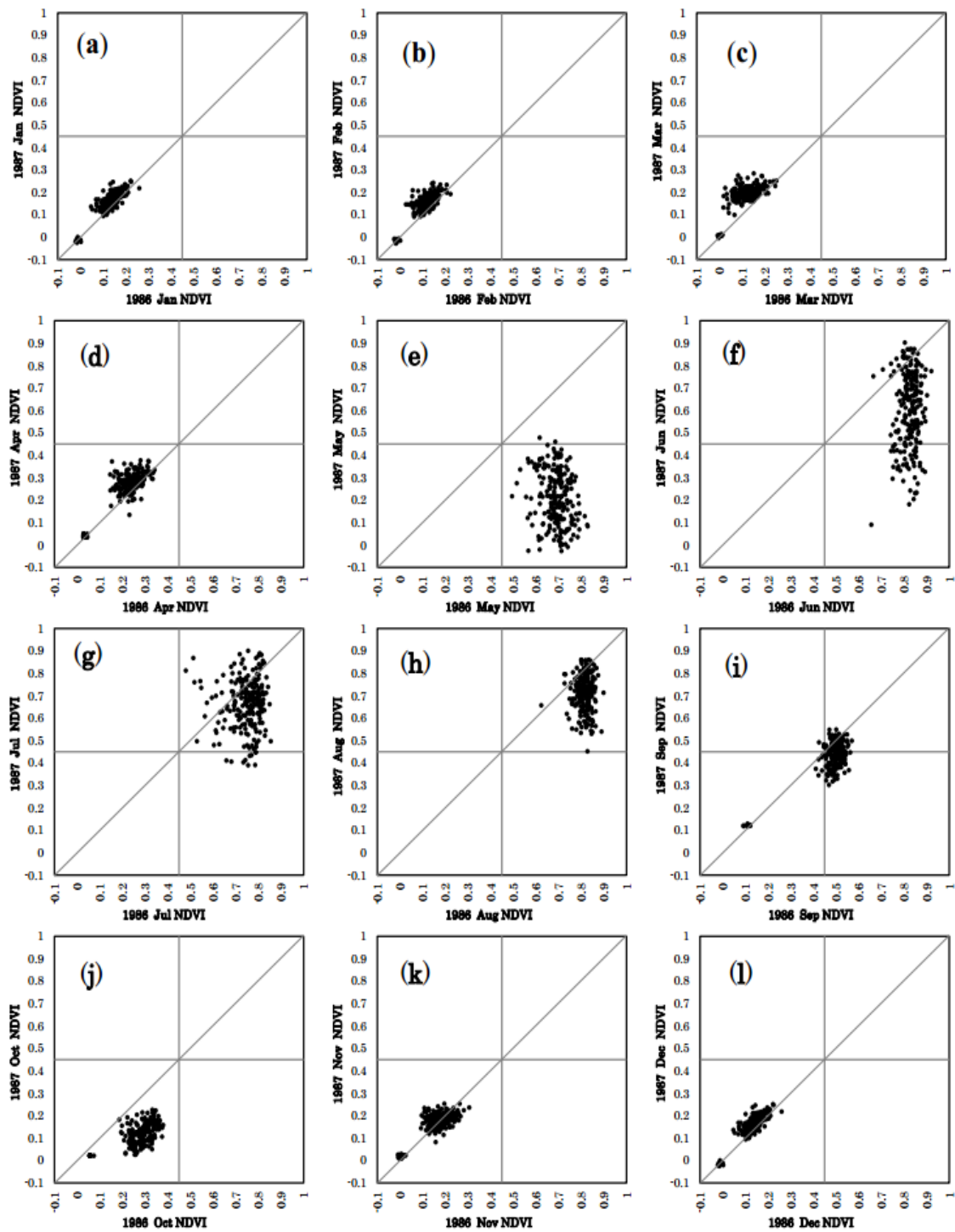
Figure 5- 5 Monthly scatterplots of post-fire NDVI (1987) versus pre-fire NDVI (1986) ((a) January, (b) February, (c) March, (d) April, (e) May, (f) June, (g) July, (h) August, (i) September, (j) October, (k) November, (l) December) for the large fire on May 1987
