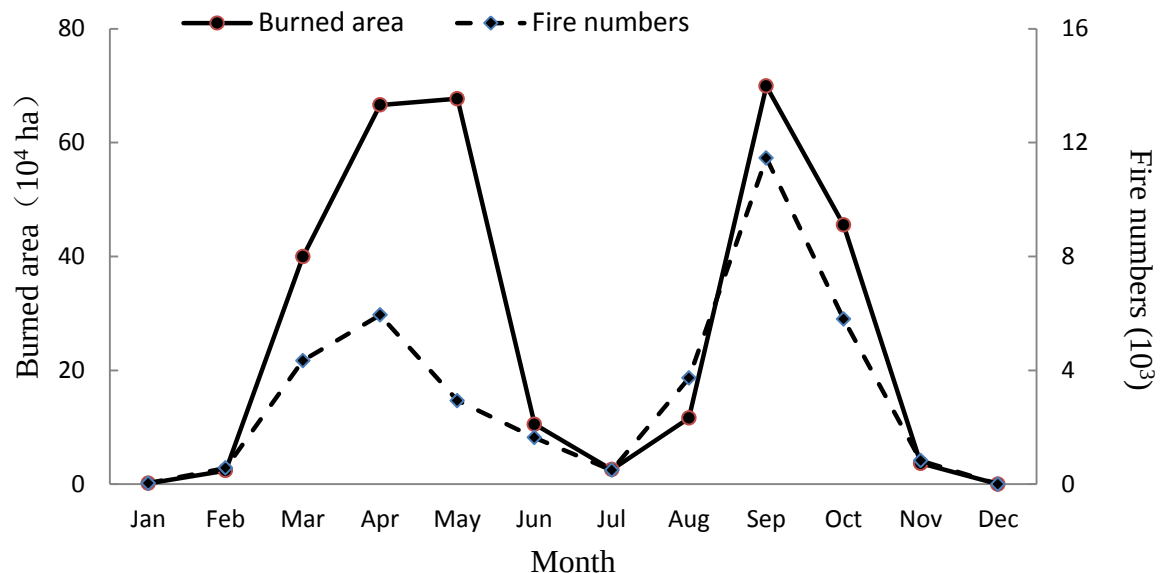
Figure 3-8 Seasonality of fire patterns in Northeast China. Here, the fire number is not the number of fire events but the number of fire patches in the MODIS image
