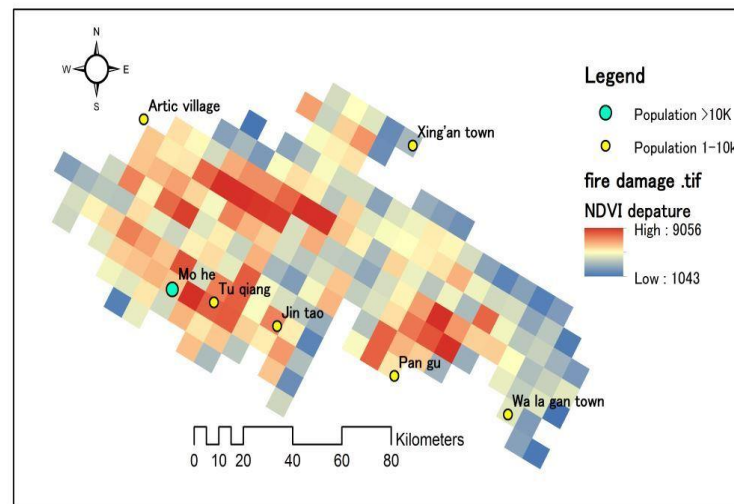
Figure 5- 2 Fire damage map of the study area for the 1987 fire event with fire damage values obtained using Equation 1
