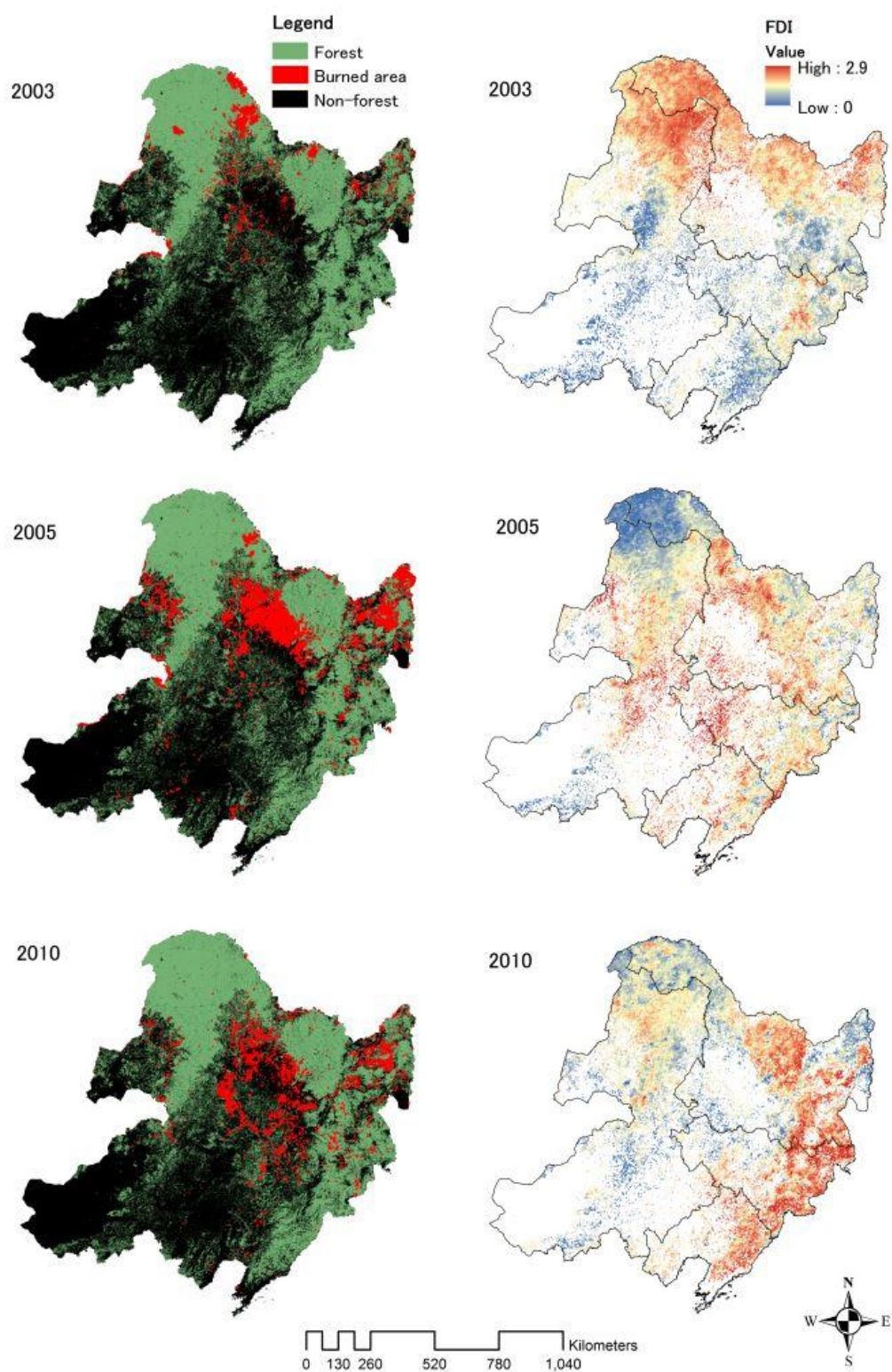
Figure 3-6 Validating the FDI algorithm (right) with MODIS burned area data (left) of three typical fire years in 2003, 2005 and 2010
