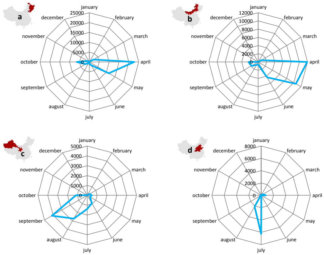
Figure 2- 11 Fire season patterns of each 9 sub-regions in China. For each region, width and length of the blue shape indicate the fire season duration and the amount of burned area, respectively.
