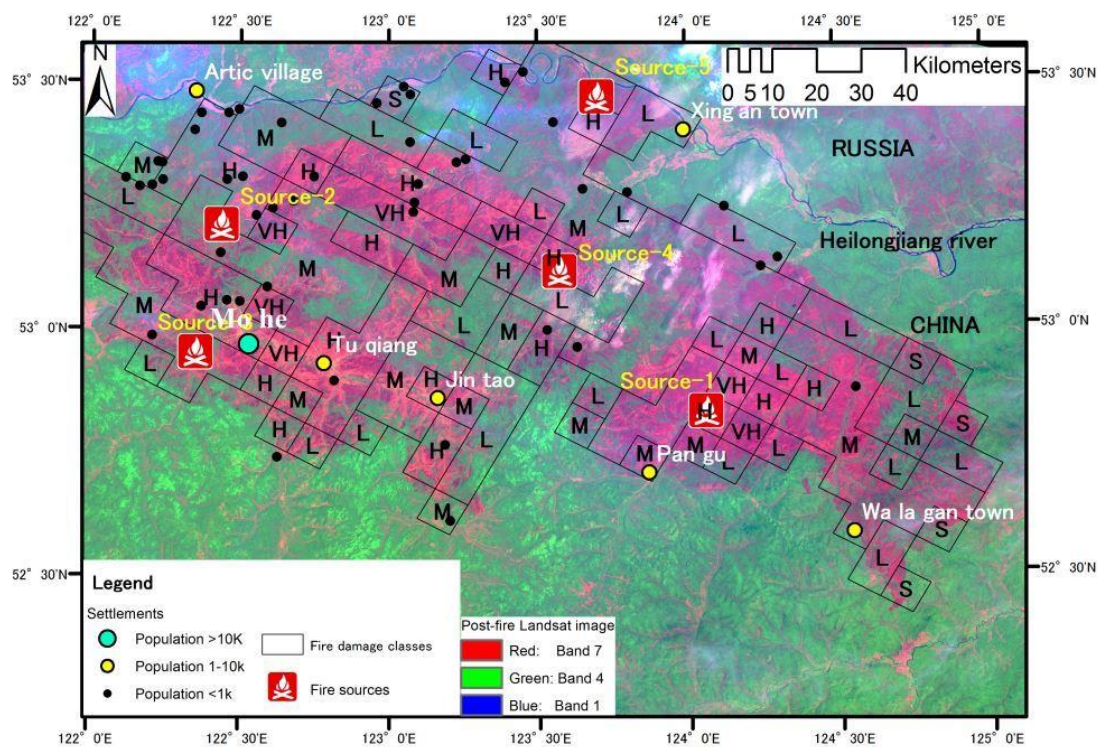
Figure 5-4 Fire sources and fire damage classes. The base map image is a composition of two Landsat 5 TM images from June 1987 (false color composite bands: red-band 7; green-band 4; blue-band 1)
