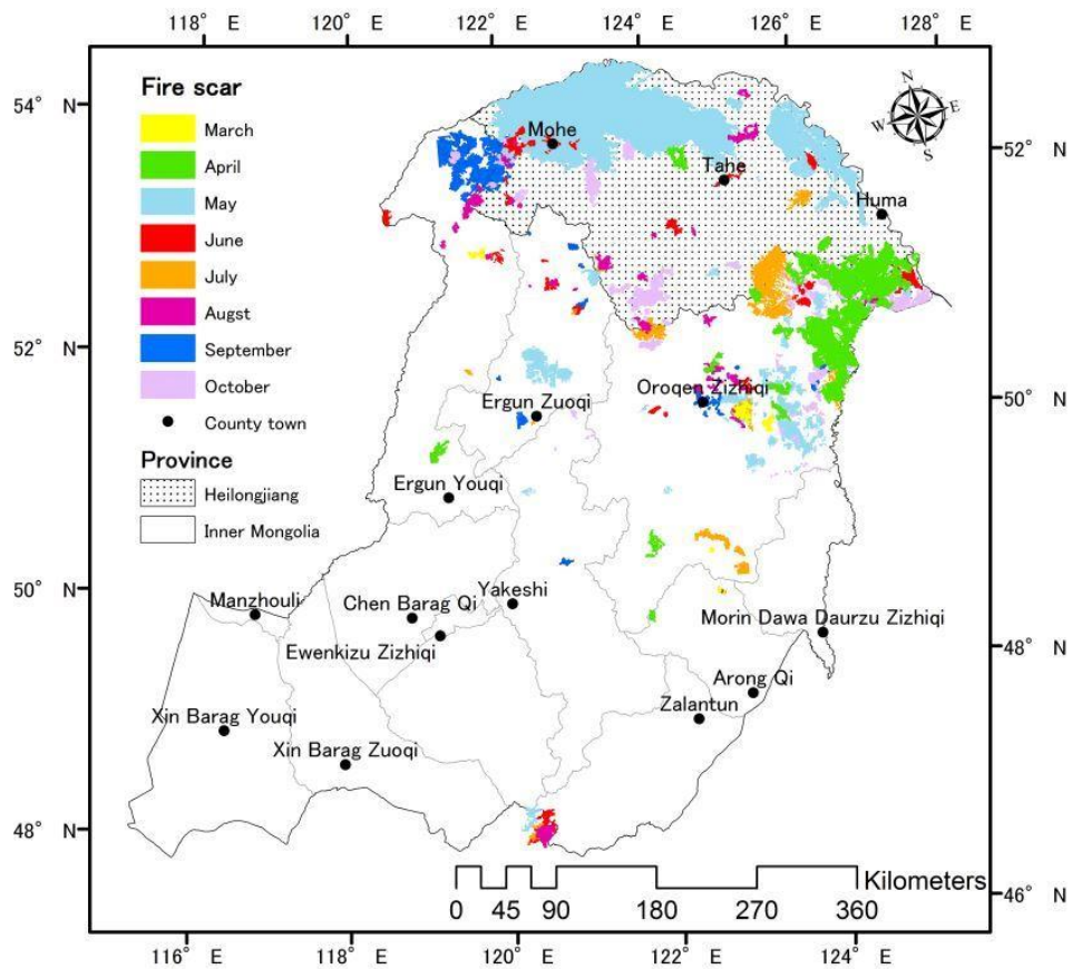
Figure 4-4 Burned areas distribution by month from 1986 to 2010. Only the fire scars which larger than 100 ha were showed in this figure. Note that the size of the burn scars increases slightly for the display purpose
