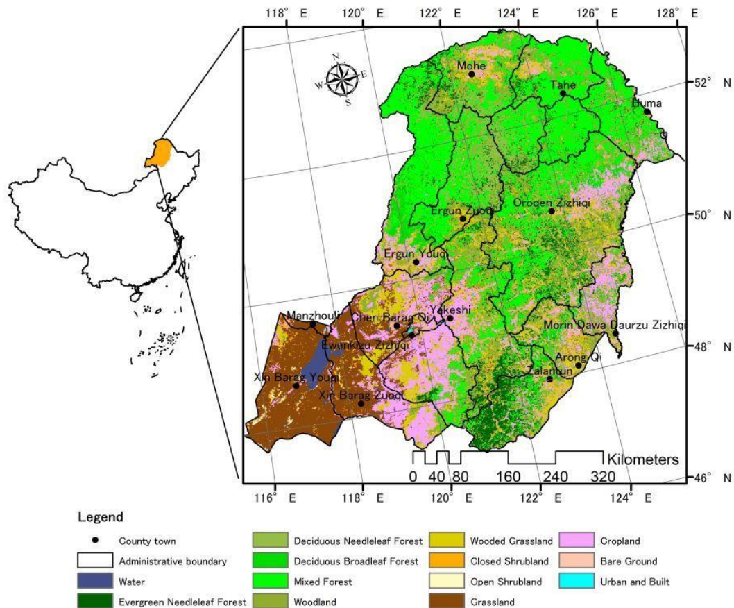
Figure 4- 1 Land cover distribution in the Great Xing'an Mountain. It is derived from University of Maryland global land cover map (UMD-GLC)
