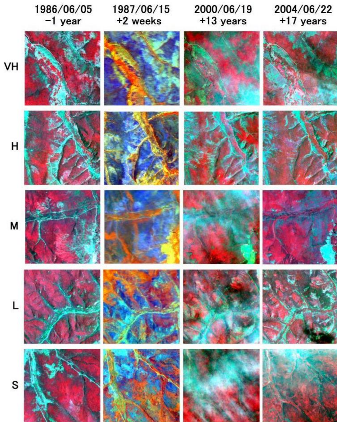
Figure 5-10 Landsat TM/ETM+ images (RGB:432) illustrating fire-caused changes on the ground vegetation. The locations of these five tracked samples can be found in Figure 5-4. Minus and plus signs represent pre-fire and post-fire period, respectively. Fire damage classes: Very High (VH); High (H); Moderate (M); Low (L); Slight (S)
