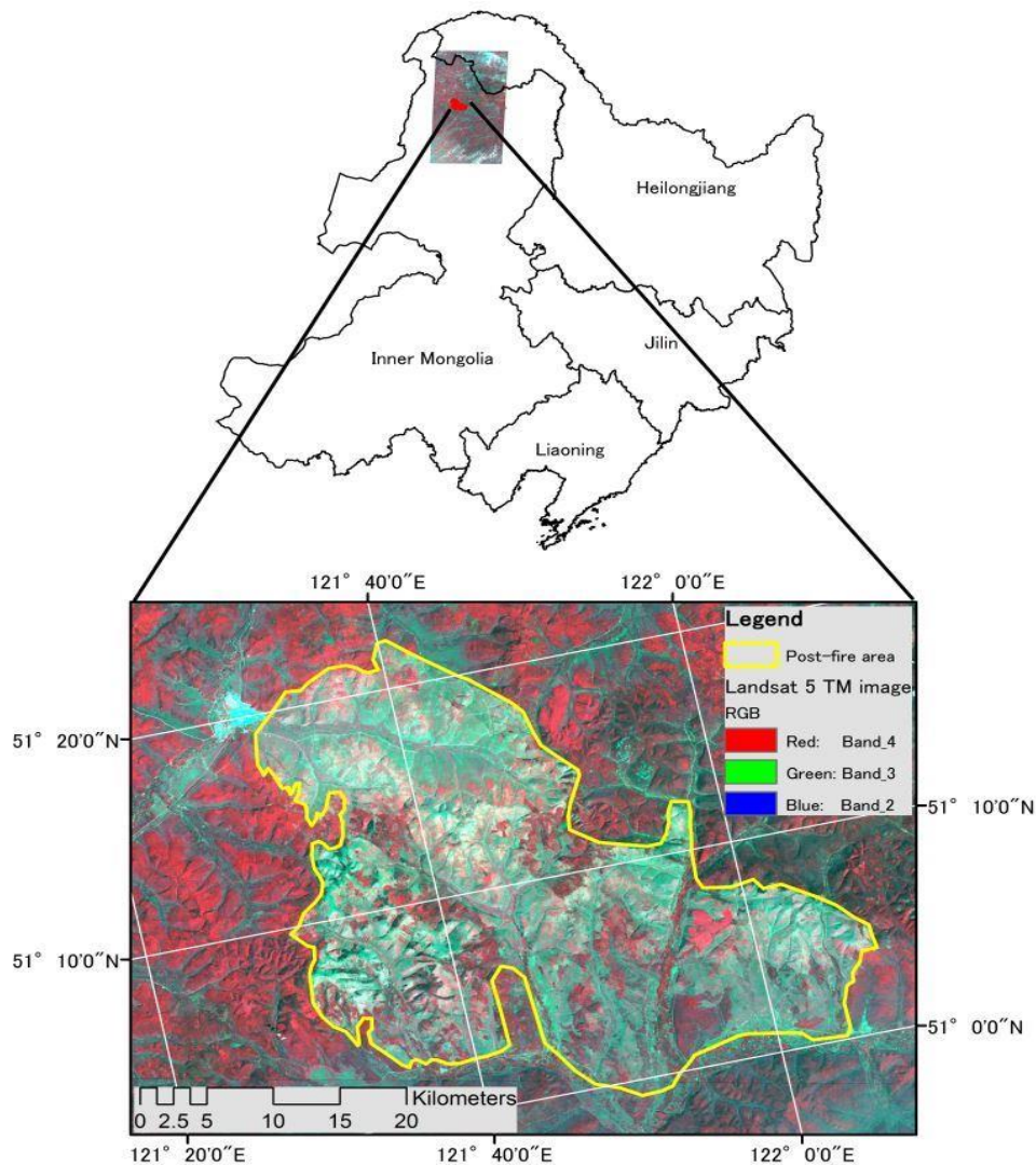
Figure 3- 3 Location of fire event in Inner Mongolia May, 2003
