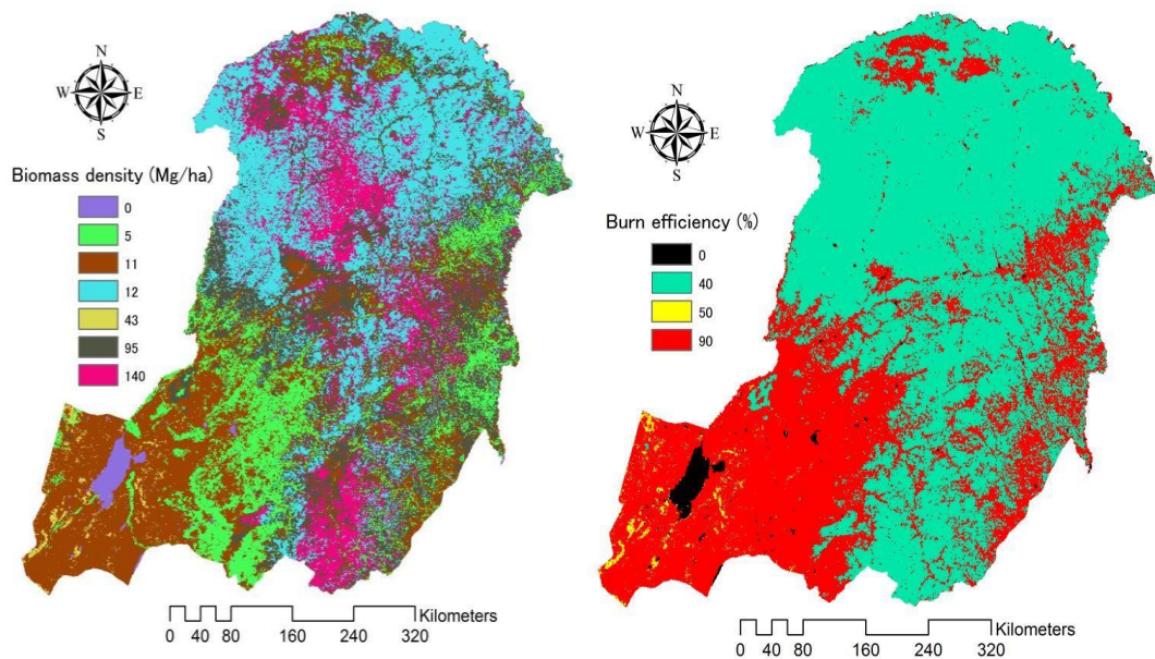
Figure 4-2 Biomass density (left) and burned efficiency (right) distribution in Great Xing'an Mountain
