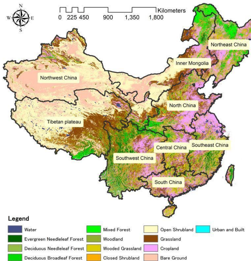
Figure 2-6 Sub-regions division and land cover characteristics in China. a, northeast China; b, inner Mongolia; c, northwest China; d, north China; e, central China; f, south China; g, southwest China; h, Tibetan plateau; i, southeast China
