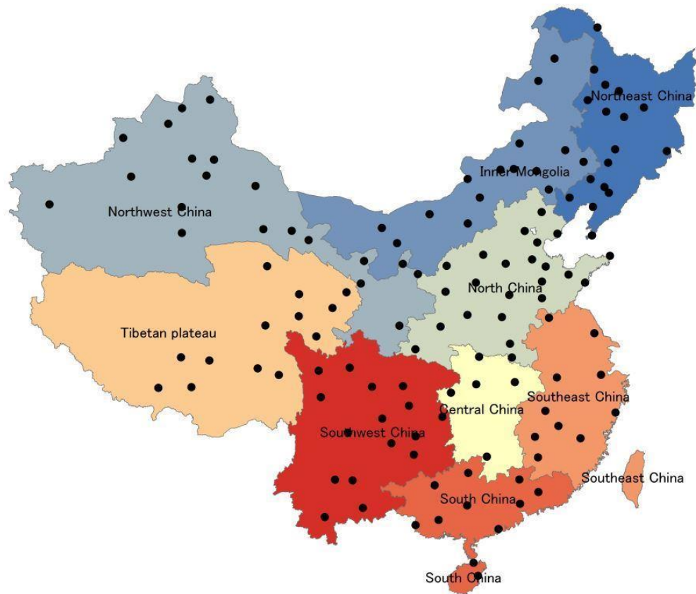
Figure 2- 13 Locations of 130 climate stations in China used to calculate the regional climate characteristics of each 9 sub-regions in China. Mean annual temperature and precipitation of stations within each region were applied to calculate the regional climate characteristics
