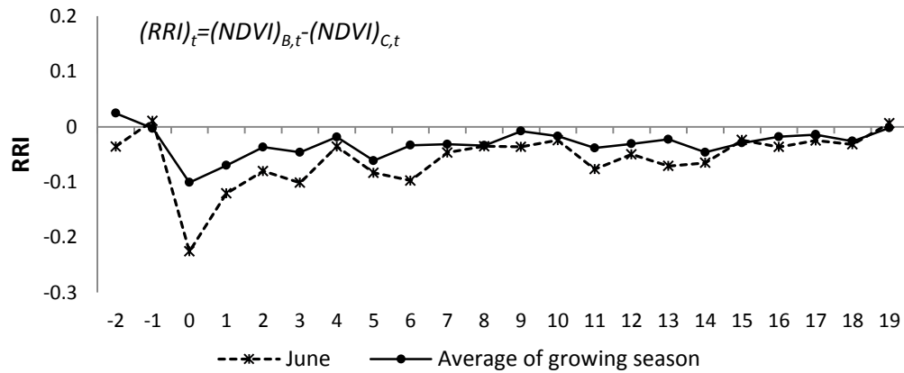
Figure 5-7 The evolution of RRI calculated using NDVI difference between fire scars and the unburned control area for the growing season average (April to October) and June (the month immediately after the fire in 1987) time series. Zero on the time scale represents the burn year, i.e., relative year 0 is the year of the wildfire event. Relative year -1 and +1 corresponds to the year before and after the fire event, respectively
