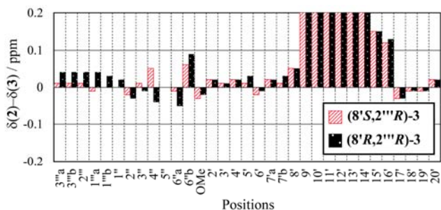
Figure 2. Deviation of ^1\text{H} NMR chemical shifts of 3 from the reported values of 2 . ^1\text{H} NMR spectra of 3 were measured in 25:2 \text{C}_6\text{D}_6/\text{DMSO}-d_6 according to the literature. 1
