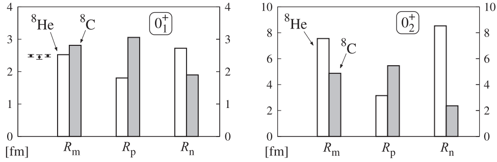
Fig. 2. Real parts of matter, proton, and neutron radii of the ground states (left panel) and the 0_2^+ states (right panel) of ^8\text{He} and ^8\text{C} in units of fm. Circles with error bars indicate experimental data of the matter radius of ^8\text{He} [3,41,42].
