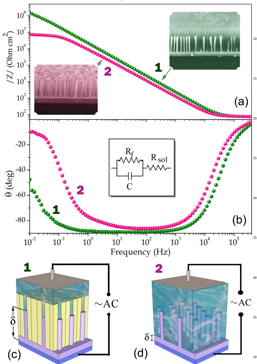
Fig. 9. Bode plots: (a) modulus of impedance |Z| vs. frequency f and (b) phase angle \theta vs. f for the as reanodized sample (curve 1) and the alumina-free sample (curve 2). The schematics show the setup for EIS measurements of the samples in solution.
