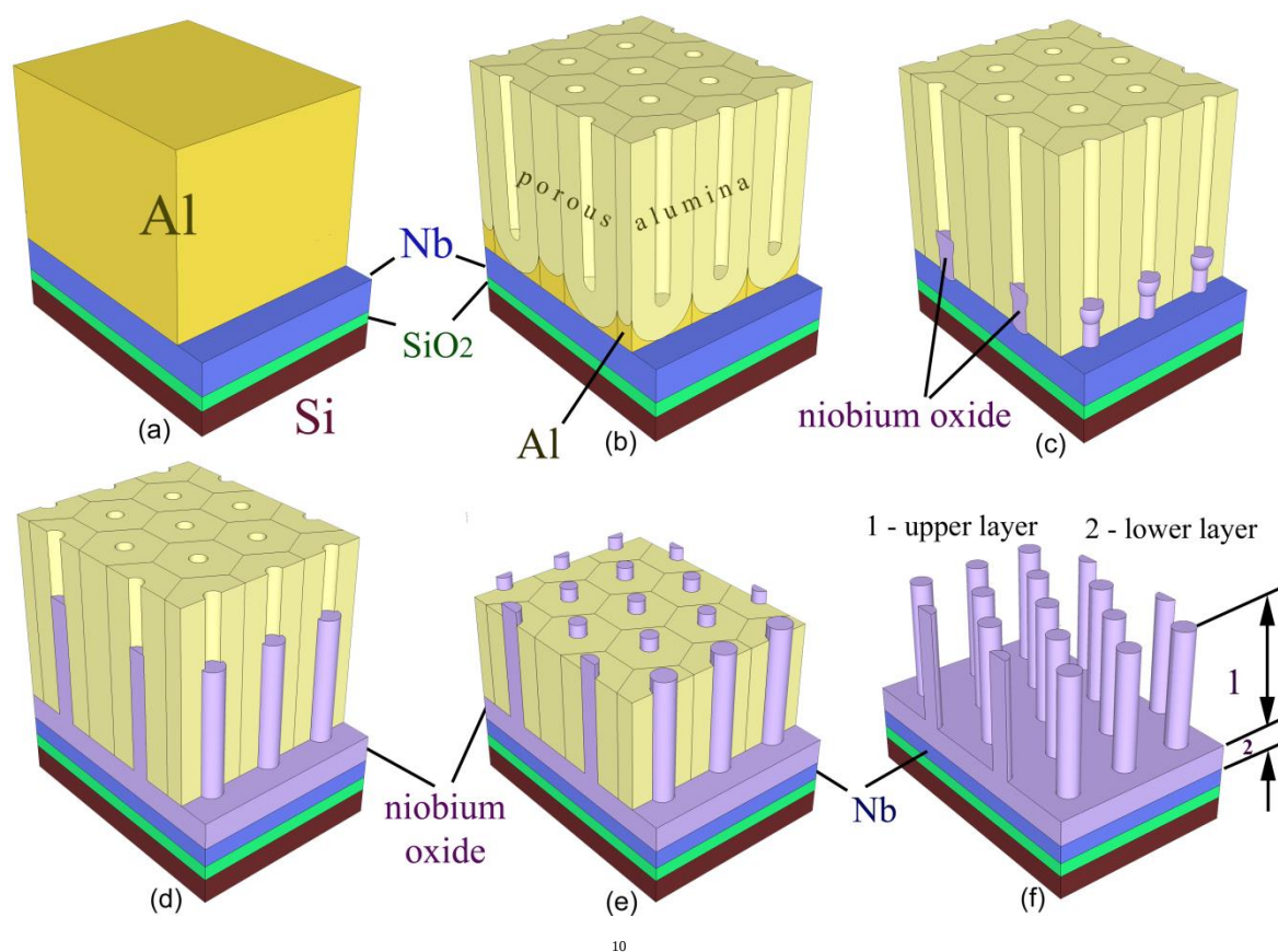
Fig. 3. The main phases of film formation process: (a) sputter-deposition of an Al/Nb bilayer on an SiO 2 /Si substrate, (b) growth of a porous alumina film, (c) anodizing the Nb underlayer through the alumina nanopores, (d) growth of niobium oxide nanocolumns in the alumina pores, (e) partial dissolution of the alumina overlayer ("pore-free" sample), and (f) complete dissolution of the alumina overlayer
