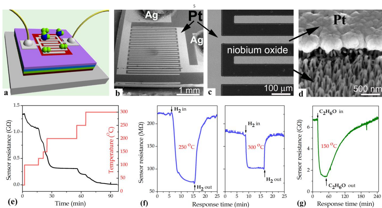
Fig. 10. (a) Schematic and (b-d) SEM images of a laboratory 10 sensor employing the nanostructured niobium oxide film as active layer and the experimental sensor characteristics: (e) resistance- temperature response, (f) resistive response to hydrogen (H 2 ) 1000 ppm, and (g) resistive response to ethanol (C 2 H 5 OH) 5 ppm.
