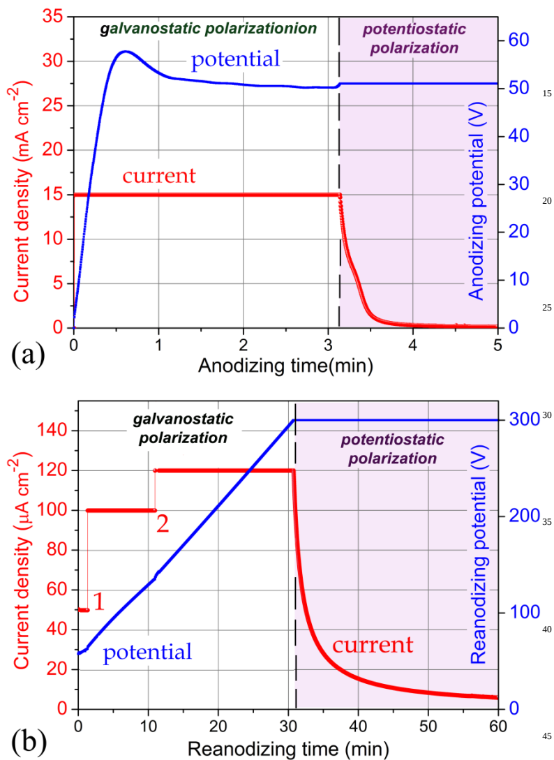
Fig. 1. The potential-time and current-time responses for (a) anodizing in 0.2 mol dm -3 H 2 C 2 O 4 electrolyte and (b) reanodizing in 0.1 mol dm -3 H 3 PO 4 electrolyte of an Al(1μm)/Nb(300nm) bilayer (aluminum-on-niobium) sputter-deposited onto an oxidized Si wafer.
