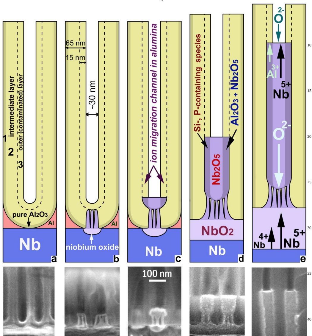
Fig. 8. Schematic model of oxide growth during the anodizing/reanodizing of an Al/Nb bilayer as in Figure 1: (a) porous anodizing of Al, (b) beginning of pore-assisted anodizing of Nb, (c) final stage of Nb anodizing, (d) beginning of Nb reanodizing, and (e) steady-state growth of niobium oxide during the reanodizing.
