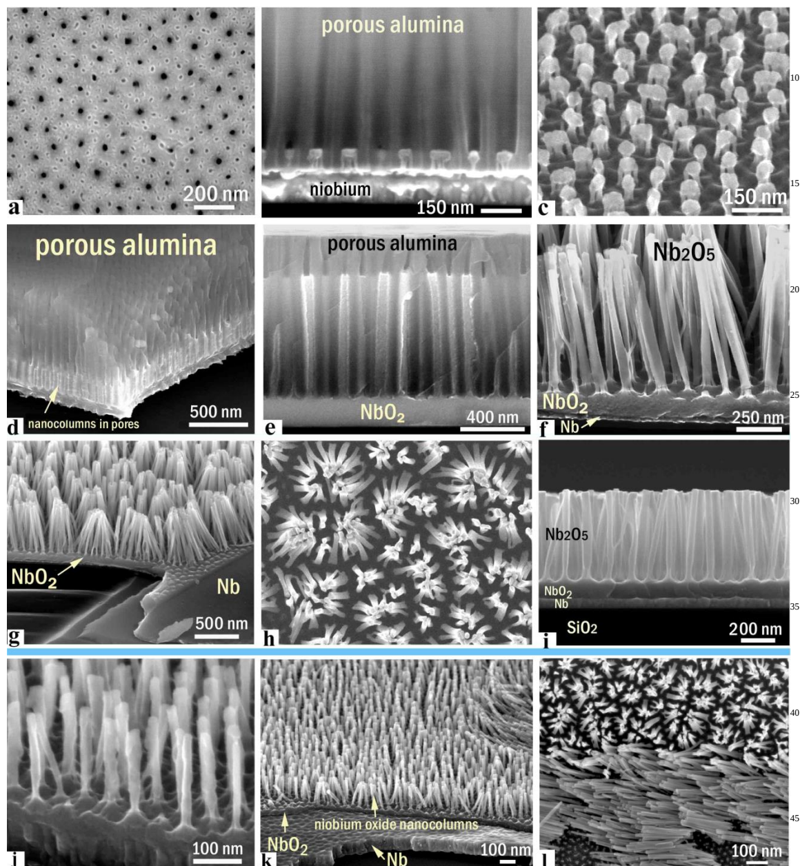
Fig. 2. SEM views of Al/Nb bilayers on SiO 2 /Si substrates: (a-c) anodized at 52 V in 0.2 mol dm -3 H 2 C 2 O 4 and then reanodized in 0.1 mol dm -3 H 3 PO 4 to (d-h) 450 V and (i) 300 V; (j-l) anodized at 26 V in 0.2 mol dm -3 H 2 SO 4 and then reanodized to 150 V in 0.1 mol dm -3 H 3 PO 4 . The images shown in (c, f-l) were obtained after the alumina layer had been dissolved away (“alumina-free” samples).
