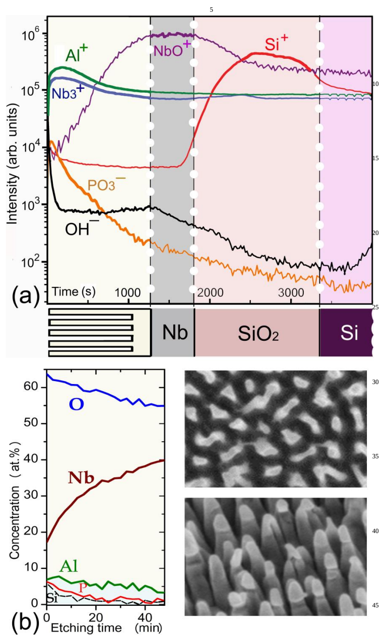
Fig. 4. (a) ToF-SIMS depth profiles and (b) XPS atomic concentration profiles for the alumina-free sample (as in Figure 2i). The SEM images show how the film surface changes after the Ar-ion sputtering.
