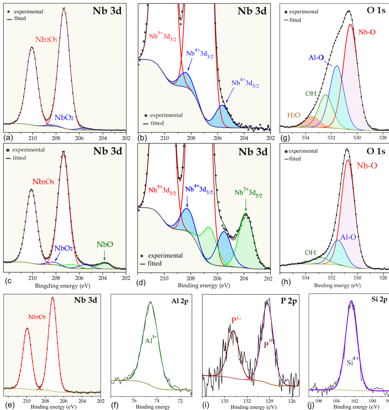
Fig. 5. Experimental and curve-fitted XPS spectra of (a,b) Nb 3d for the unspun alumina-free sample (as in Figure 2i), (c,d) Nb 3d for the unspun vacuum-annealed alumina-free sample, (e) Nb 3d for the unspun pore-free sample (as in Figure 3e), (f) Al 2p for the sputter-cleaned alumina-free sample, (g,h) O 1s for the unspun and Ar-ion sputtered alumina-free sample, respectively, (i) P 2p of the Ar-ion sputtered alumina-free sample, and (j) Si 2p for the sputter-cleaned alumina-free sample
