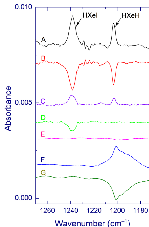
FIG. 3. HXeI and HXeH in an Ar matrix. The FTIR difference spectra show the effects of annealing at 20 K (spectrum A, HI/Xe/Ar = 1/4/1000), irradiation at 193 nm of the annealed matrix (spectrum B, HI/Xe/Ar = 1/4/1000), annealing at 20 K (spectrum C, HI/Xe/Ar = 1/2/1000), irradiation at 488 nm of the annealed matrix (spectrum D, HI/Xe/Ar = 1/2/1000), annealing at 20 K (spectrum E, HI/Ar = 1/1000), annealing at 20 K (spectrum F, HBr/Xe/Ar = 1/4/500), and irradiation at 193 nm of the annealed matrix (spectrum G, HBr/Xe/Ar = 1/4/500). Prior to annealing, the matrices were photolyzed at 193 nm. All spectra were measured at 3 K.
