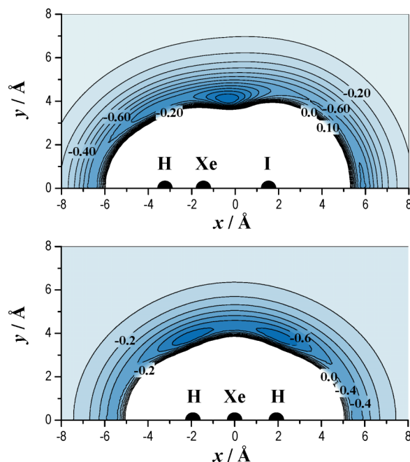
FIG. 8. Two-dimensional contour plots of the potential energy surface (in kcal mol −1 ) for the \text{HXeI} \cdots \text{Xe} and \text{HXeH} \cdots \text{Xe} complexes. The internal coordinates of \text{HXeI} and \text{HXeH} are fixed at the equilibrium values, and the origins are set to the center-of-mass of \text{HXeI} and \text{HXeH} . For \text{HXeI} , the coordinates of the H, Xe, and I atoms are (−3.232, 0.0), (−1.462, 0.0), and (1.539, 0.0), respectively. For \text{HXeH} , the coordinates of the H, Xe, and H atoms are (−1.941, 0.0), (0.0, 0.0), and (1.941, 0.0), respectively.
