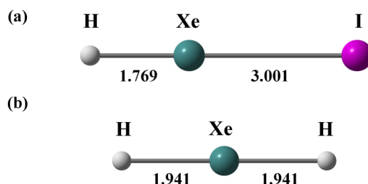
FIG. 6. Equilibrium structures of (a) HXeI and (b) HXeH. The bond lengths are given in Å.
