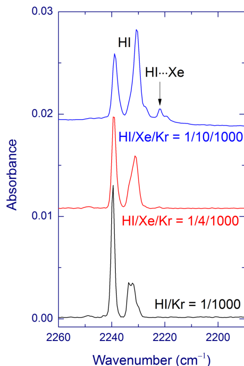
FIG. 4. FTIR spectra of HI/Xe/Kr (1/10/1000, 1/4/1000 and 1/0/1000) matrices. The deposition temperature was 25 K. The spectra were measured at 3 K.
