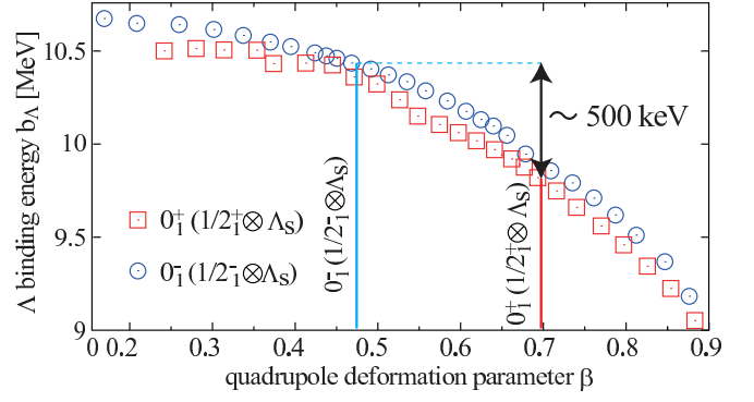
FIG. 3. (Color online) The \Lambda binding energy of the 0_1^- and 0_1^+ states as function of proton quadrupole deformation parameter \beta . Lines in the figure denote the deformation parameter of 0_1^{\pm} states given in Table I.
