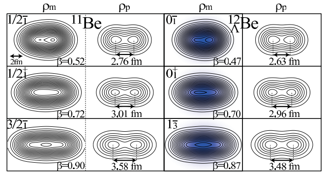
FIG. 2. (Color online) Matter ( \rho_m ) and proton ( \rho_p ) density distributions for the bandhead states of ^{11}\text{Be} and ^{12}_{\Lambda}\text{Be} . Color plots show the density distribution of the \Lambda particle.
