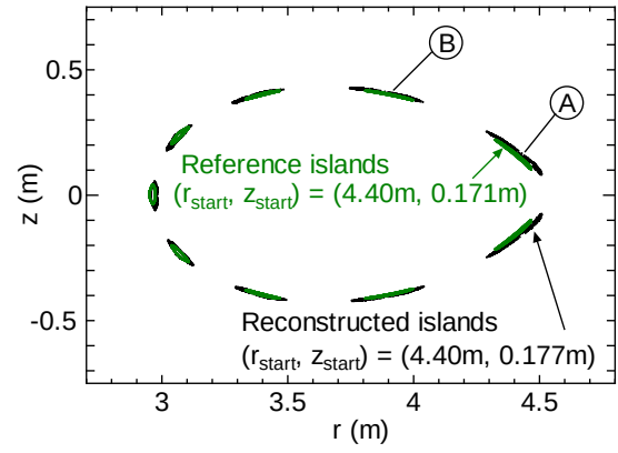
(b) Reconstructed and reference islands
