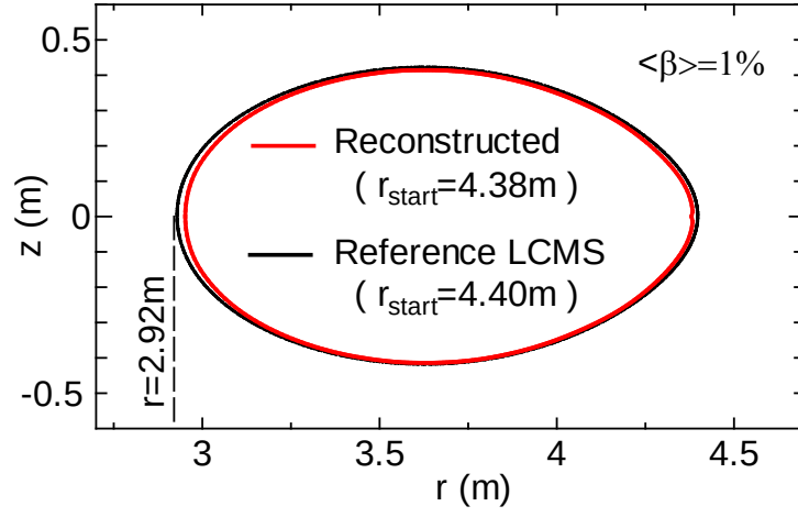
(a) \langle \beta \rangle = 1.0\%
