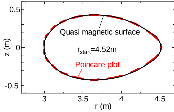
(b) r_{\text{start}} = 4.52\text{m}
