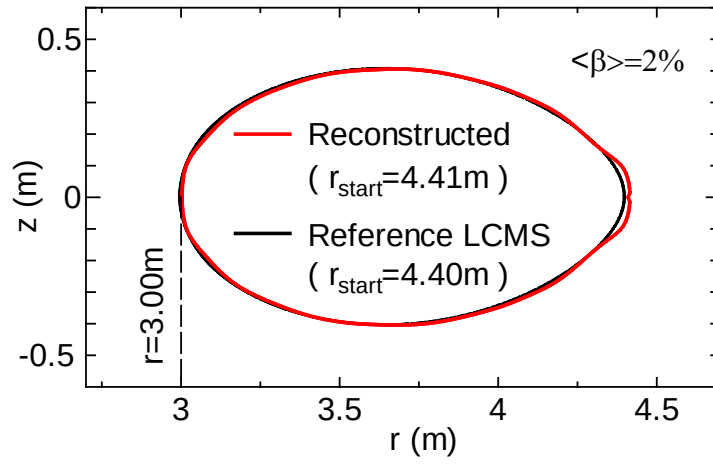
(b) \langle \beta \rangle = 2.0\%
