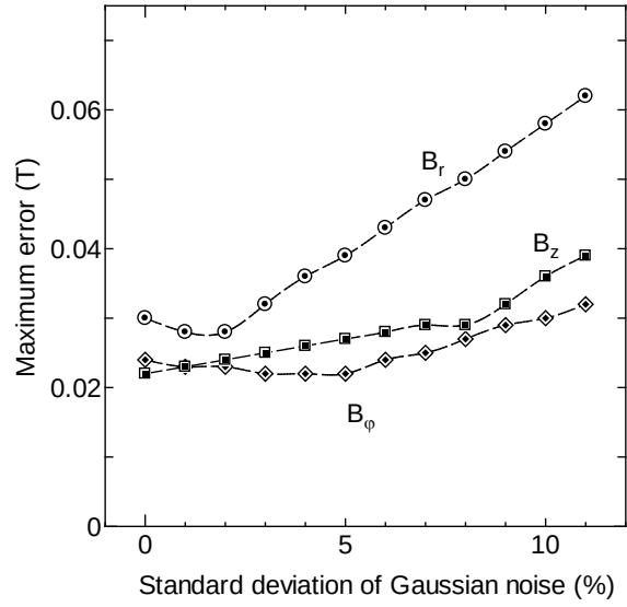
(a) Variation in the maximum errors
