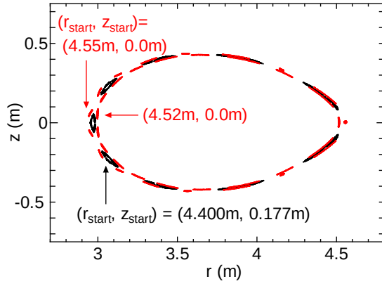
(a) Islands found for the reconstructed field
