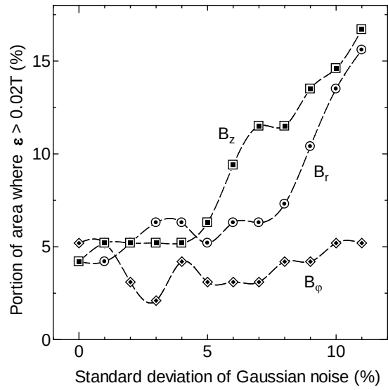
(b) Portion of area where \epsilon > 0.02T (%)
