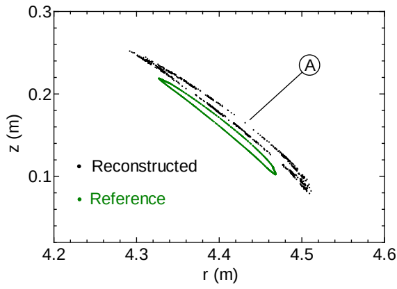
(c) Enlarged island (A)
