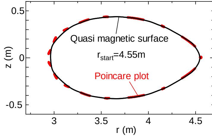
(a) r_{\text{start}} = 4.55\text{m}
