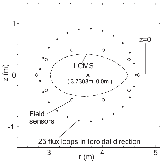
Fig. 7 Sensor locations on the horizontally elongated cross-section: 110 field sensors and 25 flux loops.
