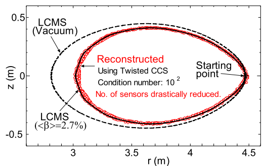
(c) Using the twisted CCS (Cond. No.: 10^2 )
