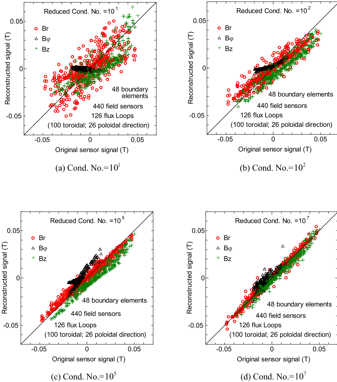
Fig. 3 Reconstructions of field sensor signals. (a) Cond. No. = 10^1 . (b) Cond. No. = 10^2 . (c) Cond. No. = 10^5 . (d) Cond. No. = 10^7 .
