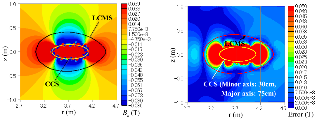
(c) B_z (Left: Reconstructed. Right: Absolute error.)
