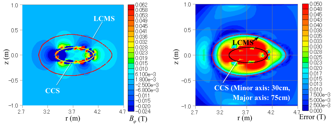
(b) B_\phi (Left: Reconstructed. Right: Absolute error.)
