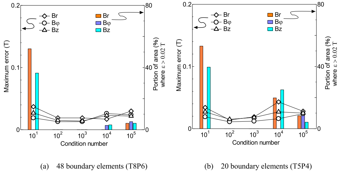
Fig. 6 Error tendency of reconstructed field when assuming 440 field sensors and 126 flux loops. (a) 48 boundary elements (T8P6) (b) 20 boundary elements (T5P4).
