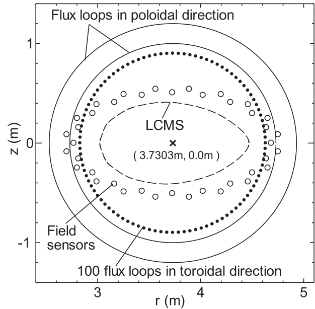
Fig. 2 Sensor locations on the horizontally elongated cross-section: 440 field sensors and 126 flux loops.
