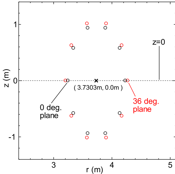
Fig. 16 Field sensor locations on the planes \varphi = 0^\circ and \varphi = 36^\circ .
