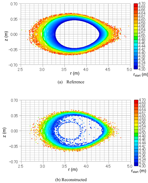
Fig. 11 Comparison of Poincaré plots for the reference and reconstructed field. (a) Reference. (b) Reconstructed.
