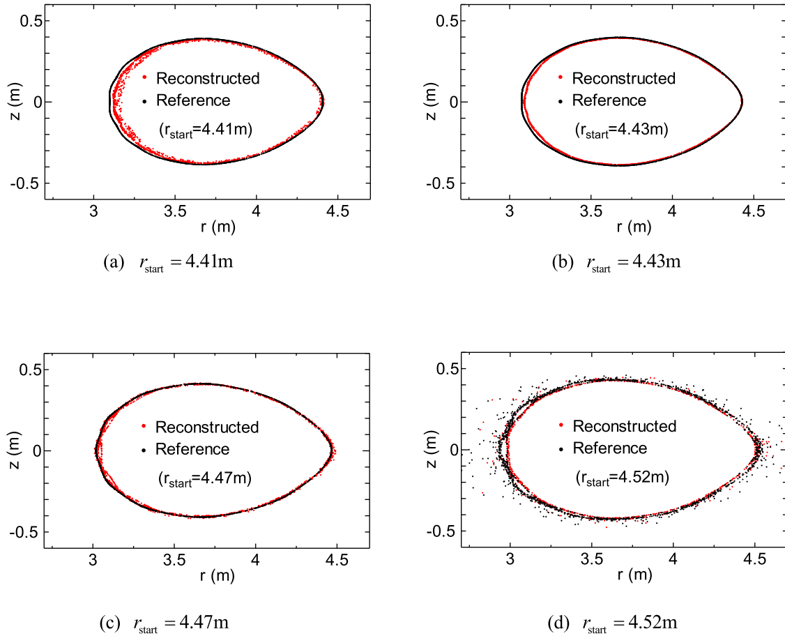
Fig. 12 Poincaré plots for traces originating at various starting points. (a) r_{\text{start}} = 4.41 m. (b) r_{\text{start}} = 4.43 m. (c) r_{\text{start}} = 4.47 m. (d) r_{\text{start}} = 4.52 m.
