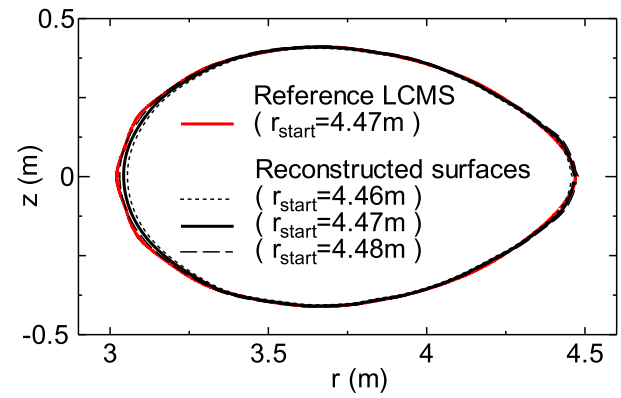
Fig. 15 Reconstructed magnetic surfaces compared with the reference LCMS
