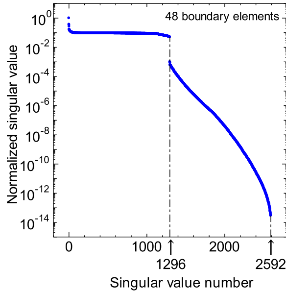
(a) Singular values for the T8P6 case
