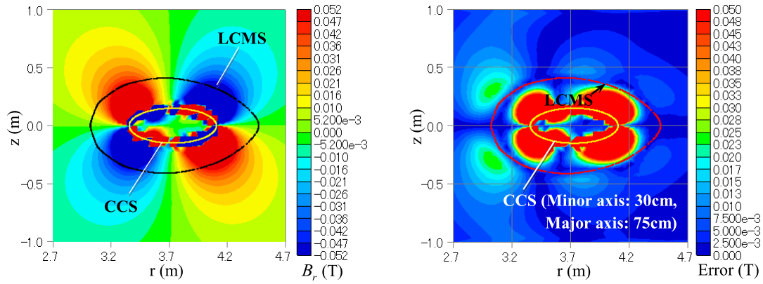
(a) B_r (Left: Reconstructed. Right: Absolute error.)
