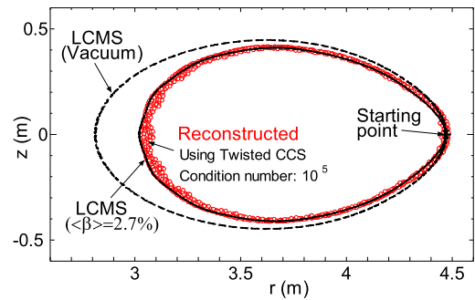
(b) Using the twisted CCS (Cond. No.: 10^5 )
