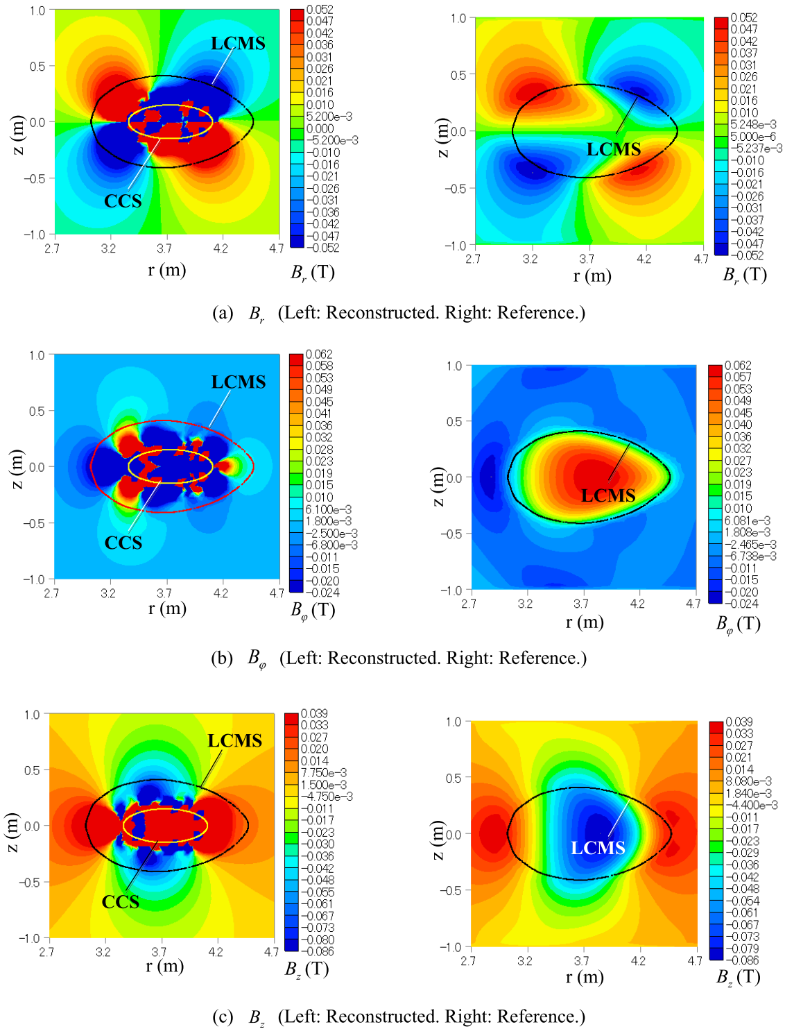
Fig. 4 Reconstructed field caused by plasma current only when assuming 440 field sensors and 126 flux loops with 48 boundary elements (T8P6). The condition number was set to be 10^5 . (a) B_r (Left: Reconstructed. Right: Reference.). (b) B_\phi (Left: Reconstructed. Right: Reference.). (c) B_z (Left: Reconstructed. Right: Reference.).
