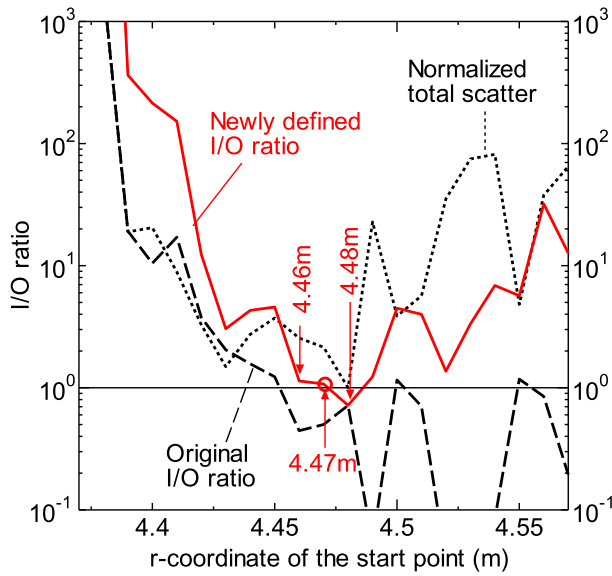
Fig. 14 Variation in the ‘inside/outside’ ratio
