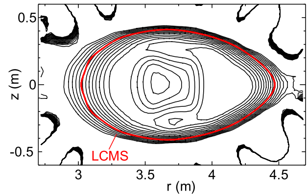
Fig. 13 Contours of quasi magnetic surface.
