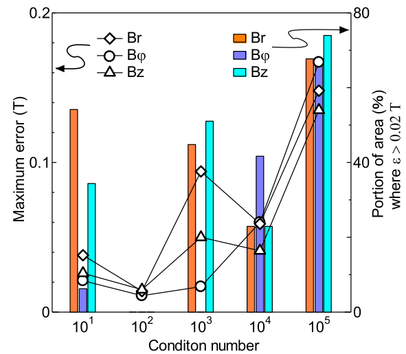
Fig. 8 Error tendency when assuming a smaller number of sensors with 12 boundary elements (T4P3).
