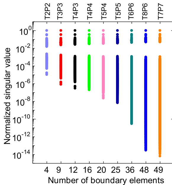
(b) Singular values as a function of the number of boundary elements when using 440 field sensors and 126 flux loops
