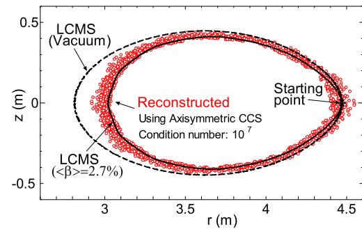
(a) Using the axisymmetric CCS (Cond. No.: 10^7 )
