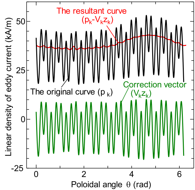
Fig. 6 Subtraction of correction vector from the original current density solution.
