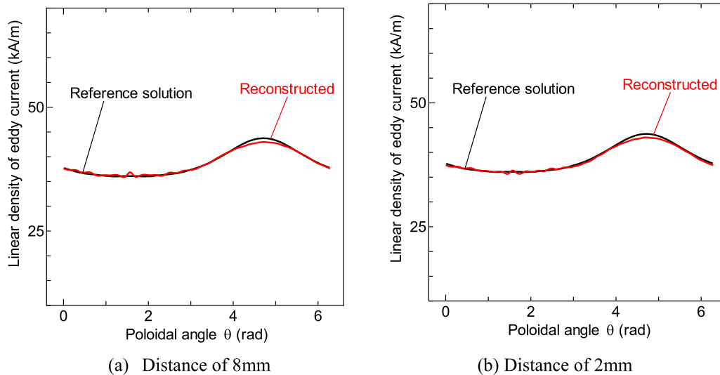
Fig. 10 The eddy current profile reconstructed assuming all sensors to be equidistant from the shell.
