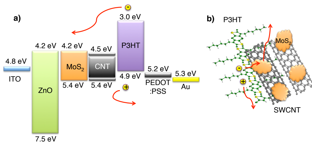
Figure 6. a) Energy band alignment of an P3HT:MoS 2 CNT solar cell where CNT is semiconducting and metallic mixed. Metallic CNT exhibits workfunction of 4.5-5.0 eV b) graphical illustration of P3HT:MoS 2 CNT photoactive layer
