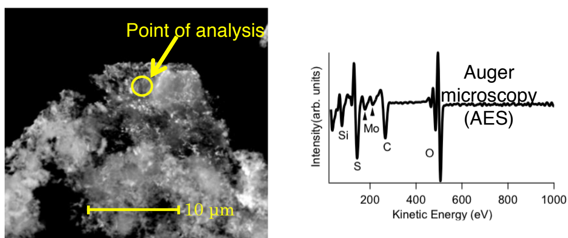
Figure 3. AES of a MoS 2 flake on a CNT bundle
