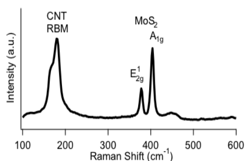
Figure 4. Raman spectrum of multilayered \text{MoS}_2 on CNT bundles
