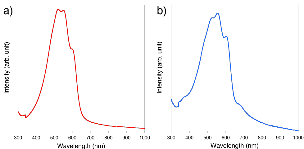
Figure 5. UV-Vis spectra of a) P3HT film and b) P3HT mixed with MoS 2 CNT (3 wt%)
