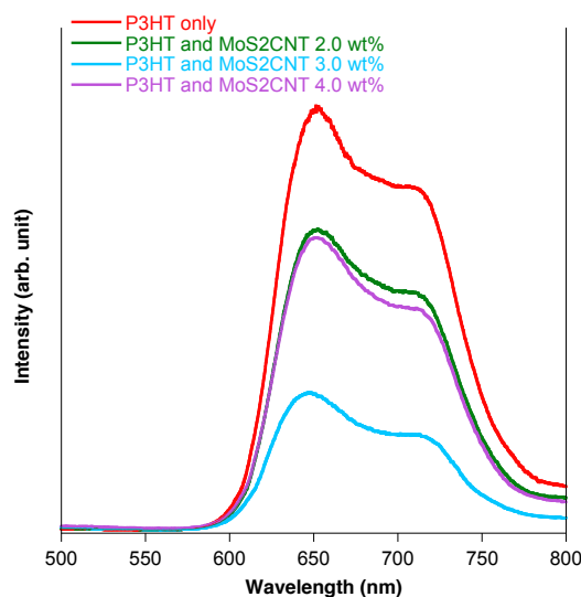
Figure 7. Photoluminescence data of the active layer with increase in \text{MoS}_2\text{CNT} concentration
