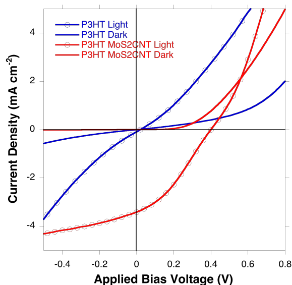
Figure 8. J-V curve of the P3HT only solar cell and P3HT:MoS 2 CNT solar cell
