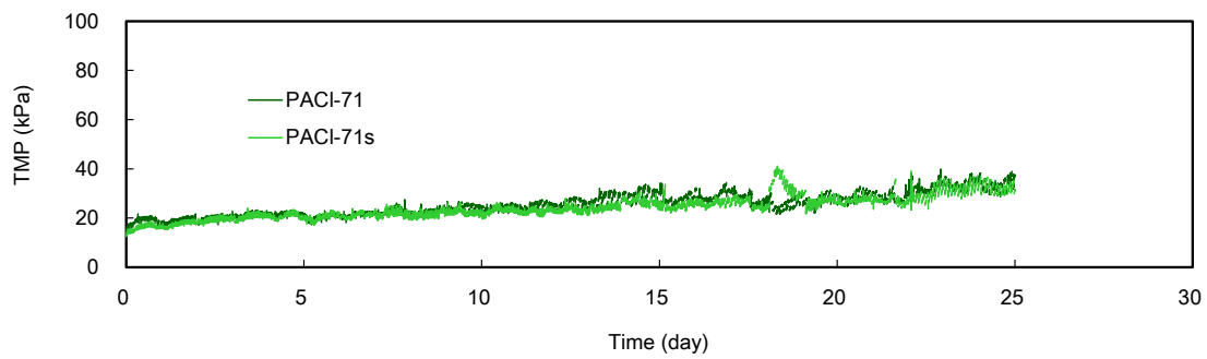
Fig. 7. Comparison of TMP variations during microfiltration after PACl-71 and PACl-71s coagulations. Run 11 (coagulation pH 7.5).
