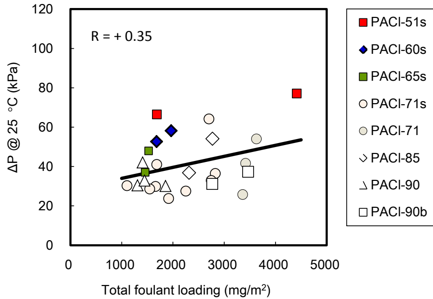
Fig. 9. Relationship between TMP normalized at 25°C and foulant loading (Runs 5–9, 11, 12 and 17–19). The total foulant loading was calculated with the assumption that Al and Si mainly exist in the forms of \text{Al}_2\text{Si}_2\text{O}_5(\text{OH})_4 according to the section 3.1, the excess Al in the form of \text{Al}(\text{OH})_3 if \text{Al}/\text{Si} > 1 , the excess Si in the form of \text{SiO}_2 if \text{Si}/\text{Al} > 1 , Ca in the form of \text{Ca}(\text{OH})_2 , Mg in the form of \text{Mg}(\text{OH})_2 , Fe in the form of \text{Fe}(\text{OH})_3 , and Mn in the form of \text{MnO}(\text{OH})_2 ; the carbon content of organic matter was 51%.
