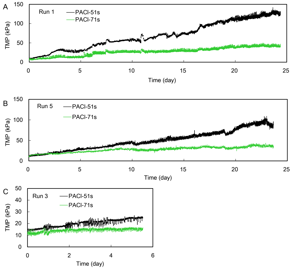
Fig. 2. Comparison of TMP variations during microfiltration after PACI-51s and PACI-71s coagulations: (A) Run 1 (coagulation pH 6.1–7.3); (B) Run 5 (coagulation pH 7.0); (C) Run 3 (coagulation pH 7.5).
