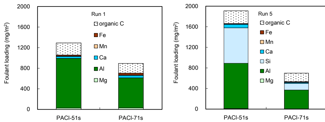
Fig. 3. Elemental compositions of membrane foulants recovered in chemical cleaning agents (Si was not analyzed for Run 1).
