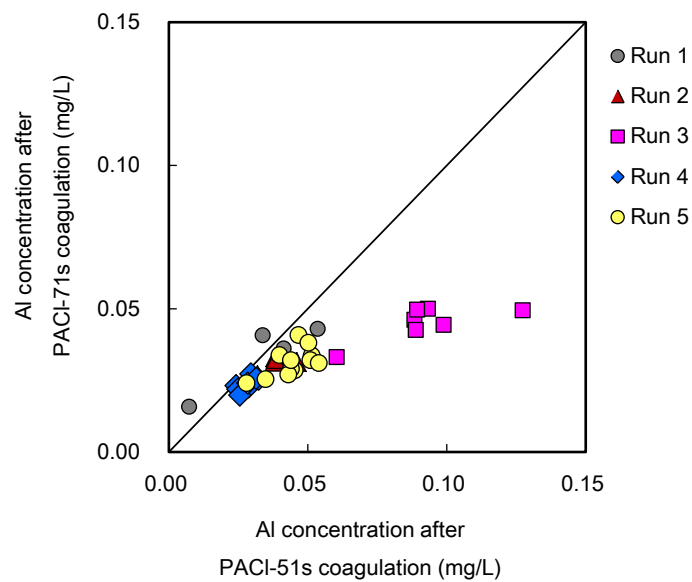
Fig. 4. Aluminum concentrations in the MF filtrates after PACI-71s and PACI-51s coagulations.
