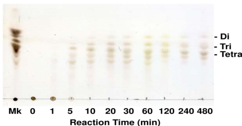
Figure 6. Analysis for the degradation products of alginate produced by FlAlyA. Alginate was degraded by FlAlyA and the degradation products were analyzed by TLC. Di, Tri, and Tetra indicate disaccharide, trisaccharide, and tetrasaccharide, respectively. Mk, degradation products of alginate produced by abalone crude enzyme [24,25]. The sizes of marker oligosaccharides were previously determined by BioGel P2 gel-filtration [24].
