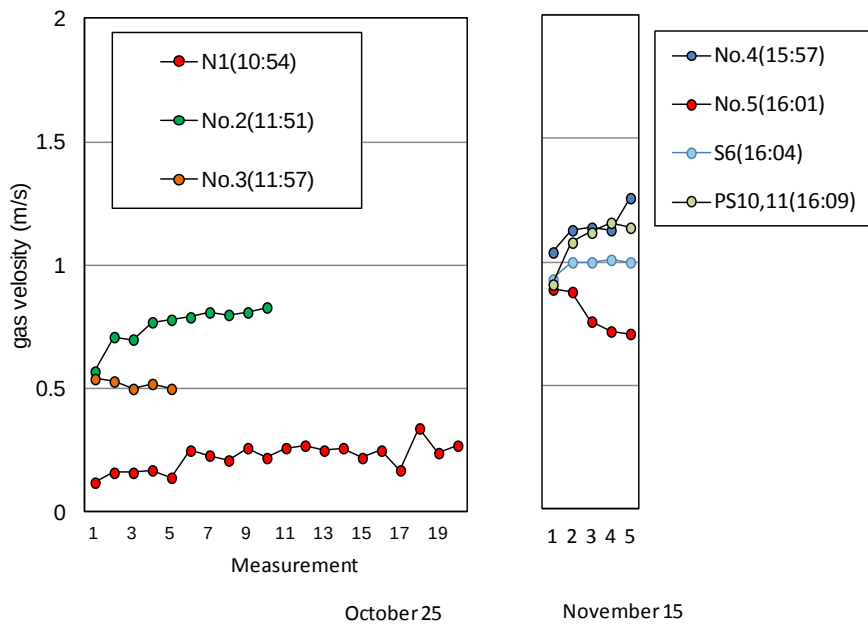
Figure 12 Consecutive measurement of gas velocity at outflow vents
