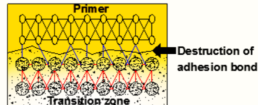
Fig. 16 Visualization of bond failure mechanism before and after exposure in (a) Normal strength concrete; and (b) High strength concrete
