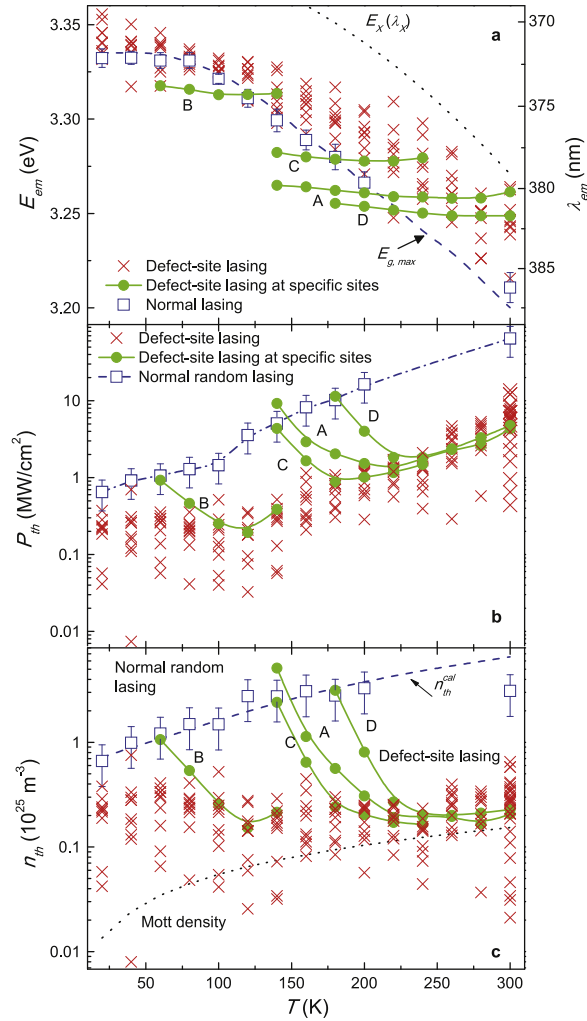
Figure 3. (a) Lasing energy (wavelength, right axis) E_{em} ( \lambda_{em} ) of defect-site lasing at various defect sites (crosses) and normal random lasing (open squares) as a function of temperature T . The dashed curve represents the plots of peak energies E_{g,max} in the gain spectra g . The solid circles show E_{em} ( \lambda_{em} ) for defect-site lasing at specific defect sites (A–D). The dotted curve represents the exciton recombination energy (wavelength) E_X ( \lambda_X ). (b) Threshold power density P_{th} of defect-site lasing at various defect sites (crosses) and those at specific defect sites A–D (solid curves) as a function of temperature T . (c) Threshold carrier density n_{th} of defect-site lasing at various defect sites (crosses) and normal random lasing (open squares) as a function of T . The dashed curve represents the calculated threshold carrier density n_{th}^{cal} . The dotted curve shows the calculated Mott density. The solid circles show n_{th} for defect-site lasing at specific defect sites (A–D).
