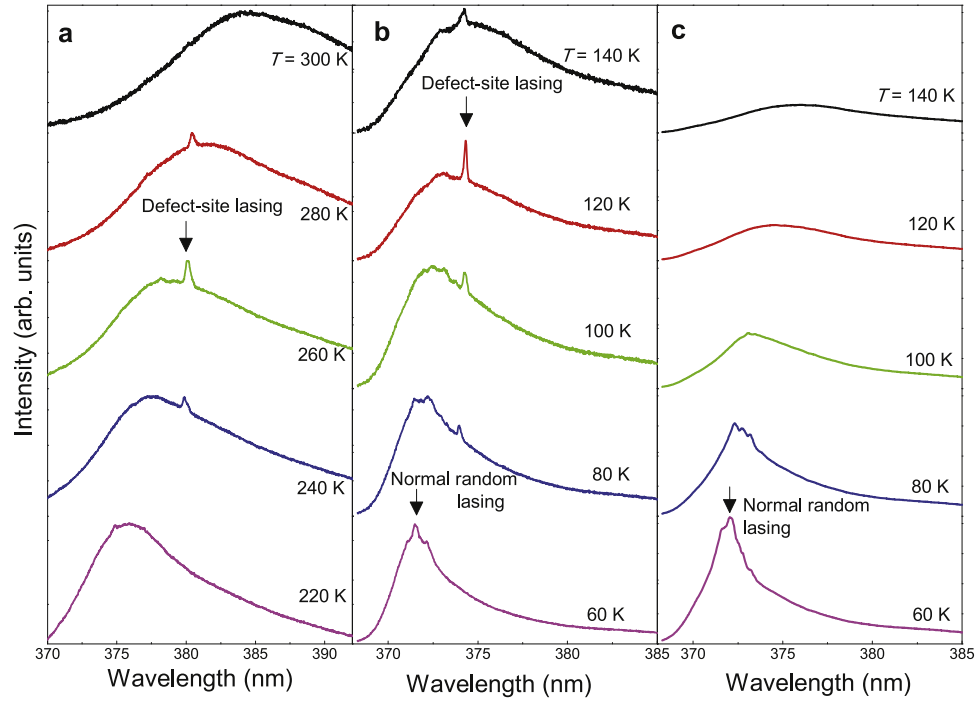
Figure 2. Lasing emission spectra of spherical ZnO powder at specific defect sites: (a) A at T = 220 – 300 K and (b) B at T = 60 – 140 K. (c) Random lasing spectra of randomly shaped ZnO powder at T = 60 – 140 K. The excitation power densities are (a) 5, (b) 0.9, (c) 2 \text{ MW cm}^{-2} .
