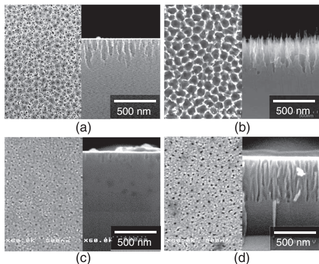
Figure 2. Top and cross-sectional SEM images of GaN-porous samples formed in FSI mode with V_a = 1 V, P_{IN} = 5 mW/cm 2 and different t_a : (a) t_a = 600 s and (b) t_a = 1800 s, and samples formed in BSI mode with V_a = 5 V, P_{IN} = 65 mW/cm 2 and different t_a : (c) t_a = 600 s and (d) t_a = 1800 s.
