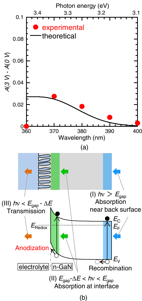
Figure 4. (a) Photo-absorbance measured as function of wavelength of incident light and (b) formation model of GaN-porous structure using photo-assisted electrochemical process.
