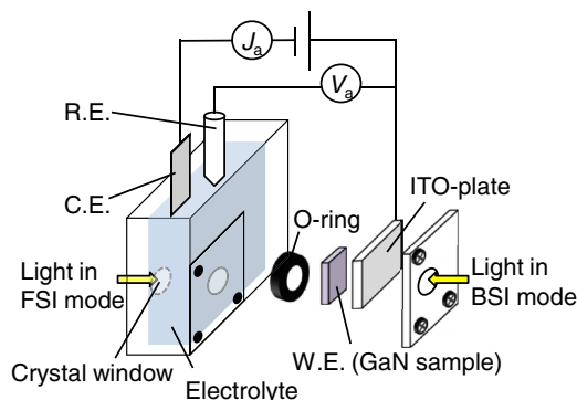
Figure 1. Schematic illustration of electrochemical setup used for both formation of porous structures and spectroscopic measurements.
