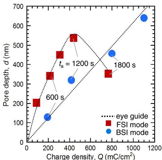
Figure 3. Relationship between pore depth d_p and charge density Q passing through during photo-assisted electrochemical process.
