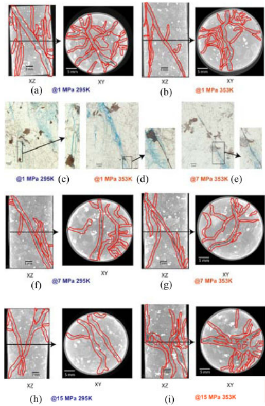
Figure 12. CT and thin section images of post compression specimens of Inada granite.
