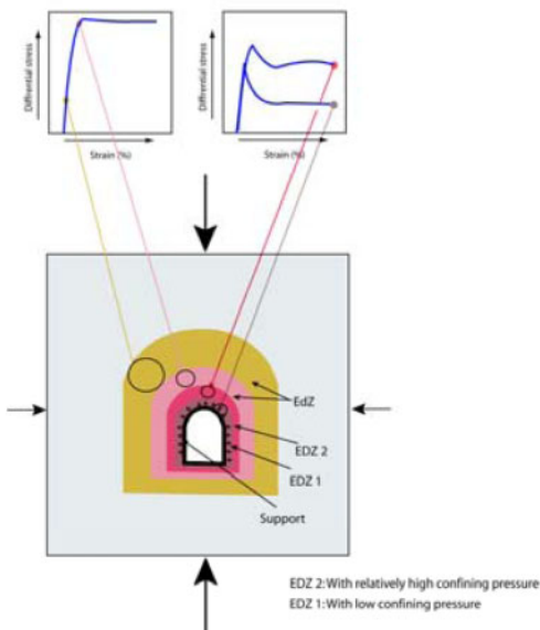
Figure 1. EdZ and EDZ around an underground excavation.
