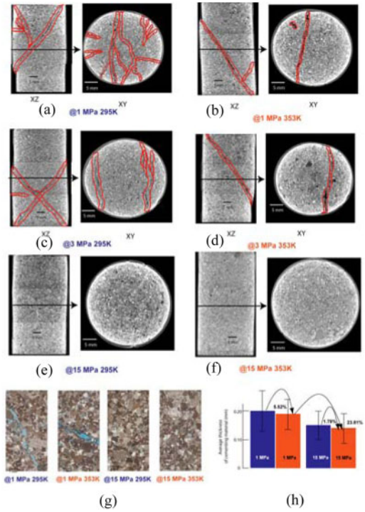
Figure 9. CT and thin section images and thickness of cementing materials of post compression specimens of Kimachi sandstone.
