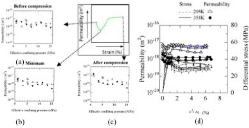
Figure 7. Permeability of Kimachi sandstone.
