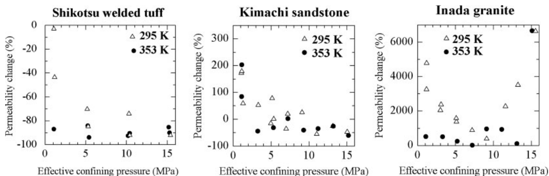
Figure 14. Permeability change due to failure.
