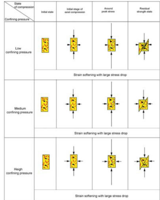
Figure 13. Confining pressure effect on structural changes of Inada granite.
