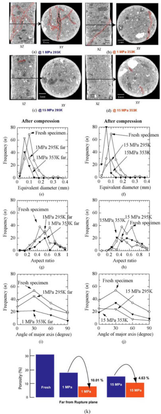
Figure 5. CT images and thin section image analyses of post compression specimens of Shikotsu welded tuff.
