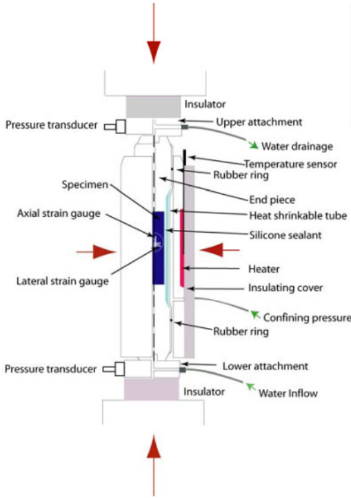
Figure 2. Ultra compact triaxial cell with heater. Showing water inflow and water drainage during constant flow method.
