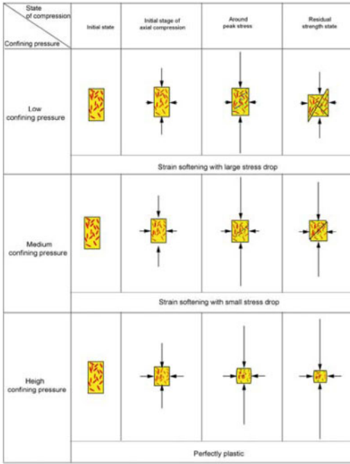
Figure 10. Confining pressure effect on structural changes of Kimachi sandstone.
