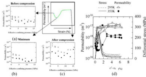
Figure 11. Permeability of Inada granite.
