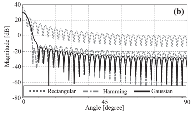
(b) patterns for m = 0 .
