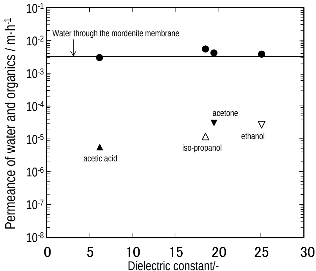
Figure 4 Permeance of water (circles) and organic molecules (triangles) through a mordenite nanocrystal-layered membrane. The solid line is water permeance from water (without organics) through the mordenite nanocrystal-layered membrane.
