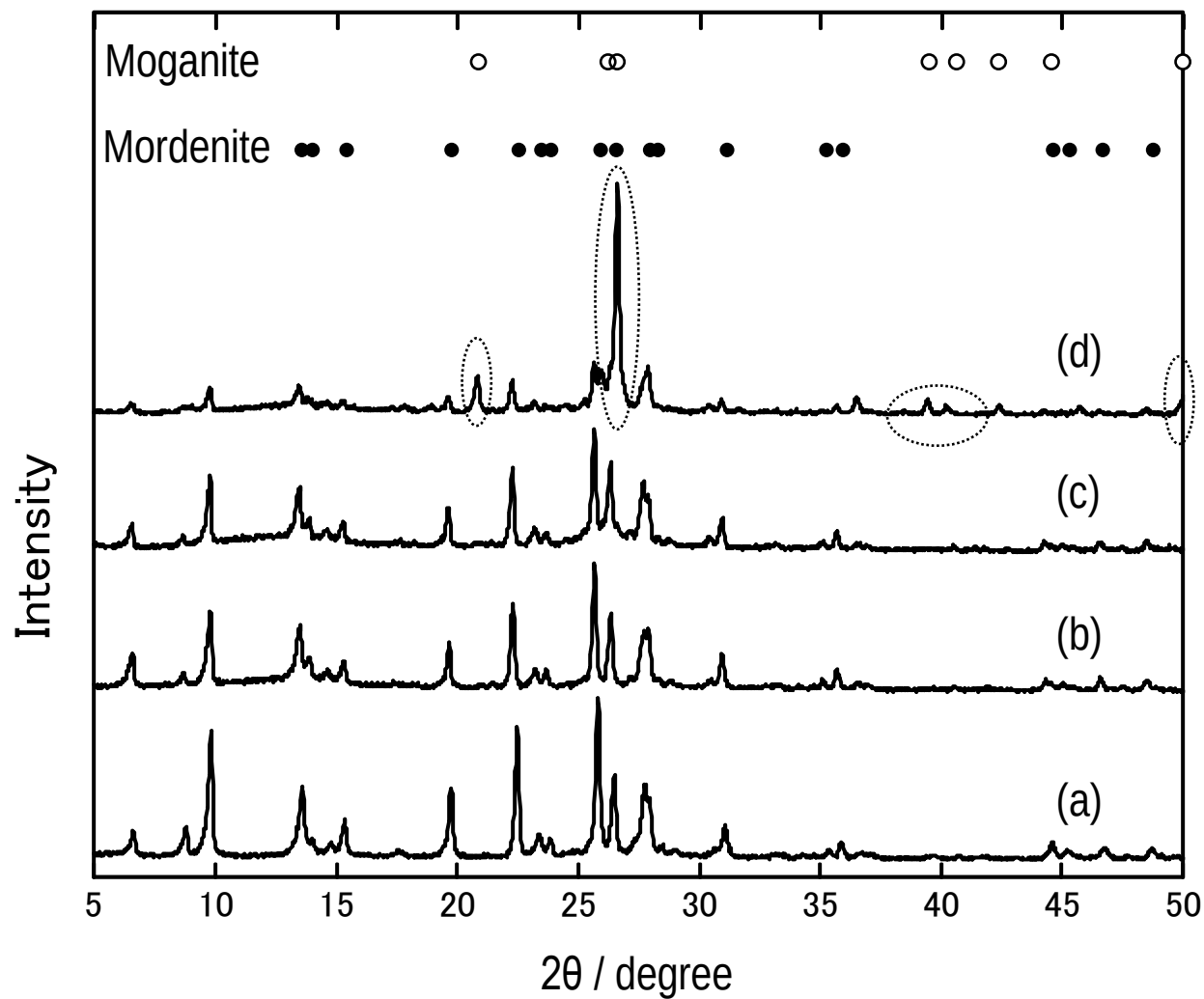
Figure 3 XRD patterns of (a) commercial mordenite, and powders obtained in solution after protection layer formation at (b) 150°C (c) 180°C and (d) 200°C
