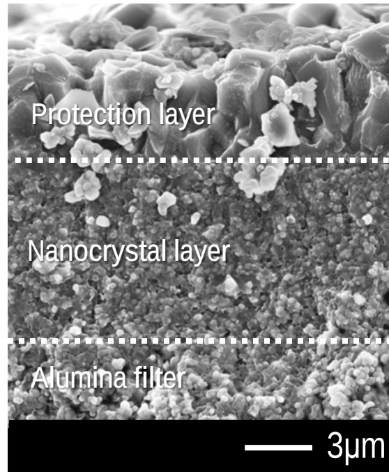
Figure 2 FE-SEM photographs of mordenite nanocrystal-layered membrane (cross-sectional area), (prepared at a hydrothermal temperature of 180 °C in Table 2).
