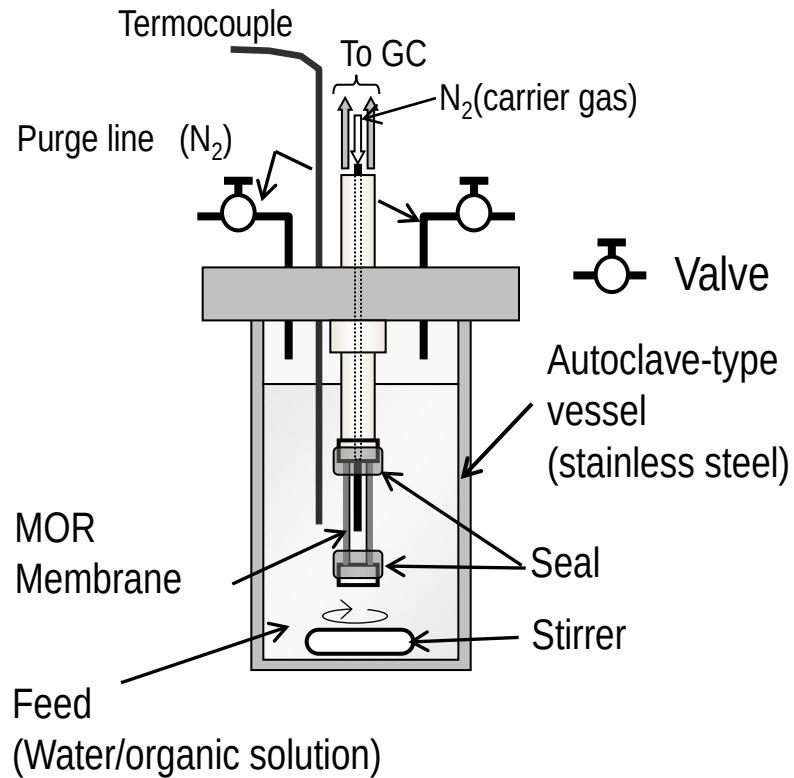
Figure 1 Schematic of the stainless steel autoclave vessel used for pervaporation experiments.
