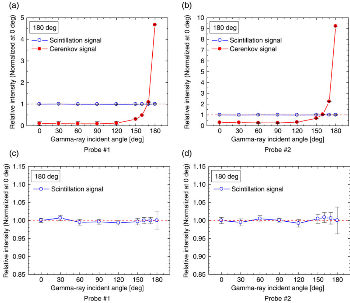
Fig. 7. Separated signals of scintillation and Cerenkov radiation as a function of incident angle for two probes for which calibrations are performed using 0^\circ and 180^\circ source position values. Scintillation and Cerenkov signals ( a , b ) and Scintillation signals fluctuated around a relative intensity of 1.00 ( c , d ).
