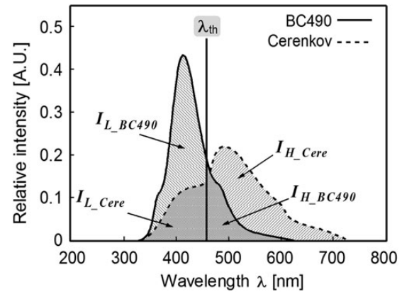
Fig. 3. Measured spectra of BC490 plastic scintillator and Cerenkov radiation. I_{L\_BC490} , I_{L\_Cere} , I_{H\_BC490} , I_{H\_Cere} represent sum of intensities of BC490, which were lower than the threshold, sum of intensities of Cerenkov radiation, which were lower than the threshold, sum of intensities of BC490, which were higher than the threshold, and sum of intensities of Cerenkov radiation, which were higher than threshold, respectively.
