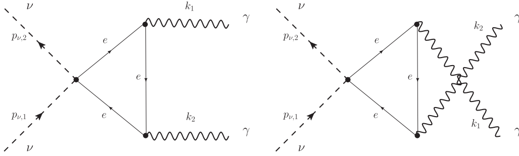
Fig. 1. Triangle diagrams of the electron loop that give contributions to 1^+(l\bar{l}) \rightarrow \gamma\gamma , \nu + \gamma \rightarrow \nu + \gamma , and \nu + \bar{\nu} \rightarrow \gamma + \gamma .
