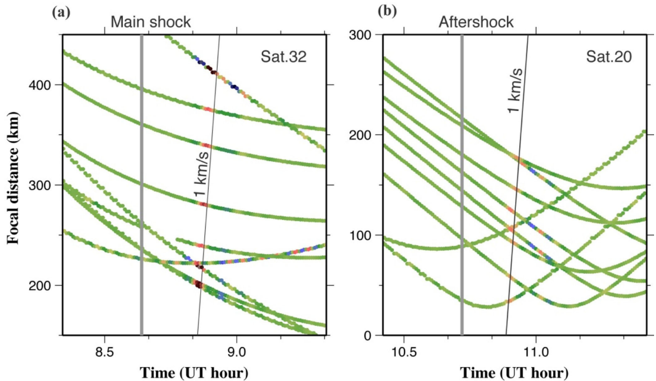
Figure 4. (a) Traveltime diagram of the CID after the 2012 North Sumatra earthquake (main shock) based on the Satellite 32 data. The CID peak (shown in red colours) detected by wavelet propagates with the apparent velocity of \sim 1 \text{ km s}^{-1} (thin black line). Distances are measured from the centre of the uplift (Fig. 3a). The grey vertical line indicates the occurrence of the main shock (08:38 UT). (b) Traveltime diagrams of the largest aftershock CID based on the Satellites 20 data. Distances are measured from the centre of uplift (Fig. 3b). The grey vertical line indicates the occurrence of the aftershock (10:43 UT). Apparent speed is also \sim 1 \text{ km s}^{-1} . In both cases, only stations with SIP to the north of the epicentre (i.e. with latitudes higher than the uplift centres) are plotted considering the directivity (Fig. 6).
