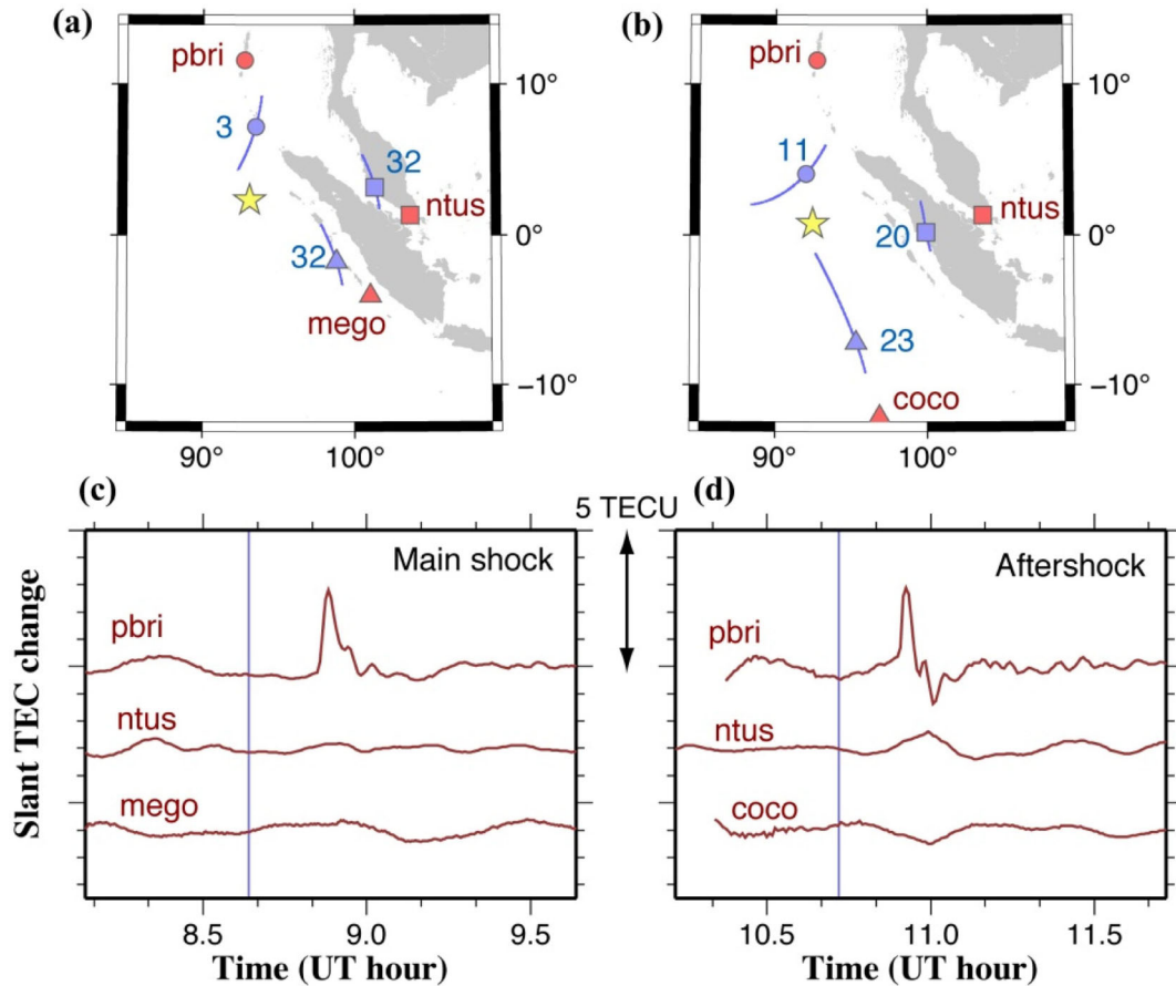
Figure 6. Comparison of the CID of the main shock (a) and the largest aftershock (b) of the 2012 North Sumatra earthquake propagating toward three directions. Their TEC time-series are shown in (c) and (d) for SIPs located to the north (top), east (middle) and south (bottom). We selected satellite-site pairs with geometries of the epicentre (yellow), SIP (blue), GPS station (red) favourable for CID detections (see Fig. 7). Strong CIDs are seen only to the north of the epicentre. Numbers attached to the SIPs in (a, b) are satellite numbers (i.e. TEC data in (c) and (d) are for different pairs of stations and satellites).
