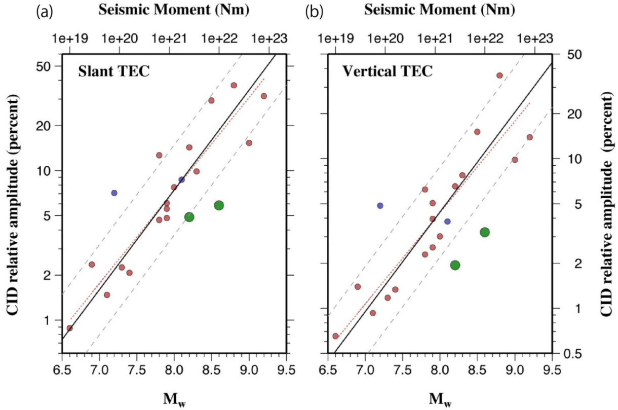
Figure 10. Comparison of moment magnitudes of the 21 earthquakes shown in Figs 8, 9, and the Wenchuan earthquake from Astafyeva et al. (2013), with their relative CID amplitudes in slant (a) and vertical (b) TEC. CID amplitudes in both (a) and (b) are normalized by the background vertical TEC. Colours of the symbols show the faulting mechanisms, that is red (reverse), blue (normal) and strike-slip (green). The black line indicates the best-fitting line with the fixed slope of 2/3, that is the difference in 3 of M_w corresponds to the two orders of difference in CID amplitudes. Dashed lines indicate uncertainties of factor two differences coming from non-ideal LOS geometry. The red dotted line indicates the best-fitting line with both slope and offset inferred by linear regression for the 17 data of reverse earthquakes. CID amplitudes of strike-slip earthquakes (green) show somewhat smaller values than other earthquakes.
