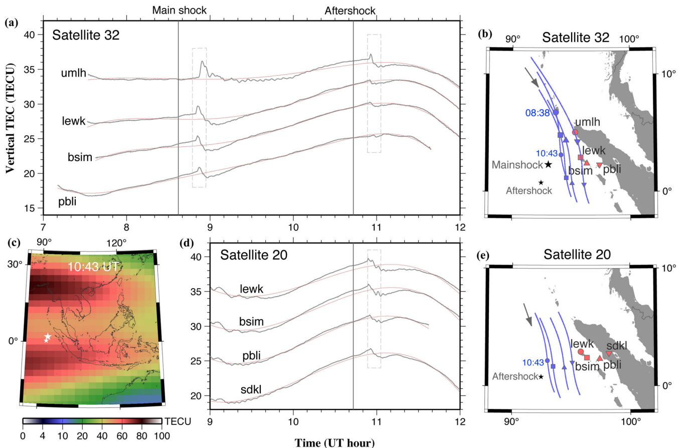
Figure 2. Vertical TEC anomalies recorded at four GPS stations with Satellites 32 (a), and 20 (d). Vertical grey lines are occurrence times of the main shock (08:38 UT) and the largest aftershock (10:43 UT) of the 2012 North Sumatra earthquake. We gave vertical separations 6 TECU between adjacent curves to avoid overlap of the curves. CIDs are seen within the dashed rectangles (10–20 min after earthquakes). Reference curves (thin red) are derived by modelling vertical TEC changes with cubic polynomials of time. Trajectories of SIPs are shown in (b) and (e). Small and large blue circles on the trajectories are SIPs at 08:38 and 10:43 UT, respectively. (c) shows vertical TEC background at 10:43 UT calculated using the Global Ionospheric Map (GIM).
