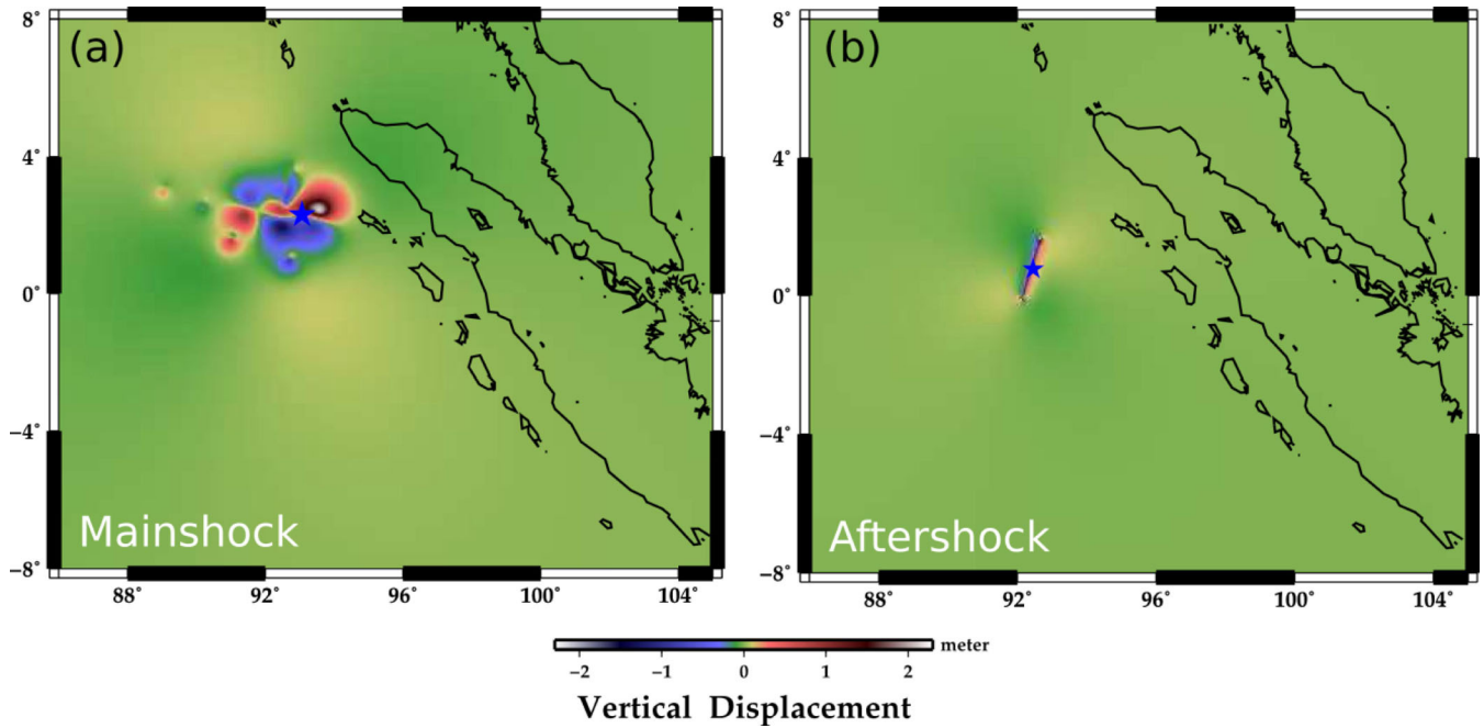
Figure 3. Vertical crustal movements of the main shock (a) and the largest aftershock (b) of the 2012 North Sumatra earthquake. Blue stars show the epicentres of the two earthquakes. They were calculated after Okada (1992), using the fault geometry taken from fig. 4 of Yue et al. (2012). Average slips of the four fault segments were inferred from the seismic moments released from the fault segments given there. Although the earthquakes were dominated by the strike-slip mechanism, significant vertical movements occurred. Focal distances in the vertical axes of Fig. 4 are measured from the centres of uplift in this figure.
