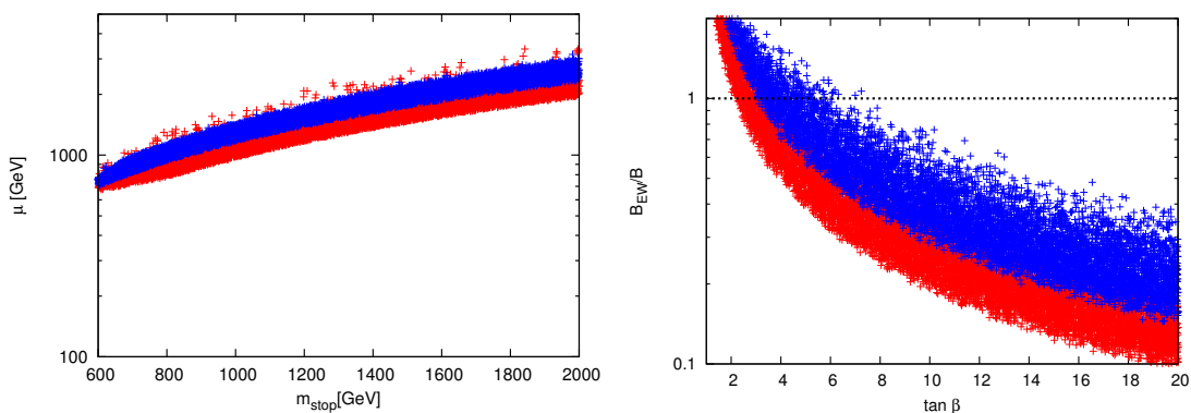
Figure 5. m_{\text{stop}} vs. \mu and \tan \beta vs. B-term in the case with (T_{\text{GUT}}, T_X) = (2 \times 10^{16} \text{ GeV}, 10^7 \text{ GeV}) and 0 \leq N_{\text{eff}} \leq (blue), 6 \leq N_{\text{eff}} \leq 8 (red). In the right figure, m_{\text{stop}} is lighter than 2 TeV. The dashed line is consistent with the condition for the EW symmetry breaking.
