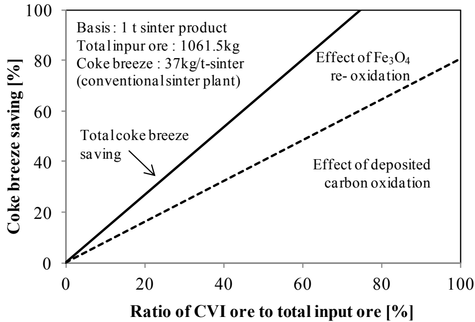
Fig. 5-9 Effect of CVI ore utilization on the consumption of coke breeze in sinter plant showed that the proposed system offered an extensive amount of coke breeze savings.
