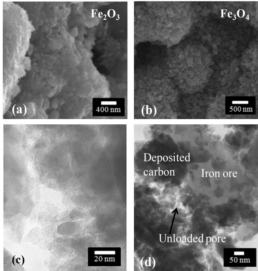
Fig. 4-3 SEM images showing change during tar decomposition: (a) untreated iron ore consisting mainly of \text{Fe}_2\text{O}_3 , (b) iron ore after tar decomposition, containing \text{Fe}_3\text{O}_4 due to the indirect reduction ( \text{CO} and \text{H}_2 ). TEM images of the iron ore after tar decomposition: (c) crack formation in the ore surface disappeared due to carbon deposition, (d) blockage of pore by deposited carbon, which caused a decrease in total carbon deposition.
