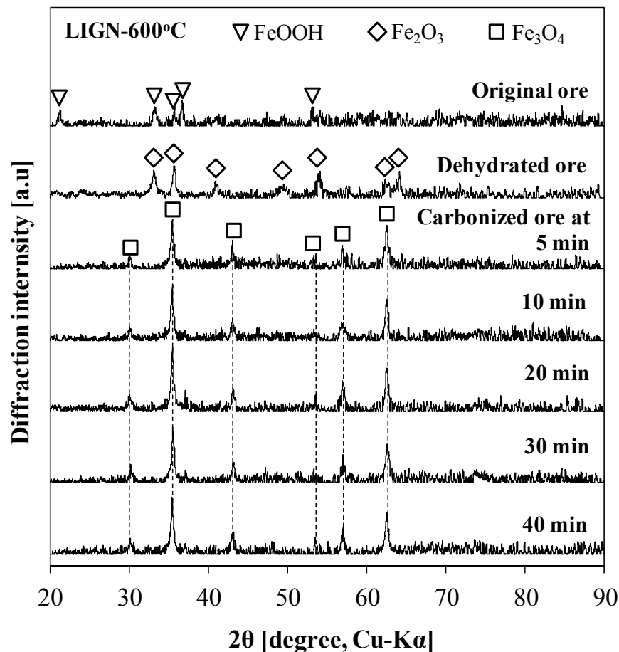
Fig. 3-6 Changing of XRD pattern at each experiment steps show that dehydration process removed OH completely while indirect reduction occurred simultaneously with decomposition process to product Fe 3 O 4 . Thermodynamic limitation caused the ore reduction reaction never proceed to FeO/Fe at longer time yet.
