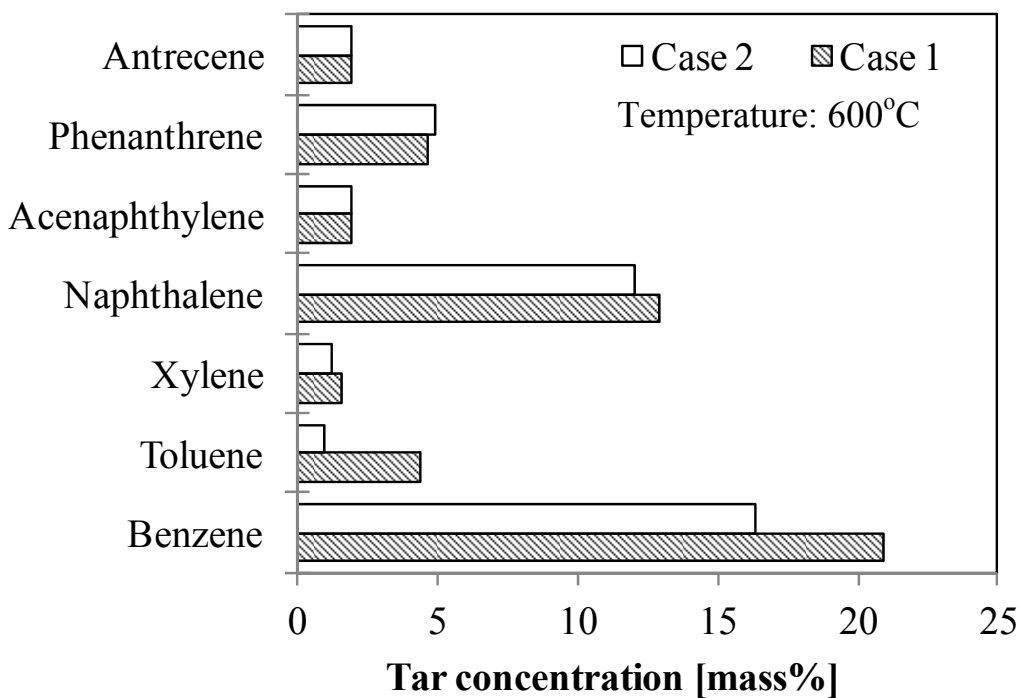
Fig. 2-5 Change of LIGN tar composition due to decomposition process over porous low grade ore. Case 1: no iron ore; case 2: 3 g of iron ore
