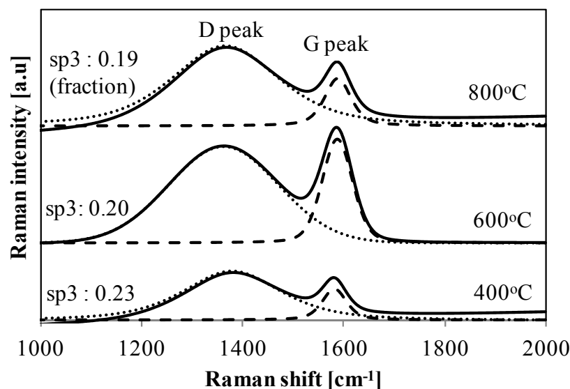
Fig. 4-7 Curve fitting of the Raman spectra and sp3 fraction of carbon deposited by tar decomposition of lignite coal at different temperatures.
