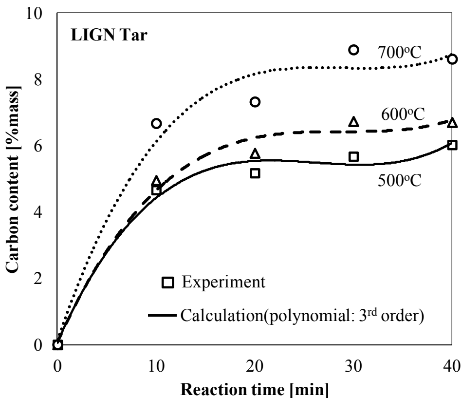
Fig. 3-5 Effect of temperature on carbon content within porous ore at different reaction time shows that high temperature attained larger carbon deposition due to large tar decomposition. Thermal hydrocarbon decomposition preferred at higher temperature.
