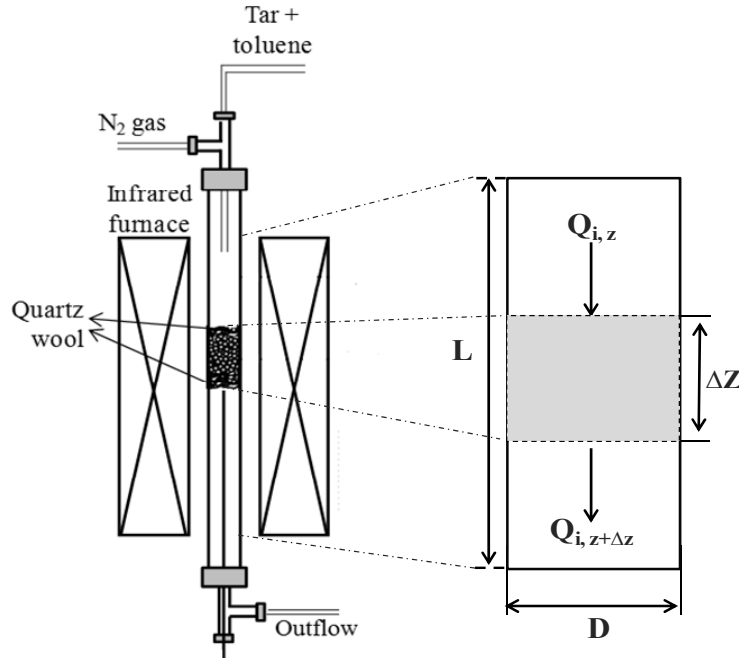
Fig. 3-1 Schematic diagram of continuous fixed bed reactor which used for development of kinetic equation model.
