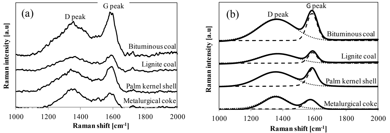
Fig. 4-5 (a) Raman spectra of metallurgical coke and carbon deposited within ore after tar decomposition from various solid fuels. (b) Curve fitting of the Raman spectra into D and G peaks, showing the differences in the intensity ratio.
