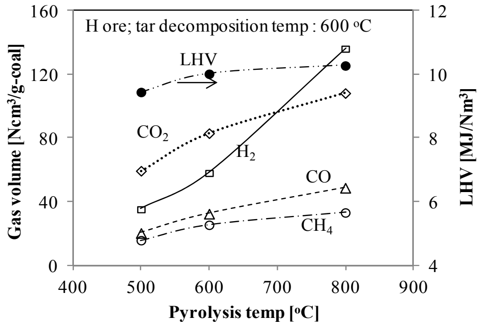
Fig. 2-18 Effect of pyrolysis temperature on gas composition and lower heating value (LHV) of integrated coal pyrolysis–tar decomposition over Hamersley iron ore; each gas volume increased at elevated temperature as a result of thermal cracking of coal and tar components.
