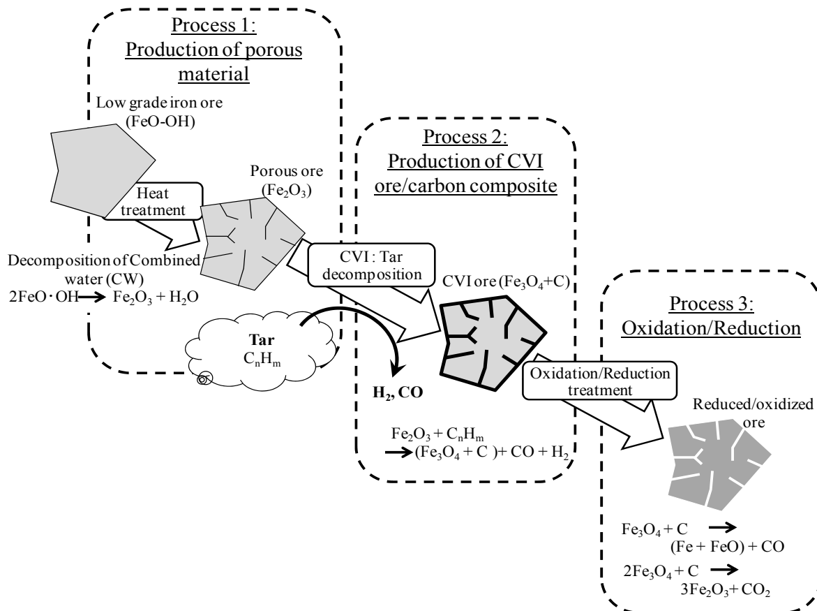
Fig. 1-8 The schematic diagram of CVI ironmaking
