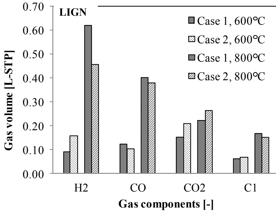
Fig. 2-10 The gas composition produced during the pyrolysis of lignite coal (LIGN) at different temperatures. Case 1: no iron ore; case 2: 3 g of iron ore.
