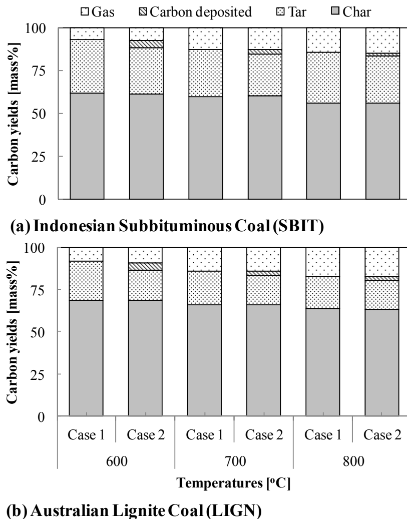
Fig. 2-9 Effect of pisolite iron ore on product distribution due to pyrolysis of two low-grade coals at different temperatures: (a) subbituminous coal from Indonesia (SBIT) and (b) Australian lignite coal (LIGN). Case 1: No iron ore (Pyrolysis), case 2: Fixed bed of 3 g of iron ore (Pyrolysis-Tar decomposition) for 40 min under the a N 2 flow rate of 250 mL/min.
