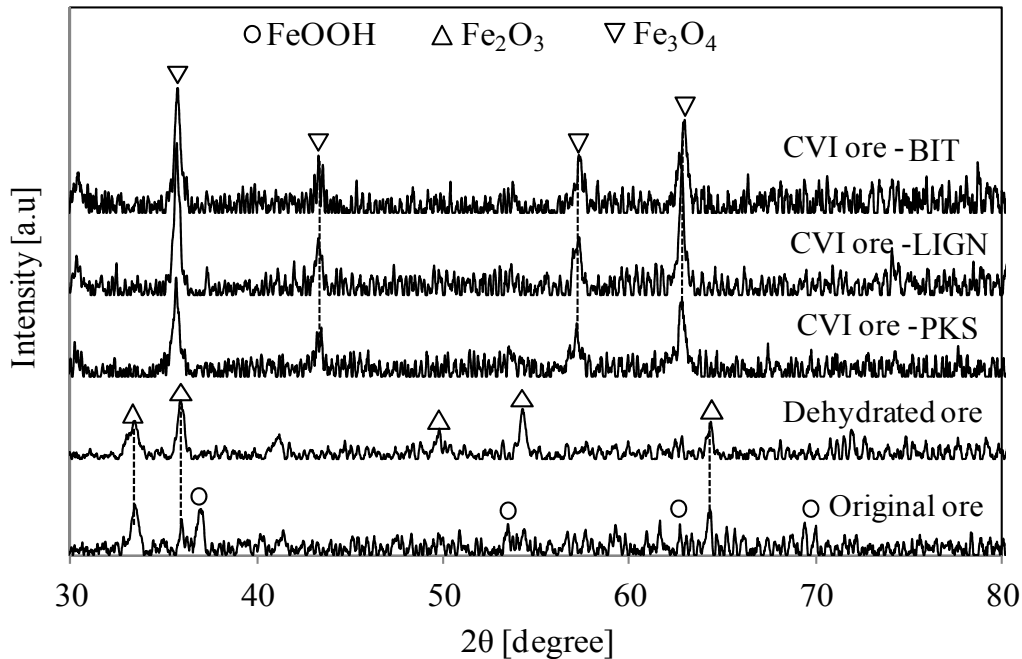
Fig. 2-8 Change of XRD pattern of iron ore for each experiment steps in the pyrolysis-tar decomposition process (case 2). Case 1: no iron ore; case 2: 3 g of iron ore
