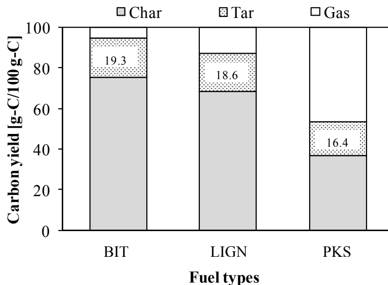
Fig. 2-3 Product distribution of the pyrolysis of various solid fuels at 600°C without tar decomposition treatment (case 1: no iron ore).
