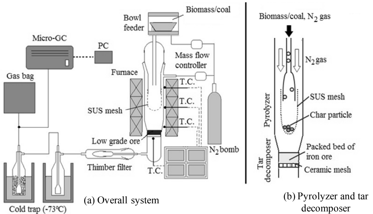
Fig. 2-1 Experimental apparatus for pyrolysis, tar decomposition, and carbon deposition. Case 1: no iron ore; case 2: 3 g of iron ore. Solid fuels were charged at a flow rate of 0.1 g/min for 40 min under N 2 flow rate of 250 mL/min. (T.C.: temperature controller, PC: personal computer, GC: gas chromatography)
