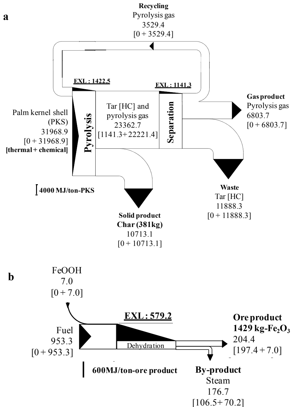
Fig. 5-3 Exergy flowchart of the conventional process (a) for producing of 381 kg-char by pyrolysis of Palm Kernel Shell (PKS) biomass and (b) for producing of 1000 kg-Fe from low grade iron ore (FeOOH) .
