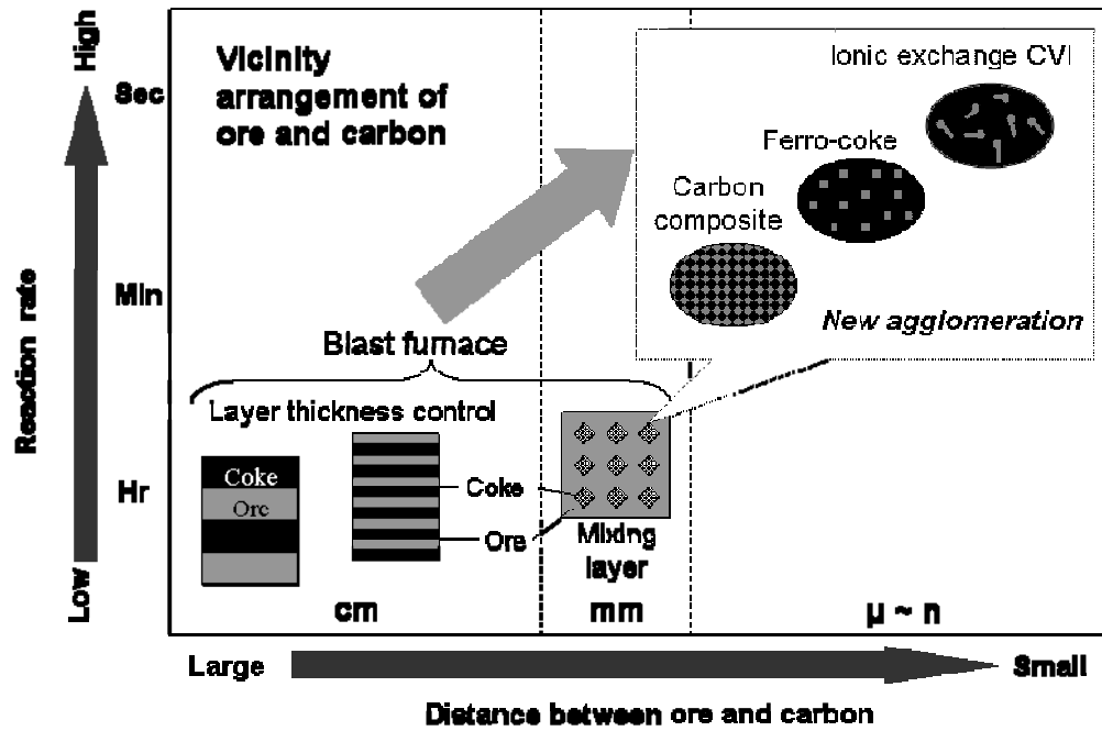
Fig. 1-7 Relationship between reaction rate and arrangement of iron ore and carbon
