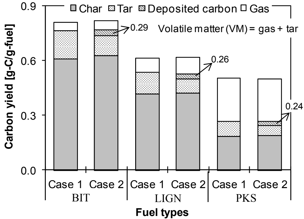
Fig. 2-4 Product distribution of the pyrolysis of various solid fuels at 600°C. Case 1: no iron ore; case 2: 3 g of iron ore.
