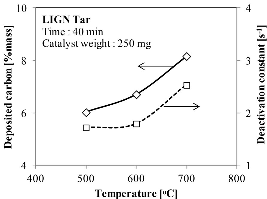
Fig. 3-8 The relationship between deposited carbon and deactivation constant at different temperature shows that the carbon deposition within ore caused decreasing of catalytic activity during tar decomposition process.
