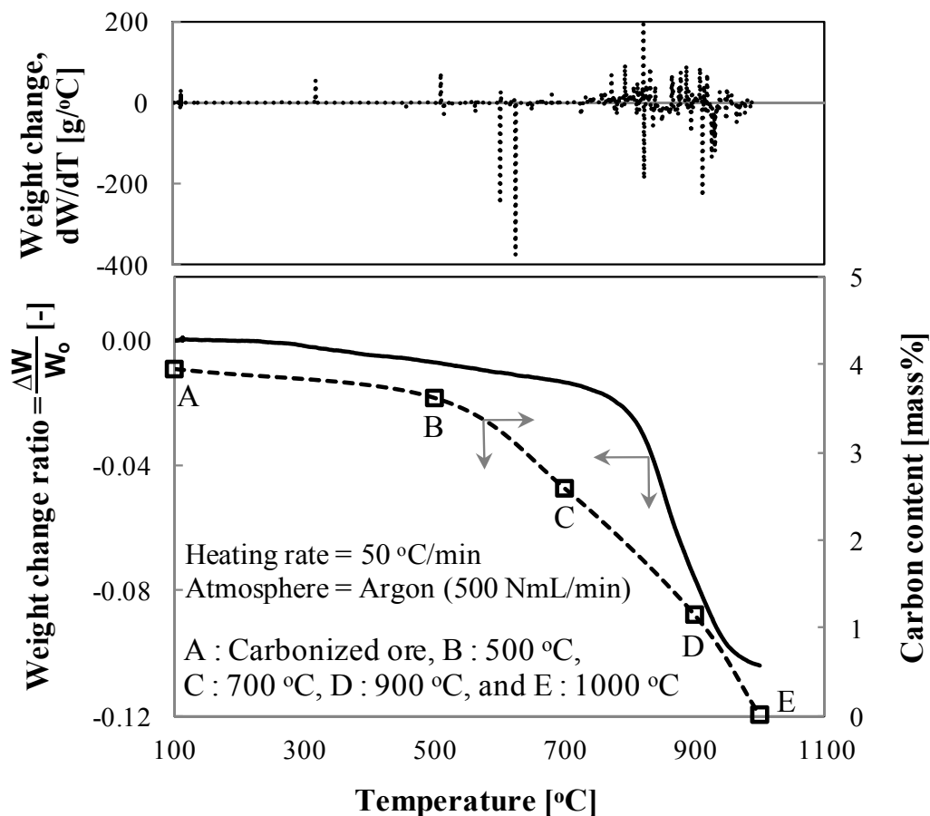
Fig. 2-15 Relationship between the reduction reaction and carbon content during direct reduction, showed that deposited carbon from tar carbonization was consumed and effective in reducing iron ore.
