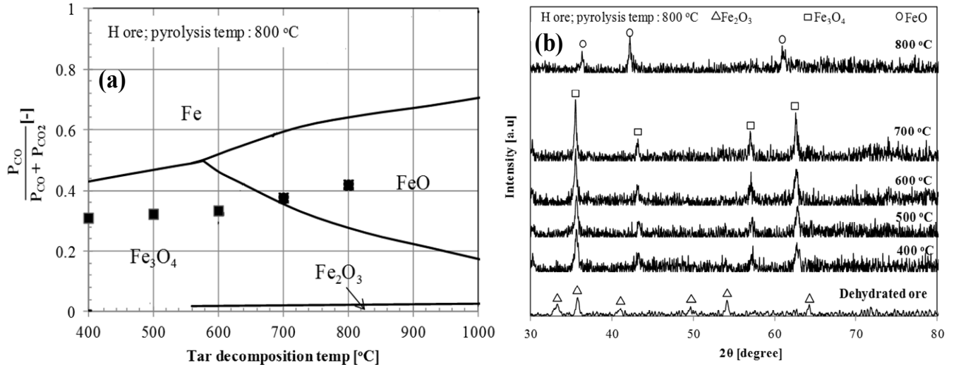
Fig. 2-20 (a) Phase diagrams for iron–wüstite–magnetite systems showed that a high temperature of tar decomposition resulted in a large reduction degree due to high amount of CO and faster reduction rate. (b) X-ray diffraction (XRD) patterns of iron ore after tar decomposition at different temperatures showed that FeO can be found at 800°C; this was consistent with the phase diagram.
