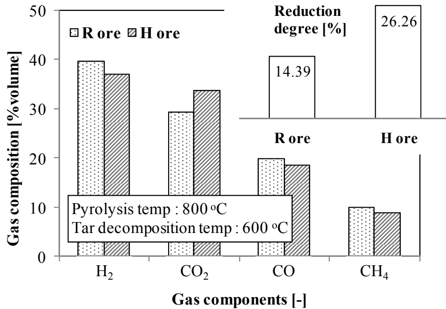
Fig. 2-24 Reduction degree of iron ore and gas composition of integrated coal pyrolysis–tar decomposition with various iron ores [Hamersley (H) and Robe-river (R)] showed that H ore produced smaller mounts of H 2 and CO, but gave higher reduction degrees, as a result of large consumption of these gases in indirect reduction
