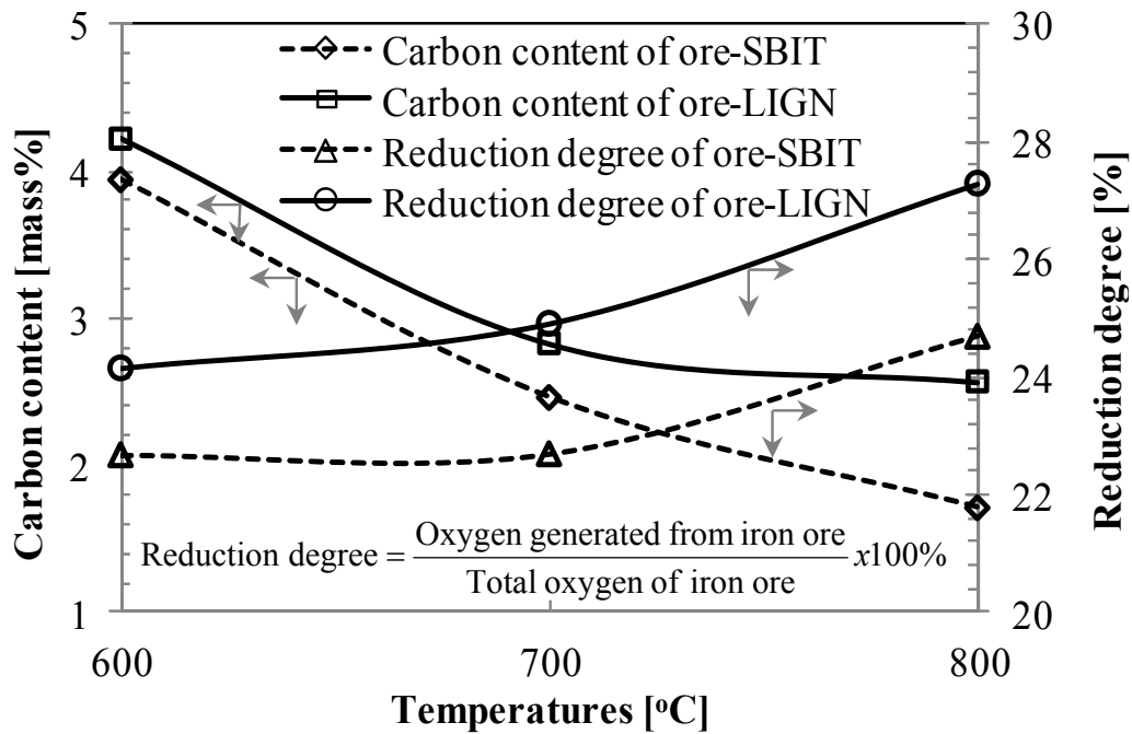
Fig. 2-12 Dependence of carbon deposited within iron ore and degree of reduction of iron ore on temperature, showed similar tendency: with increasing temperature, carbon content decreased and degree of reduction increased.
