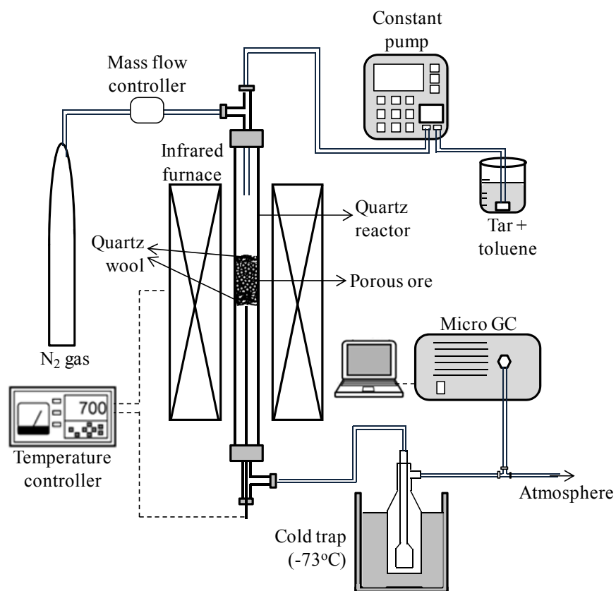
Fig. 3-2 Experimental apparatus for tar decomposition over porous ore. Total tar flow rate and porous ore were 0.25 ml/min and 250 mg , respectively. Toluene was added for tar dilution and preventing of pump problem. GC: gas chromatography.
