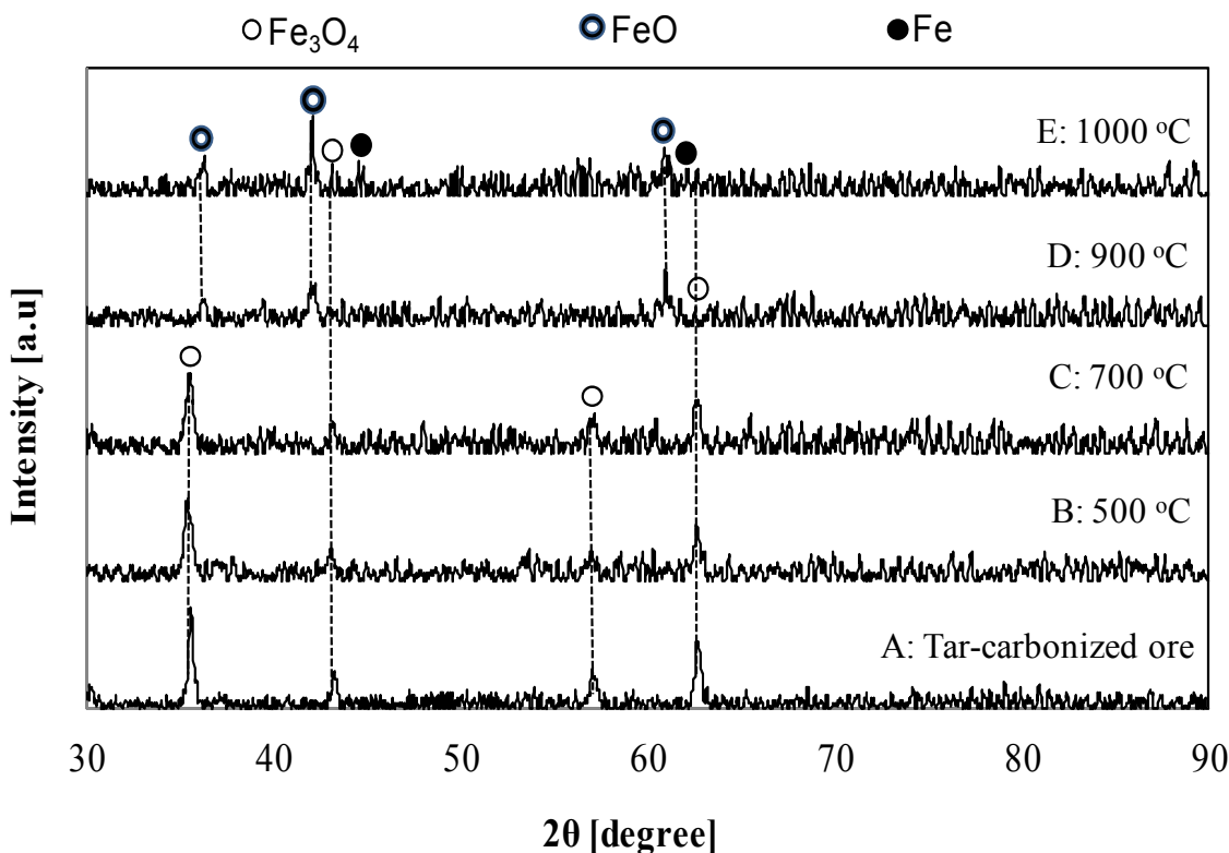
Fig. 2-16 Changes in XRD patterns of tar-carbonized iron ore during direct reduction under Ar at a flow rate of 500 NmL/min, showed that the closely contacted deposited carbon from tar carbonization was effective in reducing iron ore to wustite and metallic iron.
