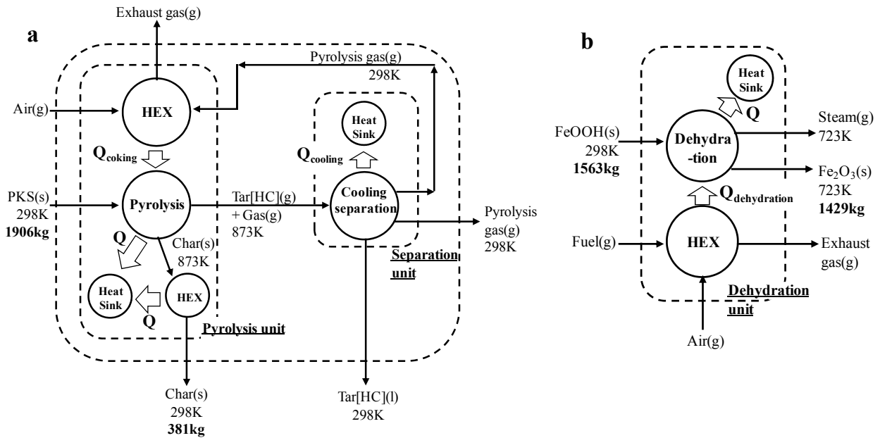
Fig. 5-2 Conventional system for (a) utilization of PKS biomass and producing of 381 kg-char through pyrolysis process and (b) dehydration process to produce 1000 kg-Fe from low grade iron ore (FeOOH) in the ironmaking industry. PKS: Palm Kernel Shell biomass, HC: Heavy hydrocarbon, LC: Light hydrocarbon, HEX: Heat Exchanger, Heat sink means environment, and the dotted line is the boundary of system
