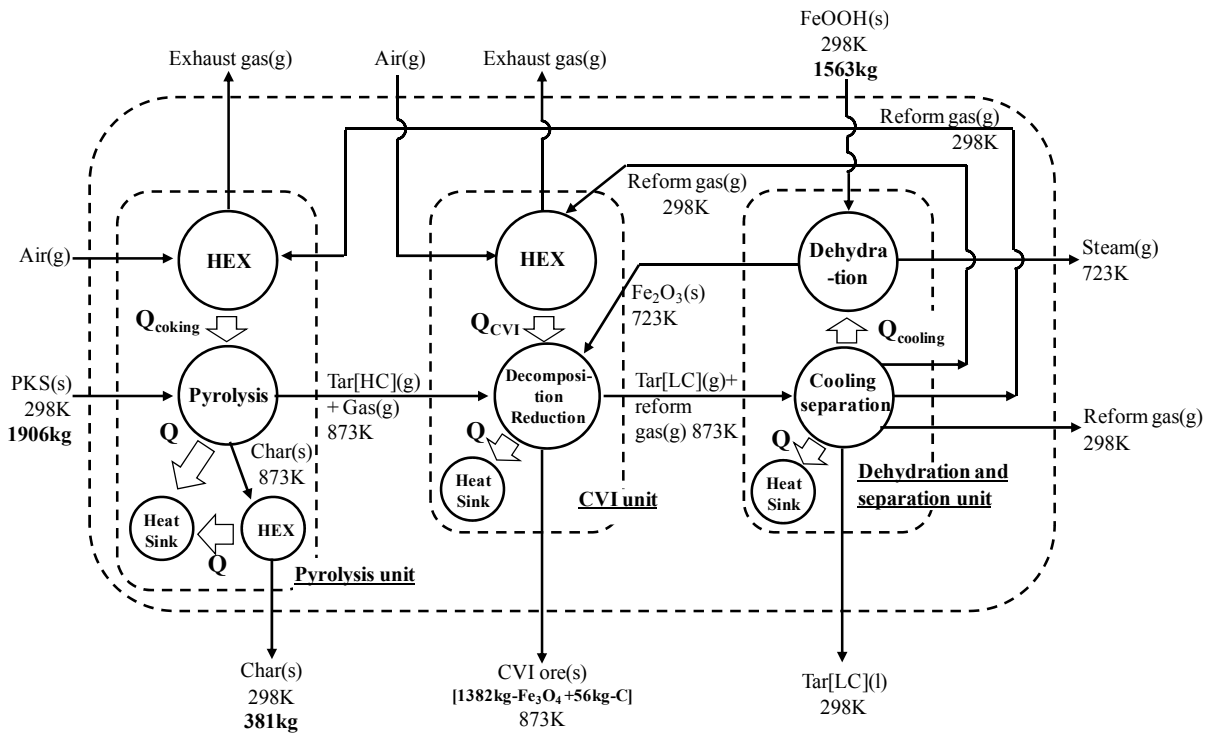
Fig. 5-1 Proposed system for utilization of PKS biomass and low grade iron ore (FeOOH) to produce 381 kg-char and 1000 kg-Fe through CVI ironmaking. PKS: Palm Kernel Shell biomass, HC: Heavy hydrocarbon, LC: Light hydrocarbon, HEX: Heat Exchanger, Heat sink means environment, and the dotted line is the boundary of system.
