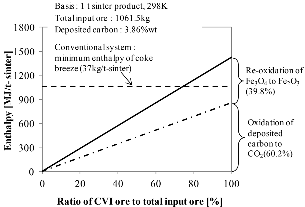
Fig. 5-8 Enthalpy content of the input iron ore in the sinter plant showed that the input enthalpy of CVI ore was higher than the minimum coke enthalpy at ratios of CVI ore above 70%.
