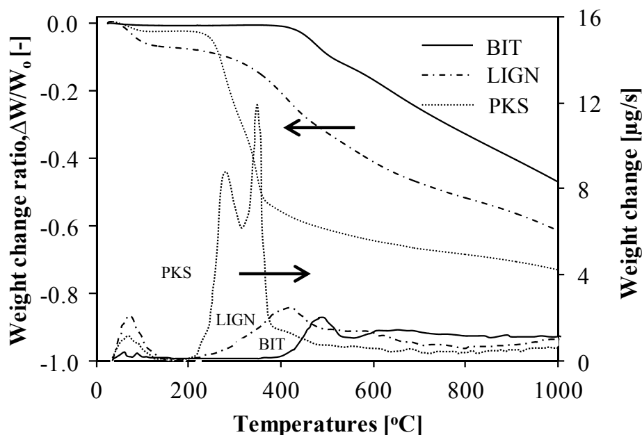
Fig. 2-2 TG/DTG profiles of various solid fuels studied during pyrolysis process at \text{N}_2 atmosphere. Sample weight: 10 mg, particle size: 250–500 \mu\text{m} and heating rate: 50°C/min
