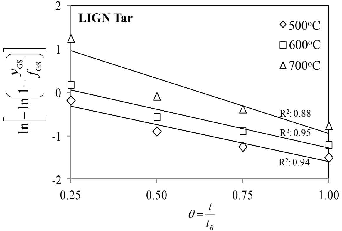
Fig. 3-7 Determination of kinetic parameters using linearization method at different experiment temperatures.
