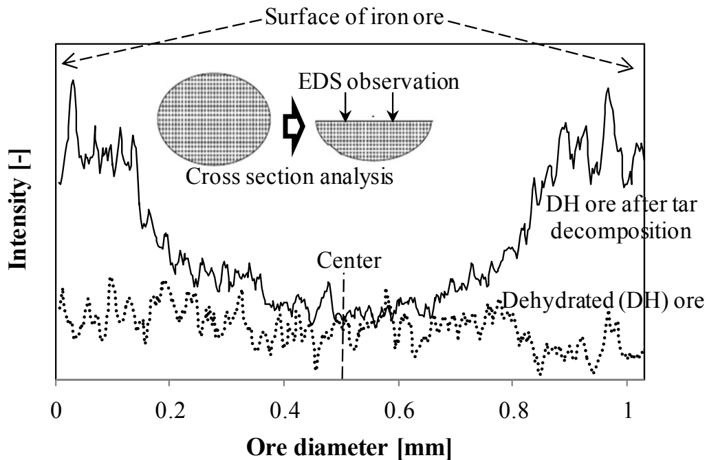
Fig. 4-4 Cross section of EDS line analysis, showing that carbon was deposited from the surface toward the center of porous dehydrated ore.
