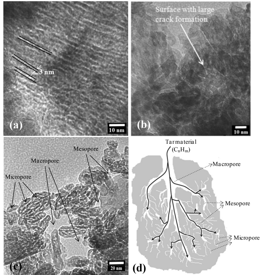
Fig. 4-2 TEM images of dehydrated iron ore at different magnifications: (a) Layered structure of dehydrated ore with a pore size of around 3 nm. (b) Large crack formation in the surface of iron ore. (c) Micropores and macropores within dehydrated iron ore. (d) Graphical representation of porous iron ore during tar decomposition and carbon deposition.
