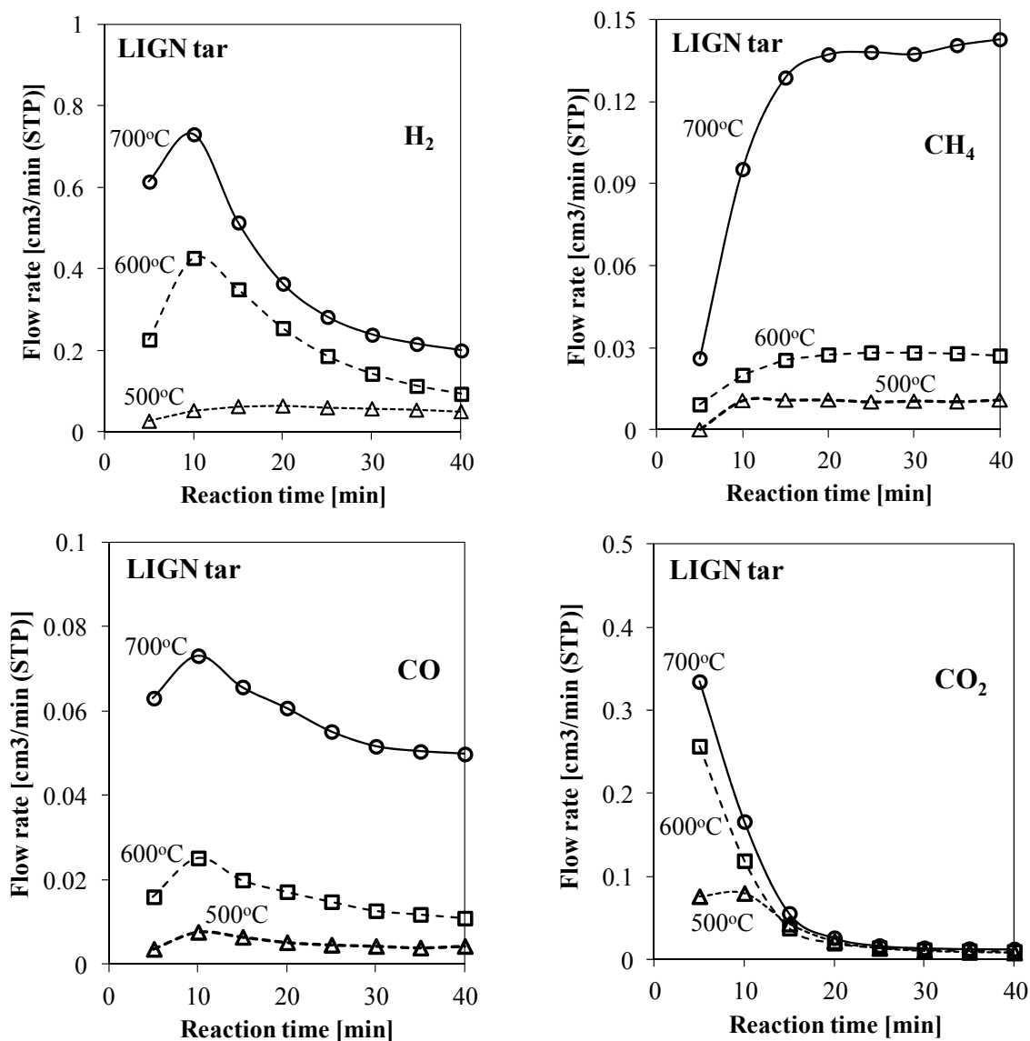
Fig. 3-4 The evolution of gas product during the experiment at various temperature shows that H 2 -CO increased at the beginning step and decreased gradually till end of reaction.
