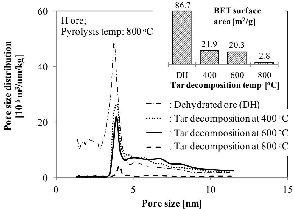
Fig. 2-21 Changes in pore size distributions and BET surface areas of Hamersley ore after tar decomposition at different carbonization temperatures showed that the BET surface area and pore size distribution at 800°C decreased significantly when the amount of deposited carbon was smallest, indicating that sintering started to occur.
