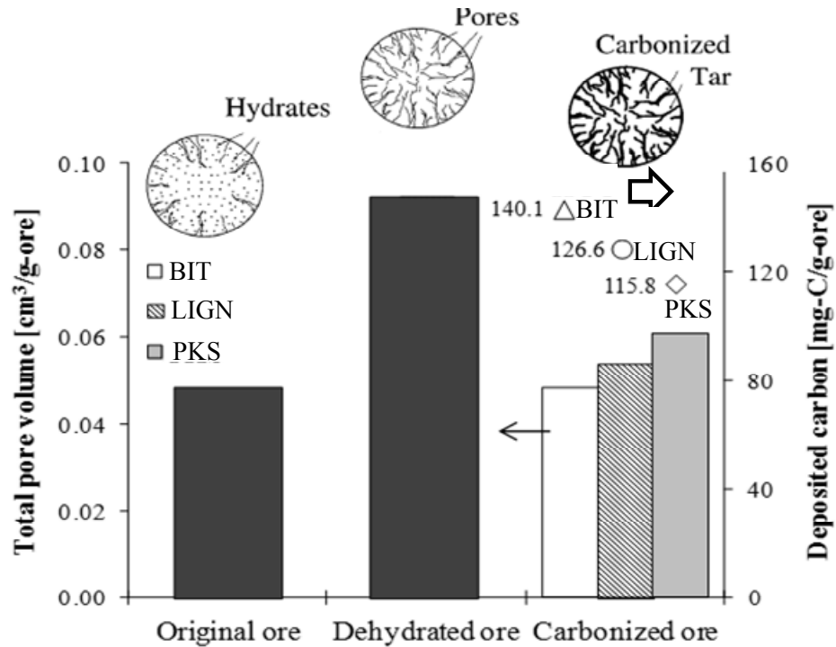
Fig. 2-7 Change in total pore volume of iron ore and the amount of deposited carbon during experiments at 600°C.
