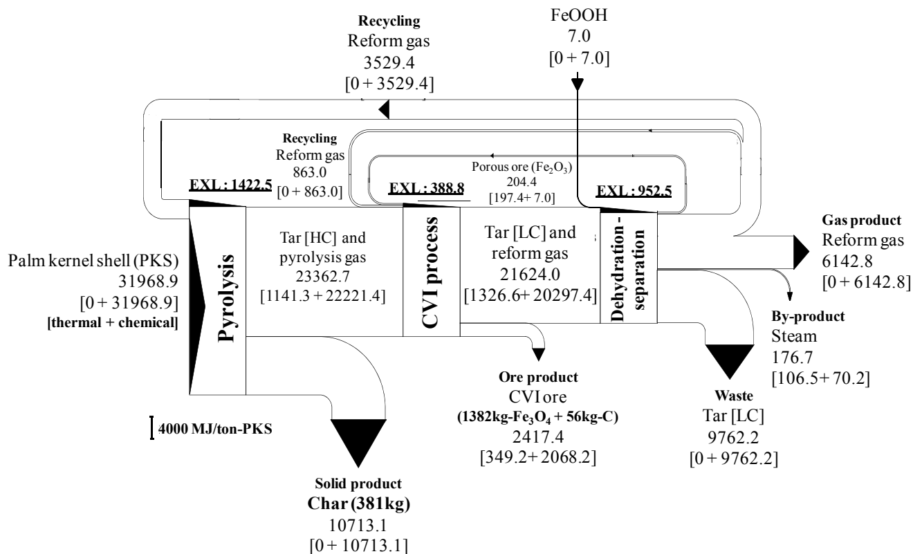
Fig. 5-4 Exergy flowchart of the proposed system for utilization of biomass and low grade iron ore (FeOOH) to produce 381 kg-char and 1000 kg-Fe through integrated pyrolysis-tar decomposition (CVI process). The integrated process showed that the CVI process increased utilization of PKS exergy by decreasing the tar exergy outflow .
