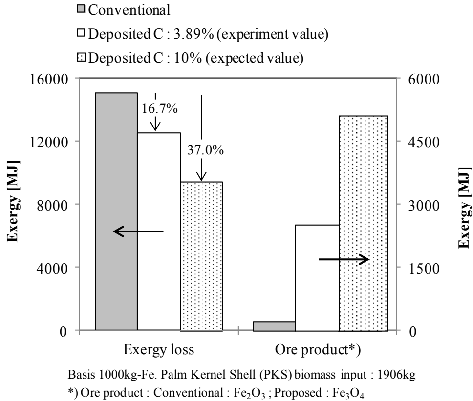
Fig. 5-6 Comparison of exergy losses and ore product for both conventional and proposed system at different amount of deposited carbon showed that the expected value of deposited carbon decreased significantly of exergy loss and enhanced dramatically of ore product exergy.
