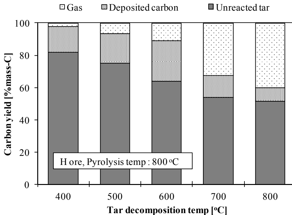
Fig. 2-19 Effect of tar decomposition temperature on tar product distribution; the tar decomposition over Hamersley ore showed that the highest carbon deposition was attained at 600°C, whereas thermal cracking was predominant to produce gases at higher temperatures (>600°C)
