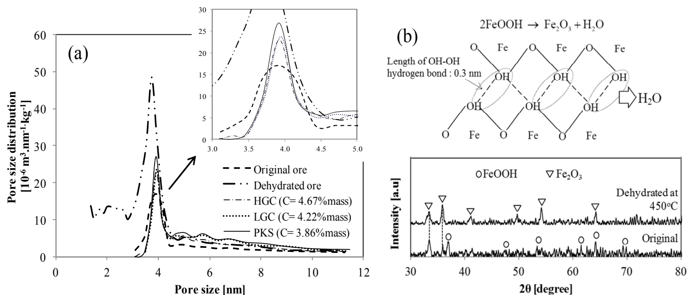
Fig. 4-1 (a) Change in pore size distribution with each experimental step; exhibiting a preference for deposition with pore sizes of less than 4 nm. (b) Effect of dehydration on the removal of the hydroxide (OH) group and the XRD pattern of the low-grade iron ore used.
