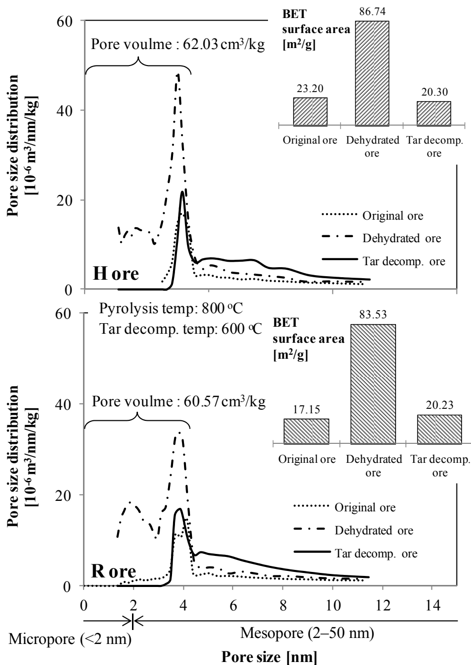
Fig. 2-23 Changes in Brunauer–Emmett–Teller (BET) surface areas and pore size distributions of two different iron ores [Hamersley (H) and Robe-river (R)] showed that larger carbon deposition in the R ore was the result of larger micropores, which were created during dehydration.
