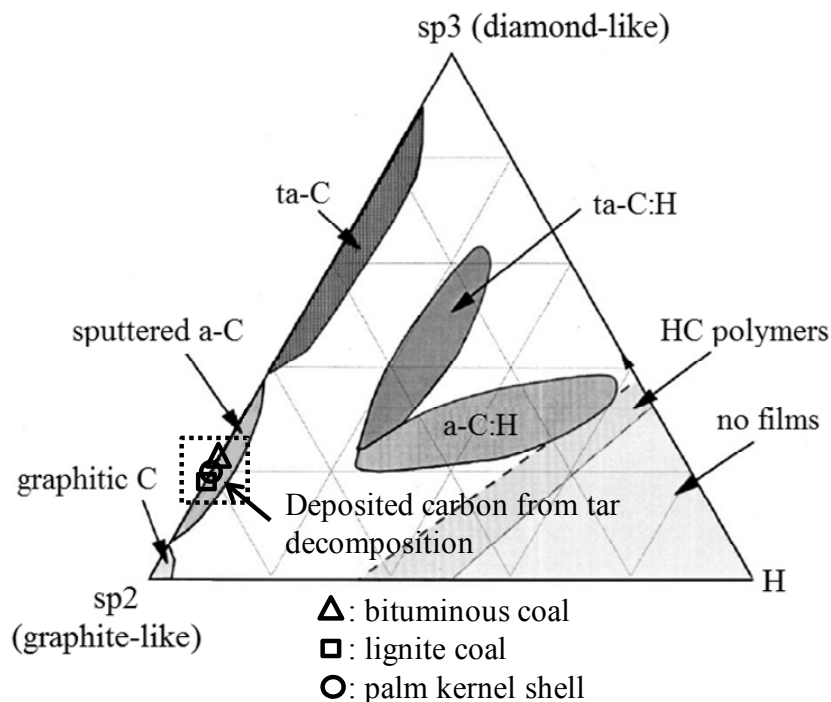
Fig. 4-8 Ternary phase diagram of carbon, showing that carbon deposited by the decomposition of tar from various solid fuels can be categorized as amorphous carbon (a:C) with an sp 3 content of 19–21 %.
