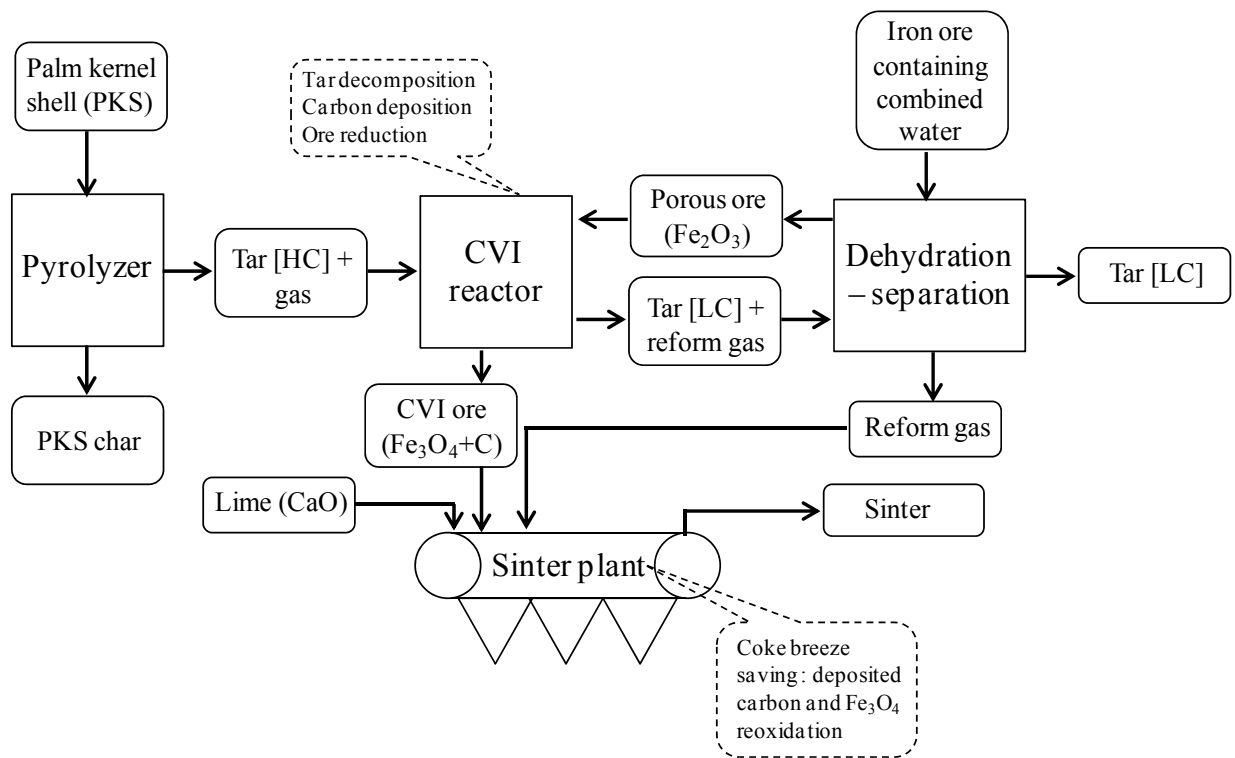
Fig. 5-7 Schematic diagram of CVI ore application in the sinter plant showed that the carbon deposited in the ore had a high potential to reduce the consumption of coke breeze in the ironmaking industry.
