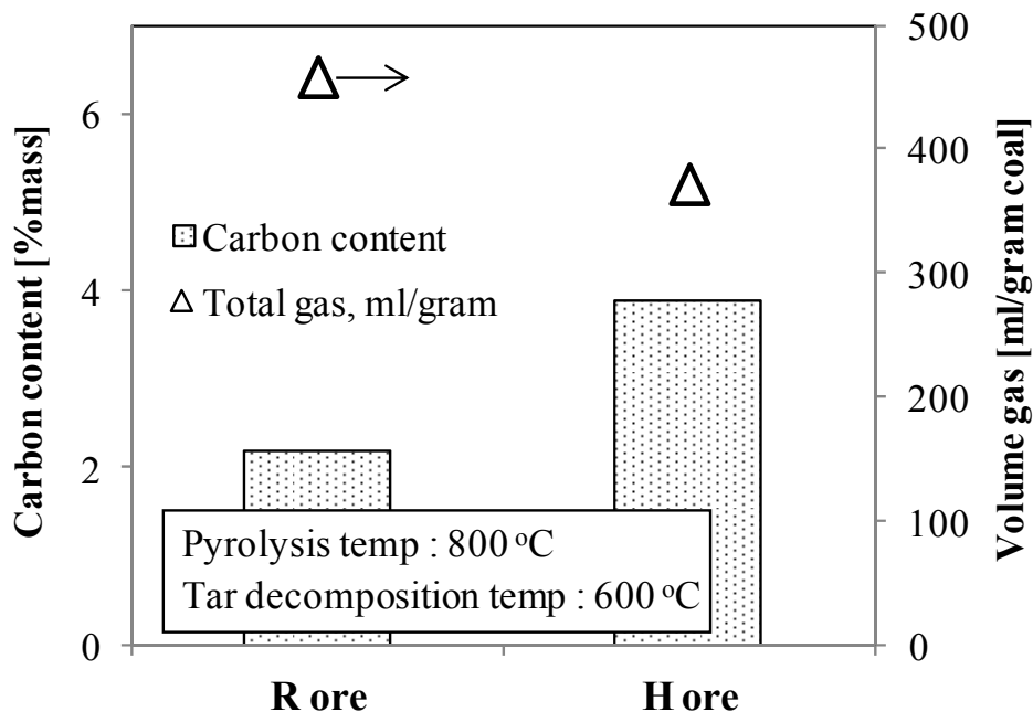
Fig. 2-22 Effect of different iron ores on deposited carbon and total gas volume showed that Hamersley (H) ore gave higher carbon deposition but a lower total gas volume compared with Robe-river (R) ore.
