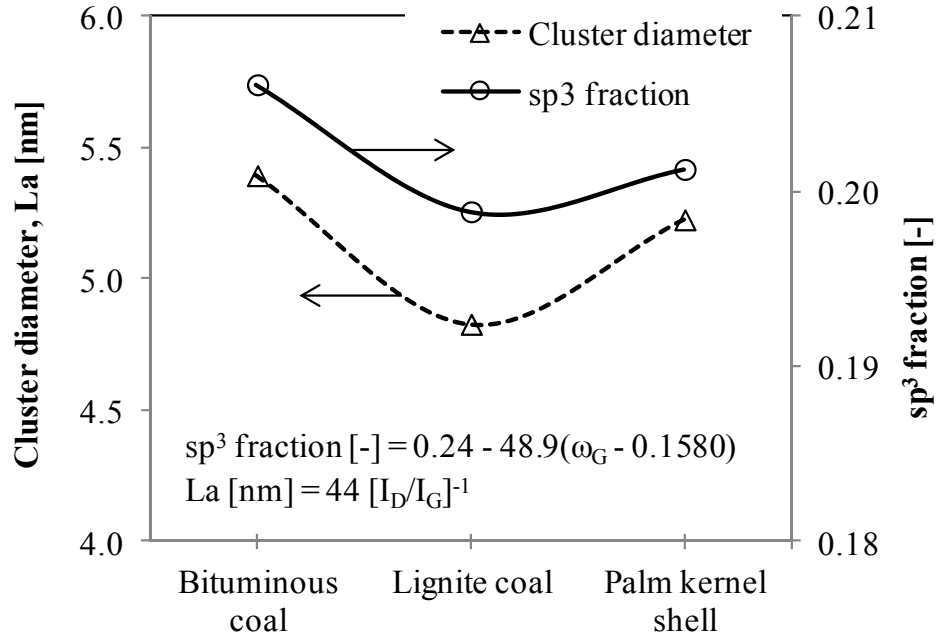
Fig. 4-6 Relationship between sp 3 fraction and cluster diameter of carbon deposited from tar decomposition of various solid fuels.
