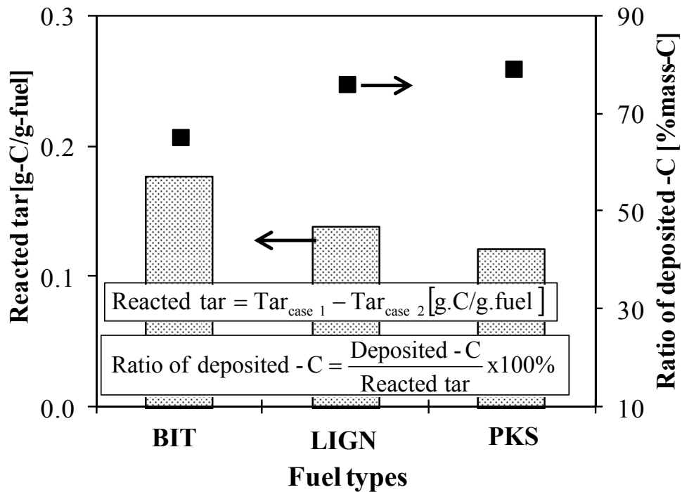
Fig. 2-6 Effect of various fuels on reacted tar and ratio of deposited-C within porous iron ore. Case 1: no iron ore; case 2: 3 g of iron ore
