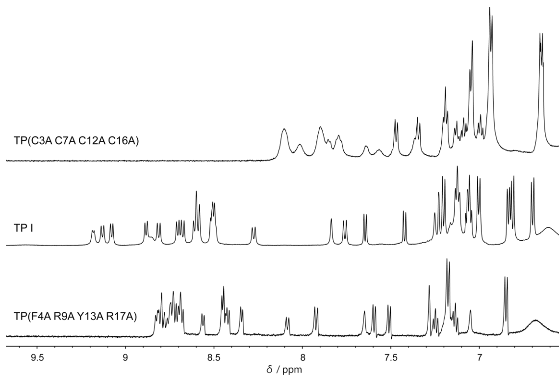
Figure 3. Low-field resonance of the 1D ^1\text{H} NMR spectra of TP(C3A C7A C12A C16A) (top), TP I (middle) and TP(F4A R9A Y13A R17A) (bottom).
