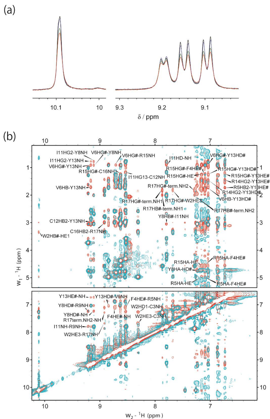
Figure 2. (a) The line-broadening by the addition of LPS to TP I solution. The TP I concentration was 750 \mu\text{M} and the LPS concentration was 0 (black), 20 (blue), 35 (green), or 50 \mu\text{M} (red) in 10% \text{D}_2\text{O} at pH 3.8. These spectra were measured at 35 ^\circ\text{C} . (b) Superimposition of the NOESY spectrum of TP I in water and the Tr-NOESY spectrum of TP I containing LPS. Red-colored peaks were observed in the measurement of Tr-NOESY and blue-colored peaks were obtained by the measurement of NOESY. Assigned peaks were observed only in the presence of LPS.
