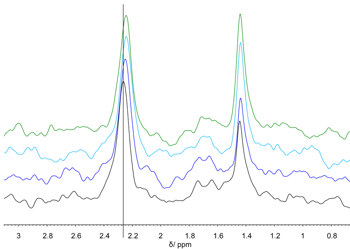
Figure 7. 1D ^{31}\text{P} NMR spectra of LPS with various concentrations of TP I measured at 35 °C. LPS was dissolved in 10% \text{D}_2\text{O} , pH 3.8, at a final concentration of 400 \mu\text{M} . The spectra displayed in black, purple, blue and green indicate LPS:TP I molar ratios of 1:0, 1:0.5, 1:1, and 1:1.5, respectively.
