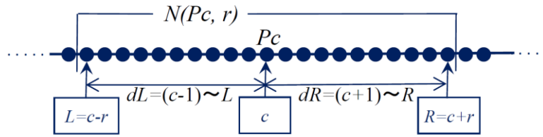
Figure 4. 3 Clustering neighborhood for JSP.
