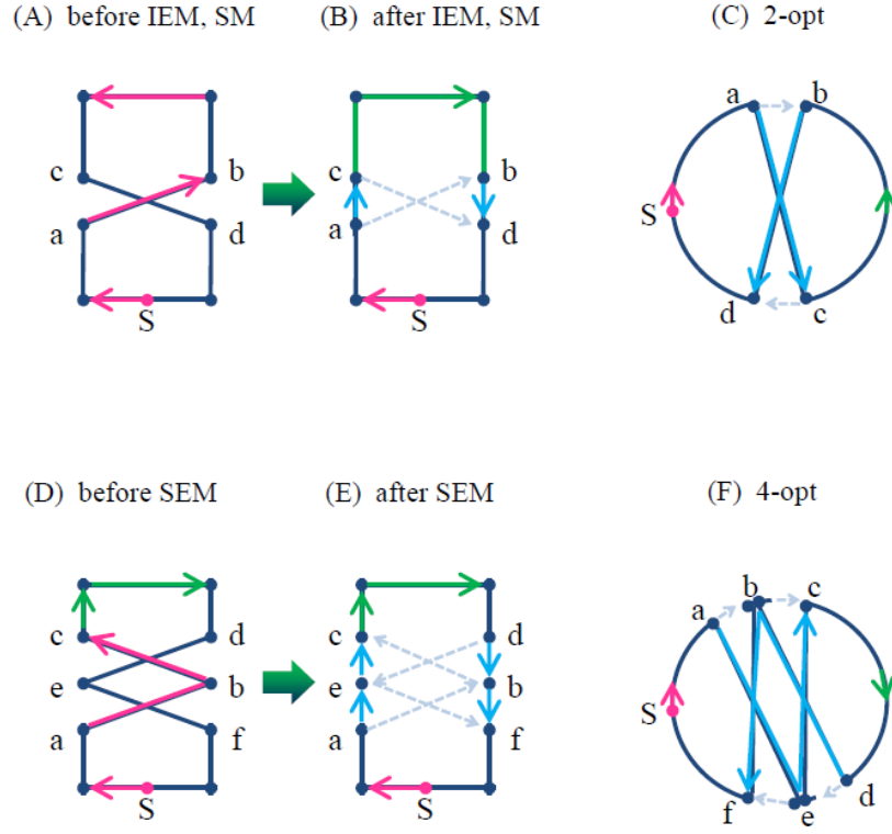
Figure 3.2 Comparison of local clustering with \lambda -opt algorithm in 1 tour.
