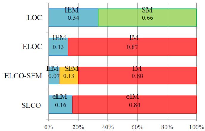
Figure 3.14 Ratio of contribution on cost of tour by LCO, ELCO, ELCO-SEM, and SLCO in usa13509.
