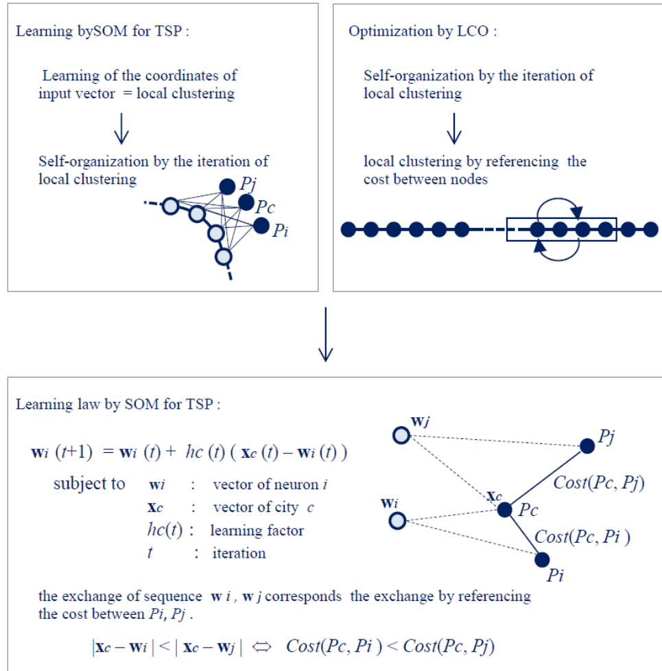
Figure 2.3 Relation of local clustering of LCO and SOM.
