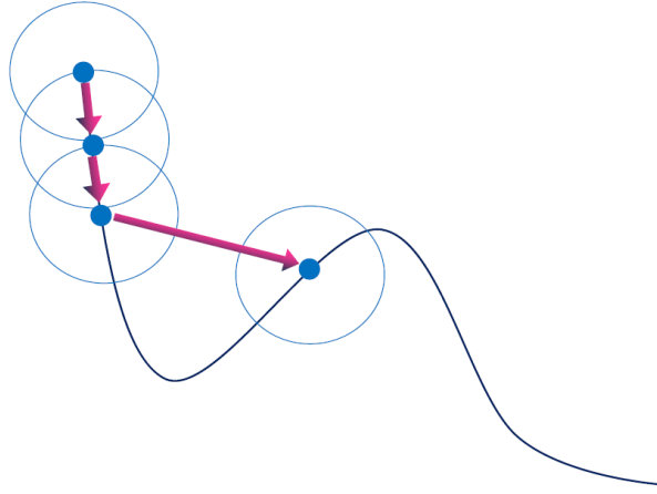
Figure 3.20 Search neighborhood.
