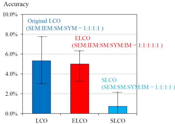
Figure 4. 12 Mean and Range of Error Given by 50Job*20Machine.
