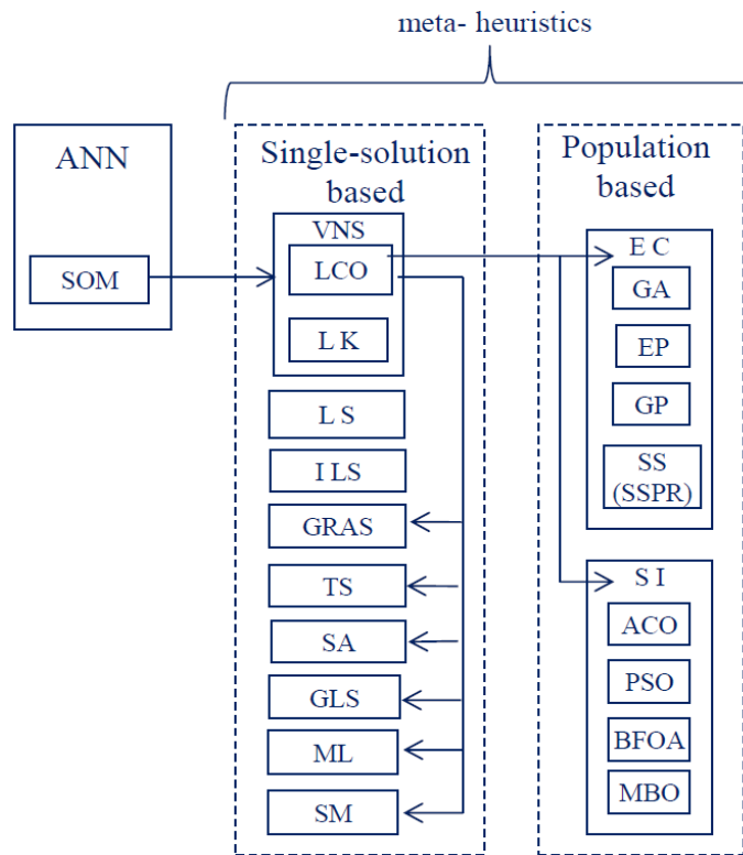
Figure 1. 1 LCO and meta-heuristics.
