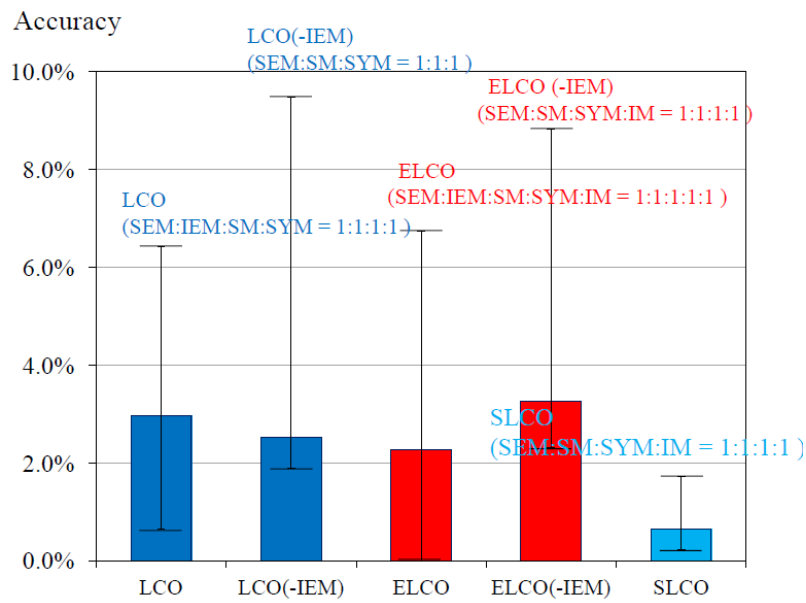
Figure 4. 13 Mean and Range of Error Given by la24 (15Job*10Machine).
