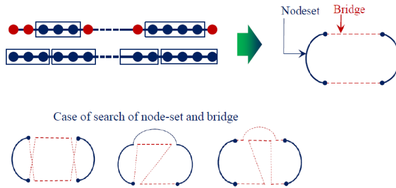
Figure 2. 13 Solution structure of structured local clustering.
