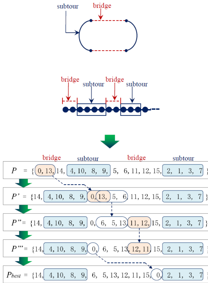
Figure 3.1 Concept of structured local clustering for TSP.
