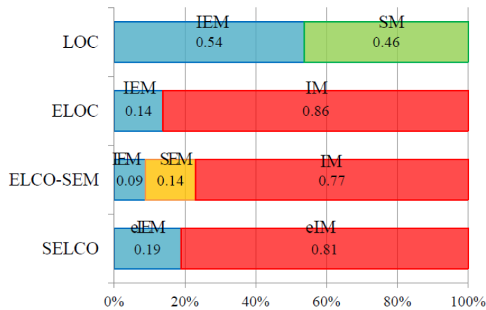
Figure 3.13 Ratio of contribution on number of improvement by LCO, ELCO, ELCO-SEM, and SLCO in usa13509.
