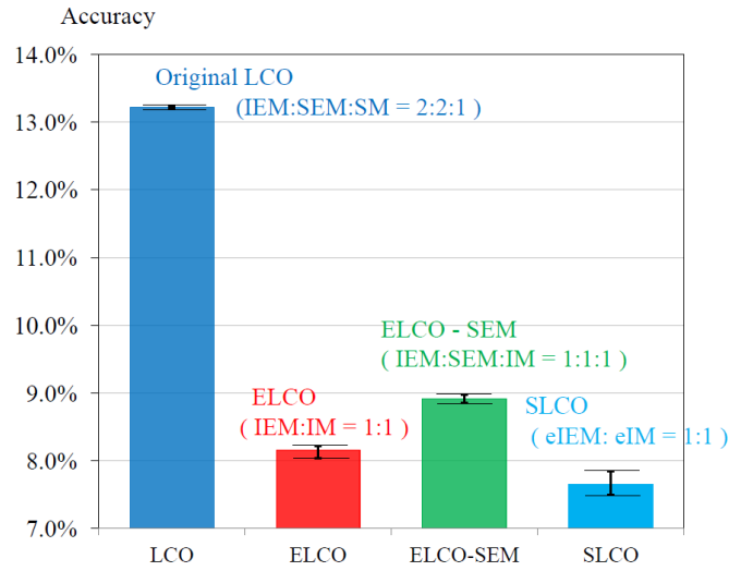
Figure 3.11 Average and the error of obtained cost by LCO, ELCO, ELCO-SEM, and SLCO in usa13509.
