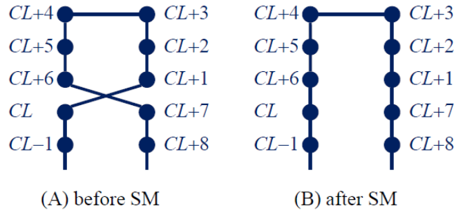
Figure 1.7 Effect of SM (applied to P_{CL} and P_{CL+7} ).
