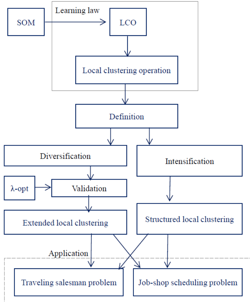
Figure 2. 2 Outline for design of structured local clustering.
