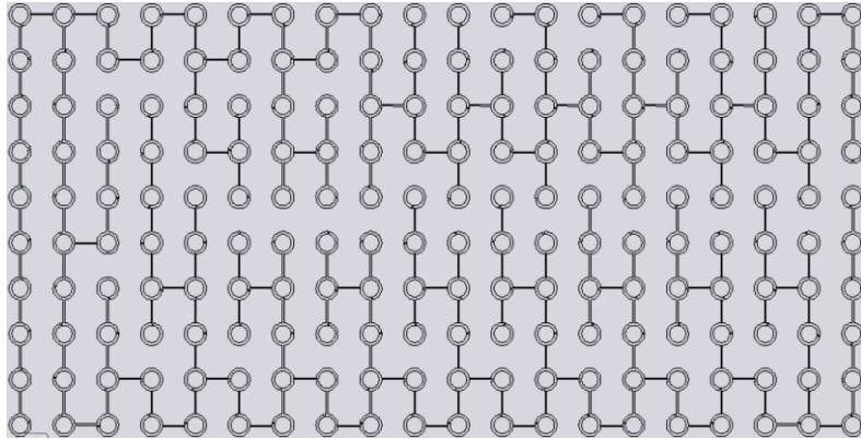
Figure 3.19 Obtained solution by ELCO and D&C applied to the 200-connected double-circles TSP.
