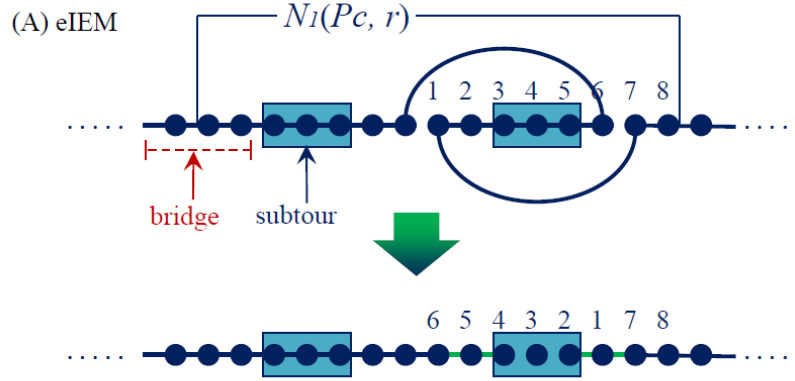
Figure 3. 6 Structured local clustering, eIEM.
