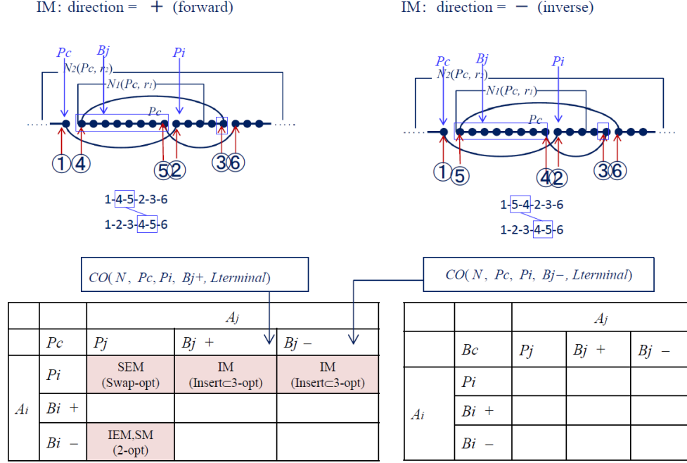
Figure 2. 11 Positioning of extended local clustering.
