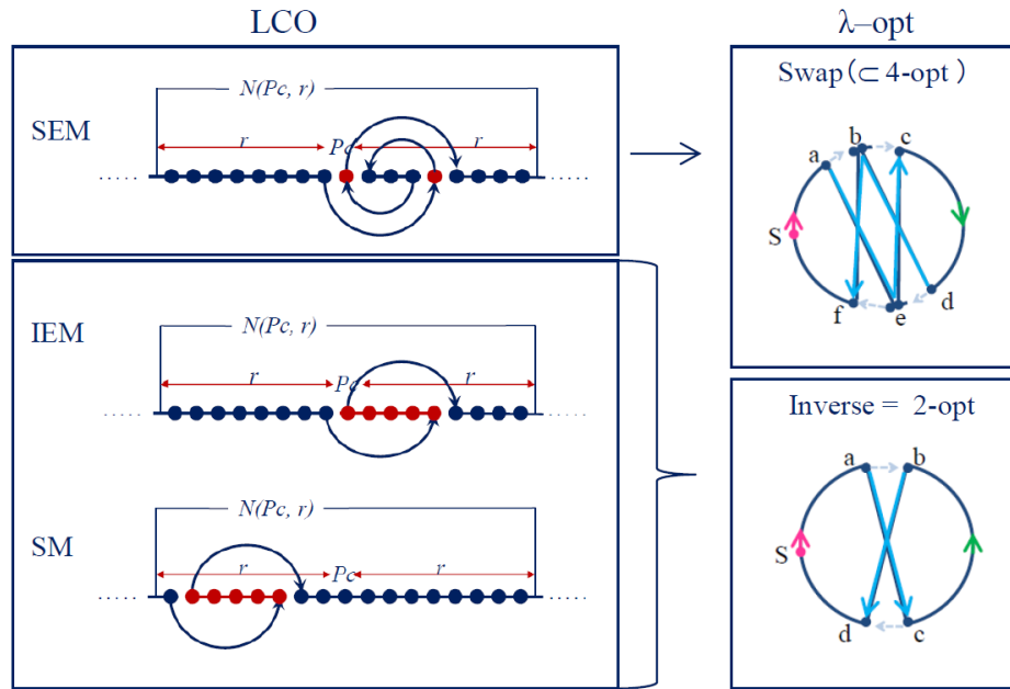
Figure 2. 9 Validation of original LCO by comparison with \lambda -opt.
