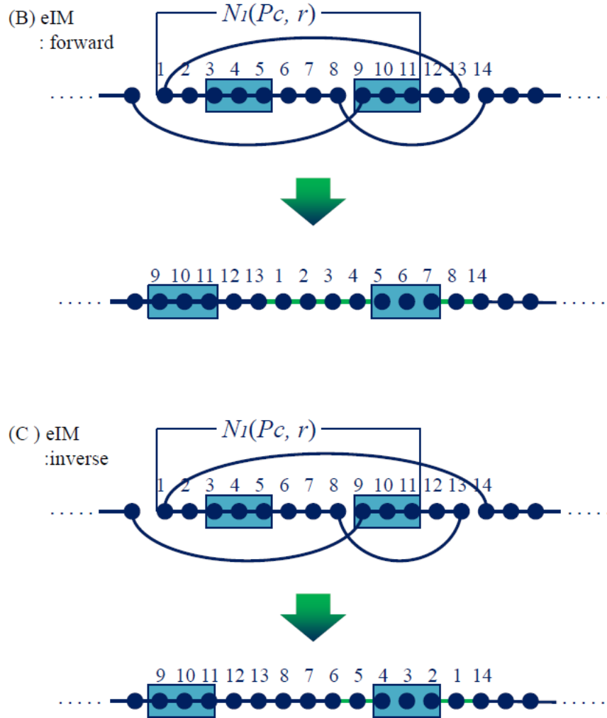
Figure 3.8 Structured local clustering, eIM.
