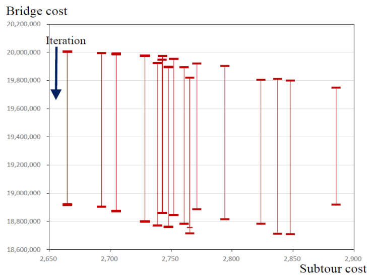
Figure 3.15 Cost to decrease by improvement of SLCO's bridges in usa13509.
