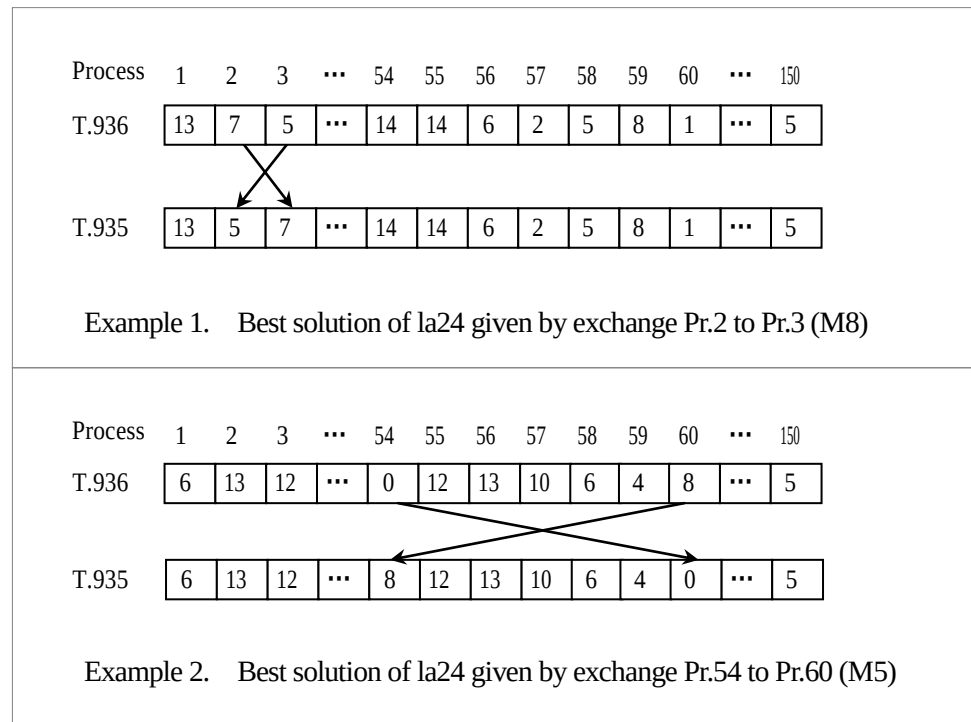
Figure 4. 9 Case of arrival to optimal solution in la24.
