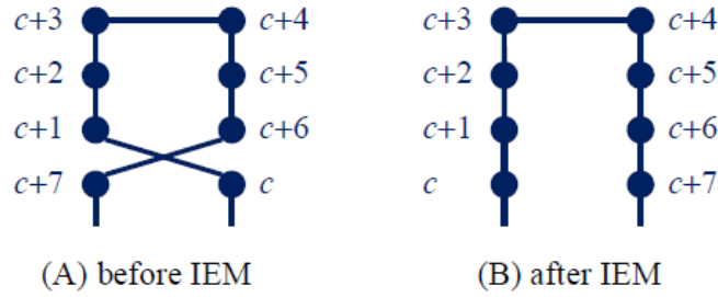
Figure 1.6 Effect of IEM (applied to P_c and P_{c+7} ).
