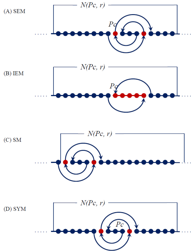
Figure 4.4 Each local clustering, SEM, IEM, SM, and SYM.
