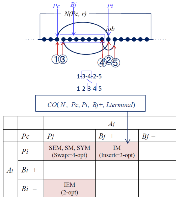
Figure 4. 7 Positioning of IM.
