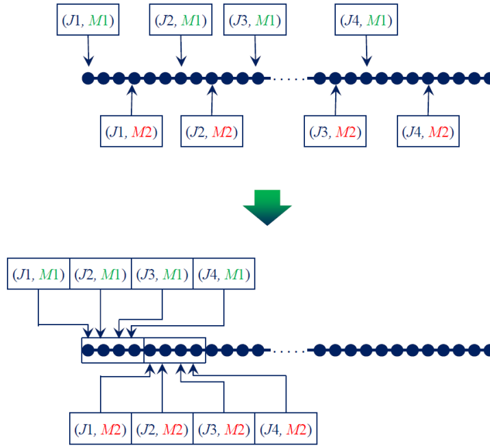
Figure 4. 1 Concept of structured local clustering for JSP.
