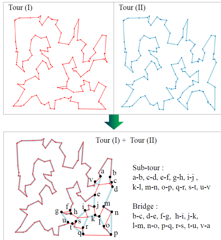
Figure 3. 5 An example of extract subtours and bridges from 2 tours in ch130 by SLCO.
