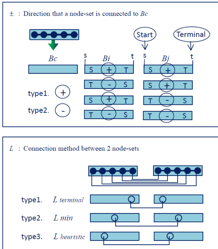
Figure 2. 6 Parameters of node-set operation, direction node-set and connection method.
