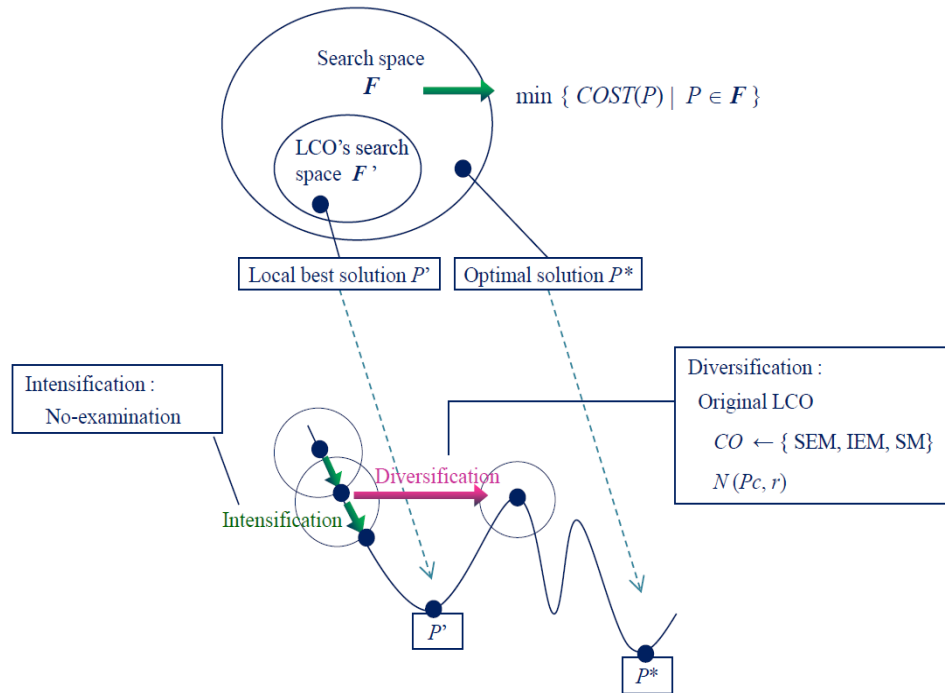
Figure 1. 2 Diversification and intensification of search.
