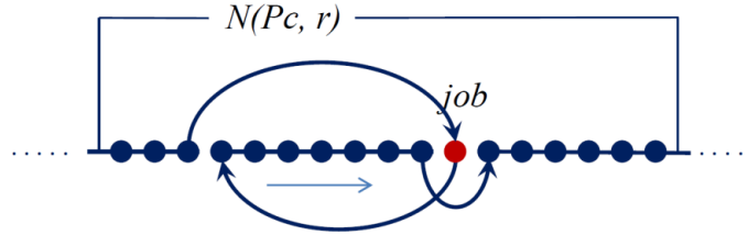
Figure 4. 6 Extended local clustering, IM.
