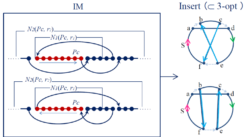
Figure 2. 10 Introduction of extended local clustering.
