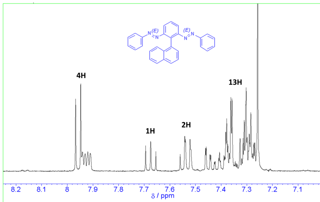
Figure 5: ^1\text{H} NMR Spectra of compound-3 in \text{CDCl}_3 at room temperature
