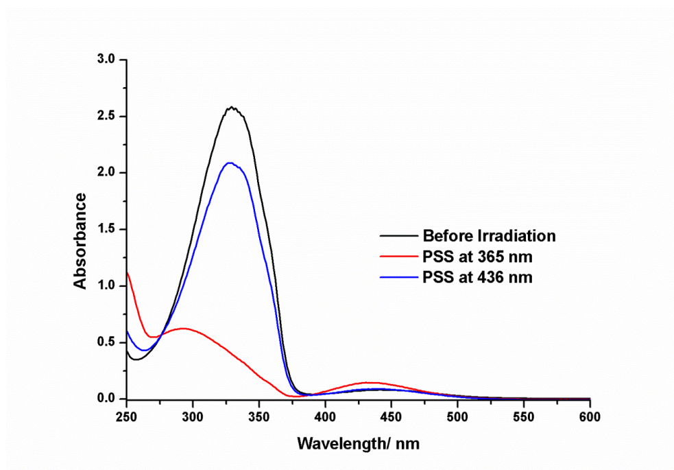
Figure 15: Absorption spectral changes of compound-1 in acetonitrile (5.1 x 10 -4 M)
