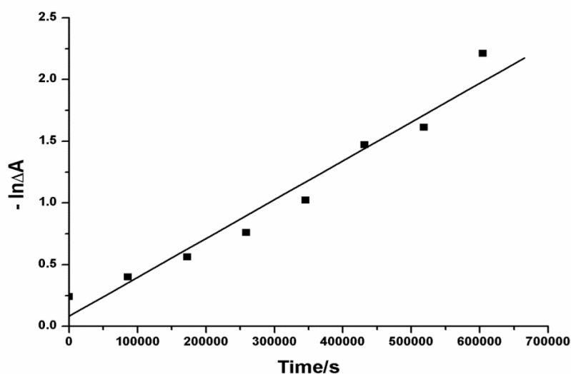
Figure 13: Plot showing linear relationship between logarithm of change in absorbance, -\ln \Delta A ( \Delta A is calculated as \Delta A = A_i - A_t from the absorbance at 320 nm of the UV spectra, where A_i is the initial absorbance before irradiation and A_t is the absorbance at time t
