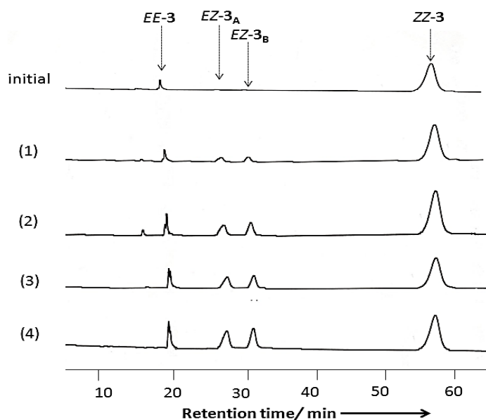
Figure 22: HPLC chromatogram showing ZZ to EE photoisomerization pathway via EZ intermediate a) before irradiation, b) after 10s irradiation at 436 nm and c) the PSS at 436 nm.
