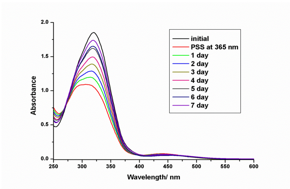
Figure 12: Changes in the UV spectra of acetonitrile solution of 3 ( 1.5 \times 10^{-3} M) during thermal back isomerization after PSS 365 nm at 30 °C under dark for 7 days.
