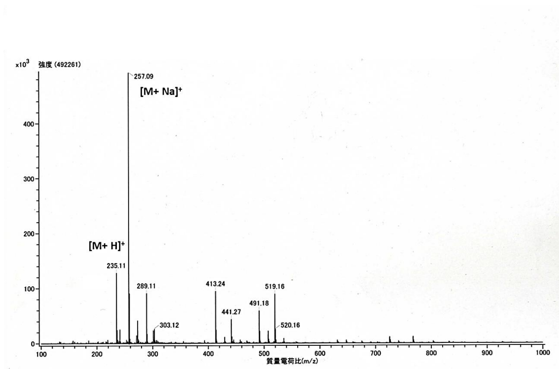
Figure 7: ESI + - Mass Spectra of compound-5 in methanol at room temperature
