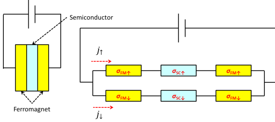
Figure 2.1. Simplified resistor model for device consisting of semiconductor with two ferromagnetic contacts. Two independent spin paths are represented by resistors.
