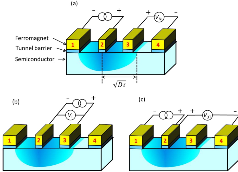
Figure 2.2. Circuit configurations of (a) a four-terminal nonlocal geometry, (b) a local geometry, and (c) three-terminal geometry.
