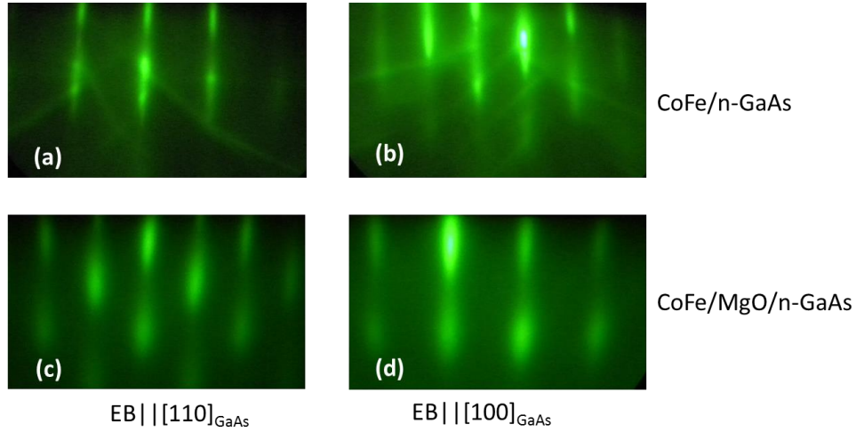
Fig. 3.2. RHEED patterns along the azimuths of [110]_{\text{GaAs}} and [100]_{\text{GaAs}} for CoFe/GaAs and CoFe/MgO/GaAs. (a) CoFe/GaAs with EB|| [110]_{\text{GaAs}} , (b) CoFe/GaAs with EB|| [100]_{\text{GaAs}} , (c) CoFe/MgO/GaAs with EB|| [110]_{\text{GaAs}} , and (d) CoFe/MgO/GaAs with EB|| [100]_{\text{GaAs}} .
