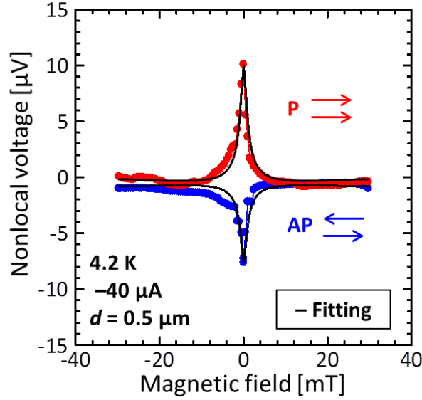
Fig. 3.9. Plot of non-local voltage as a function of out-of-plane magnetic field ( B_z ) for a \text{Co}_2\text{MnSi}/\text{CoFe}/\text{n-GaAs} sample for both P (upper curve) and AP (lower curve) configurations. The solid lines are the result of the fitting using Eq. 3.5.
