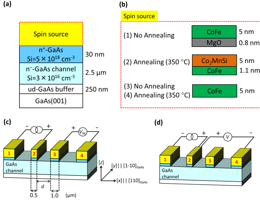
Fig. 3.1. (a) Sample layer structures and (b) Layer structure of spin source. GaAs layers were grown by MBE at 580-600 °C. Four kinds of spin sources were deposited on the same semiconductor structures. (1) CoFe/MgO/n-GaAs without annealing, (2) Co 2 MnSi/CoFe/n-GaAs annealed at 350 °C, (3) CoFe/n-GaAs without annealing to compare with (1), and CoFe/n-GaAs annealed at 350 °C to compare with (2). (c) Schematic device structure of a four-terminal lateral spin-transport device and circuit configuration for nonlocal measurements. (d) Circuit configuration for measuring the TAMR effect.
