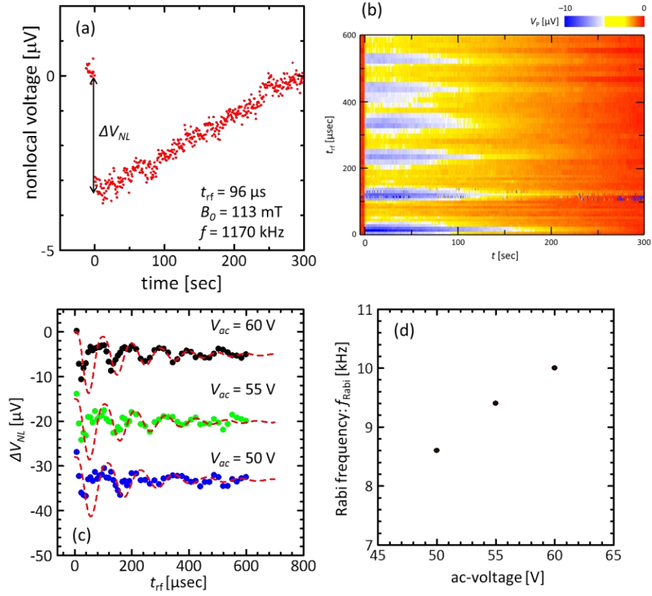
Figure 5.9 (a) Time ( t ) evolution of nonlocal voltage. A pulsed rf-magnetic field having width of t_{rf} was induced at t = 0 . Amplitude of nonlocal voltage change \Delta V_{NL} , defined by V_{NL}(t = 0) - V_{NL}(t = 300) , indicates final states of nuclear spins immediately after the rf-magnetic field pulse radiation. Similar measurements were carried out with different t_{rf} . (b) A color scale plot of V_{NL} as a function of t_{rf} and t . (c) t_{rf} dependence of V_P with different ac-voltage for the coil to apply rf-magnetic fields. (d) Applied ac-voltage dependence of f_{Rabi} . f_{Rabi} was lineally increased with increasing ac-voltage due to 2\pi f_{Rabi} = \gamma B_{rf} .
