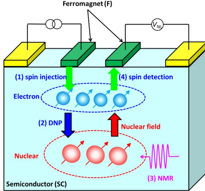
Figure 5.1. A novel NMR system using spin injection devise for quantum bit application. (1) Electron spin injection from \text{Co}_2\text{MnSi} into GaAs, (2) nuclear spin polarization through DNP, (3) quantum operation of the nuclear spin quantum bit through NMR, (4) and finally, detection of the nuclear spin state through detection of the nuclear field acting on electron spins.
