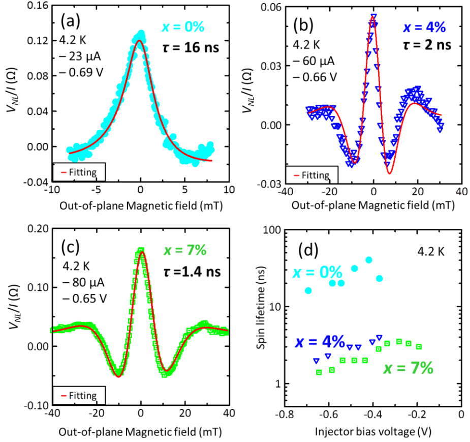
Fig 4.3. (a)-(c) Plots of V_{NL}/I for devices with d = 8.0 \mu\text{m} as a function of out-of-plane magnetic field ( B_z ) for samples with x = 0, 4, 7\% , respectively. The solid lines are the result of the fitting using Eq. 4.1. (d) Comparison of bias voltage dependence of spin lifetime with different indium composition.
