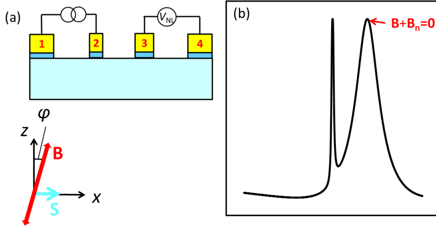
Figure 2.6. Schematics of (a) the measurement configuration for the oblique Hanle effect (b) an steady-state oblique Hanle signal. At the side peak, total magnetic field for electron is zero, resulting in no spin precession.
