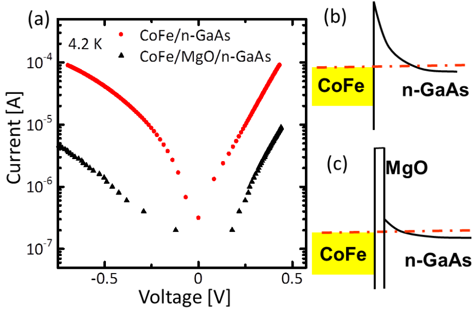
Fig. 3.3. (a) I - V characteristics measured at 4.2K for CoFe/n-GaAs single junctions with and without a MgO barrier. Both curves show non-linear and almost symmetric behavior with respect to the bias voltage polarity due to electron tunneling through a Schottky barrier for the CoFe/n-GaAs and a MgO barrier for the CoFe/MgO/n-GaAs junction. (b), (c) Schematic band diagrams for (b) CoFe/n-GaAs Schottky tunnel junction and (c) CoFe/MgO/n-GaAs tunnel junction.
