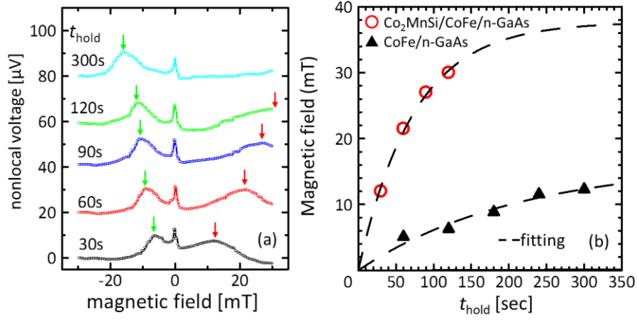
Figure 5.5. (a) t_{\text{hold}} dependence oblique Hanle signals. t_{\text{hold}} ranging from 30 to 300 seconds (b) The t_{\text{hold}} dependence of the observed satellite peak position at B_{\text{ob}} > 0 for a \text{Co}_2\text{MnSi/CoFe/n-GaAs} sample and a \text{CoFe/n-GaAs} sample. The satellite peak position shows almost exponential dependence (dash line).
