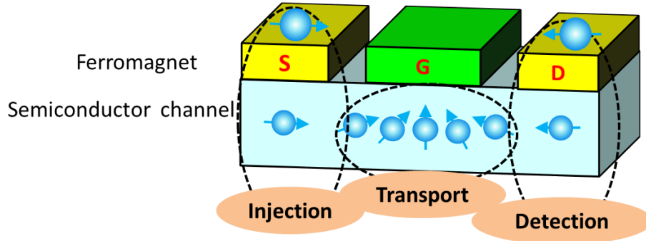
Figure 1.1. Schematic images of spin transistor proposed by Datta and Das. Electron spins are injected from ferromagnet source(S) contact and are detected at ferromagnet drain(D) contact. Polarized spins are controlled by a gate controllable spin-orbit-interaction.
