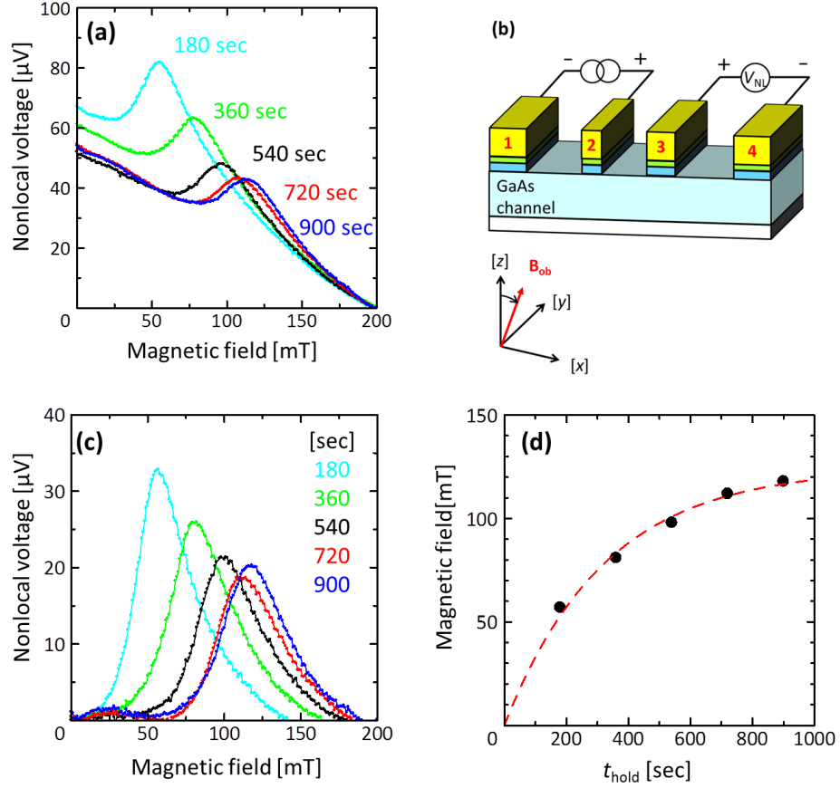
Figure 5.6. (a) Oblique Hanle signals with different t_{\text{hold}} . Injection current of 90 \mu\text{A} was applied with initializing magnetic field of 200 mT for t_{\text{hold}} seconds at 4.2 K. Due to the anti-parallel configuration between nuclear field and external field, electron spins stop precession at the side peak. (b) Schematic geometry of the oblique Hanle measurements. The magnetic field was applied along the direction oblique by approximately 5 degree from the z -axis in the x - z plane. (c) Oblique Hanle signals with subtracting linear component from Fig. 5.6(a). The peak height decreased and the full width at half maximum increased as the t_{\text{hold}} increased, suggesting the distribution of the nuclear spins increased. (d) t_{\text{hold}} dependence of the peak position. Exponential dependence was obtained as discussed in the Sec. 5.3.
