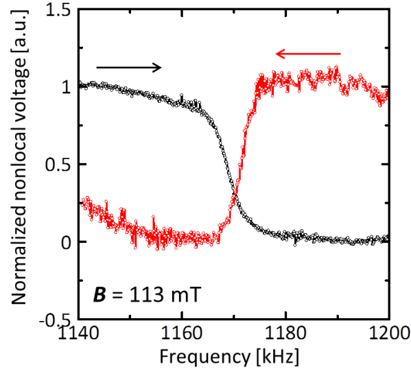
Figure 5.8. Frequency dependence of the nonlocal voltage with a static magnetic field of 113 mT. The rf-magnetic field was continuously applied and the frequency of the rf-magnetic field was swept from higher (lower) to lower (higher) frequency, corresponding to the red (black) curve.
