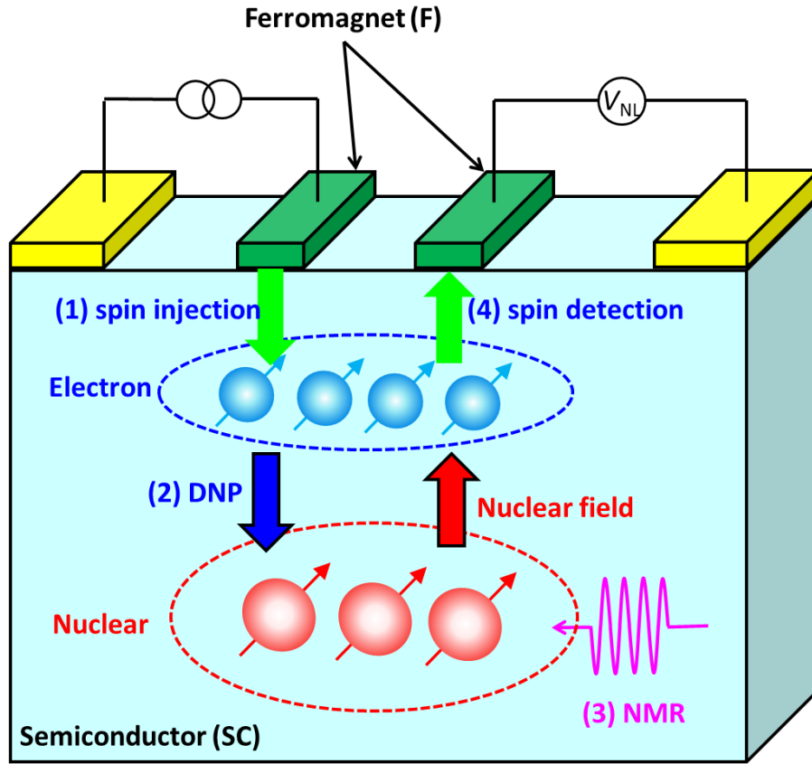
Figure 1.2. Novel NMR system using spin injection device for quantum bit applications. (1) Electron spin injection from \text{Co}_2\text{MnSi} into GaAs, (2) nuclear spin polarization using DNP, (3) quantum control of nuclear spin quantum bits using NMR, and (4) finally, determination of nuclear spin state by detecting nuclear field acting on electron spins.
