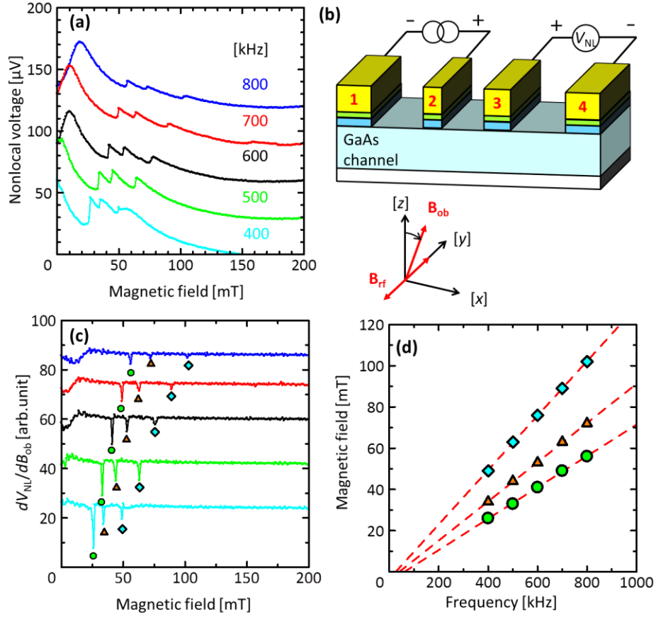
Figure 5.7. (a) Oblique Hanle signals for t_{\text{hold}} = 180 seconds with rf-magnetic field of 400-800 kHz applied. (b) Schematic geometry of the oblique Hanle measurements. The rf-magnetic field was applied parallel to the y-axis direction. (c) The derivative of oblique Hanle signals with rf-magnetic field. Clear three resonant positions were extracted. (d) Applied frequency dependence of the dip positions. Linear dependences were obtained between the applied frequency and the dip positions. The slopes of the curves for the dip positions vs. frequency were close to respective gyromagnetic ratio values of ^{71}\text{Ga} , ^{69}\text{Ga} , and ^{75}\text{As} , indicating that the origin of the dips was NMR.
