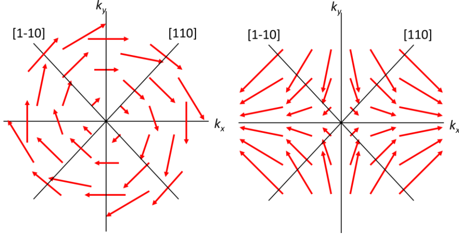
Figure 2.5. Schematics of the effective magnetic field (a) Rashba SOI and (b) Dresselhaus SOI. Thin arrows represent a vector plot of the spin orbit effective field.
