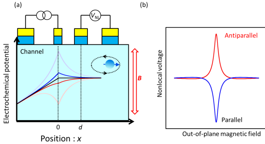
Figure 2.4. (a) Splitting of electro chemical potential for up and down spins. Due to out-of-plane magnetic field, electron spins precess, resulting in reduction of the splitting. (b) Schematic Hanle signals with parallel, antiparallel.
