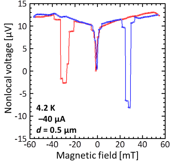
Fig. 3.8. Plot of non-local voltage as a function of in-plane magnetic field ( B_x ) for a lateral spin transport device with \text{Co}_2\text{MnSi}/\text{CoFe}/\text{n-GaAs} junctions. A background signal consisting of a constant term and linear and quadratic terms of B_x has been subtracted.
