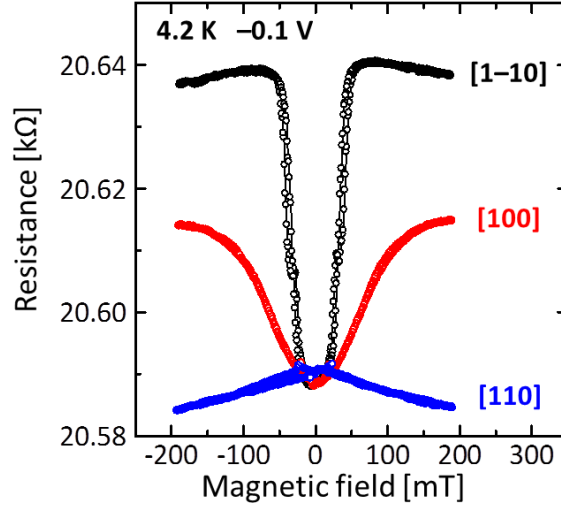
Fig. 3.7. MR curves measured at 4.2K for \text{Co}_2\text{MnSi}/\text{CoFe}/\text{n-GaAs} single junctions. An in-plane magnetic field was applied along [110], [100], and [1-10] of GaAs, respectively.
