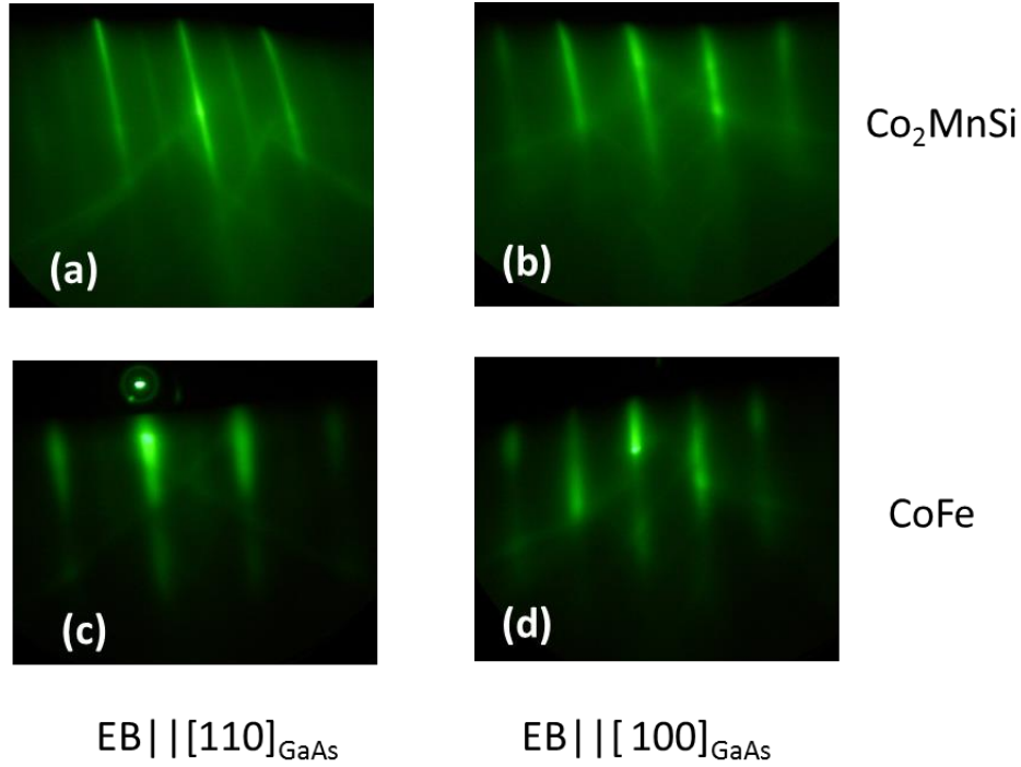
Fig. 3.6. RHEED patterns along the azimuths of [110] GaAs and [100] GaAs for the Co 2 MnSi layer and the CoFe insertion layer. (a) Co 2 MnSi with EB||[110] GaAs , (b) Co 2 MnSi with EB||[100] GaAs , (c) CoFe with EB||[110] GaAs , and (d) CoFe with EB||[100] GaAs .
