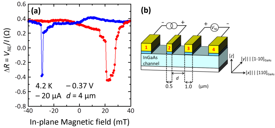
Fig. 4.2. (a) Plot of non-local voltage ( V_{NL} ) divided by injection current ( I ) as a function of in-plane magnetic field for a lateral spin transport device with indium composition x = 4\% . (b) Schematic device structure of a four-terminal lateral spin transport device and circuit configuration for the nonlocal measurement.
