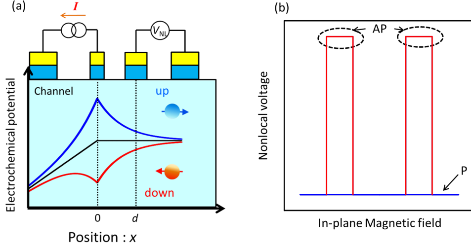
Figure 2.3. (a) Splitting of electro chemical potential for up and down spins. Due to diffusion currents, electron spins flow to the right side direction. (b) Schematic spin-valve signal. P and AP indicate parallel and anti-parallel magnetization configuration for the injector and detector contact.
