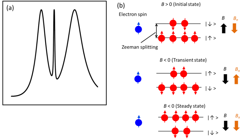
Figure 2.7. Schematic of (a) a transient-state oblique Hanle signal and (b) diagram of nuclear spin moments.
