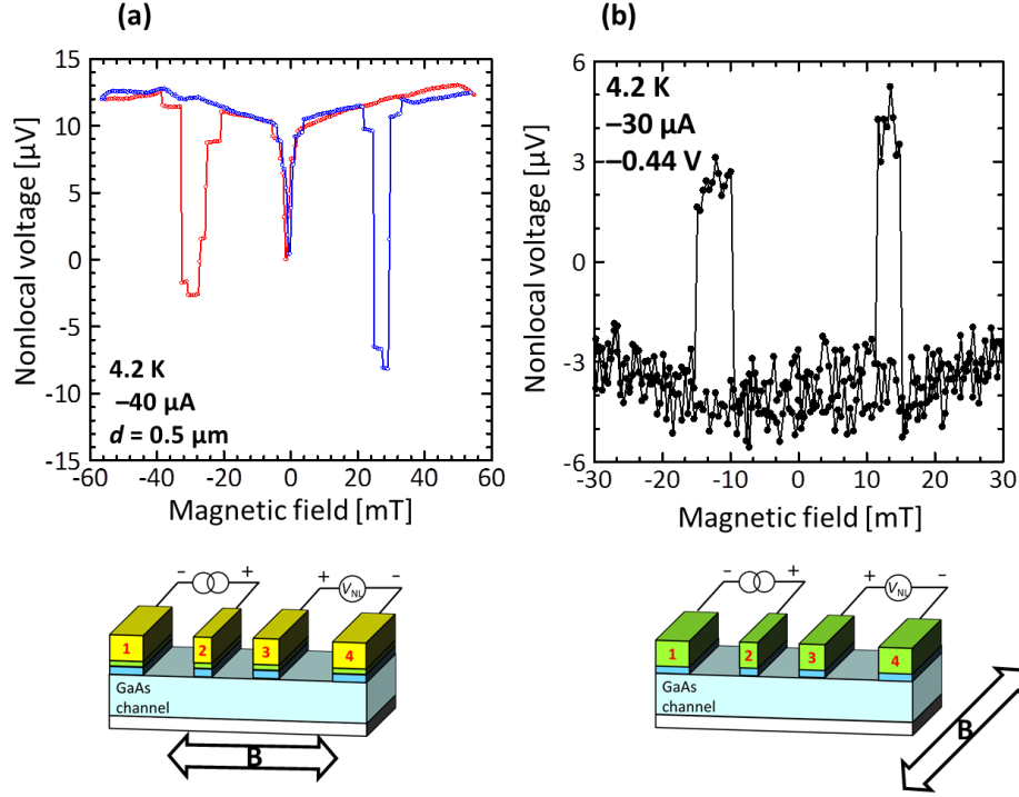
Figure 5.4. (a) Spin-valve signal in the \text{Co}_2\text{MnSi}/\text{CoFe}/\text{n-GaAs} sample. In-plane magnetic field was applied parallel to the x-axis direction. (b) Spin-valve signal in the \text{CoFe}/\text{n-GaAs} sample. In-plane magnetic field was applied parallel to the y-axis direction.
