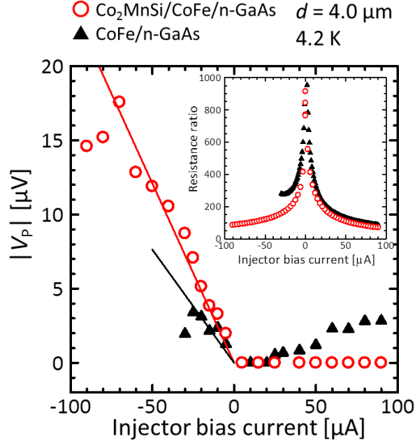
Fig. 3.10. Bias current dependence of V_p measured for a \text{Co}_2\text{MnSi}/\text{CoFe}/\text{n-GaAs} sample and a \text{CoFe}/\text{n-GaAs} reference sample. The solid lines indicate linear least-squares fitting in the low negative-bias region. Inset shows the bias current dependence of the injector junction resistance for both \text{Co}_2\text{MnSi}/\text{CoFe}/\text{n-GaAs}
