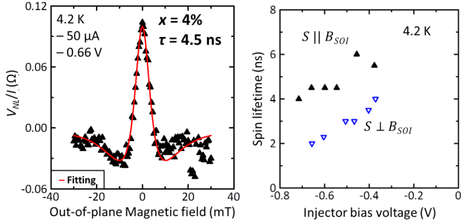
Figure 4.4. (a) Plot of V_{NL}/I as a function of B_z for a device which has the effective magnetic field ( B_{SOI} ) and electron spins ( S ) are parallel configuration ( S \parallel B_{SOI} ). (b) Comparison of bias voltage dependence of spin lifetime for devices with the S \parallel B_{SOI} and the S \perp B_{SOI} configuration.
