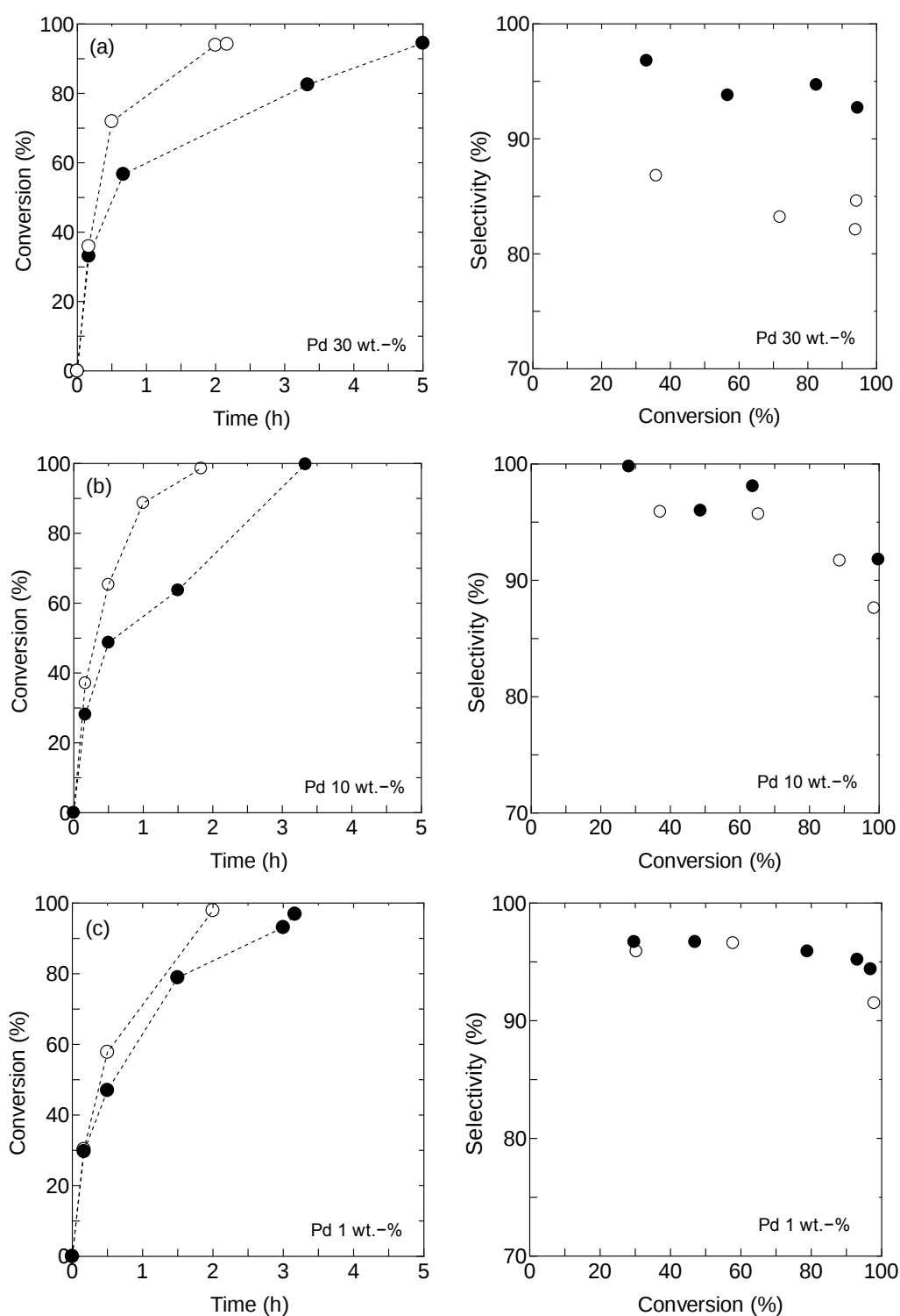
Fig. 1 Conversion – time and styrene selectivity – conversion profiles in hydrogenation of phenylacetylene over Pd (○) and PdZn alloy (●) catalysts including different amounts of Pd on ZnO. Pd loading: (a) 30 wt.-%, (b) 10 wt.-%, (c) 1 wt.-%.
