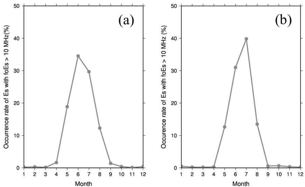
Figure 1.3. Occurrence rate of Es (foEs > 10 MHz) at (a) Kokubunji, 35°N, and (b) Wakkanai, 45°N. foEs data during 2003-2012 and 2004-2012 are used in (a) and (b), respectively.
