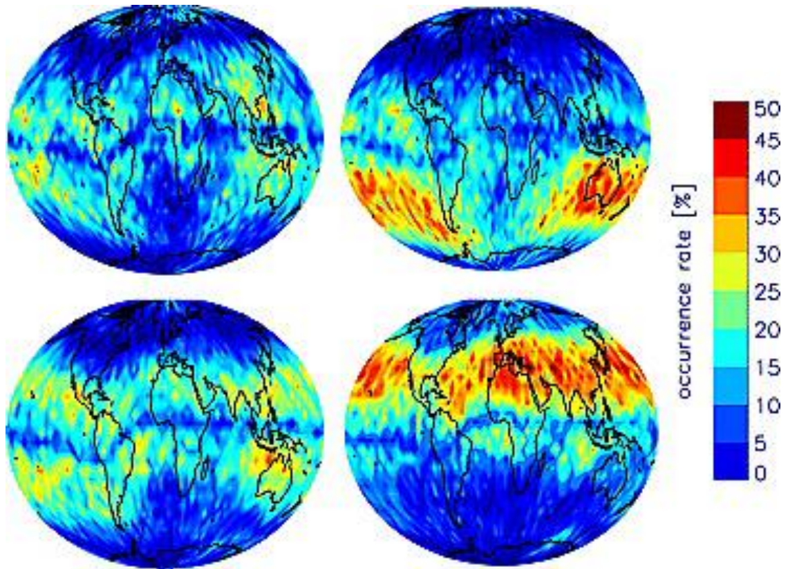
Figure 1.4. Global distribution of Es occurrences retrieved from GPS-RO measurements by low Earth orbiting satellites, such as CHAMP, GRACE, and FORMOSAT-3/COSMIC [Arras et al., 2008]. Panels represent autumn, winter, spring, and summer (in the Northern Hemisphere) in clockwise from top left.
